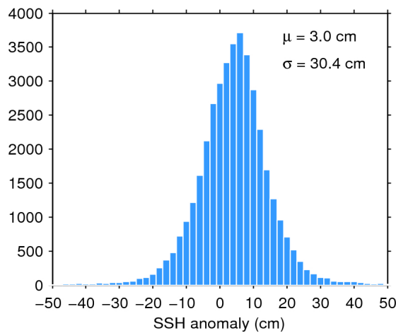
Figure 7. Histogram of flag-valid SSH anomaly over oceans and lakes for 15/06/2020. The mean ( \mu ) and standard deviation ( \sigma ) are also shown. Note that values outside [-50\ 50] cm are excluded from the histogram for the sake of readability but not from the computation of \mu and \sigma .
