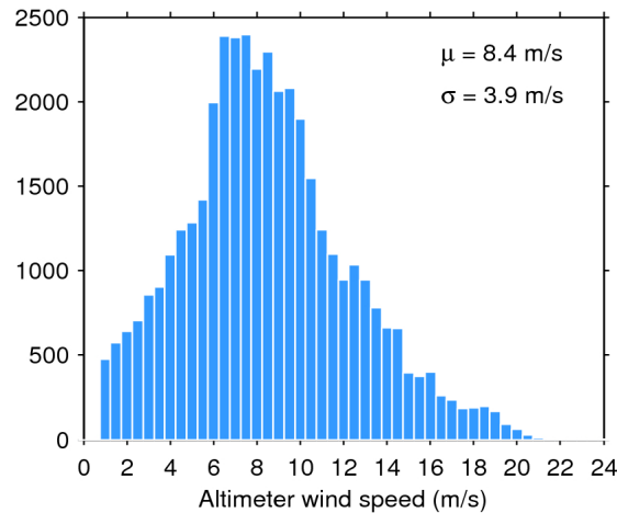
Figure 33. Histogram of flag-valid wind over oceans and lakes for 15/06/2020. The mean ( \mu ) and standard deviation ( \sigma ) are also shown. Note that values larger than 24 m/s are excluded from the histogram for the sake of readability but not from the computation of \mu and \sigma .
