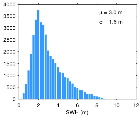
Figure 17. Histogram of flag-valid SWH over oceans and lakes for 15/06/2020. The mean ( \mu ) and standard deviation ( \sigma ) are also shown. Note that values larger than 12 m are excluded from the histogram for the sake of readability but not from the computation of \mu and \sigma .
