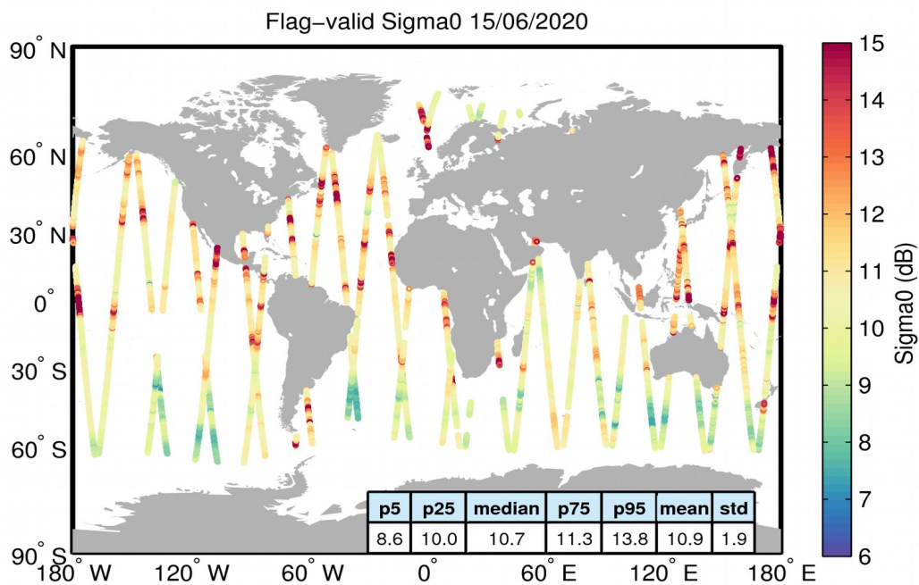
Figure 23. Geographical distribution of flag-valid sigma0 data over oceans and lakes for 15/06/2020. The statistical values shown in the table refer to the sigma0 in dB and are calculated over all measurements shown in the figure.
