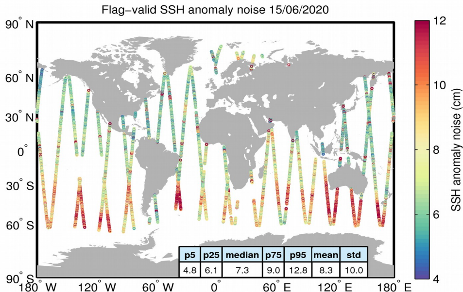
Figure 8. Geographical distribution of flag-valid 20-Hz SSH anomaly measurement noise over oceans and lakes for 15/06/2020. The statistical values shown in the table refer to the SSH anomaly noise and are calculated over all measurements shown in the figure.
