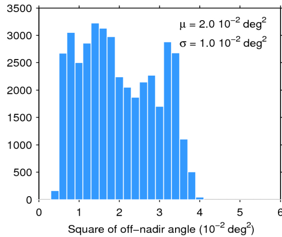
Figure 39. Histogram of flag-valid mispointing over oceans and lakes for 15/06/2020. The mean ( \mu ) and standard deviation ( \sigma ) are also shown. Note that values larger than 6 \cdot 10^{-2} \text{ deg}^2 are excluded from the histogram for the sake of readability but not from the computation of \mu and \sigma .
