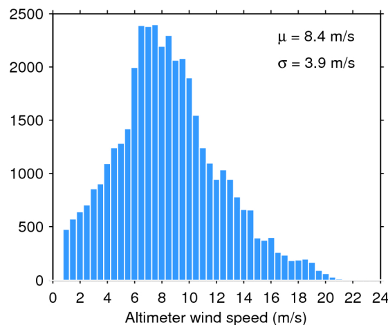
Figure 35. Histogram of science-valid wind over oceans and lakes for 15/06/2020. The mean ( \mu ) and standard deviation ( \sigma ) are also shown. Note that values larger than 24 m/s are excluded from the histogram for the sake of readability but not from the computation of \mu and \sigma .
