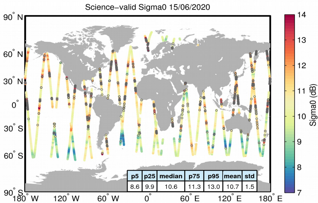
Figure 27. Geographical distribution of science-valid sigma0 data over oceans and lakes for 15/06/2020. The statistical values shown in the table refer to the sigma0 in dB and are calculated over all measurements shown in the figure. Gray circles denote records that have been rejected based on the editing criteria described in Table 4.
