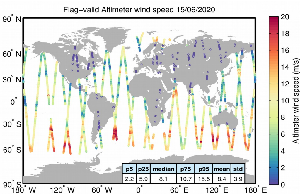
Figure 31. Geographical distribution of flag-valid wind data over oceans and lakes for 15/06/2020. The statistical values shown in the table refer to the wind in m/s and are calculated over all measurements shown in the figure.
