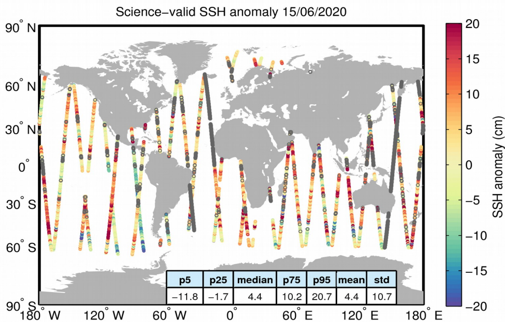
Figure 10. Geographical distribution of science-valid SSH anomaly data over oceans and lakes for 15/06/2020. The statistical values shown in the table refer to the SSH anomaly in cm and are calculated over all measurements shown in the figure. Gray circles denote records that have been rejected based on the editing criteria described in Table 2.
