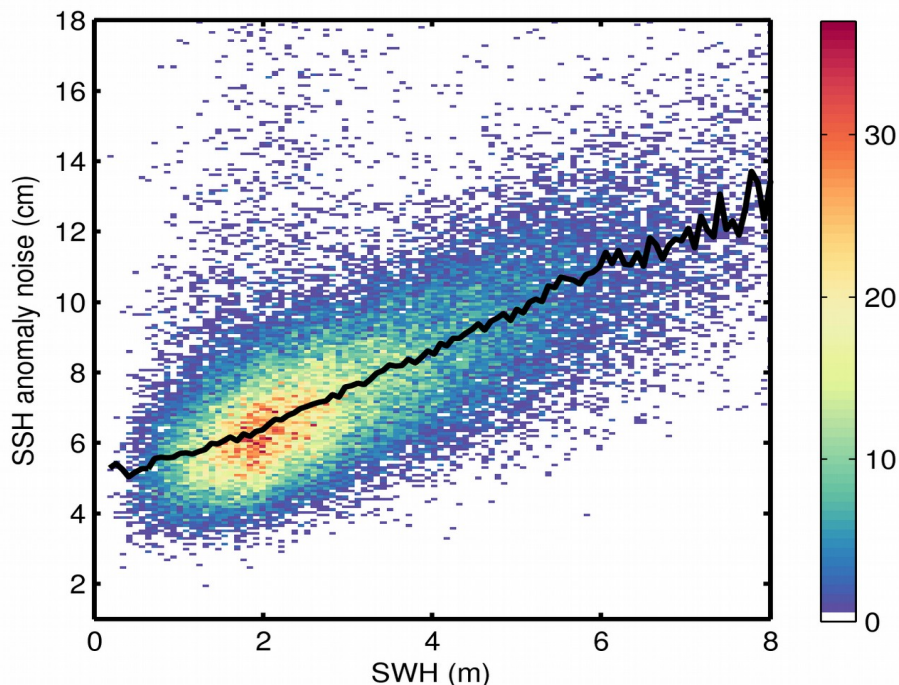
Figure 9. 2D histogram showing flag-valid SSH anomaly noise as a function of SWH for 15/06/2020. The black line denotes the median SSH anomaly noise as a function of SWH.
