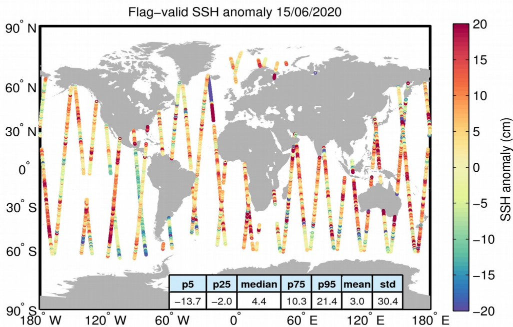
Figure 5. Geographical distribution of flag-valid 1-Hz SSH anomaly data over oceans and lakes for 15/06/2020. The statistical values shown in the table refer to the SSH anomaly in cm and are calculated over all measurements shown in the figure.
