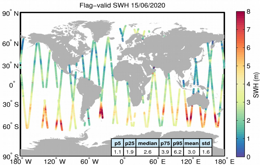
Figure 15. Geographical distribution of flag-valid SWH data over oceans and lakes for 15/06/2020. The statistical values shown in the table refer to the SWH in m and are calculated over all measurements shown in the figure.
