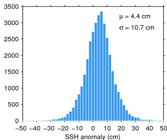
Figure 11. Histogram of science-valid SSH anomaly over oceans and lakes for 15/06/2020. The mean ( \mu ) and standard deviation ( \sigma ) are also shown. Note that values outside [-50 50] cm are excluded from the histogram for the sake of readability but not from the computation of \mu and \sigma .
