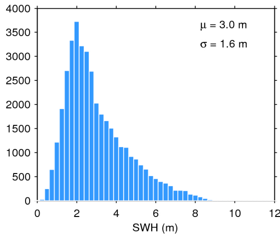
Figure 20. Histogram of science-valid SWH over oceans and lakes for 15/06/2020. The mean ( \mu ) and standard deviation ( \sigma ) are also shown. Note that values larger than 12 m are excluded from the histogram for the sake of readability but not from the computation of \mu and \sigma .
