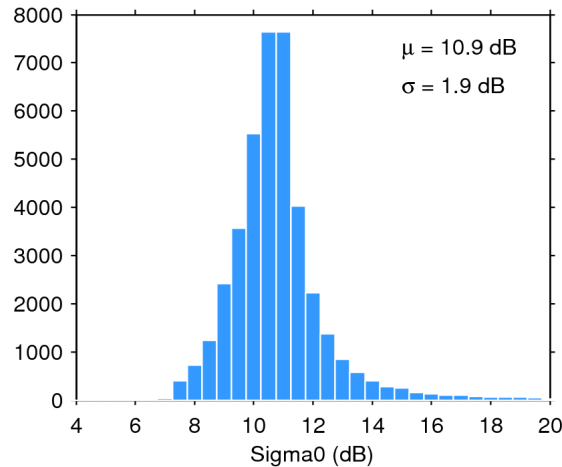
Figure 25. Histogram of flag-valid sigma0 over oceans and lakes for 15/06/2020. The mean ( \mu ) and standard deviation ( \sigma ) are also shown. Note that values outside [4 20] dB are excluded from the histogram for the sake of readability but not from the computation of \mu and \sigma .
