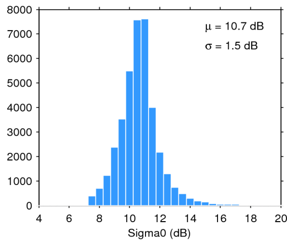
Figure 28. Histogram of science-valid sigma0 over oceans and lakes for 15/06/2020. The mean ( \mu ) and standard deviation ( \sigma ) are also shown. Note that values outside [4 20] dB are excluded from the histogram for the sake of readability but not from the computation of \mu and \sigma .
