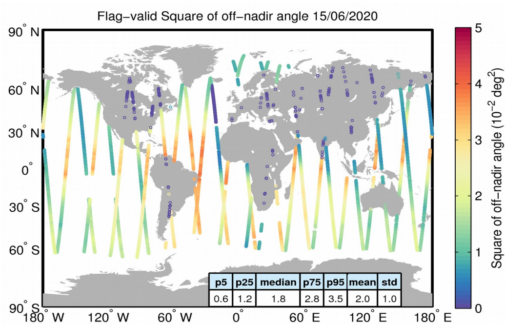
Figure 37. Geographical distribution of flag-valid mispointing data over oceans and lakes for 15/06/2020. The statistical values shown in the table refer to the mispointing in 10^{-2} deg 2 and are calculated over all measurements shown in the figure.
