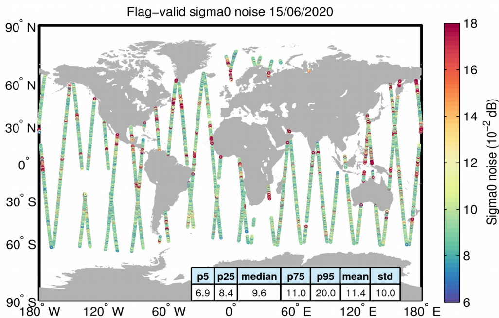
Figure 26. Geographical distribution of flag-valid 20-Hz sigma0 measurement noise over oceans and lakes for 15/06/2020. The statistical values shown in the table refer to the sigma0 noise and are calculated over all measurements shown in the figure.
