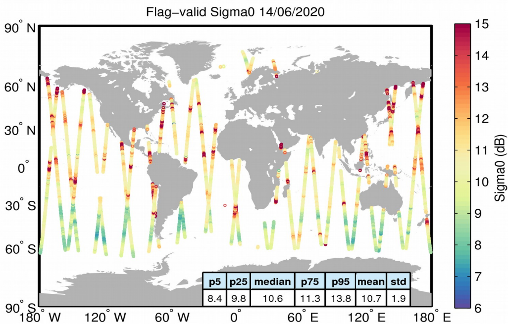
Figure 23. Geographical distribution of flag-valid sigma0 data over oceans and lakes for 14/06/2020. The statistical values shown in the table refer to the sigma0 in dB and are calculated over all measurements shown in the figure.
