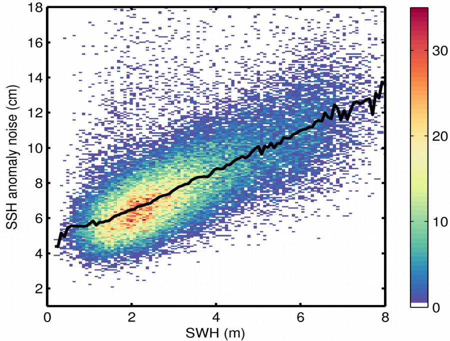
Figure 9. 2D histogram showing flag-valid SSH anomaly noise as a function of SWH for 14/06/2020. The black line denotes the median SSH anomaly noise as a function of SWH.
