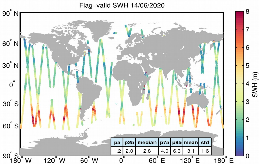
Figure 15. Geographical distribution of flag-valid SWH data over oceans and lakes for 14/06/2020. The statistical values shown in the table refer to the SWH in m and are calculated over all measurements shown in the figure.
