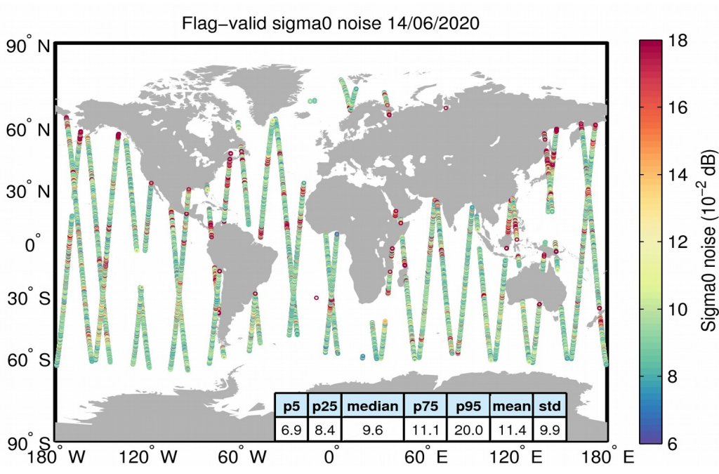
Figure 26. Geographical distribution of flag-valid 20-Hz sigma0 measurement noise over oceans and lakes for 14/06/2020. The statistical values shown in the table refer to the sigma0 noise and are calculated over all measurements shown in the figure.
