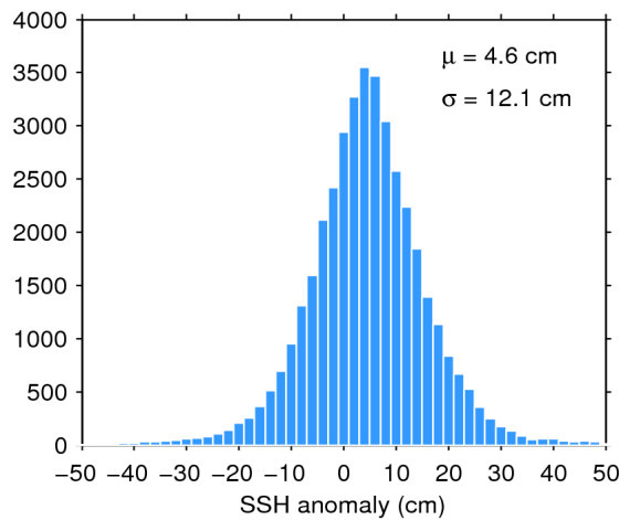
Figure 11. Histogram of science-valid SSH anomaly over oceans and lakes for 14/06/2020. The mean ( \mu ) and standard deviation ( \sigma ) are also shown. Note that values outside [-50 50] cm are excluded from the histogram for the sake of readability but not from the computation of \mu and \sigma .
