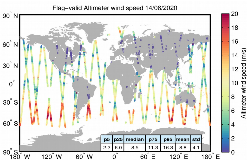
Figure 31. Geographical distribution of flag-valid wind data over oceans and lakes for 14/06/2020. The statistical values shown in the table refer to the wind in m/s and are calculated over all measurements shown in the figure.
