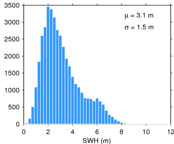
Figure 20. Histogram of science-valid SWH over oceans and lakes for 14/06/2020. The mean ( \mu ) and standard deviation ( \sigma ) are also shown. Note that values larger than 12 m are excluded from the histogram for the sake of readability but not from the computation of \mu and \sigma .
