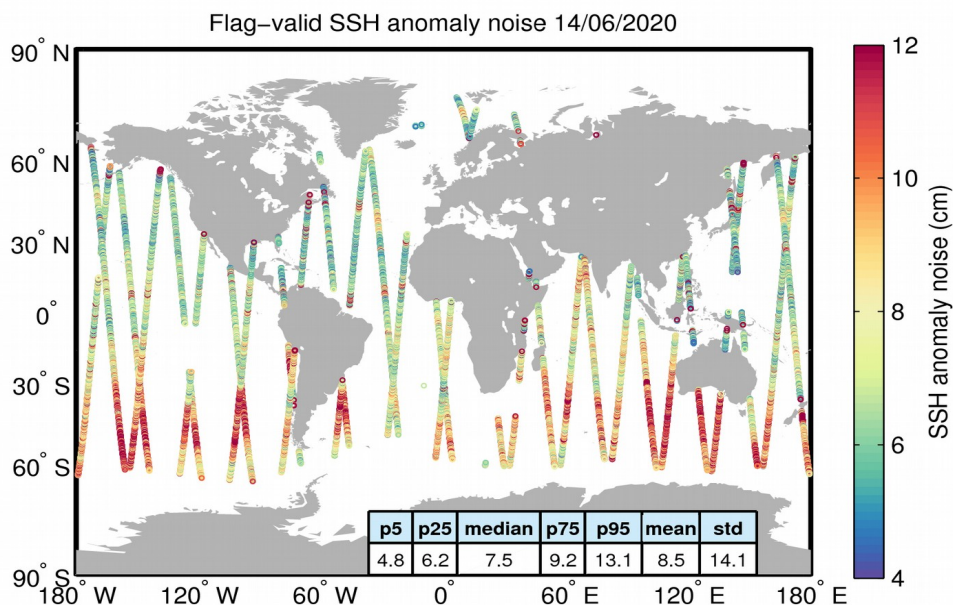
Figure 8. Geographical distribution of flag-valid 20-Hz SSH anomaly measurement noise over oceans and lakes for 14/06/2020. The statistical values shown in the table refer to the SSH anomaly noise and are calculated over all measurements shown in the figure.
