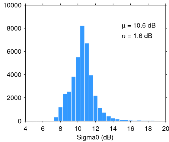
Figure 28. Histogram of science-valid sigma0 over oceans and lakes for 14/06/2020. The mean ( \mu ) and standard deviation ( \sigma ) are also shown. Note that values outside [4 20] dB are excluded from the histogram for the sake of readability but not from the computation of \mu and \sigma .
