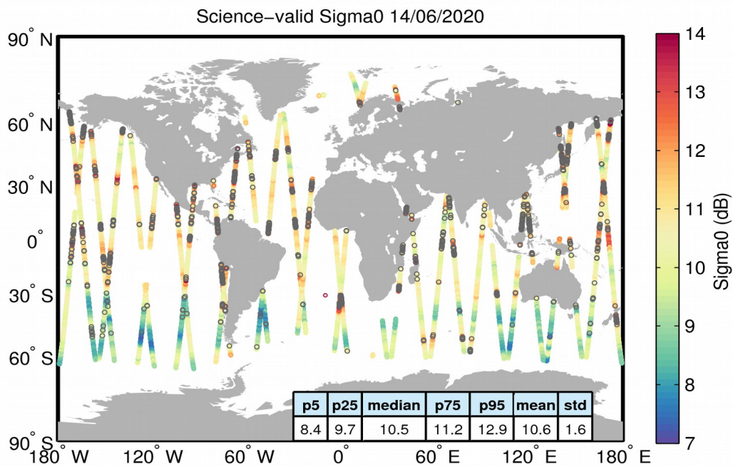
Figure 27. Geographical distribution of science-valid sigma0 data over oceans and lakes for 14/06/2020. The statistical values shown in the table refer to the sigma0 in dB and are calculated over all measurements shown in the figure. Gray circles denote records that have been rejected based on the editing criteria described in Table 4.
