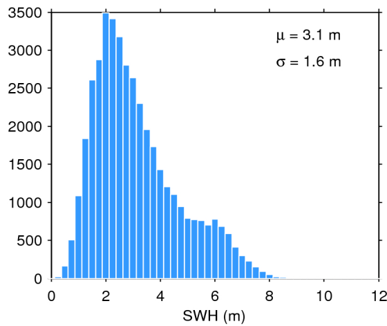
Figure 17. Histogram of flag-valid SWH over oceans and lakes for 14/06/2020. The mean ( \mu ) and standard deviation ( \sigma ) are also shown. Note that values larger than 12 m are excluded from the histogram for the sake of readability but not from the computation of \mu and \sigma .
