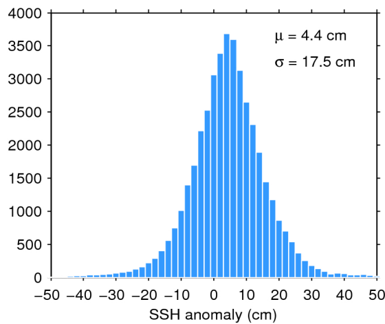
Figure 7. Histogram of flag-valid SSH anomaly over oceans and lakes for 14/06/2020. The mean ( \mu ) and standard deviation ( \sigma ) are also shown. Note that values outside [-50 50] cm are excluded from the histogram for the sake of readability but not from the computation of \mu and \sigma .
