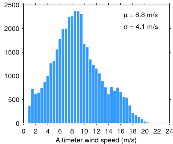
Figure 33. Histogram of flag-valid wind over oceans and lakes for 14/06/2020. The mean ( \mu ) and standard deviation ( \sigma ) are also shown. Note that values larger than 24 m/s are excluded from the histogram for the sake of readability but not from the computation of \mu and \sigma .
