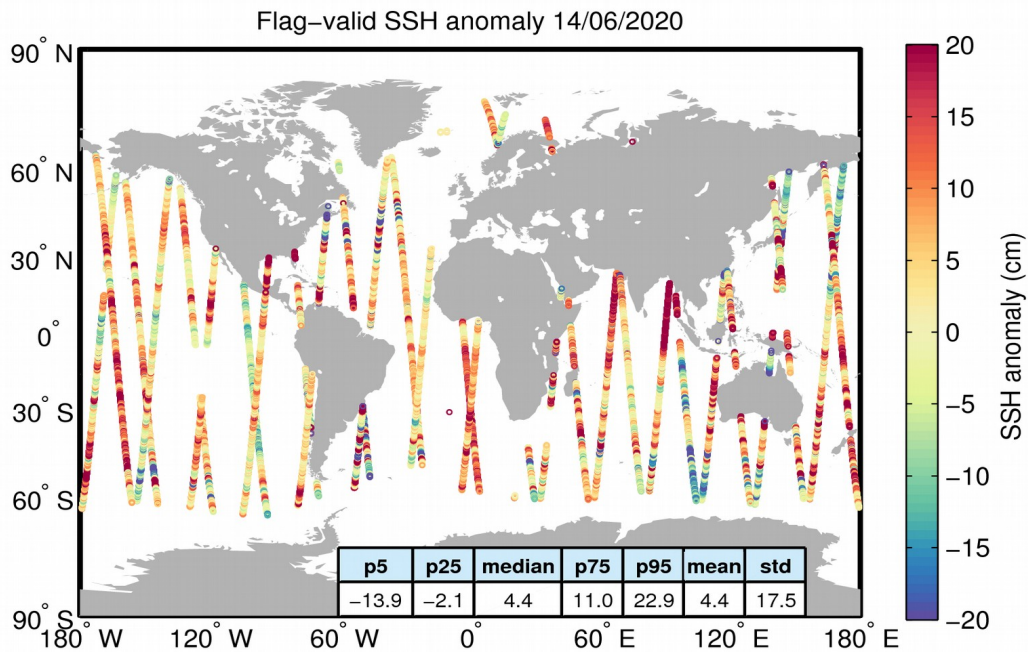
Figure 5. Geographical distribution of flag-valid 1-Hz SSH anomaly data over oceans and lakes for 14/06/2020. The statistical values shown in the table refer to the SSH anomaly in cm and are calculated over all measurements shown in the figure.
