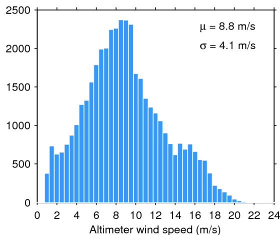
Figure 35. Histogram of science-valid wind over oceans and lakes for 14/06/2020. The mean ( \mu ) and standard deviation ( \sigma ) are also shown. Note that values larger than 24 m/s are excluded from the histogram for the sake of readability but not from the computation of \mu and \sigma .
