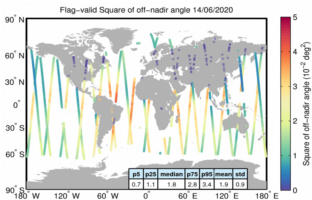
Figure 37. Geographical distribution of flag-valid mispointing data over oceans and lakes for 14/06/2020. The statistical values shown in the table refer to the mispointing in 10^{-2} \text{ deg}^2 and are calculated over all measurements shown in the figure.
