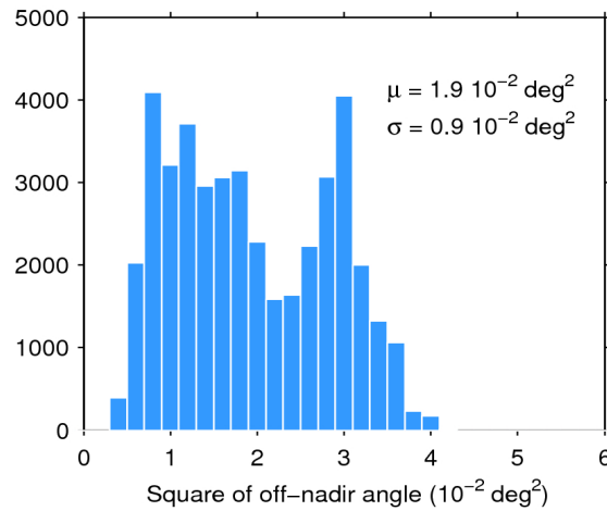
Figure 39. Histogram of flag-valid mispointing over oceans and lakes for 14/06/2020. The mean ( \mu ) and standard deviation ( \sigma ) are also shown. Note that values larger than 6 \cdot 10^{-2} \text{ deg}^2 are excluded from the histogram for the sake of readability but not from the computation of \mu and \sigma .
