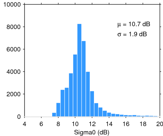
Figure 25. Histogram of flag-valid sigma0 over oceans and lakes for 14/06/2020. The mean ( \mu ) and standard deviation ( \sigma ) are also shown. Note that values outside [4 20] dB are excluded from the histogram for the sake of readability but not from the computation of \mu and \sigma .
