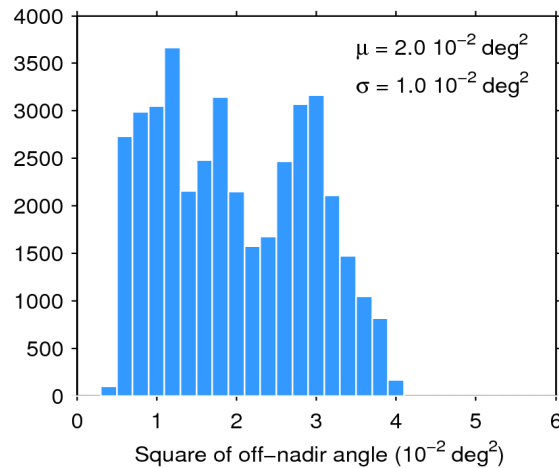
Figure 39. Histogram of flag-valid mispointing over oceans and lakes for 13/06/2020. The mean ( \mu ) and standard deviation ( \sigma ) are also shown. Note that values larger than 6 \cdot 10^{-2} \text{ deg}^2 are excluded from the histogram for the sake of readability but not from the computation of \mu and \sigma .
