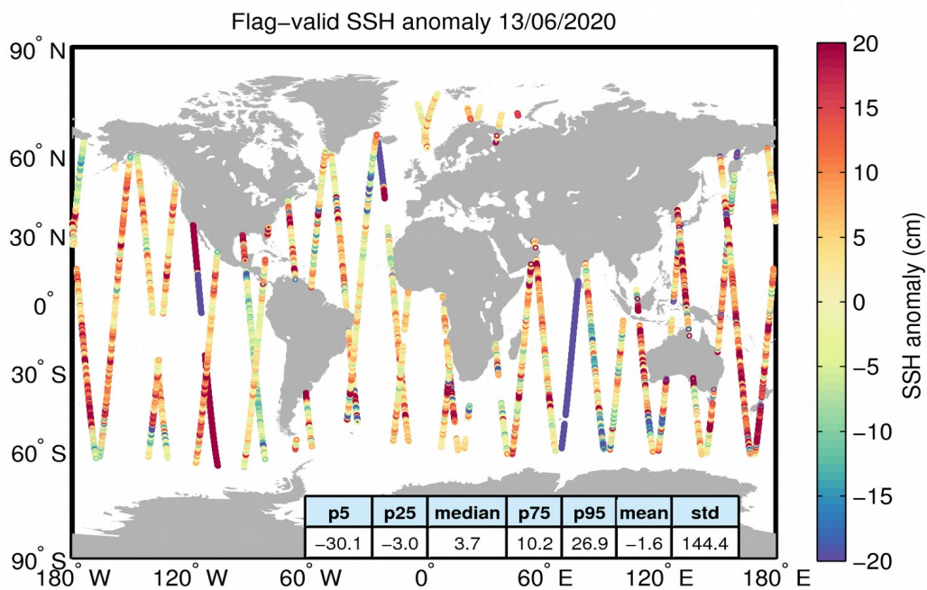
Figure 5. Geographical distribution of flag-valid 1-Hz SSH anomaly data over oceans and lakes for 13/06/2020. The statistical values shown in the table refer to the SSH anomaly in cm and are calculated over all measurements shown in the figure.
