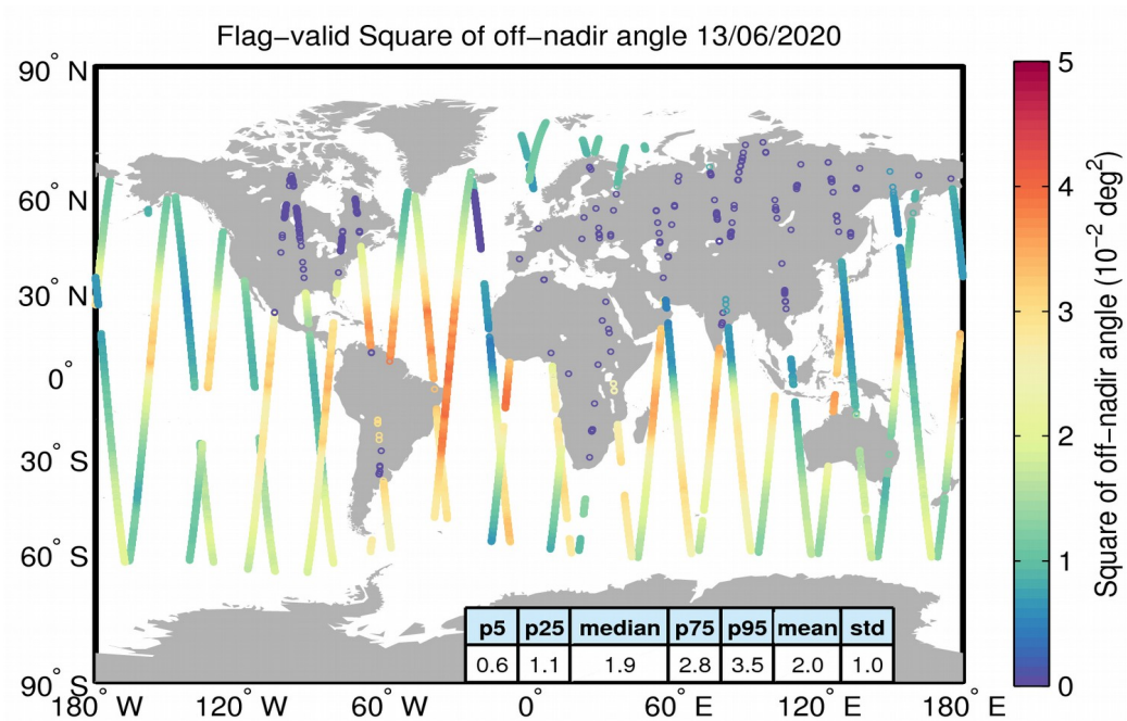
Figure 37. Geographical distribution of flag-valid mispointing data over oceans and lakes for 13/06/2020. The statistical values shown in the table refer to the mispointing in 10^{-2} deg 2 and are calculated over all measurements shown in the figure.
