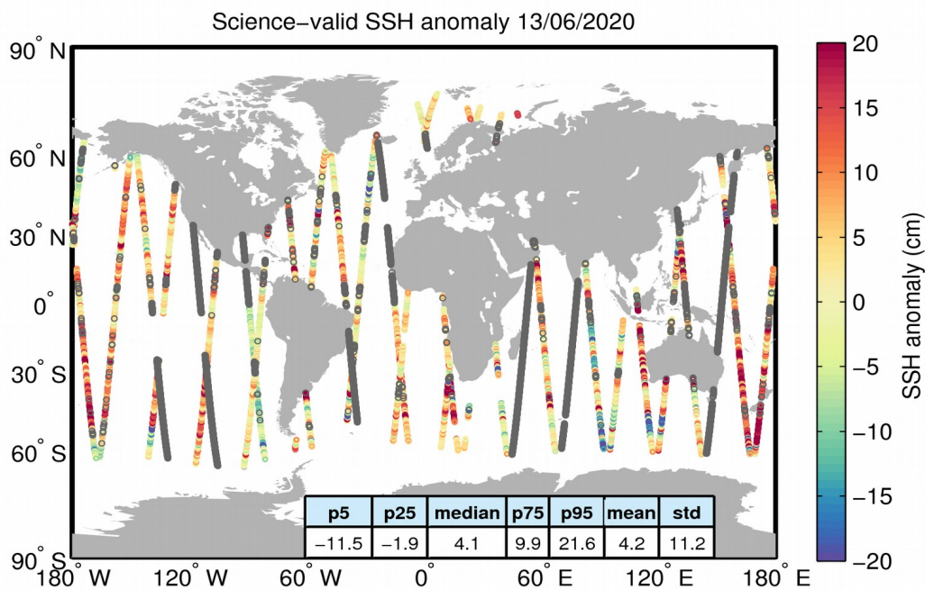
Figure 10. Geographical distribution of science-valid SSH anomaly data over oceans and lakes for 13/06/2020. The statistical values shown in the table refer to the SSH anomaly in cm and are calculated over all measurements shown in the figure. Gray circles denote records that have been rejected based on the editing criteria described in Table 2.
