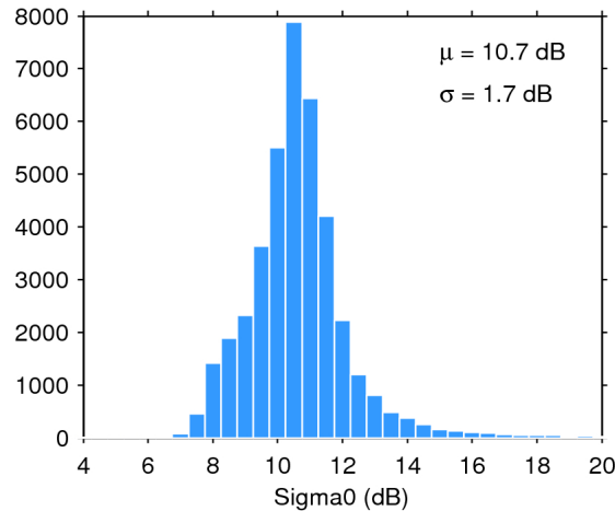
Figure 25. Histogram of flag-valid sigma0 over oceans and lakes for 13/06/2020. The mean ( \mu ) and standard deviation ( \sigma ) are also shown. Note that values outside [4 20] dB are excluded from the histogram for the sake of readability but not from the computation of \mu and \sigma .
