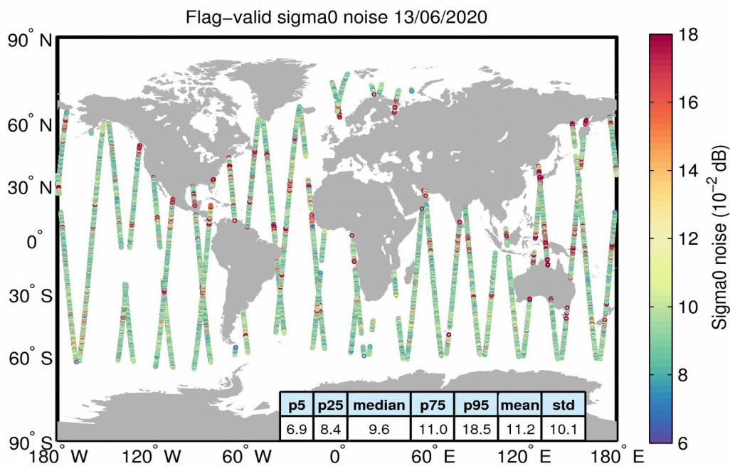
Figure 26. Geographical distribution of flag-valid 20-Hz sigma0 measurement noise over oceans and lakes for 13/06/2020. The statistical values shown in the table refer to the sigma0 noise and are calculated over all measurements shown in the figure.
