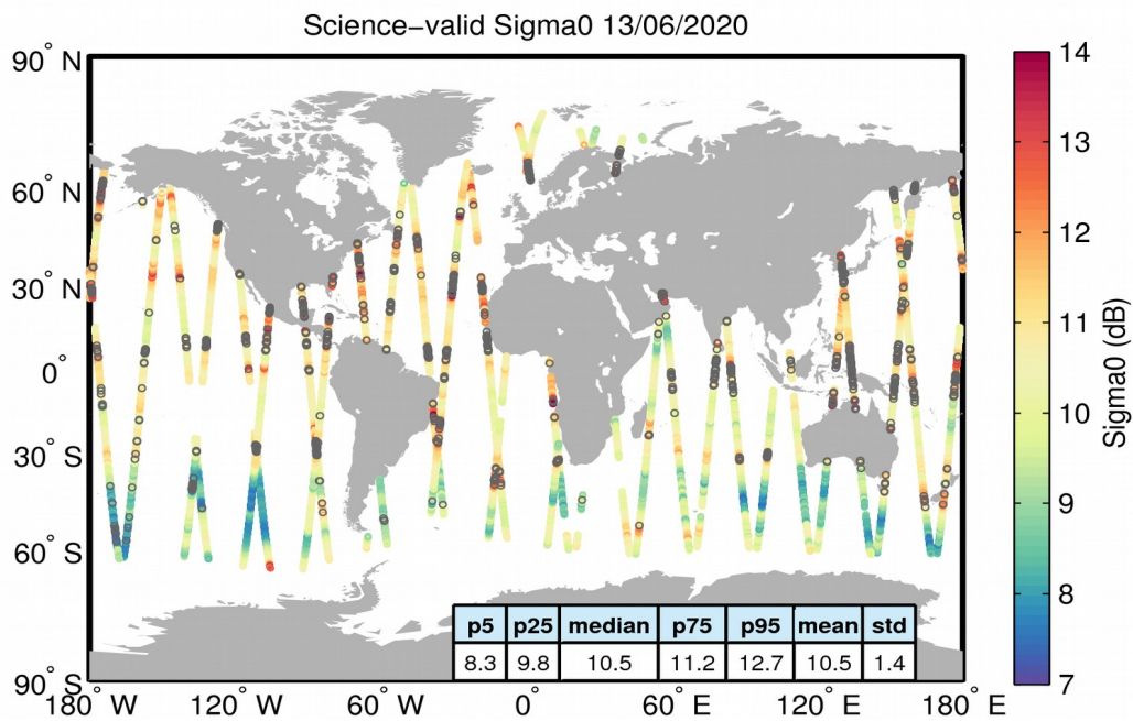
Figure 27. Geographical distribution of science-valid sigma0 data over oceans and lakes for 13/06/2020. The statistical values shown in the table refer to the sigma0 in dB and are calculated over all measurements shown in the figure. Gray circles denote records that have been rejected based on the editing criteria described in Table 4.
