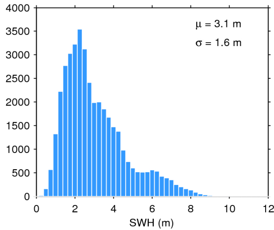
Figure 17. Histogram of flag-valid SWH over oceans and lakes for 13/06/2020. The mean ( \mu ) and standard deviation ( \sigma ) are also shown. Note that values larger than 12 m are excluded from the histogram for the sake of readability but not from the computation of \mu and \sigma .
