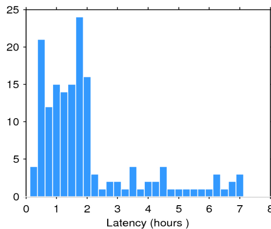
Figure 2. Histogram of the data latency for 13/06/2020. The y-axis denotes the number of files that are made available with a delay of x-hours with respect to the mean time of the records stored in the file.
