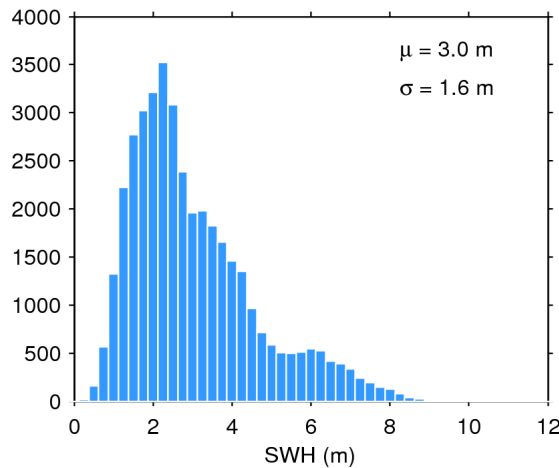
Figure 20. Histogram of science-valid SWH over oceans and lakes for 13/06/2020. The mean ( \mu ) and standard deviation ( \sigma ) are also shown. Note that values larger than 12 m are excluded from the histogram for the sake of readability but not from the computation of \mu and \sigma .
