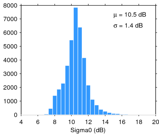
Figure 28. Histogram of science-valid sigma0 over oceans and lakes for 13/06/2020. The mean ( \mu ) and standard deviation ( \sigma ) are also shown. Note that values outside [4 20] dB are excluded from the histogram for the sake of readability but not from the computation of \mu and \sigma .
