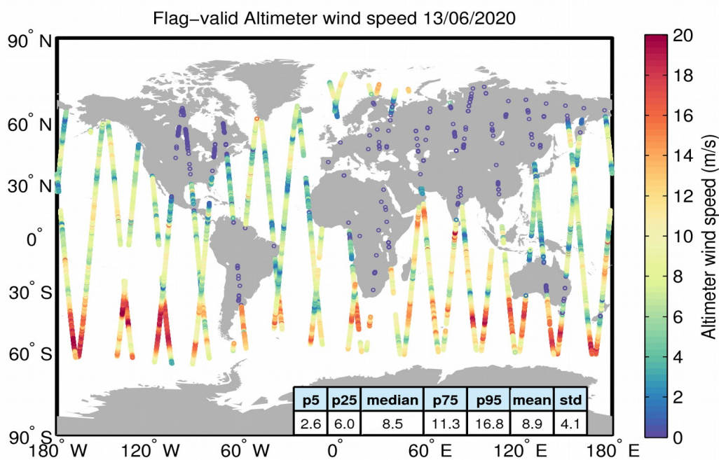
Figure 31. Geographical distribution of flag-valid wind data over oceans and lakes for 13/06/2020. The statistical values shown in the table refer to the wind in m/s and are calculated over all measurements shown in the figure.
