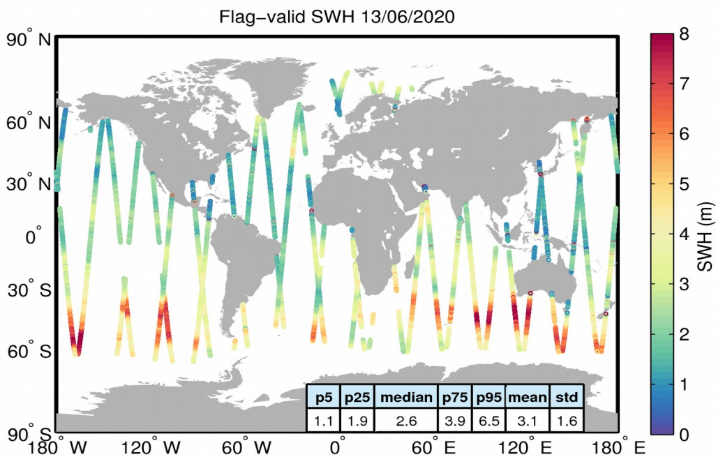
Figure 15. Geographical distribution of flag-valid SWH data over oceans and lakes for 13/06/2020. The statistical values shown in the table refer to the SWH in m and are calculated over all measurements shown in the figure.
