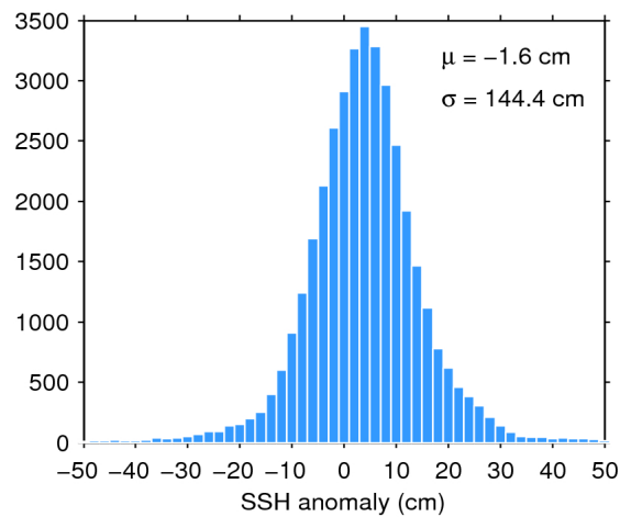
Figure 7. Histogram of flag-valid SSH anomaly over oceans and lakes for 13/06/2020. The mean ( \mu ) and standard deviation ( \sigma ) are also shown. Note that values outside [-50 50] cm are excluded from the histogram for the sake of readability but not from the computation of \mu and \sigma .
