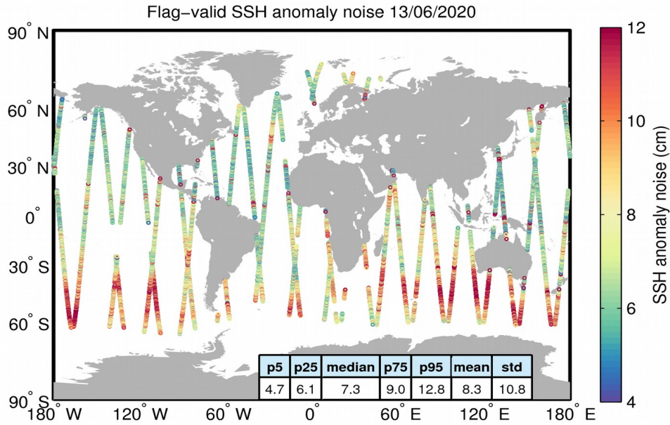
Figure 8. Geographical distribution of flag-valid 20-Hz SSH anomaly measurement noise over oceans and lakes for 13/06/2020. The statistical values shown in the table refer to the SSH anomaly noise and are calculated over all measurements shown in the figure.
