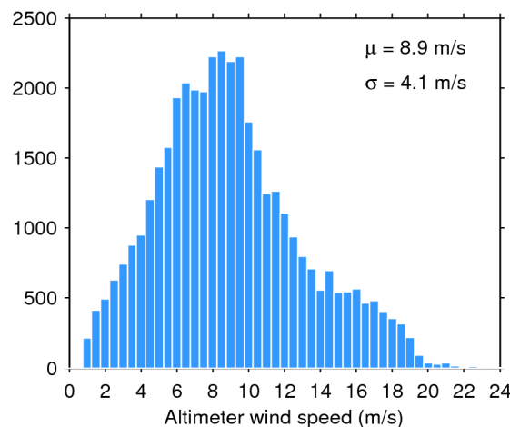
Figure 35. Histogram of science-valid wind over oceans and lakes for 13/06/2020. The mean ( \mu ) and standard deviation ( \sigma ) are also shown. Note that values larger than 24 m/s are excluded from the histogram for the sake of readability but not from the computation of \mu and \sigma .
