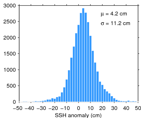
Figure 11. Histogram of science-valid SSH anomaly over oceans and lakes for 13/06/2020. The mean ( \mu ) and standard deviation ( \sigma ) are also shown. Note that values outside [-50 50] cm are excluded from the histogram for the sake of readability but not from the computation of \mu and \sigma .
