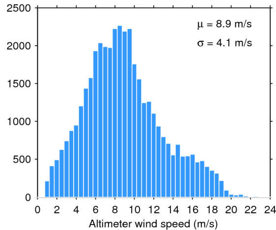
Figure 33. Histogram of flag-valid wind over oceans and lakes for 13/06/2020. The mean ( \mu ) and standard deviation ( \sigma ) are also shown. Note that values larger than 24 m/s are excluded from the histogram for the sake of readability but not from the computation of \mu and \sigma .
