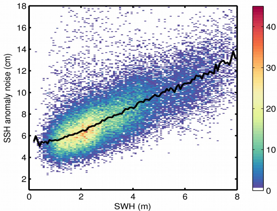
Figure 9. 2D histogram showing flag-valid SSH anomaly noise as a function of SWH for 13/06/2020. The black line denotes the median SSH anomaly noise as a function of SWH.
