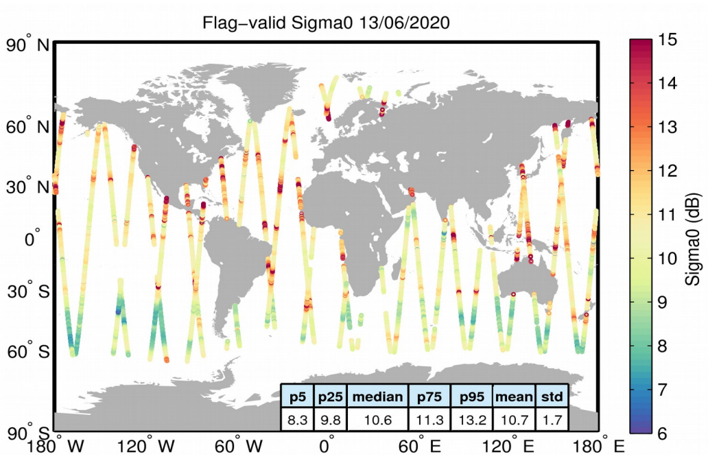
Figure 23. Geographical distribution of flag-valid sigma0 data over oceans and lakes for 13/06/2020. The statistical values shown in the table refer to the sigma0 in dB and are calculated over all measurements shown in the figure.
