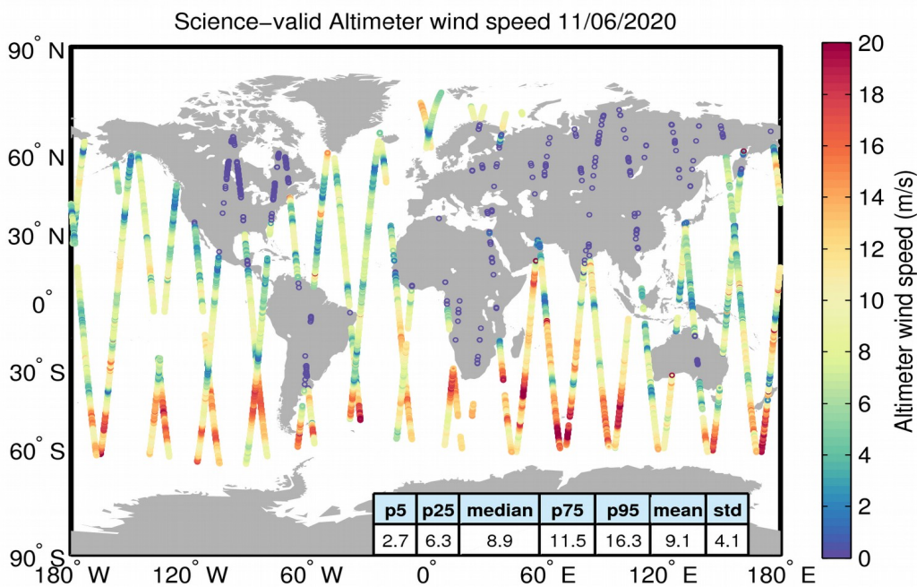
Figure 34. Geographical distribution of science-valid wind data over oceans and lakes for 11/06/2020. The statistical values shown in the table refer to the wind in m/s and are calculated over all measurements shown in the figure. Gray circles denote records that have been rejected based on the editing criteria described in Table 5.
