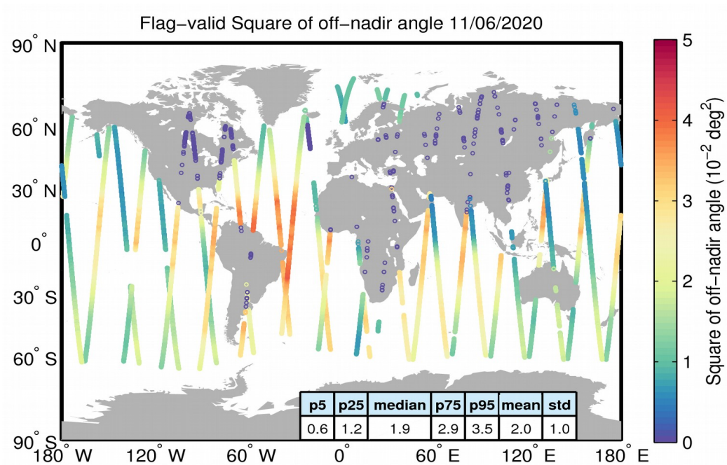
Figure 37. Geographical distribution of flag-valid mispointing data over oceans and lakes for 11/06/2020. The statistical values shown in the table refer to the mispointing in 10^{-2} \text{ deg}^2 and are calculated over all measurements shown in the figure.
