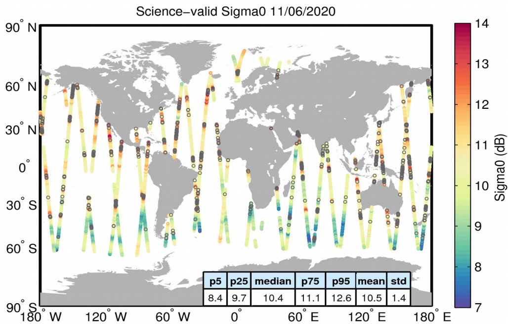
Figure 27. Geographical distribution of science-valid sigma0 data over oceans and lakes for 11/06/2020. The statistical values shown in the table refer to the sigma0 in dB and are calculated over all measurements shown in the figure. Gray circles denote records that have been rejected based on the editing criteria described in Table 4.
