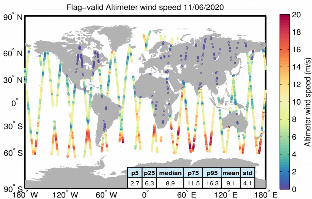
Figure 31. Geographical distribution of flag-valid wind data over oceans and lakes for 11/06/2020. The statistical values shown in the table refer to the wind in m/s and are calculated over all measurements shown in the figure.
