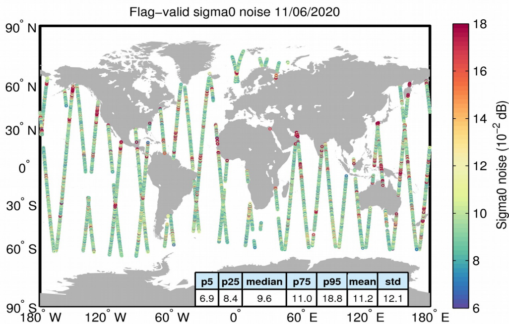
Figure 26. Geographical distribution of flag-valid 20-Hz sigma0 measurement noise over oceans and lakes for 11/06/2020. The statistical values shown in the table refer to the sigma0 noise and are calculated over all measurements shown in the figure.
