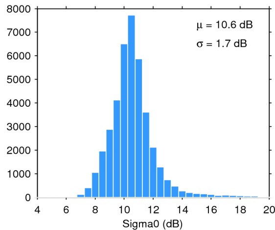
Figure 25. Histogram of flag-valid sigma0 over oceans and lakes for 11/06/2020. The mean ( \mu ) and standard deviation ( \sigma ) are also shown. Note that values outside [4 20] dB are excluded from the histogram for the sake of readability but not from the computation of \mu and \sigma .
