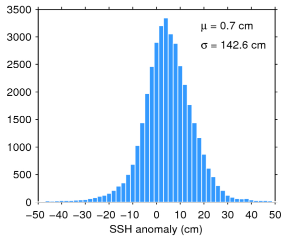
Figure 7. Histogram of flag-valid SSH anomaly over oceans and lakes for 11/06/2020. The mean ( \mu ) and standard deviation ( \sigma ) are also shown. Note that values outside [-50 50] cm are excluded from the histogram for the sake of readability but not from the computation of \mu and \sigma .
