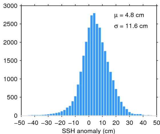
Figure 11. Histogram of science-valid SSH anomaly over oceans and lakes for 11/06/2020. The mean ( \mu ) and standard deviation ( \sigma ) are also shown. Note that values outside [-50 50] cm are excluded from the histogram for the sake of readability but not from the computation of \mu and \sigma .
