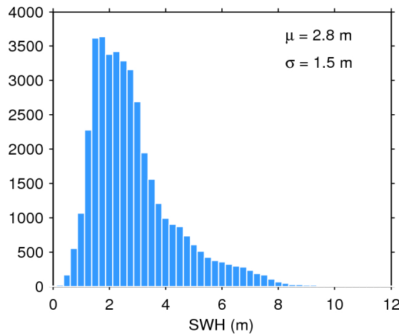
Figure 20. Histogram of science-valid SWH over oceans and lakes for 11/06/2020. The mean ( \mu ) and standard deviation ( \sigma ) are also shown. Note that values larger than 12 m are excluded from the histogram for the sake of readability but not from the computation of \mu and \sigma .
