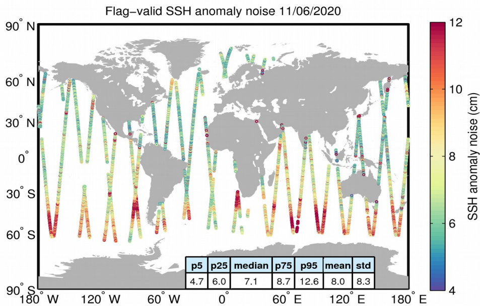
Figure 8. Geographical distribution of flag-valid 20-Hz SSH anomaly measurement noise over oceans and lakes for 11/06/2020. The statistical values shown in the table refer to the SSH anomaly noise and are calculated over all measurements shown in the figure.
