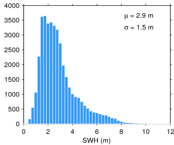
Figure 17. Histogram of flag-valid SWH over oceans and lakes for 11/06/2020. The mean ( \mu ) and standard deviation ( \sigma ) are also shown. Note that values larger than 12 m are excluded from the histogram for the sake of readability but not from the computation of \mu and \sigma .
