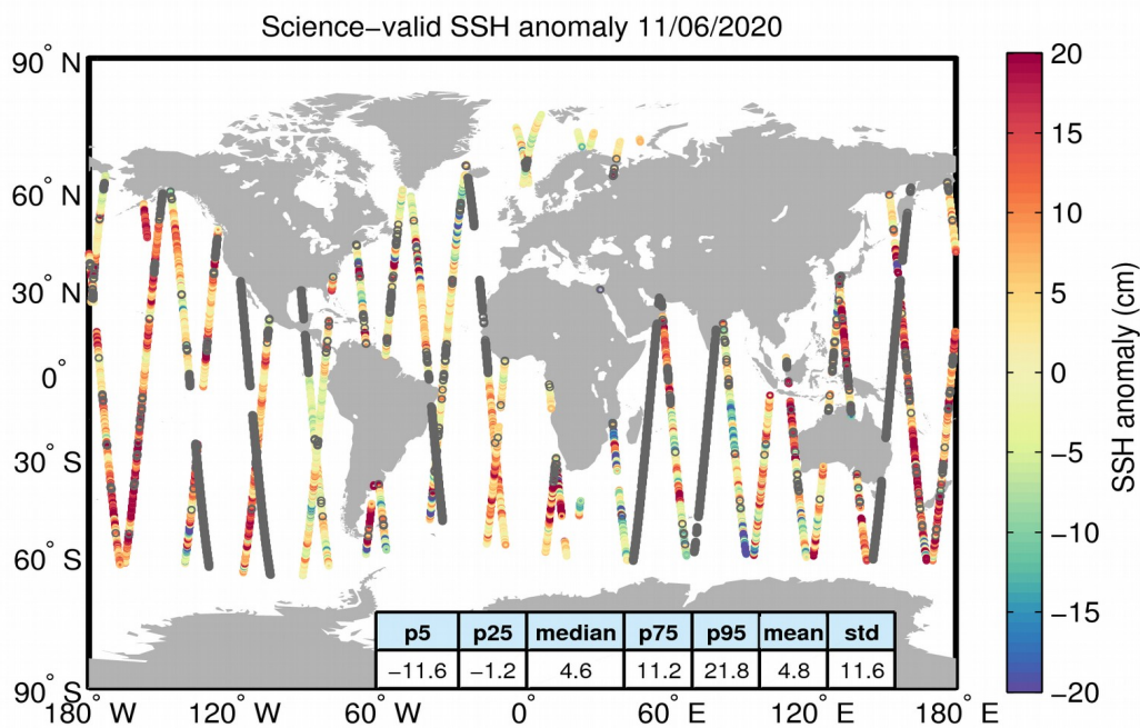
Figure 10. Geographical distribution of science-valid SSH anomaly data over oceans and lakes for 11/06/2020. The statistical values shown in the table refer to the SSH anomaly in cm and are calculated over all measurements shown in the figure. Gray circles denote records that have been rejected based on the editing criteria described in Table 2.
