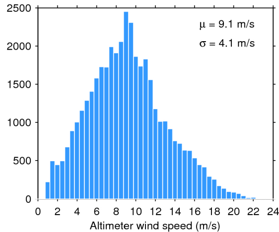
Figure 33. Histogram of flag-valid wind over oceans and lakes for 11/06/2020. The mean ( \mu ) and standard deviation ( \sigma ) are also shown. Note that values larger than 24 m/s are excluded from the histogram for the sake of readability but not from the computation of \mu and \sigma .
