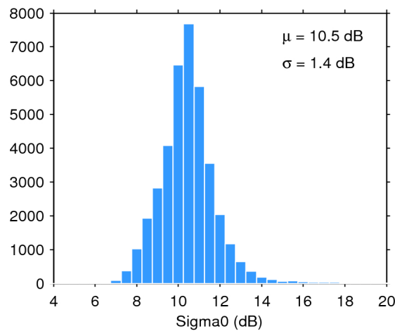
Figure 28. Histogram of science-valid sigma0 over oceans and lakes for 11/06/2020. The mean ( \mu ) and standard deviation ( \sigma ) are also shown. Note that values outside [4 20] dB are excluded from the histogram for the sake of readability but not from the computation of \mu and \sigma .
