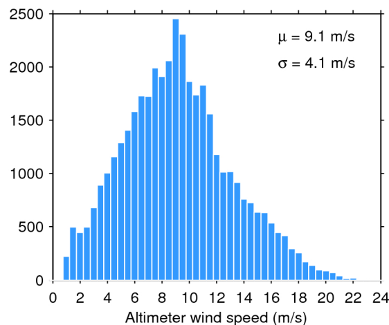
Figure 35. Histogram of science-valid wind over oceans and lakes for 11/06/2020. The mean ( \mu ) and standard deviation ( \sigma ) are also shown. Note that values larger than 24 m/s are excluded from the histogram for the sake of readability but not from the computation of \mu and \sigma .
