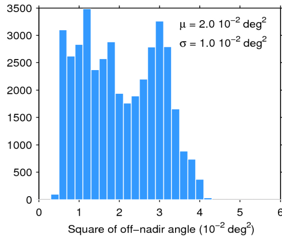
Figure 39. Histogram of flag-valid mispointing over oceans and lakes for 11/06/2020. The mean ( \mu ) and standard deviation ( \sigma ) are also shown. Note that values larger than 6 \cdot 10^{-2} \text{ deg}^2 are excluded from the histogram for the sake of readability but not from the computation of \mu and \sigma .
