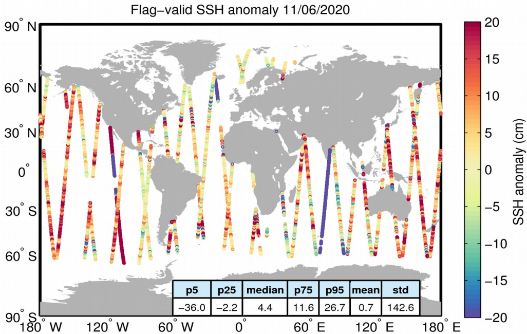
Figure 5. Geographical distribution of flag-valid 1-Hz SSH anomaly data over oceans and lakes for 11/06/2020. The statistical values shown in the table refer to the SSH anomaly in cm and are calculated over all measurements shown in the figure.
