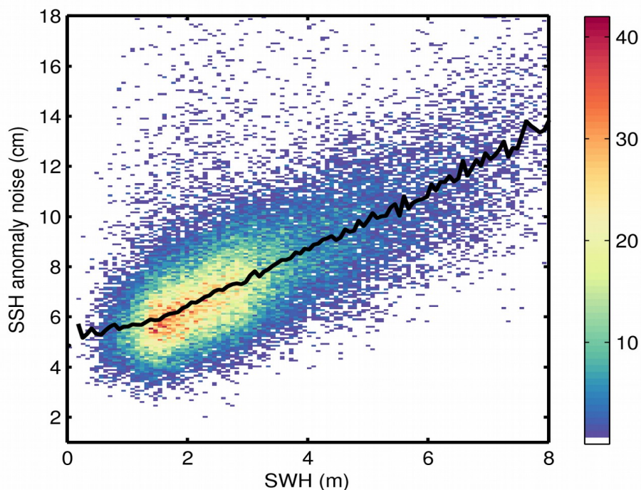
Figure 9. 2D histogram showing flag-valid SSH anomaly noise as a function of SWH for 11/06/2020. The black line denotes the median SSH anomaly noise as a function of SWH.
