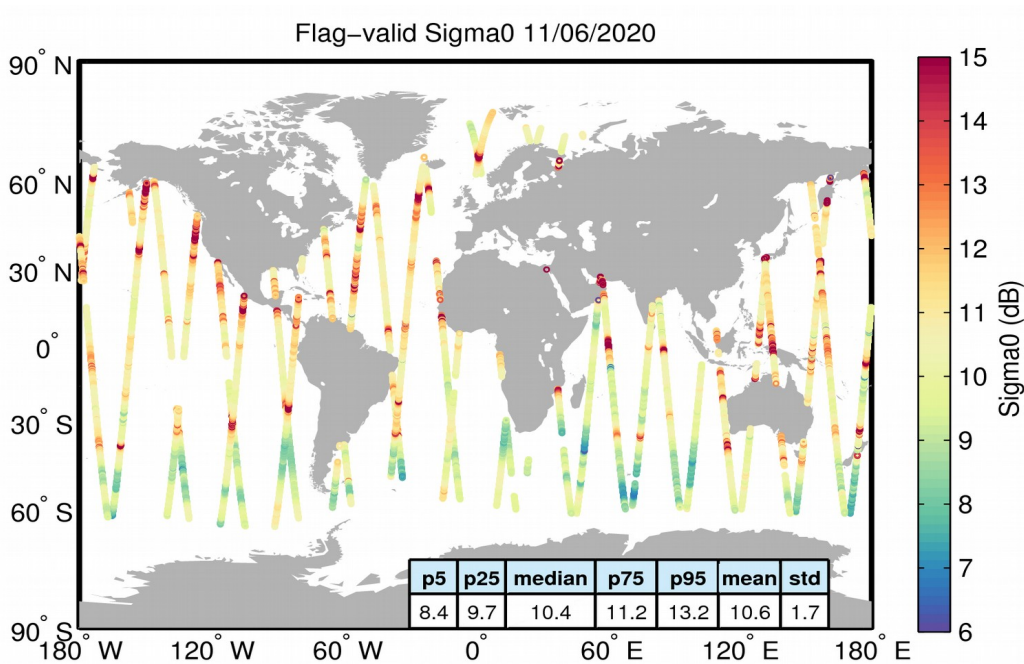
Figure 23. Geographical distribution of flag-valid sigma0 data over oceans and lakes for 11/06/2020. The statistical values shown in the table refer to the sigma0 in dB and are calculated over all measurements shown in the figure.
