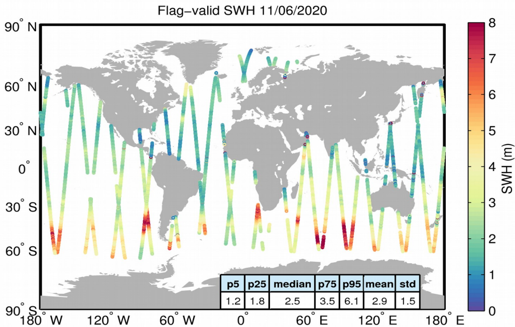
Figure 15. Geographical distribution of flag-valid SWH data over oceans and lakes for 11/06/2020. The statistical values shown in the table refer to the SWH in m and are calculated over all measurements shown in the figure.
