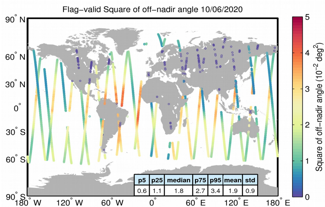
Figure 37. Geographical distribution of flag-valid mispointing data over oceans and lakes for 10/06/2020. The statistical values shown in the table refer to the mispointing in 10^{-2} deg 2 and are calculated over all measurements shown in the figure.
