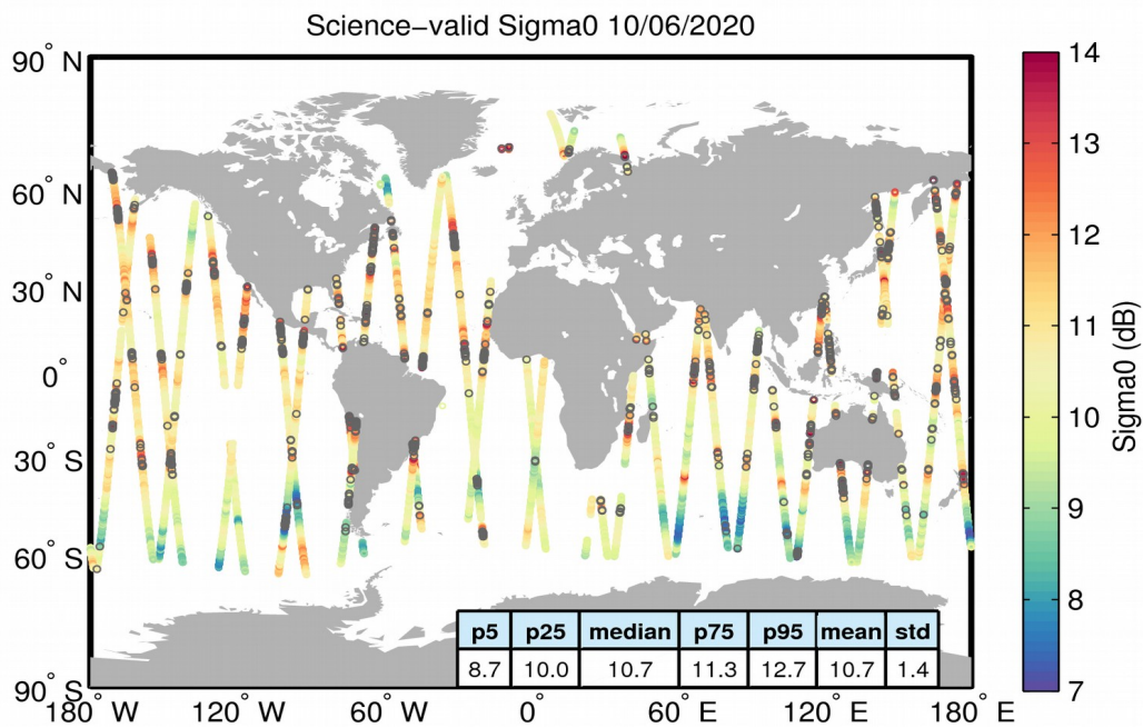
Figure 27. Geographical distribution of science-valid sigma0 data over oceans and lakes for 10/06/2020. The statistical values shown in the table refer to the sigma0 in dB and are calculated over all measurements shown in the figure. Gray circles denote records that have been rejected based on the editing criteria described in Table 4.
