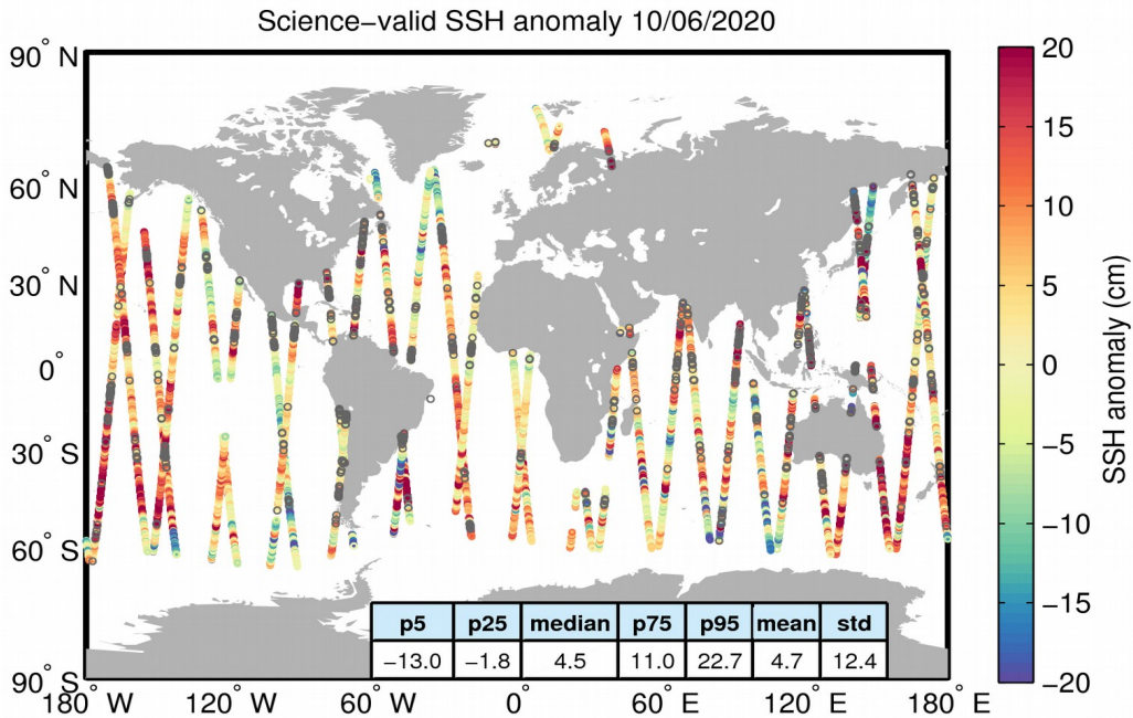
Figure 10. Geographical distribution of science-valid SSH anomaly data over oceans and lakes for 10/06/2020. The statistical values shown in the table refer to the SSH anomaly in cm and are calculated over all measurements shown in the figure. Gray circles denote records that have been rejected based on the editing criteria described in Table 2.
