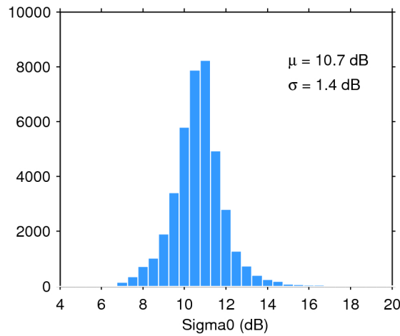
Figure 28. Histogram of science-valid sigma0 over oceans and lakes for 10/06/2020. The mean ( \mu ) and standard deviation ( \sigma ) are also shown. Note that values outside [4 20] dB are excluded from the histogram for the sake of readability but not from the computation of \mu and \sigma .
