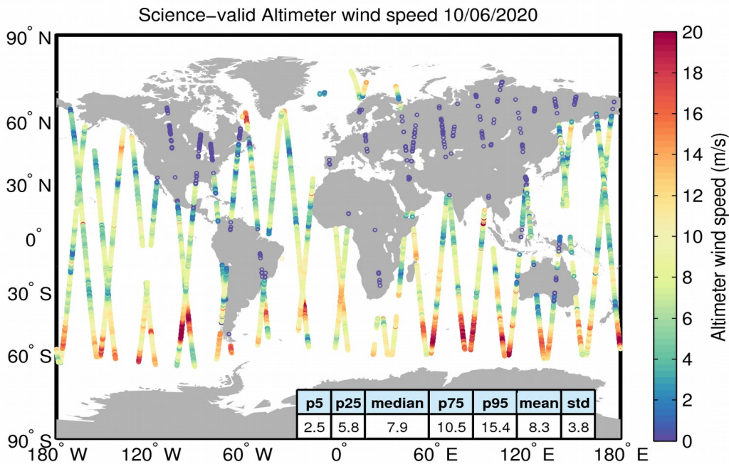
Figure 34. Geographical distribution of science-valid wind data over oceans and lakes for 10/06/2020. The statistical values shown in the table refer to the wind in m/s and are calculated over all measurements shown in the figure. Gray circles denote records that have been rejected based on the editing criteria described in Table 5.
