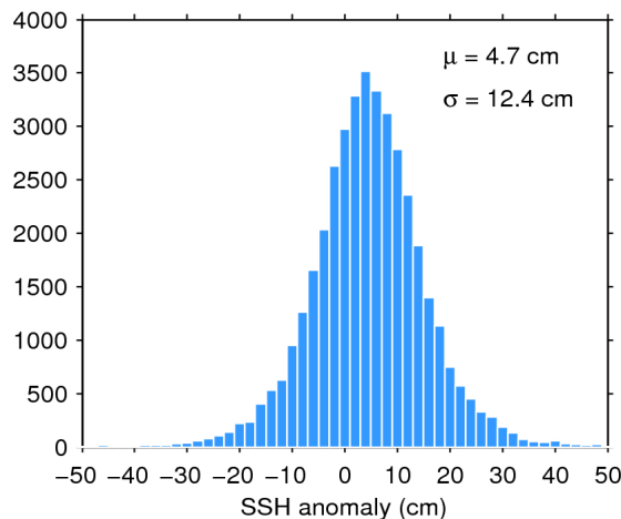
Figure 11. Histogram of science-valid SSH anomaly over oceans and lakes for 10/06/2020. The mean ( \mu ) and standard deviation ( \sigma ) are also shown. Note that values outside [-50 50] cm are excluded from the histogram for the sake of readability but not from the computation of \mu and \sigma .
