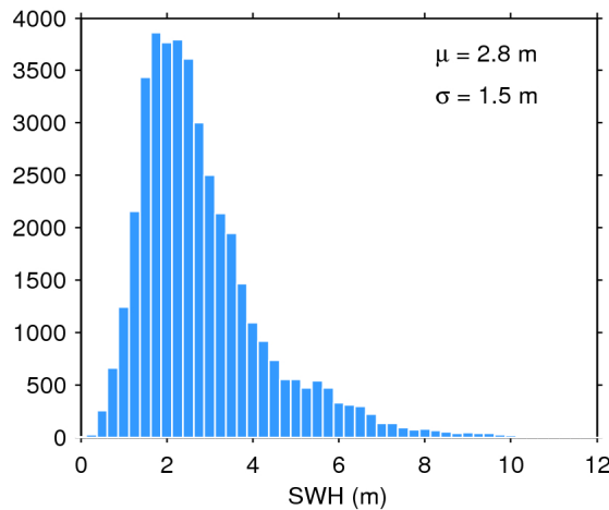
Figure 20. Histogram of science-valid SWH over oceans and lakes for 10/06/2020. The mean ( \mu ) and standard deviation ( \sigma ) are also shown. Note that values larger than 12 m are excluded from the histogram for the sake of readability but not from the computation of \mu and \sigma .
