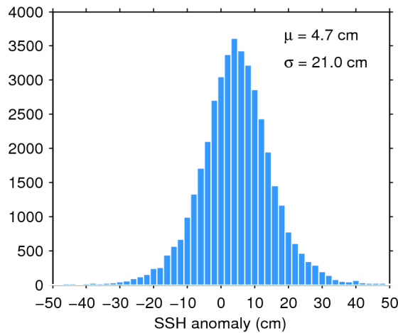
Figure 7. Histogram of flag-valid SSH anomaly over oceans and lakes for 10/06/2020. The mean ( \mu ) and standard deviation ( \sigma ) are also shown. Note that values outside [-50\ 50] cm are excluded from the histogram for the sake of readability but not from the computation of \mu and \sigma .
