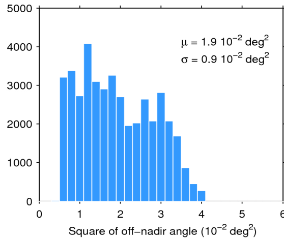
Figure 39. Histogram of flag-valid mispointing over oceans and lakes for 10/06/2020. The mean ( \mu ) and standard deviation ( \sigma ) are also shown. Note that values larger than 6 \cdot 10^{-2} \text{ deg}^2 are excluded from the histogram for the sake of readability but not from the computation of \mu and \sigma .
