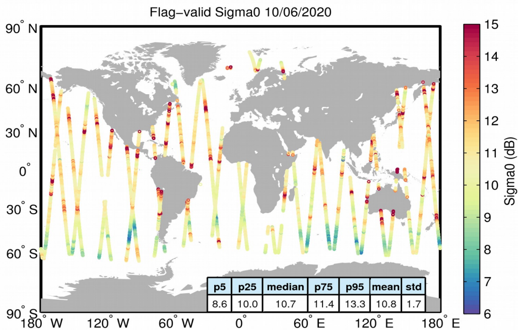
Figure 23. Geographical distribution of flag-valid sigma0 data over oceans and lakes for 10/06/2020. The statistical values shown in the table refer to the sigma0 in dB and are calculated over all measurements shown in the figure.
