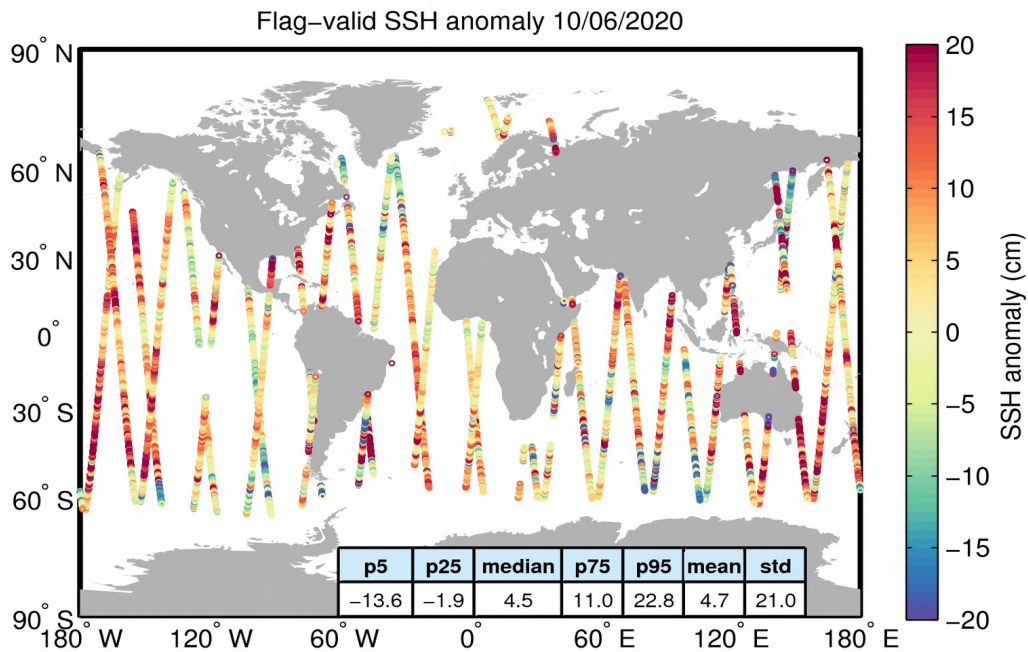
Figure 5. Geographical distribution of flag-valid 1-Hz SSH anomaly data over oceans and lakes for 10/06/2020. The statistical values shown in the table refer to the SSH anomaly in cm and are calculated over all measurements shown in the figure.
