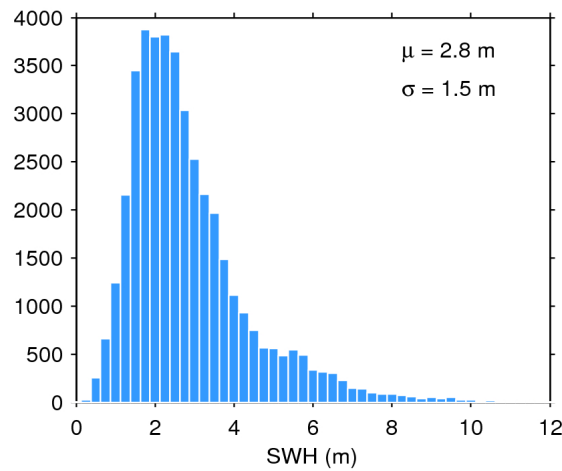
Figure 17. Histogram of flag-valid SWH over oceans and lakes for 10/06/2020. The mean ( \mu ) and standard deviation ( \sigma ) are also shown. Note that values larger than 12 m are excluded from the histogram for the sake of readability but not from the computation of \mu and \sigma .
