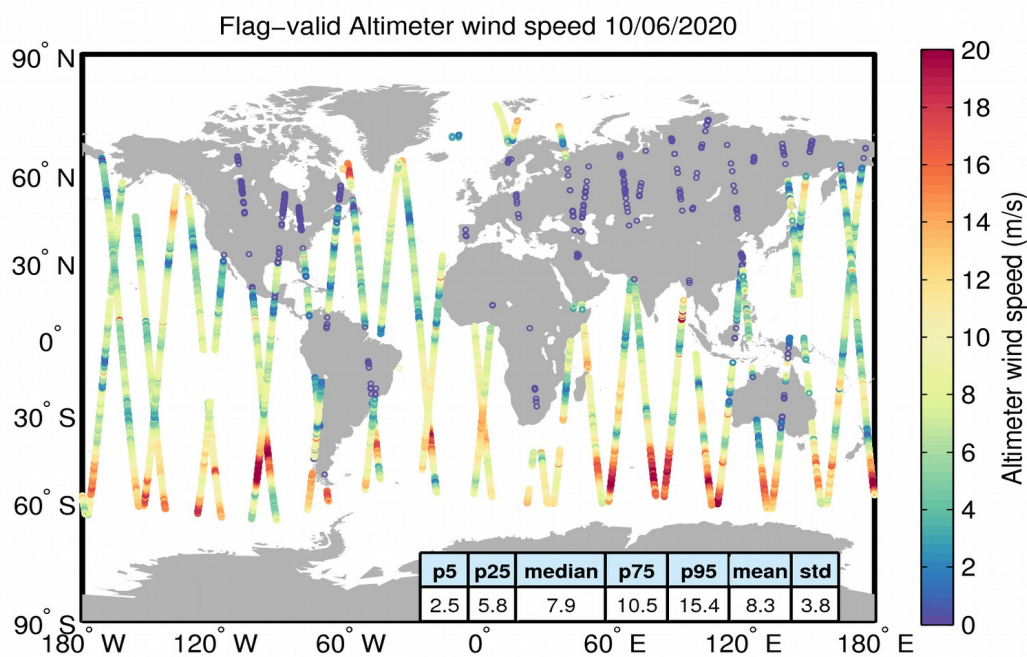
Figure 31. Geographical distribution of flag-valid wind data over oceans and lakes for 10/06/2020. The statistical values shown in the table refer to the wind in m/s and are calculated over all measurements shown in the figure.
