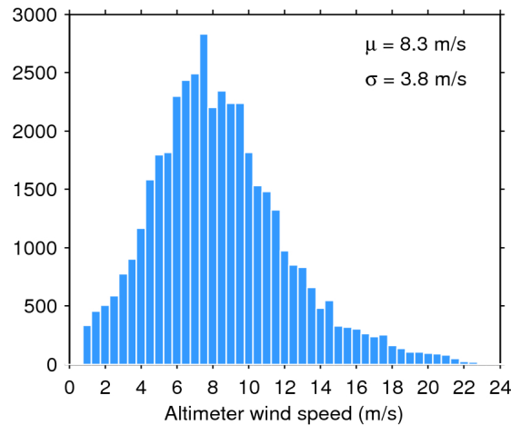
Figure 33. Histogram of flag-valid wind over oceans and lakes for 10/06/2020. The mean ( \mu ) and standard deviation ( \sigma ) are also shown. Note that values larger than 24 m/s are excluded from the histogram for the sake of readability but not from the computation of \mu and \sigma .
