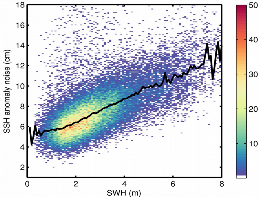
Figure 9. 2D histogram showing flag-valid SSH anomaly noise as a function of SWH for 10/06/2020. The black line denotes the median SSH anomaly noise as a function of SWH.
