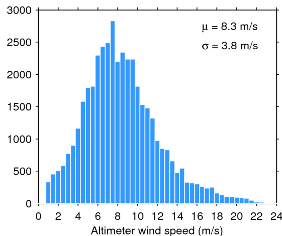
Figure 35. Histogram of science-valid wind over oceans and lakes for 10/06/2020. The mean ( \mu ) and standard deviation ( \sigma ) are also shown. Note that values larger than 24 m/s are excluded from the histogram for the sake of readability but not from the computation of \mu and \sigma .
