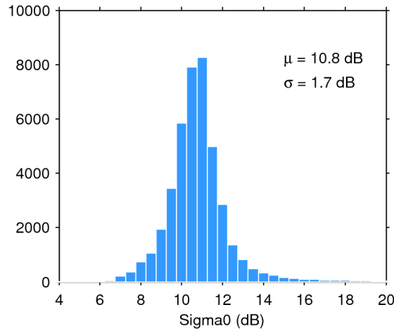
Figure 25. Histogram of flag-valid sigma0 over oceans and lakes for 10/06/2020. The mean ( \mu ) and standard deviation ( \sigma ) are also shown. Note that values outside [4 20] dB are excluded from the histogram for the sake of readability but not from the computation of \mu and \sigma .
