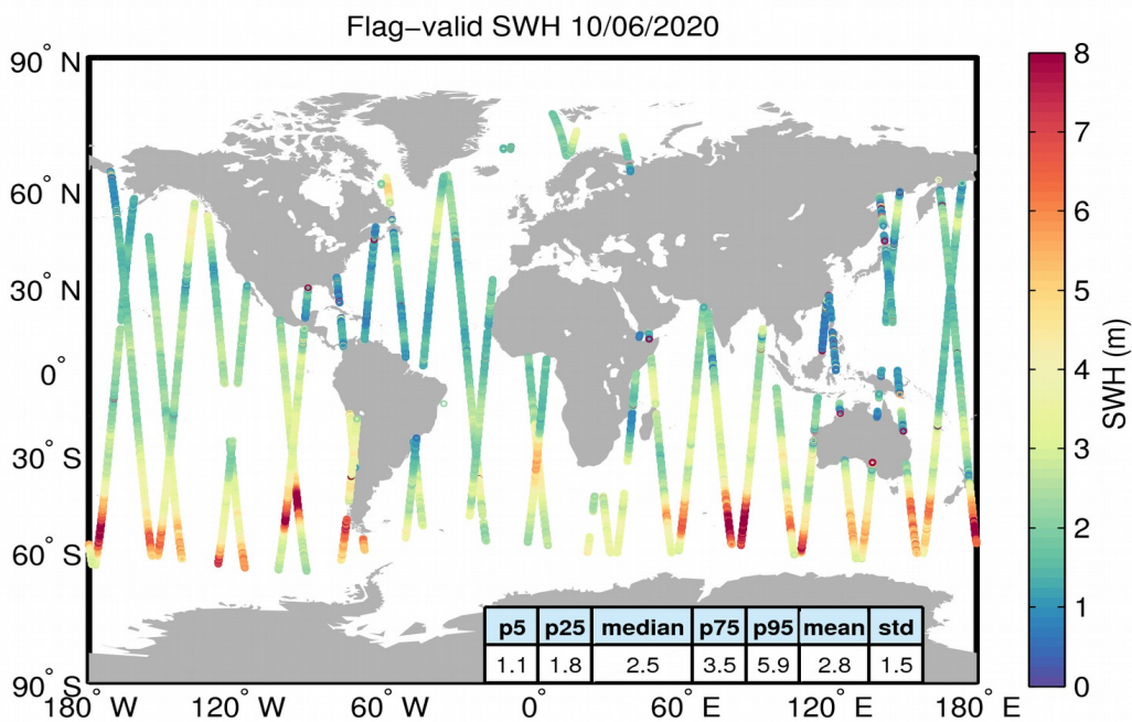
Figure 15. Geographical distribution of flag-valid SWH data over oceans and lakes for 10/06/2020. The statistical values shown in the table refer to the SWH in m and are calculated over all measurements shown in the figure.
