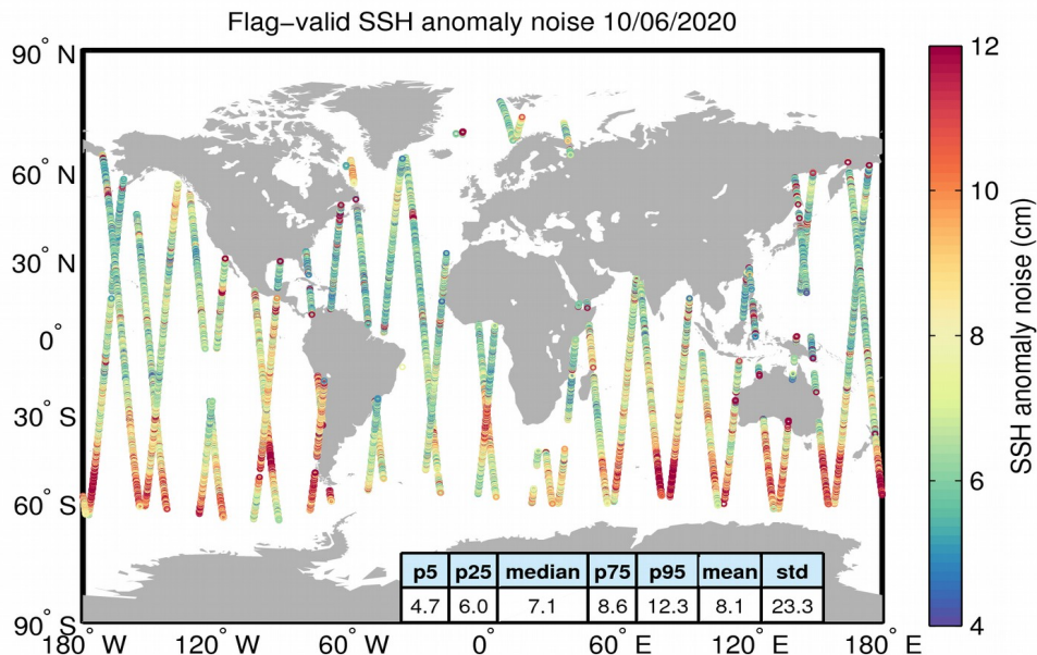
Figure 8. Geographical distribution of flag-valid 20-Hz SSH anomaly measurement noise over oceans and lakes for 10/06/2020. The statistical values shown in the table refer to the SSH anomaly noise and are calculated over all measurements shown in the figure.
