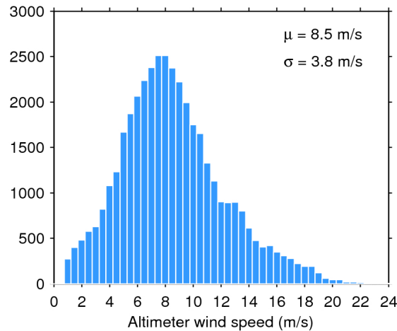
Figure 33. Histogram of flag-valid wind over oceans and lakes for 09/06/2020. The mean ( \mu ) and standard deviation ( \sigma ) are also shown. Note that values larger than 24 m/s are excluded from the histogram for the sake of readability but not from the computation of \mu and \sigma .
