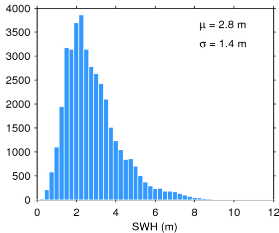
Figure 20. Histogram of science-valid SWH over oceans and lakes for 09/06/2020. The mean ( \mu ) and standard deviation ( \sigma ) are also shown. Note that values larger than 12 m are excluded from the histogram for the sake of readability but not from the computation of \mu and \sigma .
