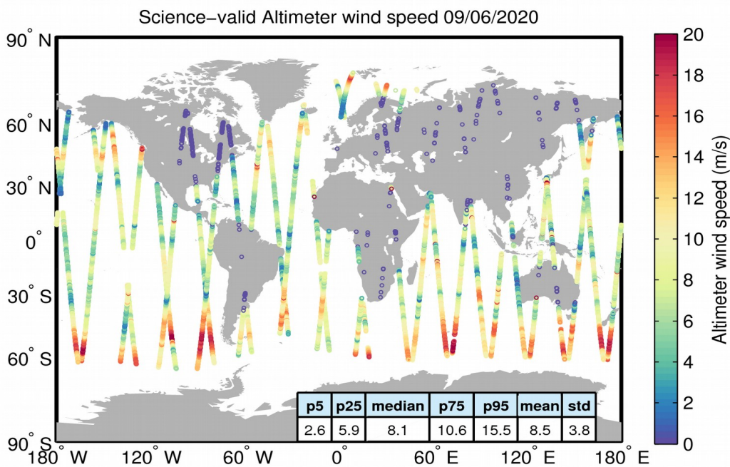
Figure 34. Geographical distribution of science-valid wind data over oceans and lakes for 09/06/2020. The statistical values shown in the table refer to the wind in m/s and are calculated over all measurements shown in the figure. Gray circles denote records that have been rejected based on the editing criteria described in Table 5.
