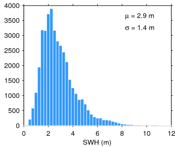
Figure 17. Histogram of flag-valid SWH over oceans and lakes for 09/06/2020. The mean ( \mu ) and standard deviation ( \sigma ) are also shown. Note that values larger than 12 m are excluded from the histogram for the sake of readability but not from the computation of \mu and \sigma .
