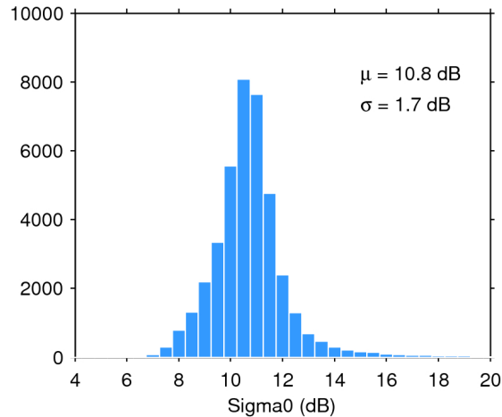
Figure 25. Histogram of flag-valid sigma0 over oceans and lakes for 09/06/2020. The mean ( \mu ) and standard deviation ( \sigma ) are also shown. Note that values outside [4 20] dB are excluded from the histogram for the sake of readability but not from the computation of \mu and \sigma .
