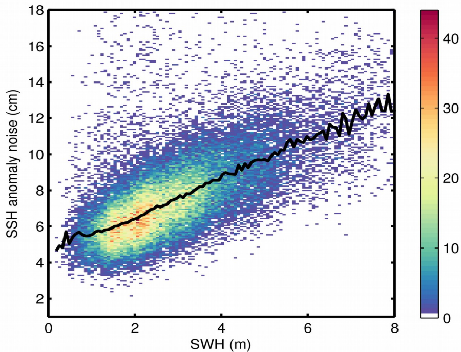
Figure 9. 2D histogram showing flag-valid SSH anomaly noise as a function of SWH for 09/06/2020. The black line denotes the median SSH anomaly noise as a function of SWH.
