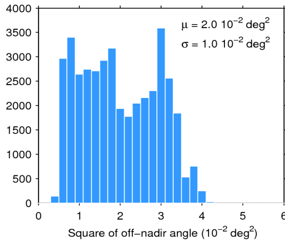
Figure 39. Histogram of flag-valid mispointing over oceans and lakes for 09/06/2020. The mean ( \mu ) and standard deviation ( \sigma ) are also shown. Note that values larger than 6 \cdot 10^{-2} \text{ deg}^2 are excluded from the histogram for the sake of readability but not from the computation of \mu and \sigma .
