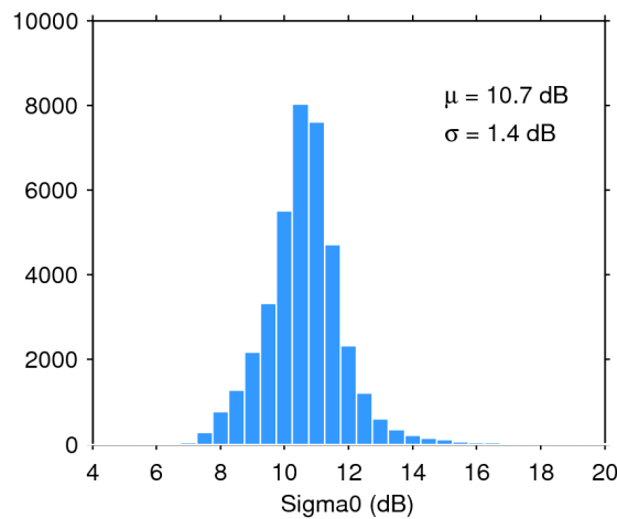
Figure 28. Histogram of science-valid sigma0 over oceans and lakes for 09/06/2020. The mean ( \mu ) and standard deviation ( \sigma ) are also shown. Note that values outside [4 20] dB are excluded from the histogram for the sake of readability but not from the computation of \mu and \sigma .
