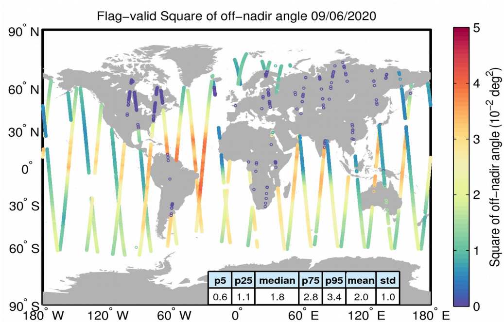
Figure 37. Geographical distribution of flag-valid mispointing data over oceans and lakes for 09/06/2020. The statistical values shown in the table refer to the mispointing in 10^{-2} deg 2 and are calculated over all measurements shown in the figure.
