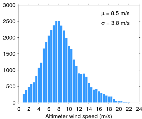
Figure 35. Histogram of science-valid wind over oceans and lakes for 09/06/2020. The mean ( \mu ) and standard deviation ( \sigma ) are also shown. Note that values larger than 24 m/s are excluded from the histogram for the sake of readability but not from the computation of \mu and \sigma .
