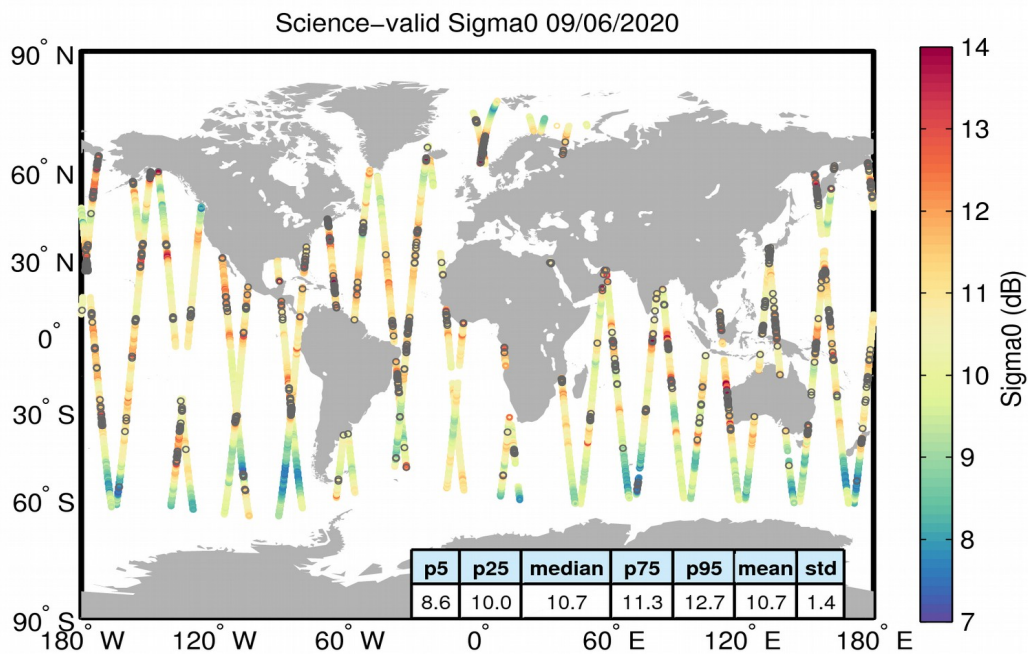
Figure 27. Geographical distribution of science-valid sigma0 data over oceans and lakes for 09/06/2020. The statistical values shown in the table refer to the sigma0 in dB and are calculated over all measurements shown in the figure. Gray circles denote records that have been rejected based on the editing criteria described in Table 4.
