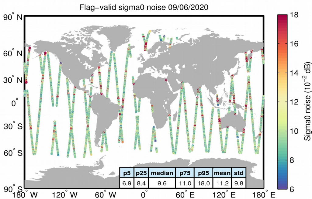
Figure 26. Geographical distribution of flag-valid 20-Hz sigma0 measurement noise over oceans and lakes for 09/06/2020. The statistical values shown in the table refer to the sigma0 noise and are calculated over all measurements shown in the figure.
