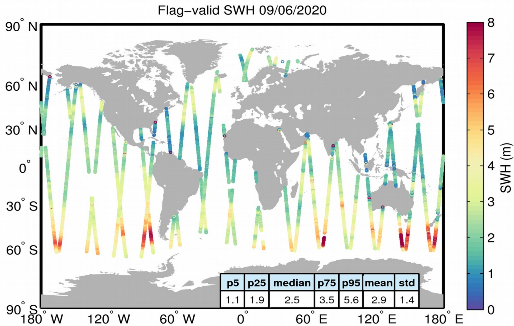
Figure 15. Geographical distribution of flag-valid SWH data over oceans and lakes for 09/06/2020. The statistical values shown in the table refer to the SWH in m and are calculated over all measurements shown in the figure.
