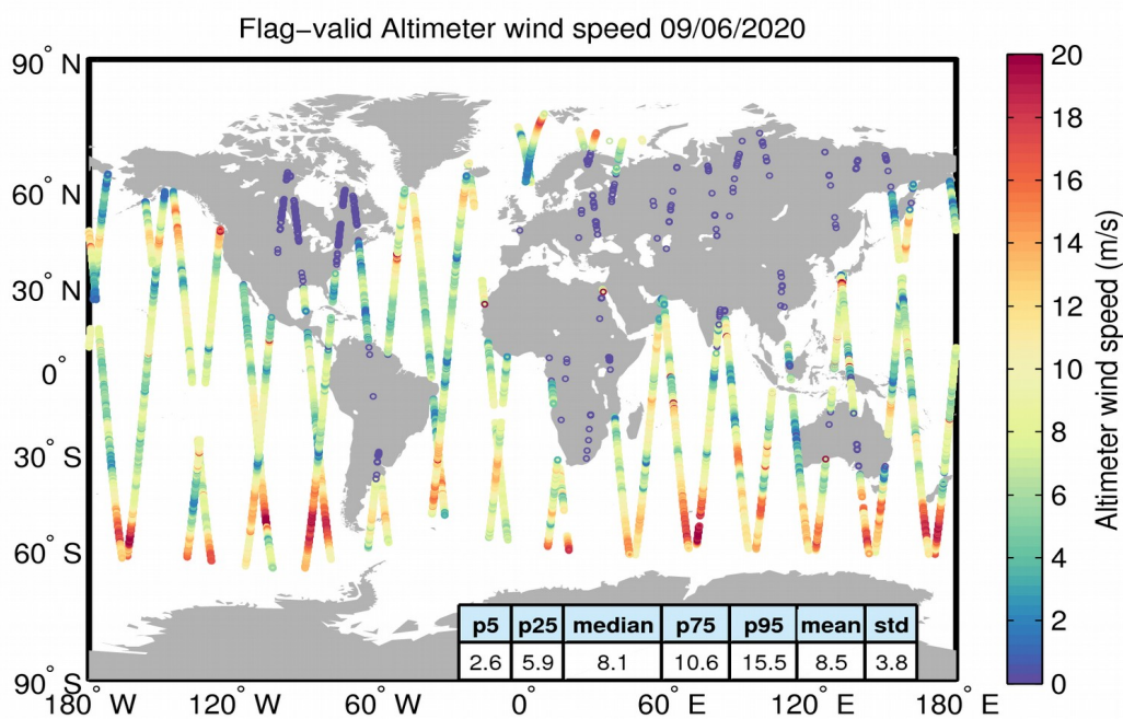
Figure 31. Geographical distribution of flag-valid wind data over oceans and lakes for 09/06/2020. The statistical values shown in the table refer to the wind in m/s and are calculated over all measurements shown in the figure.
