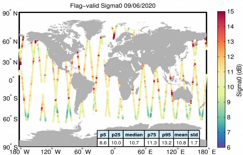
Figure 23. Geographical distribution of flag-valid sigma0 data over oceans and lakes for 09/06/2020. The statistical values shown in the table refer to the sigma0 in dB and are calculated over all measurements shown in the figure.
