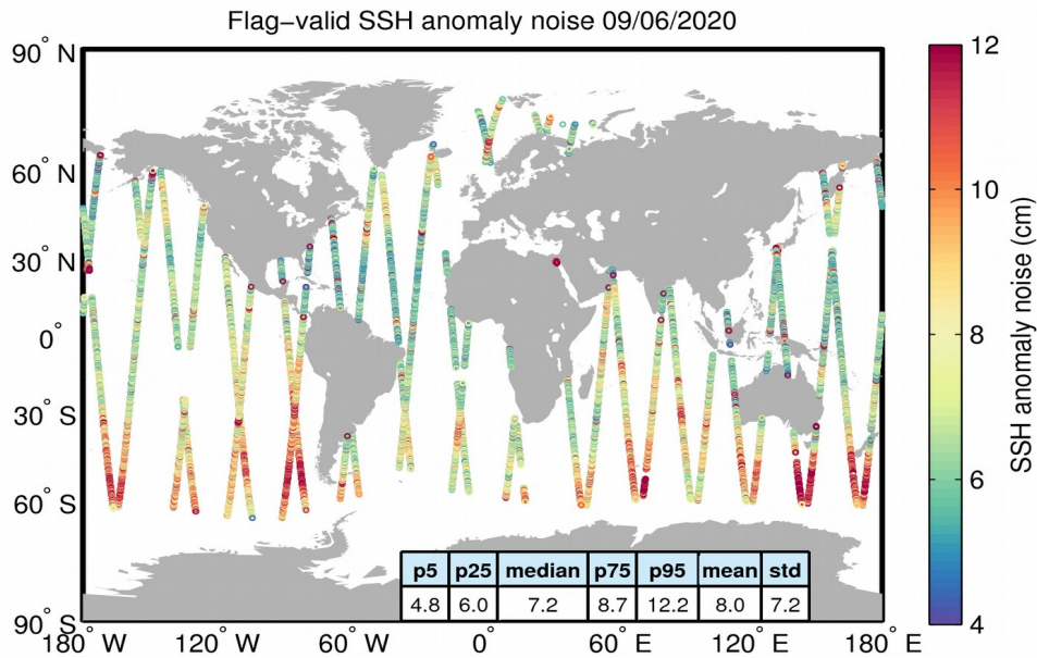
Figure 8. Geographical distribution of flag-valid 20-Hz SSH anomaly measurement noise over oceans and lakes for 09/06/2020. The statistical values shown in the table refer to the SSH anomaly noise and are calculated over all measurements shown in the figure.
