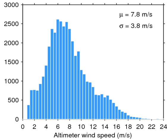
Figure 33. Histogram of flag-valid wind over oceans and lakes for 08/06/2020. The mean ( \mu ) and standard deviation ( \sigma ) are also shown. Note that values larger than 24 m/s are excluded from the histogram for the sake of readability but not from the computation of \mu and \sigma .
