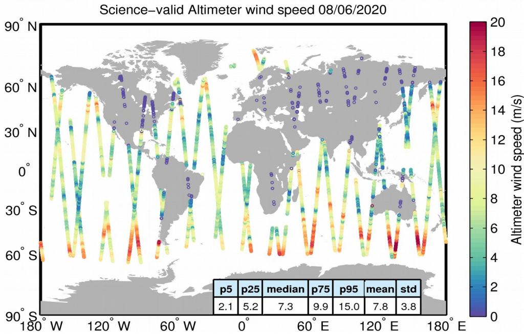
Figure 34. Geographical distribution of science-valid wind data over oceans and lakes for 08/06/2020. The statistical values shown in the table refer to the wind in m/s and are calculated over all measurements shown in the figure. Gray circles denote records that have been rejected based on the editing criteria described in Table 5.
