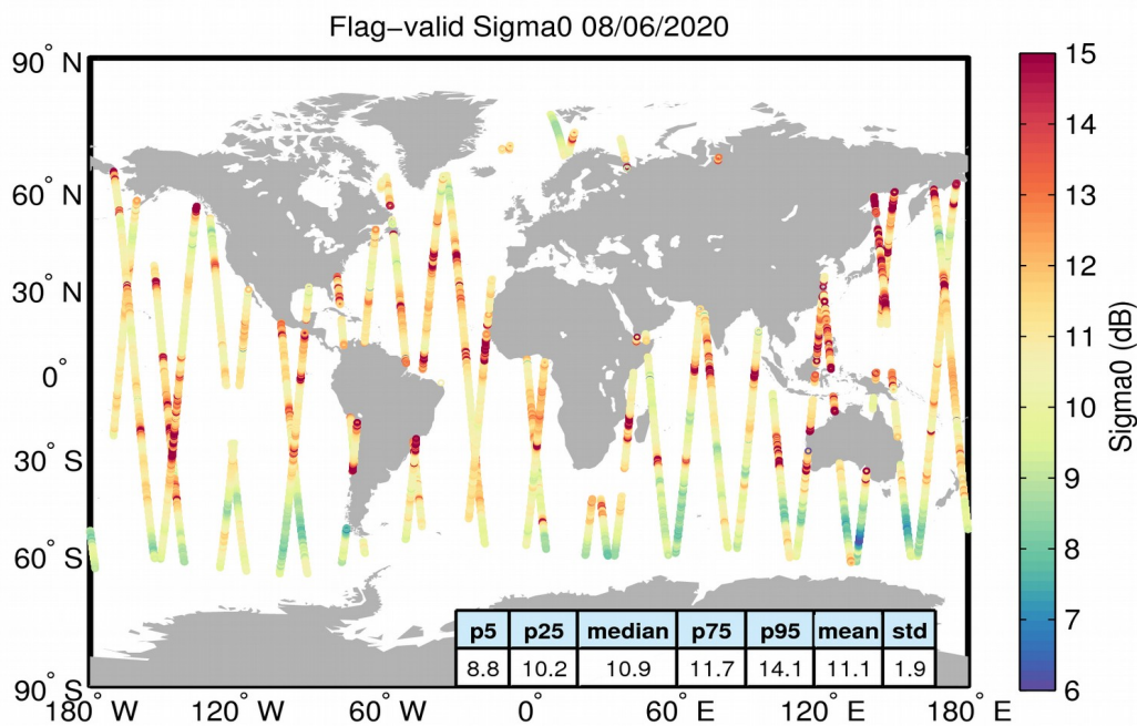
Figure 23. Geographical distribution of flag-valid sigma0 data over oceans and lakes for 08/06/2020. The statistical values shown in the table refer to the sigma0 in dB and are calculated over all measurements shown in the figure.
