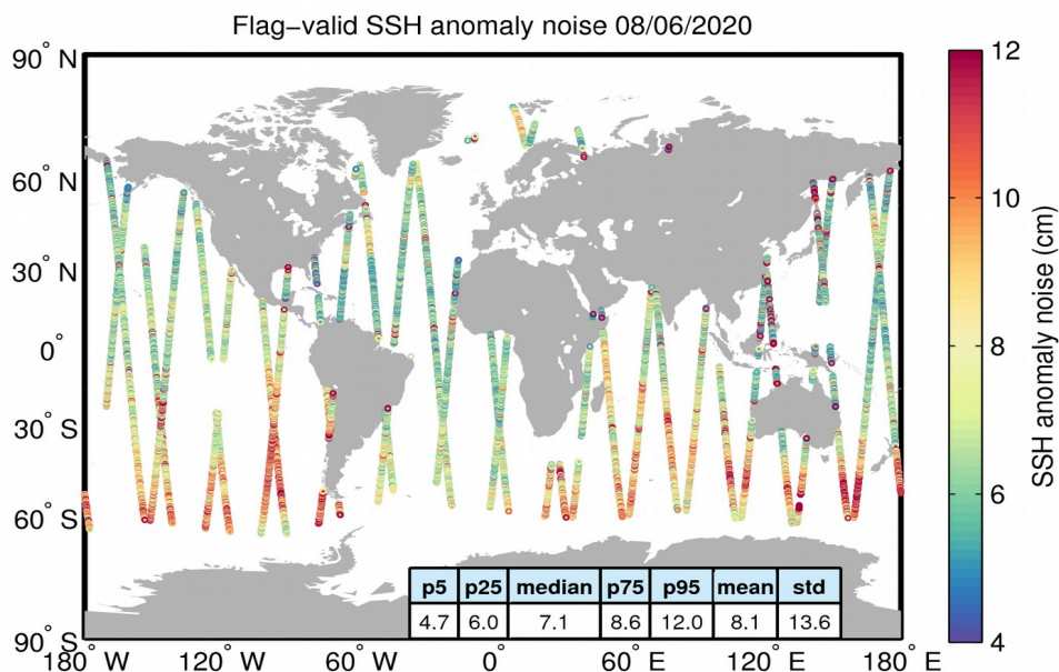
Figure 8. Geographical distribution of flag-valid 20-Hz SSH anomaly measurement noise over oceans and lakes for 08/06/2020. The statistical values shown in the table refer to the SSH anomaly noise and are calculated over all measurements shown in the figure.
