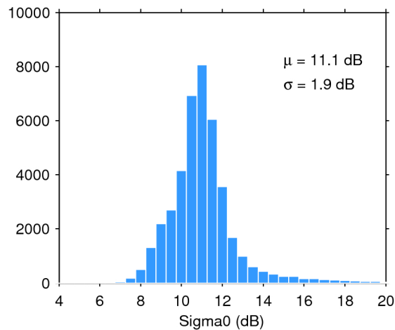
Figure 25. Histogram of flag-valid sigma0 over oceans and lakes for 08/06/2020. The mean ( \mu ) and standard deviation ( \sigma ) are also shown. Note that values outside [4 20] dB are excluded from the histogram for the sake of readability but not from the computation of \mu and \sigma .
