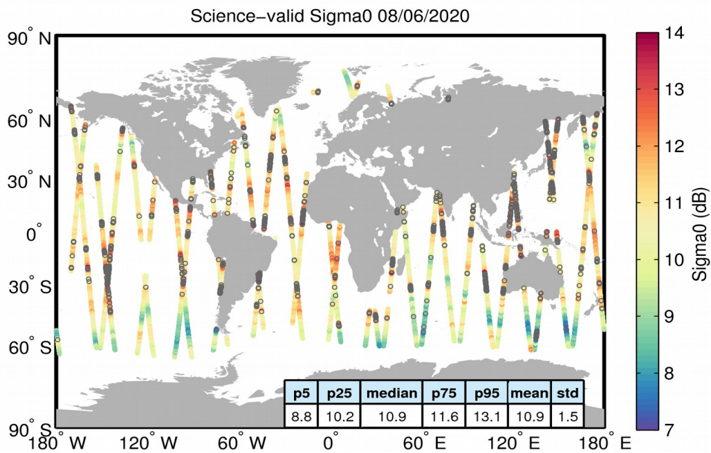
Figure 27. Geographical distribution of science-valid sigma0 data over oceans and lakes for 08/06/2020. The statistical values shown in the table refer to the sigma0 in dB and are calculated over all measurements shown in the figure. Gray circles denote records that have been rejected based on the editing criteria described in Table 4.
