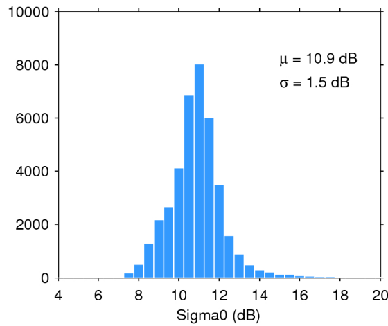
Figure 28. Histogram of science-valid sigma0 over oceans and lakes for 08/06/2020. The mean ( \mu ) and standard deviation ( \sigma ) are also shown. Note that values outside [4 20] dB are excluded from the histogram for the sake of readability but not from the computation of \mu and \sigma .
