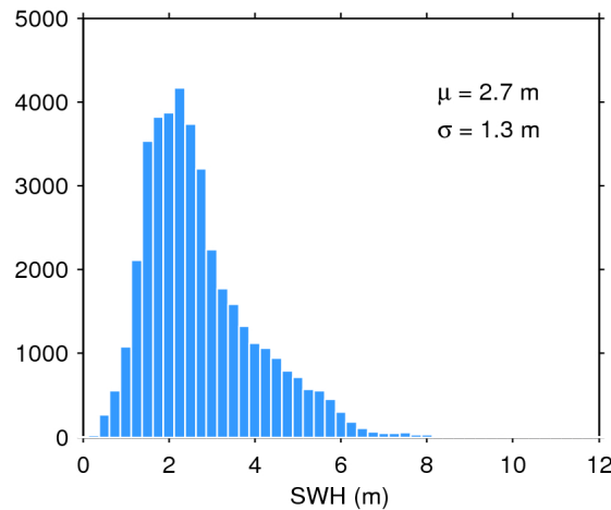
Figure 20. Histogram of science-valid SWH over oceans and lakes for 08/06/2020. The mean ( \mu ) and standard deviation ( \sigma ) are also shown. Note that values larger than 12 m are excluded from the histogram for the sake of readability but not from the computation of \mu and \sigma .
