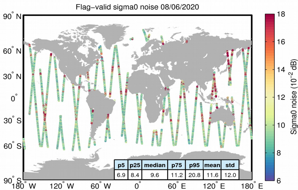
Figure 26. Geographical distribution of flag-valid 20-Hz sigma0 measurement noise over oceans and lakes for 08/06/2020. The statistical values shown in the table refer to the sigma0 noise and are calculated over all measurements shown in the figure.
