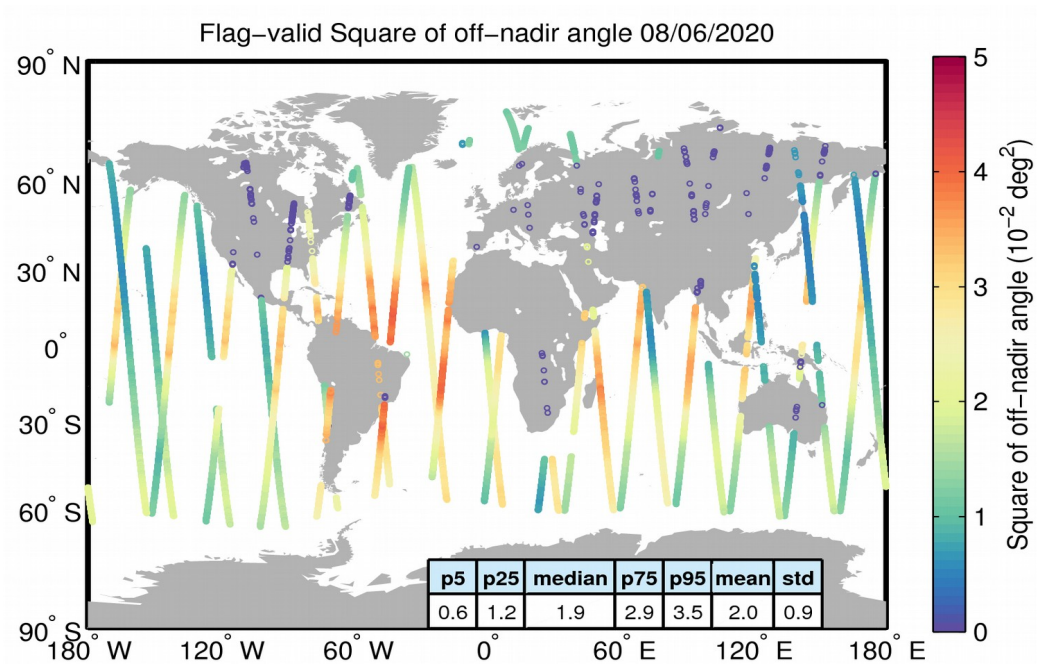
Figure 37. Geographical distribution of flag-valid mispointing data over oceans and lakes for 08/06/2020. The statistical values shown in the table refer to the mispointing in 10^{-2} deg 2 and are calculated over all measurements shown in the figure.
