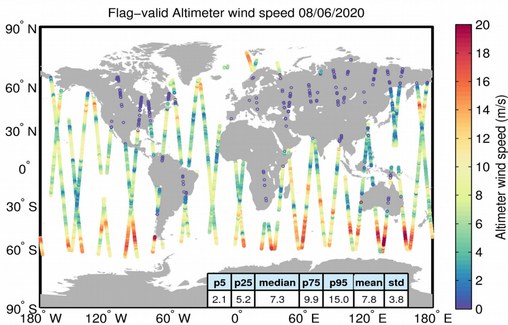
Figure 31. Geographical distribution of flag-valid wind data over oceans and lakes for 08/06/2020. The statistical values shown in the table refer to the wind in m/s and are calculated over all measurements shown in the figure.
