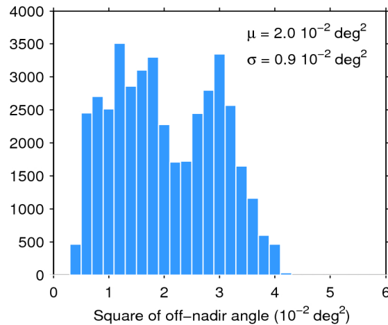
Figure 39. Histogram of flag-valid mispointing over oceans and lakes for 08/06/2020. The mean ( \mu ) and standard deviation ( \sigma ) are also shown. Note that values larger than 6 \cdot 10^{-2} \text{ deg}^2 are excluded from the histogram for the sake of readability but not from the computation of \mu and \sigma .
