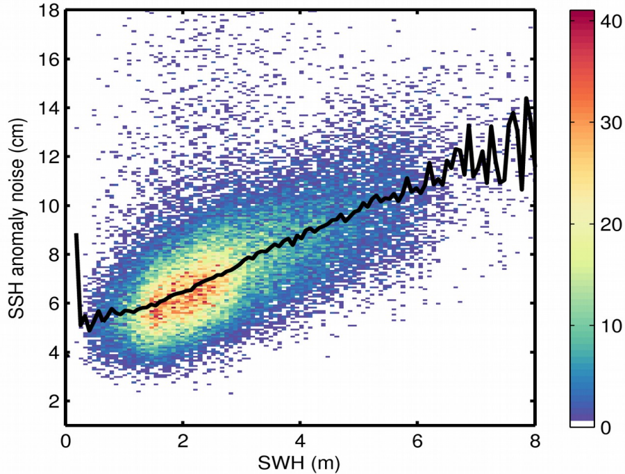
Figure 9. 2D histogram showing flag-valid SSH anomaly noise as a function of SWH for 08/06/2020. The black line denotes the median SSH anomaly noise as a function of SWH.
