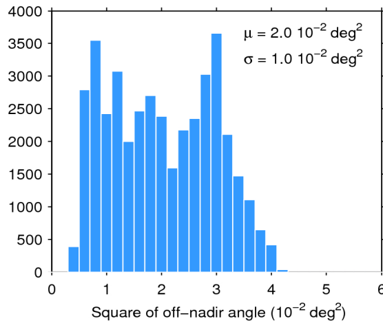
Figure 39. Histogram of flag-valid mispointing over oceans and lakes for 07/06/2020. The mean ( \mu ) and standard deviation ( \sigma ) are also shown. Note that values larger than 6 \cdot 10^{-2} \text{ deg}^2 are excluded from the histogram for the sake of readability but not from the computation of \mu and \sigma .
