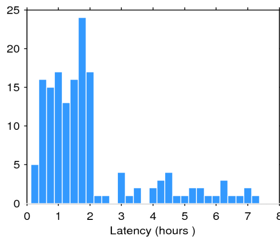
Figure 2. Histogram of the data latency for 07/06/2020. The y-axis denotes the number of files that are made available with a delay of x-hours with respect to the mean time of the records stored in the file.
