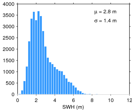
Figure 20. Histogram of science-valid SWH over oceans and lakes for 07/06/2020. The mean ( \mu ) and standard deviation ( \sigma ) are also shown. Note that values larger than 12 m are excluded from the histogram for the sake of readability but not from the computation of \mu and \sigma .
