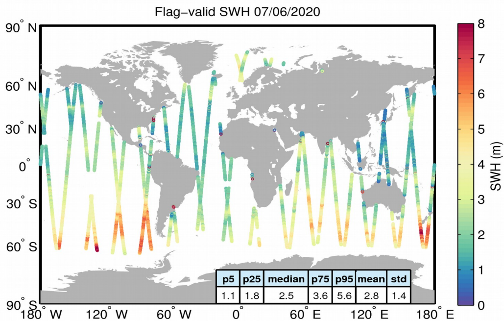
Figure 15. Geographical distribution of flag-valid SWH data over oceans and lakes for 07/06/2020. The statistical values shown in the table refer to the SWH in m and are calculated over all measurements shown in the figure.
