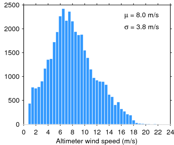
Figure 33. Histogram of flag-valid wind over oceans and lakes for 07/06/2020. The mean ( \mu ) and standard deviation ( \sigma ) are also shown. Note that values larger than 24 m/s are excluded from the histogram for the sake of readability but not from the computation of \mu and \sigma .
