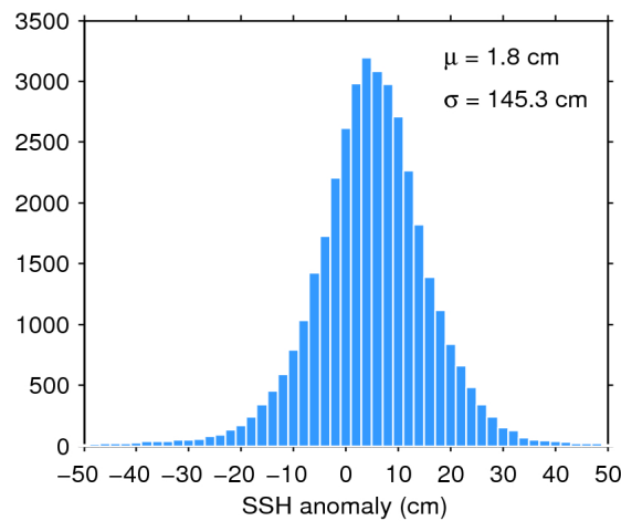
Figure 7. Histogram of flag-valid SSH anomaly over oceans and lakes for 07/06/2020. The mean ( \mu ) and standard deviation ( \sigma ) are also shown. Note that values outside [-50\ 50] cm are excluded from the histogram for the sake of readability but not from the computation of \mu and \sigma .
