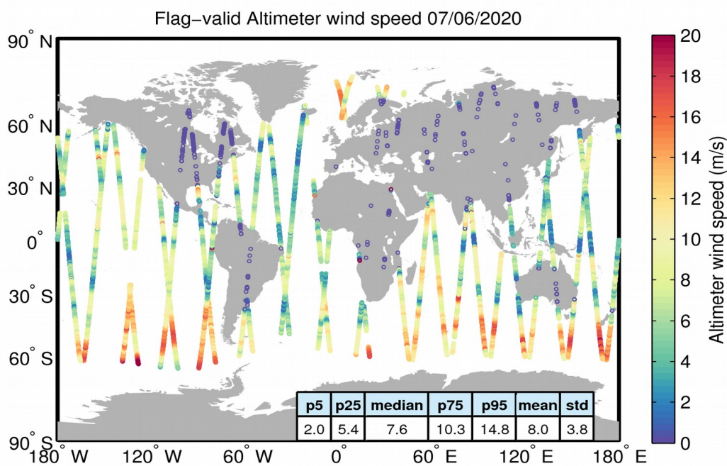
Figure 31. Geographical distribution of flag-valid wind data over oceans and lakes for 07/06/2020. The statistical values shown in the table refer to the wind in m/s and are calculated over all measurements shown in the figure.
