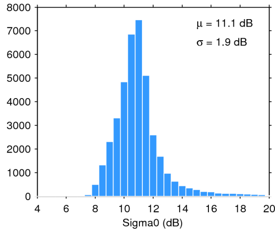
Figure 25. Histogram of flag-valid sigma0 over oceans and lakes for 07/06/2020. The mean ( \mu ) and standard deviation ( \sigma ) are also shown. Note that values outside [4 20] dB are excluded from the histogram for the sake of readability but not from the computation of \mu and \sigma .
