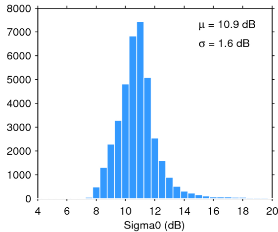
Figure 28. Histogram of science-valid sigma0 over oceans and lakes for 07/06/2020. The mean ( \mu ) and standard deviation ( \sigma ) are also shown. Note that values outside [4 20] dB are excluded from the histogram for the sake of readability but not from the computation of \mu and \sigma .
