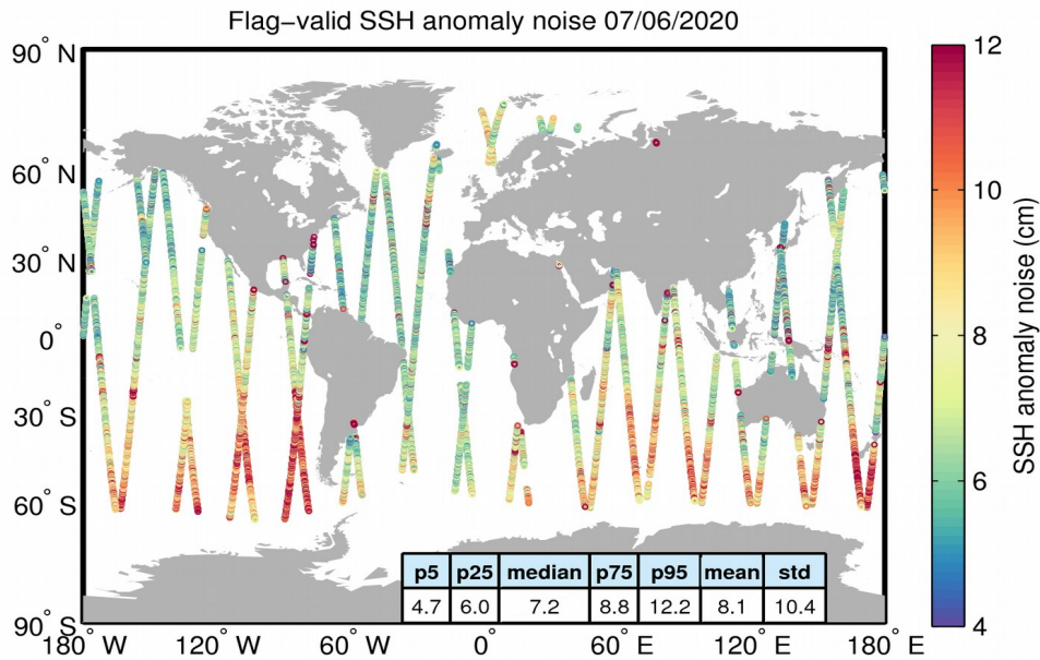
Figure 8. Geographical distribution of flag-valid 20-Hz SSH anomaly measurement noise over oceans and lakes for 07/06/2020. The statistical values shown in the table refer to the SSH anomaly noise and are calculated over all measurements shown in the figure.
