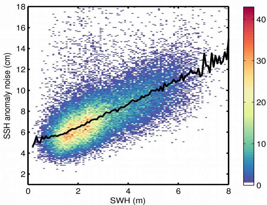
Figure 9. 2D histogram showing flag-valid SSH anomaly noise as a function of SWH for 07/06/2020. The black line denotes the median SSH anomaly noise as a function of SWH.
