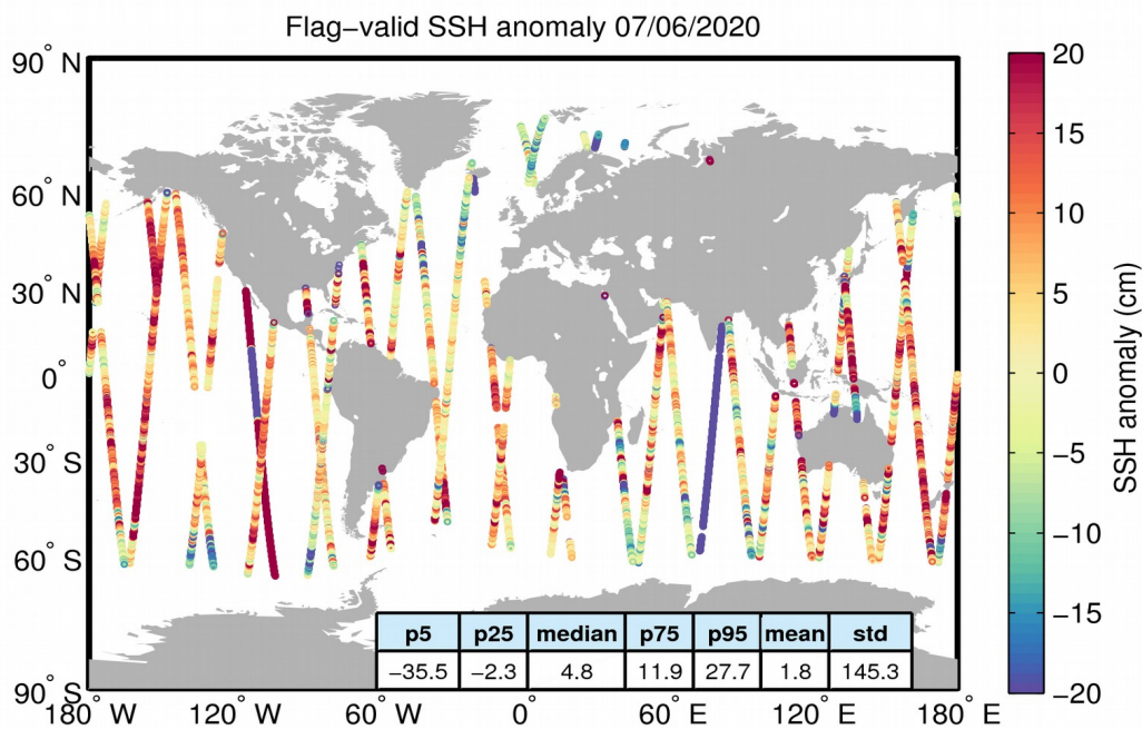
Figure 5. Geographical distribution of flag-valid 1-Hz SSH anomaly data over oceans and lakes for 07/06/2020. The statistical values shown in the table refer to the SSH anomaly in cm and are calculated over all measurements shown in the figure.
