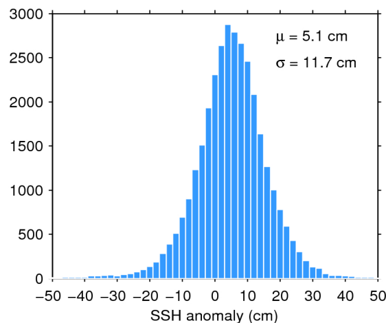
Figure 11. Histogram of science-valid SSH anomaly over oceans and lakes for 07/06/2020. The mean ( \mu ) and standard deviation ( \sigma ) are also shown. Note that values outside [-50 50] cm are excluded from the histogram for the sake of readability but not from the computation of \mu and \sigma .
