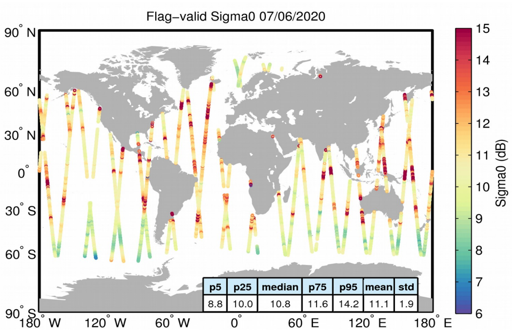
Figure 23. Geographical distribution of flag-valid sigma0 data over oceans and lakes for 07/06/2020. The statistical values shown in the table refer to the sigma0 in dB and are calculated over all measurements shown in the figure.
