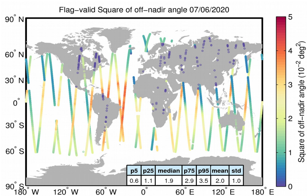
Figure 37. Geographical distribution of flag-valid mispointing data over oceans and lakes for 07/06/2020. The statistical values shown in the table refer to the mispointing in 10^{-2} deg 2 and are calculated over all measurements shown in the figure.
