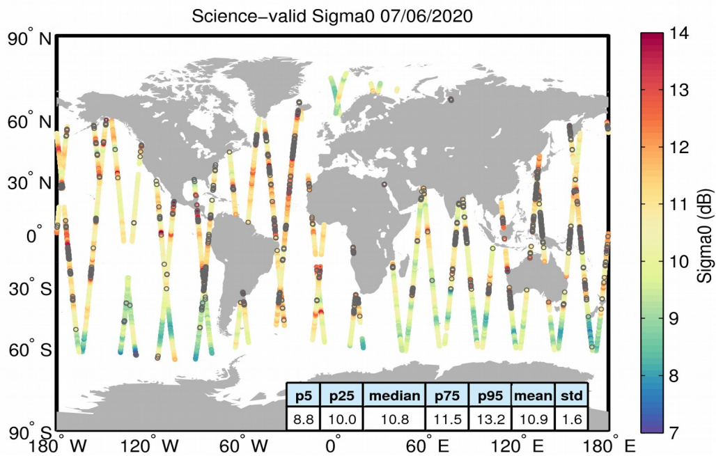
Figure 27. Geographical distribution of science-valid sigma0 data over oceans and lakes for 07/06/2020. The statistical values shown in the table refer to the sigma0 in dB and are calculated over all measurements shown in the figure. Gray circles denote records that have been rejected based on the editing criteria described in Table 4.
