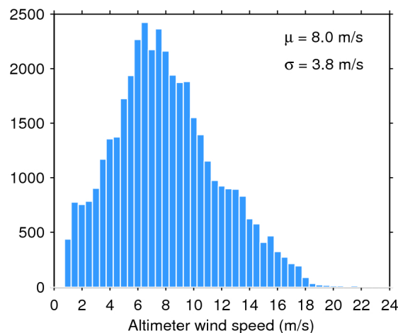
Figure 35. Histogram of science-valid wind over oceans and lakes for 07/06/2020. The mean ( \mu ) and standard deviation ( \sigma ) are also shown. Note that values larger than 24 m/s are excluded from the histogram for the sake of readability but not from the computation of \mu and \sigma .
