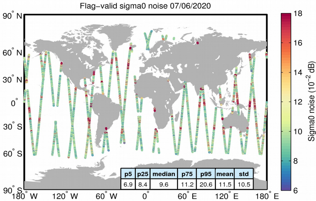
Figure 26. Geographical distribution of flag-valid 20-Hz sigma0 measurement noise over oceans and lakes for 07/06/2020. The statistical values shown in the table refer to the sigma0 noise and are calculated over all measurements shown in the figure.
