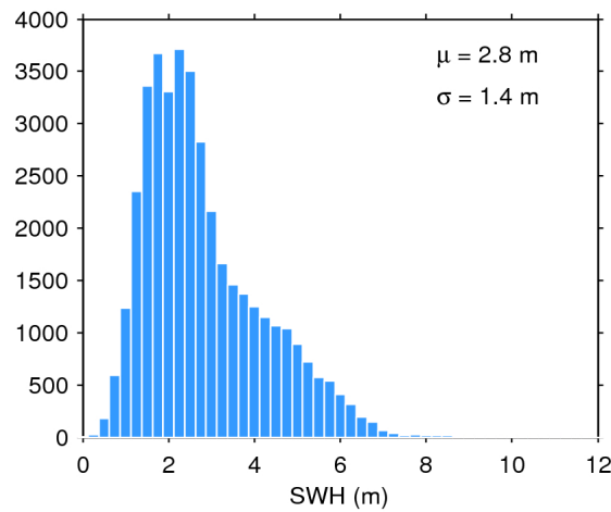
Figure 17. Histogram of flag-valid SWH over oceans and lakes for 07/06/2020. The mean ( \mu ) and standard deviation ( \sigma ) are also shown. Note that values larger than 12 m are excluded from the histogram for the sake of readability but not from the computation of \mu and \sigma .
