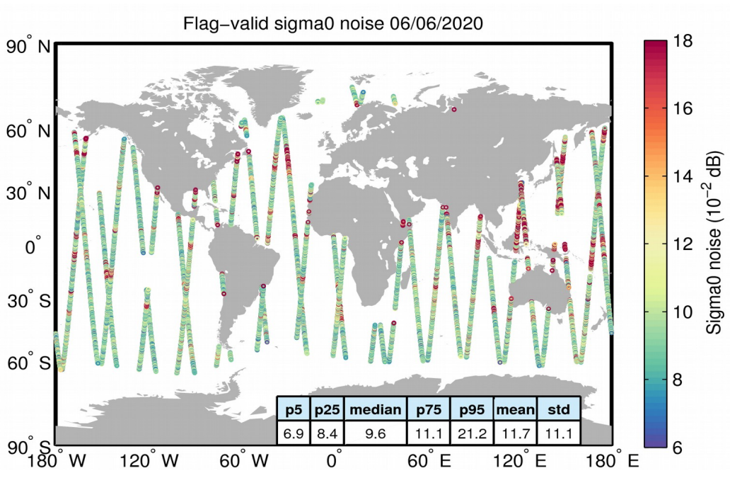
Figure 26. Geographical distribution of flag-valid 20-Hz sigma0 measurement noise over oceans and lakes for 06/06/2020. The statistical values shown in the table refer to the sigma0 noise and are calculated over all measurements shown in the figure.
