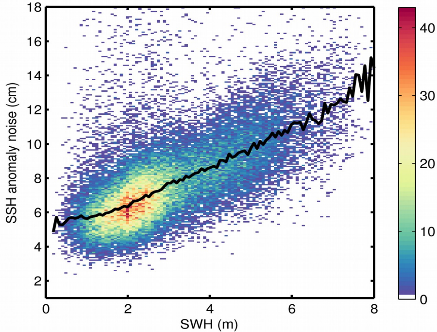
Figure 9. 2D histogram showing flag-valid SSH anomaly noise as a function of SWH for 06/06/2020. The black line denotes the median SSH anomaly noise as a function of SWH.
