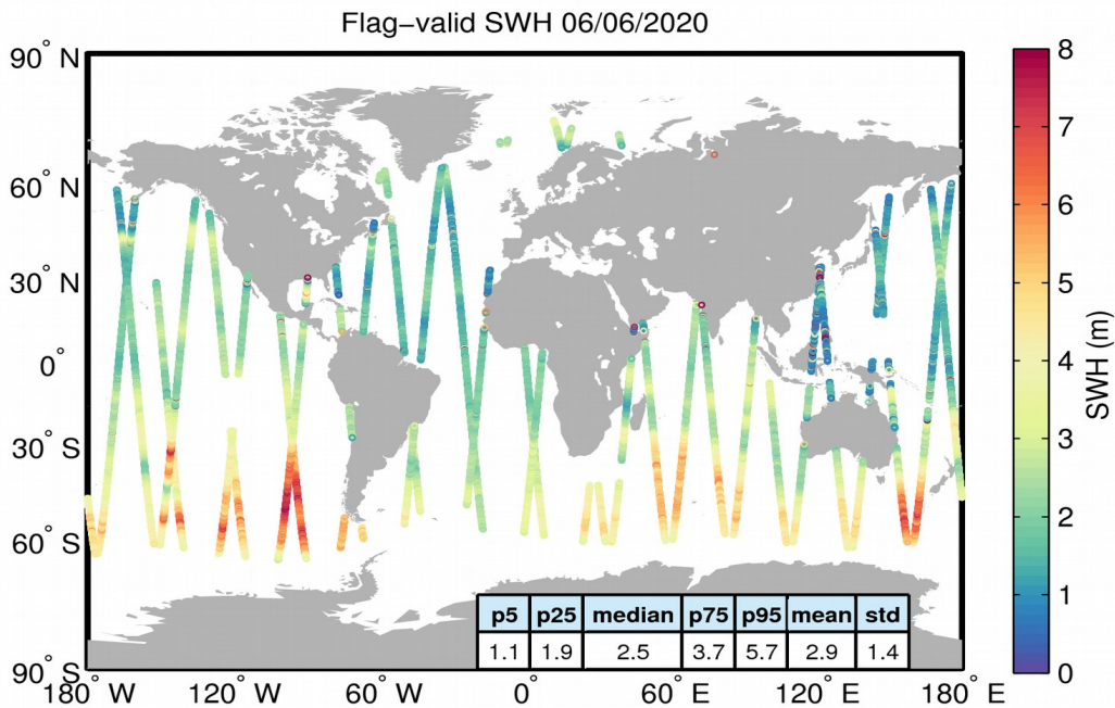
Figure 15. Geographical distribution of flag-valid SWH data over oceans and lakes for 06/06/2020. The statistical values shown in the table refer to the SWH in m and are calculated over all measurements shown in the figure.
