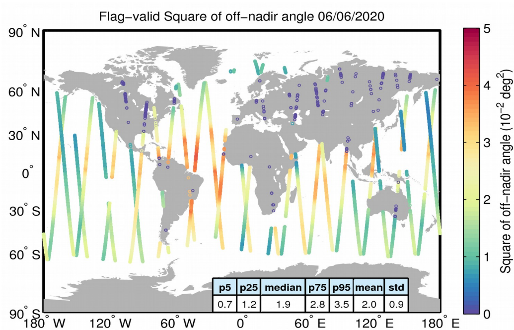
Figure 37. Geographical distribution of flag-valid mispointing data over oceans and lakes for 06/06/2020. The statistical values shown in the table refer to the mispointing in 10^{-2} \text{ deg}^2 and are calculated over all measurements shown in the figure.
