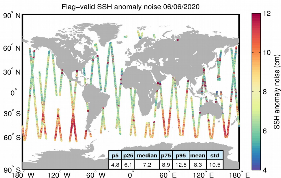
Figure 8. Geographical distribution of flag-valid 20-Hz SSH anomaly measurement noise over oceans and lakes for 06/06/2020. The statistical values shown in the table refer to the SSH anomaly noise and are calculated over all measurements shown in the figure.
