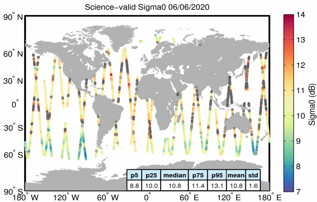
Figure 27. Geographical distribution of science-valid sigma0 data over oceans and lakes for 06/06/2020. The statistical values shown in the table refer to the sigma0 in dB and are calculated over all measurements shown in the figure. Gray circles denote records that have been rejected based on the editing criteria described in Table 4.
