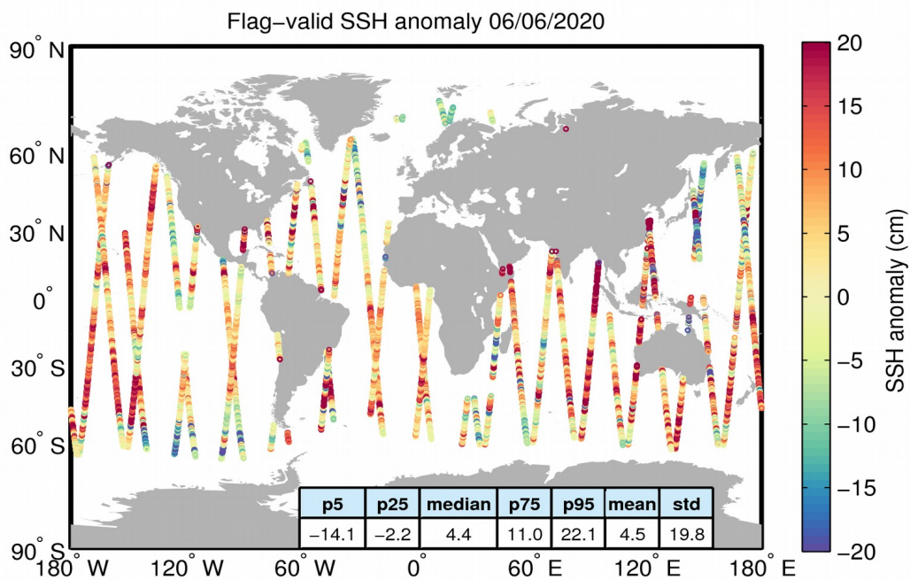
Figure 5. Geographical distribution of flag-valid 1-Hz SSH anomaly data over oceans and lakes for 06/06/2020. The statistical values shown in the table refer to the SSH anomaly in cm and are calculated over all measurements shown in the figure.
