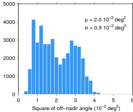
Figure 39. Histogram of flag-valid mispointing over oceans and lakes for 06/06/2020. The mean ( \mu ) and standard deviation ( \sigma ) are also shown. Note that values larger than 6 \cdot 10^{-2} \text{ deg}^2 are excluded from the histogram for the sake of readability but not from the computation of \mu and \sigma .
