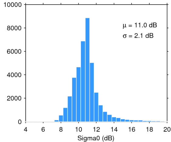
Figure 25. Histogram of flag-valid sigma0 over oceans and lakes for 06/06/2020. The mean ( \mu ) and standard deviation ( \sigma ) are also shown. Note that values outside [4 20] dB are excluded from the histogram for the sake of readability but not from the computation of \mu and \sigma .
