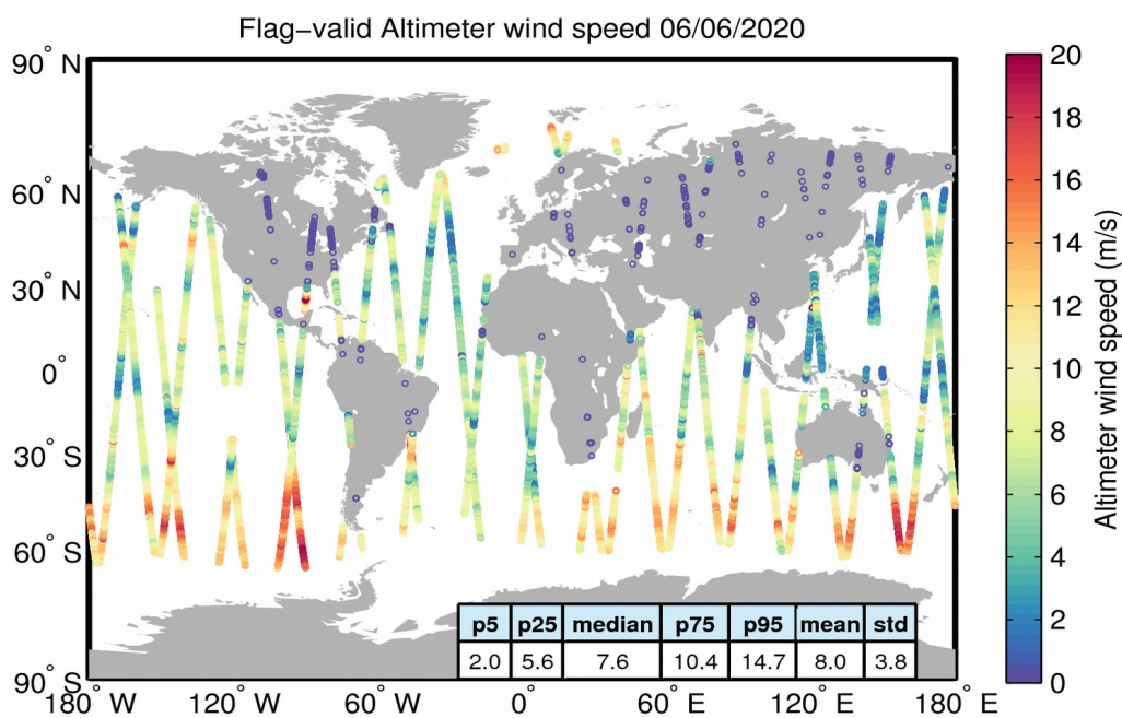
Figure 31. Geographical distribution of flag-valid wind data over oceans and lakes for 06/06/2020. The statistical values shown in the table refer to the wind in m/s and are calculated over all measurements shown in the figure.
