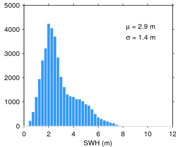
Figure 20. Histogram of science-valid SWH over oceans and lakes for 06/06/2020. The mean ( \mu ) and standard deviation ( \sigma ) are also shown. Note that values larger than 12 m are excluded from the histogram for the sake of readability but not from the computation of \mu and \sigma .
