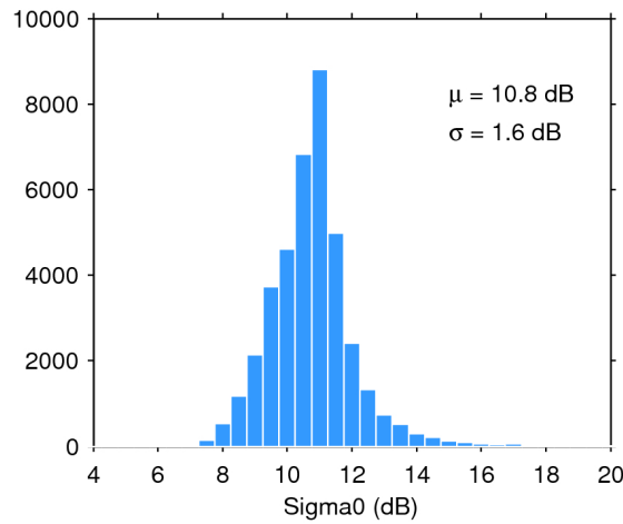
Figure 28. Histogram of science-valid sigma0 over oceans and lakes for 06/06/2020. The mean ( \mu ) and standard deviation ( \sigma ) are also shown. Note that values outside [4 20] dB are excluded from the histogram for the sake of readability but not from the computation of \mu and \sigma .
