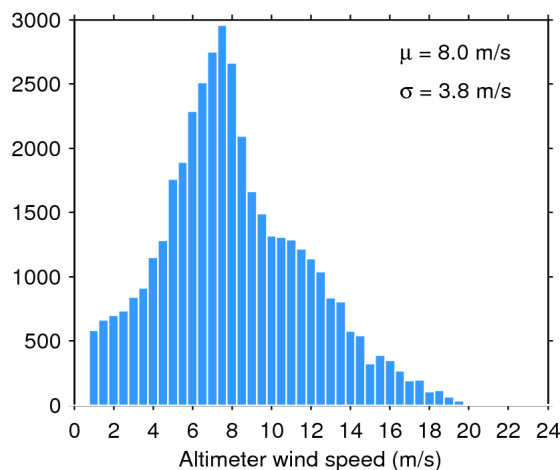
Figure 35. Histogram of science-valid wind over oceans and lakes for 06/06/2020. The mean ( \mu ) and standard deviation ( \sigma ) are also shown. Note that values larger than 24 m/s are excluded from the histogram for the sake of readability but not from the computation of \mu and \sigma .
