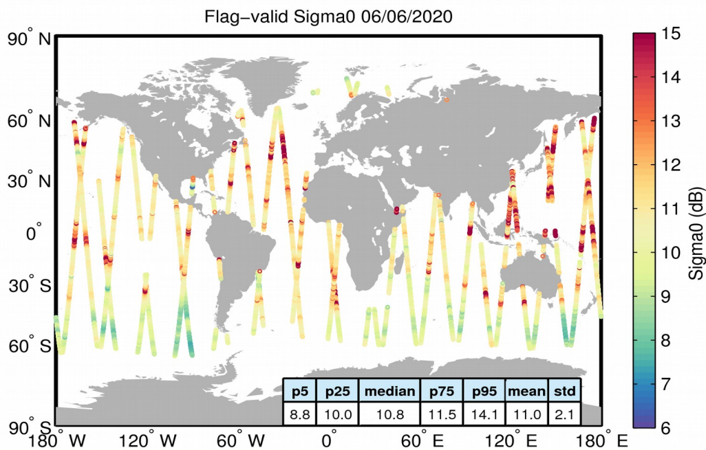
Figure 23. Geographical distribution of flag-valid sigma0 data over oceans and lakes for 06/06/2020. The statistical values shown in the table refer to the sigma0 in dB and are calculated over all measurements shown in the figure.
