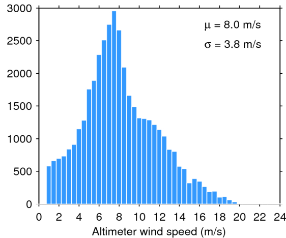
Figure 33. Histogram of flag-valid wind over oceans and lakes for 06/06/2020. The mean ( \mu ) and standard deviation ( \sigma ) are also shown. Note that values larger than 24 m/s are excluded from the histogram for the sake of readability but not from the computation of \mu and \sigma .
