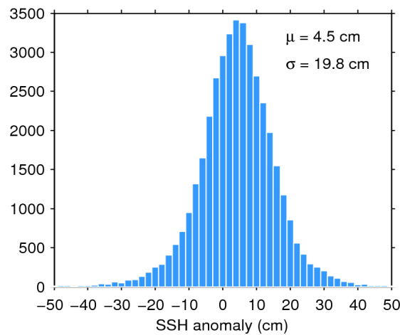
Figure 7. Histogram of flag-valid SSH anomaly over oceans and lakes for 06/06/2020. The mean ( \mu ) and standard deviation ( \sigma ) are also shown. Note that values outside [-50\ 50] cm are excluded from the histogram for the sake of readability but not from the computation of \mu and \sigma .
