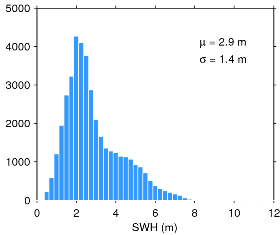
Figure 17. Histogram of flag-valid SWH over oceans and lakes for 06/06/2020. The mean ( \mu ) and standard deviation ( \sigma ) are also shown. Note that values larger than 12 m are excluded from the histogram for the sake of readability but not from the computation of \mu and \sigma .
