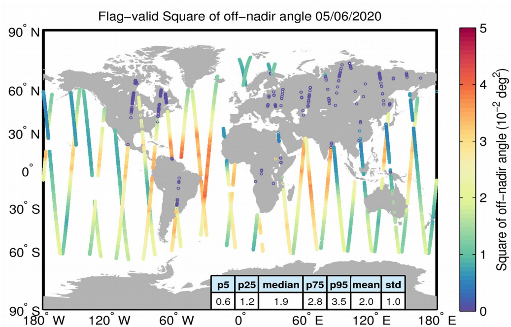
Figure 37. Geographical distribution of flag-valid mispointing data over oceans and lakes for 05/06/2020. The statistical values shown in the table refer to the mispointing in 10^{-2} \text{ deg}^2 and are calculated over all measurements shown in the figure.
