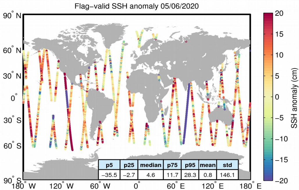
Figure 5. Geographical distribution of flag-valid 1-Hz SSH anomaly data over oceans and lakes for 05/06/2020. The statistical values shown in the table refer to the SSH anomaly in cm and are calculated over all measurements shown in the figure.
