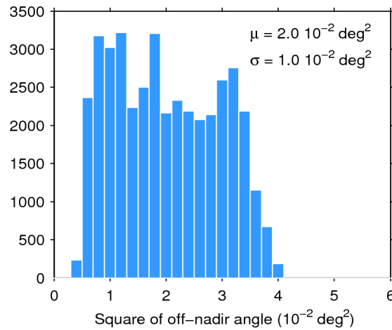
Figure 39. Histogram of flag-valid mispointing over oceans and lakes for 05/06/2020. The mean ( \mu ) and standard deviation ( \sigma ) are also shown. Note that values larger than 6 \cdot 10^{-2} \text{ deg}^2 are excluded from the histogram for the sake of readability but not from the computation of \mu and \sigma .
