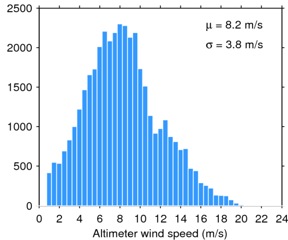
Figure 33. Histogram of flag-valid wind over oceans and lakes for 05/06/2020. The mean ( \mu ) and standard deviation ( \sigma ) are also shown. Note that values larger than 24 m/s are excluded from the histogram for the sake of readability but not from the computation of \mu and \sigma .
