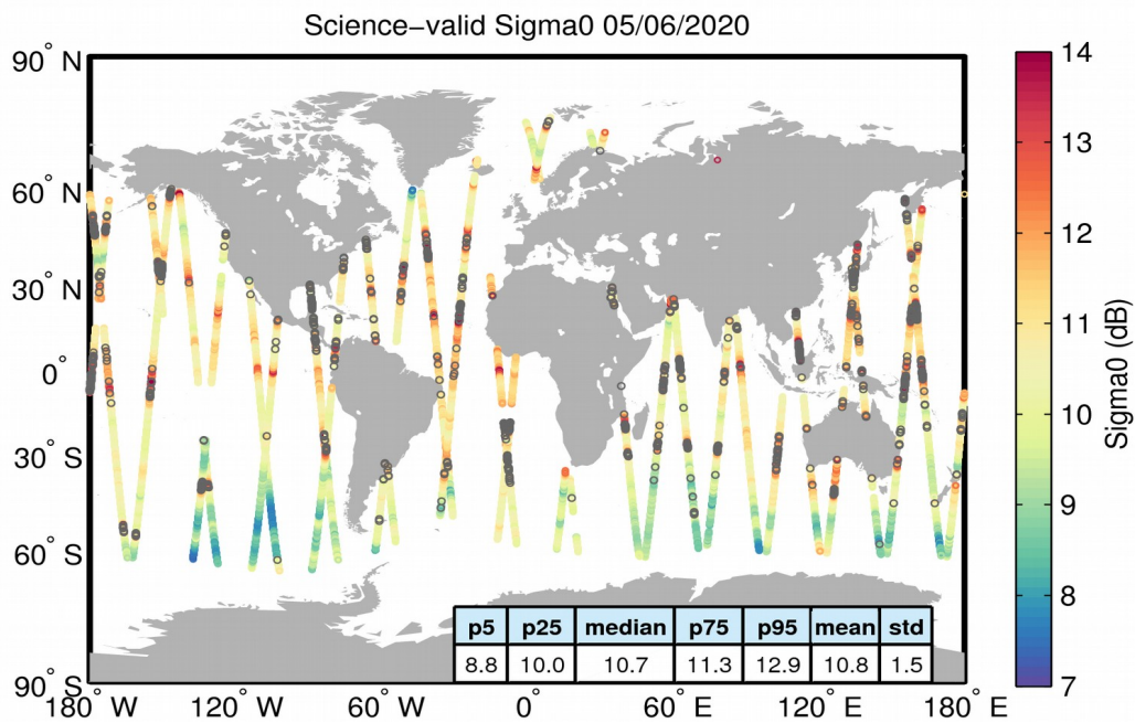
Figure 27. Geographical distribution of science-valid sigma0 data over oceans and lakes for 05/06/2020. The statistical values shown in the table refer to the sigma0 in dB and are calculated over all measurements shown in the figure. Gray circles denote records that have been rejected based on the editing criteria described in Table 4.
