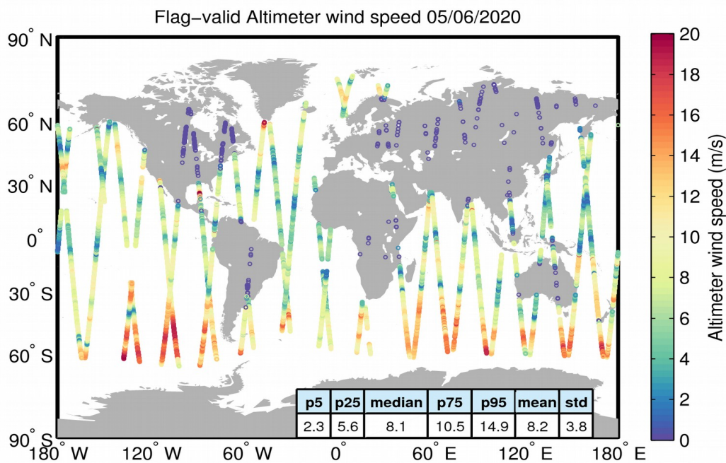
Figure 31. Geographical distribution of flag-valid wind data over oceans and lakes for 05/06/2020. The statistical values shown in the table refer to the wind in m/s and are calculated over all measurements shown in the figure.
