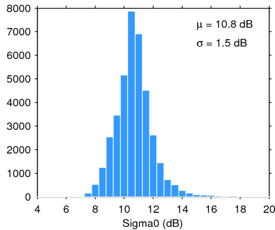
Figure 28. Histogram of science-valid sigma0 over oceans and lakes for 05/06/2020. The mean ( \mu ) and standard deviation ( \sigma ) are also shown. Note that values outside [4 20] dB are excluded from the histogram for the sake of readability but not from the computation of \mu and \sigma .
