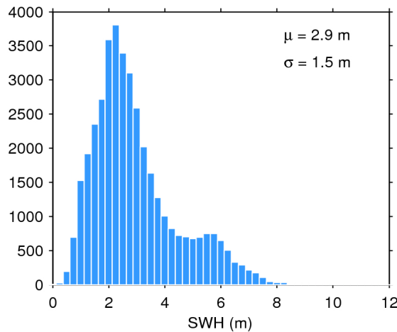
Figure 20. Histogram of science-valid SWH over oceans and lakes for 05/06/2020. The mean ( \mu ) and standard deviation ( \sigma ) are also shown. Note that values larger than 12 m are excluded from the histogram for the sake of readability but not from the computation of \mu and \sigma .
