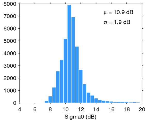
Figure 25. Histogram of flag-valid sigma0 over oceans and lakes for 05/06/2020. The mean ( \mu ) and standard deviation ( \sigma ) are also shown. Note that values outside [4 20] dB are excluded from the histogram for the sake of readability but not from the computation of \mu and \sigma .
