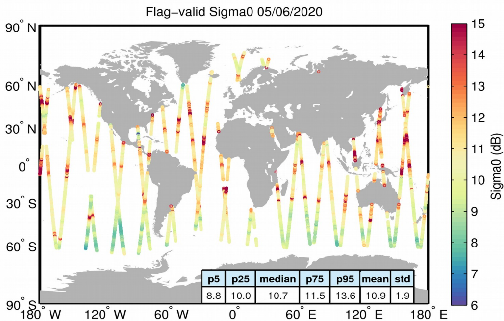
Figure 23. Geographical distribution of flag-valid sigma0 data over oceans and lakes for 05/06/2020. The statistical values shown in the table refer to the sigma0 in dB and are calculated over all measurements shown in the figure.
