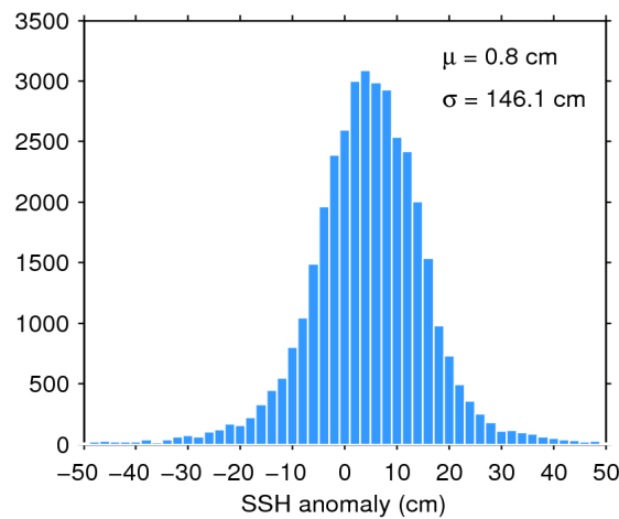
Figure 7. Histogram of flag-valid SSH anomaly over oceans and lakes for 05/06/2020. The mean ( \mu ) and standard deviation ( \sigma ) are also shown. Note that values outside [-50 50] cm are excluded from the histogram for the sake of readability but not from the computation of \mu and \sigma .
