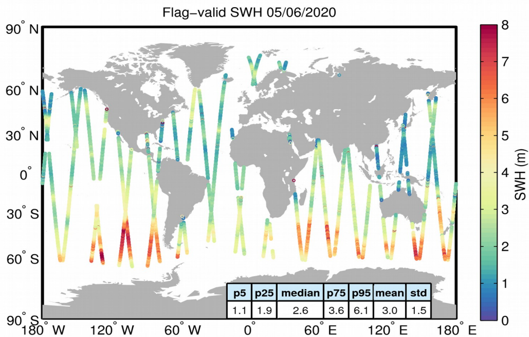
Figure 15. Geographical distribution of flag-valid SWH data over oceans and lakes for 05/06/2020. The statistical values shown in the table refer to the SWH in m and are calculated over all measurements shown in the figure.
