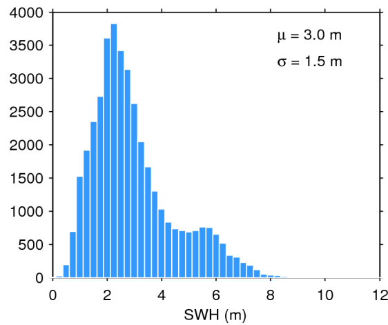
Figure 17. Histogram of flag-valid SWH over oceans and lakes for 05/06/2020. The mean ( \mu ) and standard deviation ( \sigma ) are also shown. Note that values larger than 12 m are excluded from the histogram for the sake of readability but not from the computation of \mu and \sigma .
