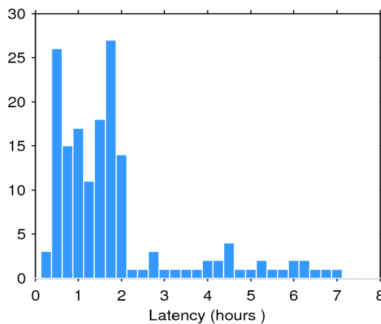
Figure 2. Histogram of the data latency for 05/06/2020. The y-axis denotes the number of files that are made available with a delay of x-hours with respect to the mean time of the records stored in the file.
