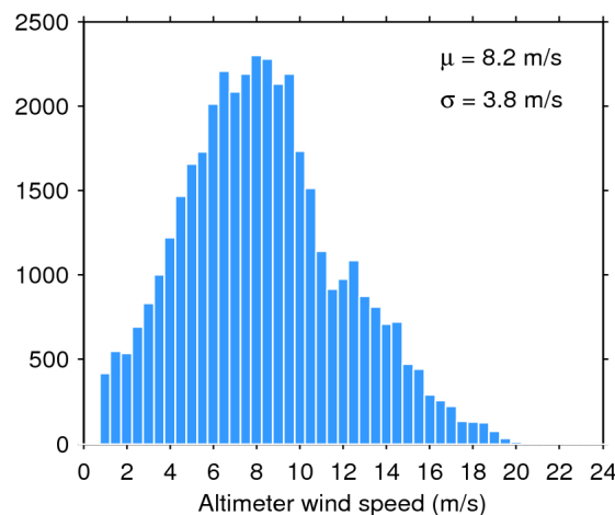
Figure 35. Histogram of science-valid wind over oceans and lakes for 05/06/2020. The mean ( \mu ) and standard deviation ( \sigma ) are also shown. Note that values larger than 24 m/s are excluded from the histogram for the sake of readability but not from the computation of \mu and \sigma .
