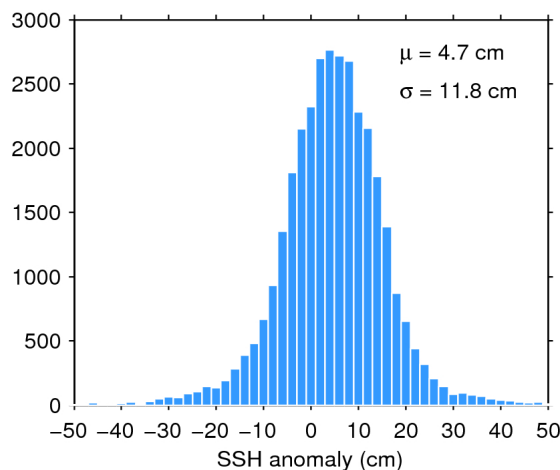
Figure 11. Histogram of science-valid SSH anomaly over oceans and lakes for 05/06/2020. The mean ( \mu ) and standard deviation ( \sigma ) are also shown. Note that values outside [-50 50] cm are excluded from the histogram for the sake of readability but not from the computation of \mu and \sigma .
