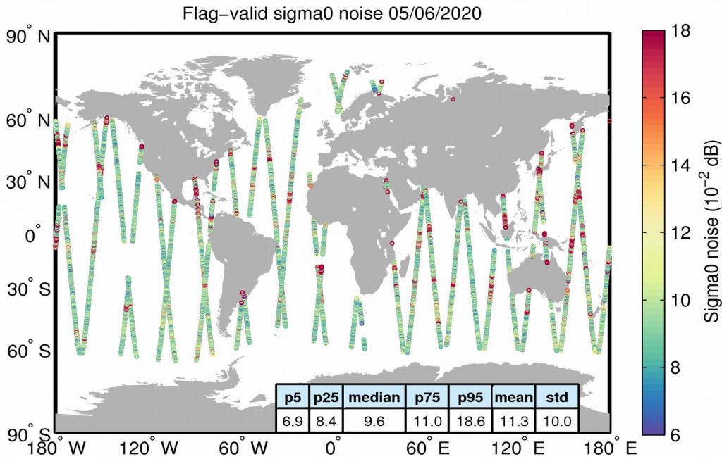
Figure 26. Geographical distribution of flag-valid 20-Hz sigma0 measurement noise over oceans and lakes for 05/06/2020. The statistical values shown in the table refer to the sigma0 noise and are calculated over all measurements shown in the figure.
