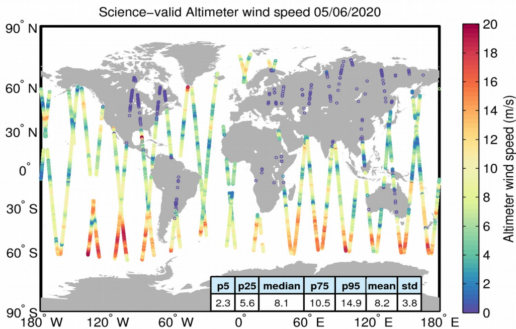
Figure 34. Geographical distribution of science-valid wind data over oceans and lakes for 05/06/2020. The statistical values shown in the table refer to the wind in m/s and are calculated over all measurements shown in the figure. Gray circles denote records that have been rejected based on the editing criteria described in Table 5.
