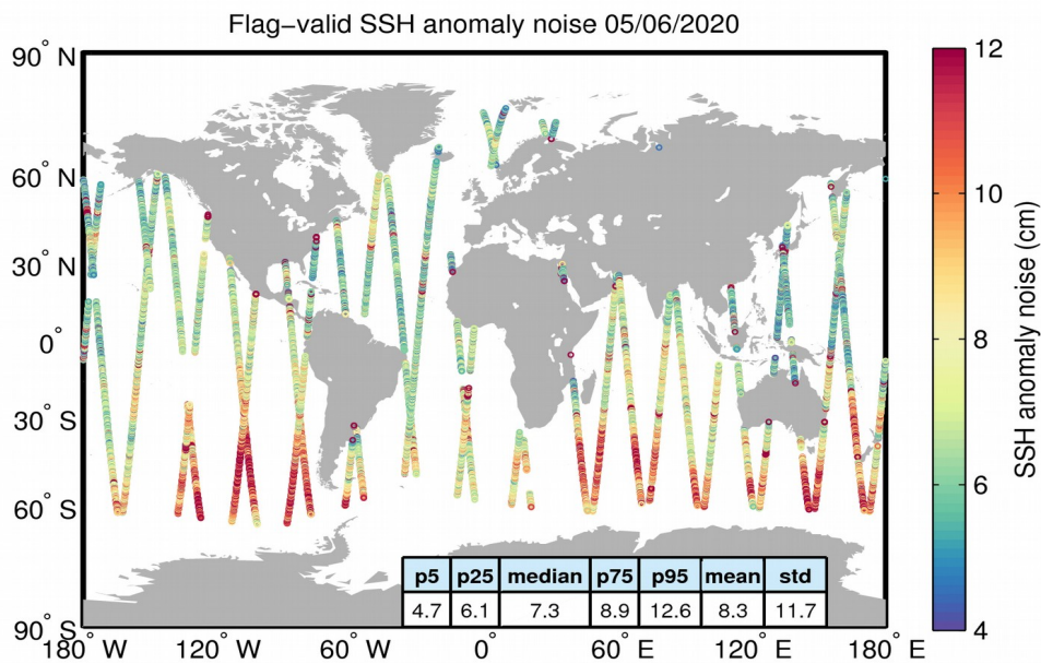
Figure 8. Geographical distribution of flag-valid 20-Hz SSH anomaly measurement noise over oceans and lakes for 05/06/2020. The statistical values shown in the table refer to the SSH anomaly noise and are calculated over all measurements shown in the figure.
