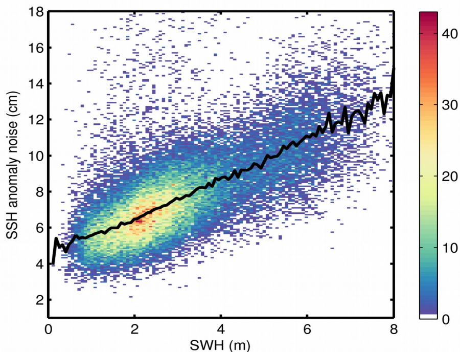
Figure 9. 2D histogram showing flag-valid SSH anomaly noise as a function of SWH for 05/06/2020. The black line denotes the median SSH anomaly noise as a function of SWH.
