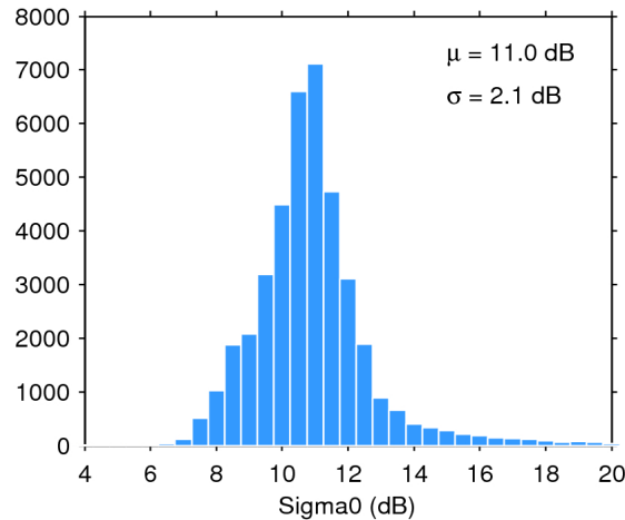
Figure 25. Histogram of flag-valid sigma0 over oceans and lakes for 04/06/2020. The mean ( \mu ) and standard deviation ( \sigma ) are also shown. Note that values outside [4 20] dB are excluded from the histogram for the sake of readability but not from the computation of \mu and \sigma .
