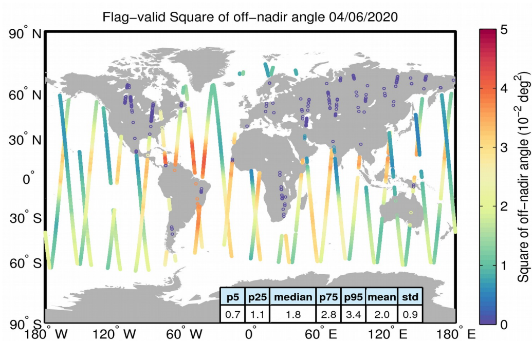
Figure 37. Geographical distribution of flag-valid mispointing data over oceans and lakes for 04/06/2020. The statistical values shown in the table refer to the mispointing in 10^{-2} \text{ deg}^2 and are calculated over all measurements shown in the figure.
