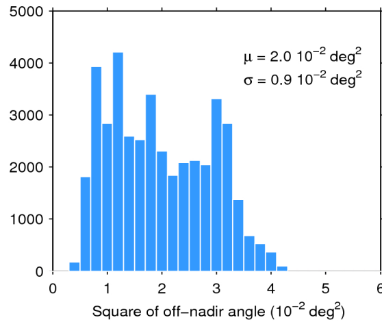
Figure 39. Histogram of flag-valid mispointing over oceans and lakes for 04/06/2020. The mean ( \mu ) and standard deviation ( \sigma ) are also shown. Note that values larger than 6 \cdot 10^{-2} \text{ deg}^2 are excluded from the histogram for the sake of readability but not from the computation of \mu and \sigma .
