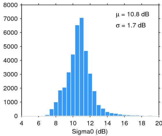
Figure 28. Histogram of science-valid sigma0 over oceans and lakes for 04/06/2020. The mean ( \mu ) and standard deviation ( \sigma ) are also shown. Note that values outside [4 20] dB are excluded from the histogram for the sake of readability but not from the computation of \mu and \sigma .
