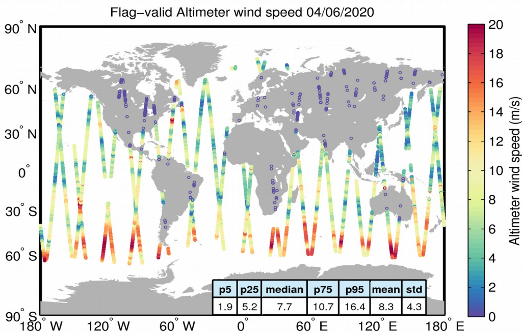
Figure 31. Geographical distribution of flag-valid wind data over oceans and lakes for 04/06/2020. The statistical values shown in the table refer to the wind in m/s and are calculated over all measurements shown in the figure.
