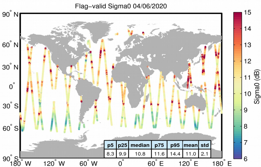
Figure 23. Geographical distribution of flag-valid sigma0 data over oceans and lakes for 04/06/2020. The statistical values shown in the table refer to the sigma0 in dB and are calculated over all measurements shown in the figure.
