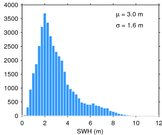
Figure 20. Histogram of science-valid SWH over oceans and lakes for 04/06/2020. The mean ( \mu ) and standard deviation ( \sigma ) are also shown. Note that values larger than 12 m are excluded from the histogram for the sake of readability but not from the computation of \mu and \sigma .
