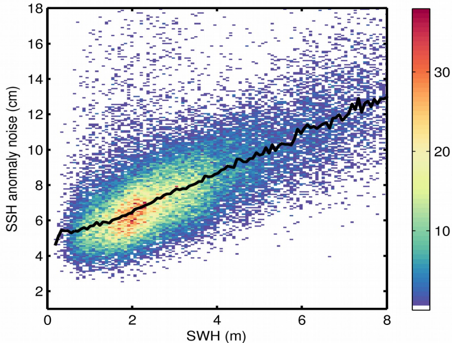
Figure 9. 2D histogram showing flag-valid SSH anomaly noise as a function of SWH for 04/06/2020. The black line denotes the median SSH anomaly noise as a function of SWH.
