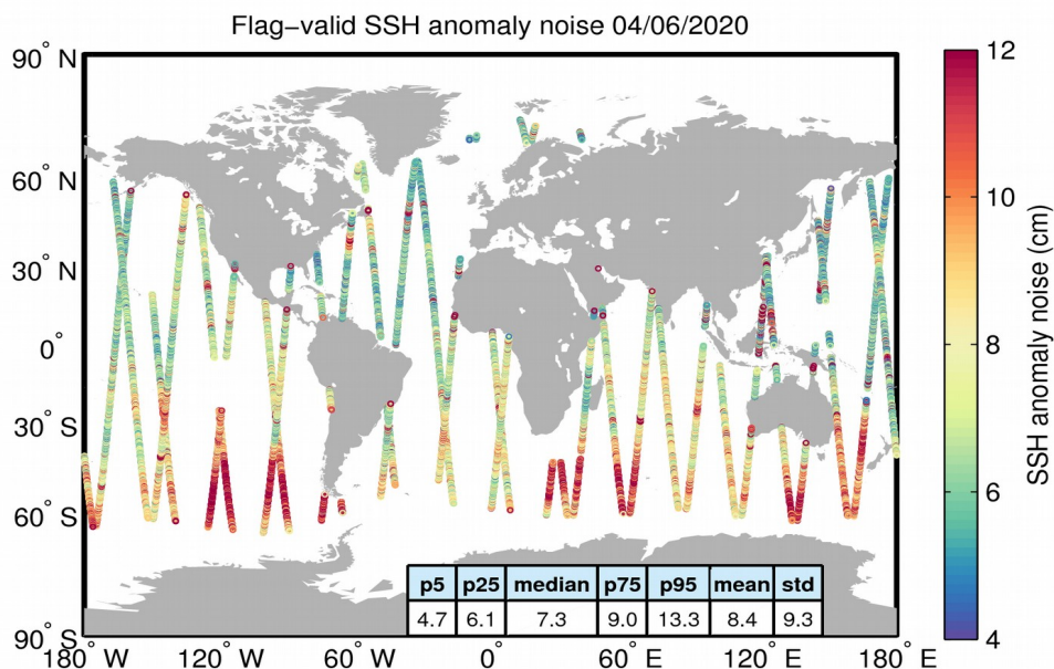
Figure 8. Geographical distribution of flag-valid 20-Hz SSH anomaly measurement noise over oceans and lakes for 04/06/2020. The statistical values shown in the table refer to the SSH anomaly noise and are calculated over all measurements shown in the figure.
