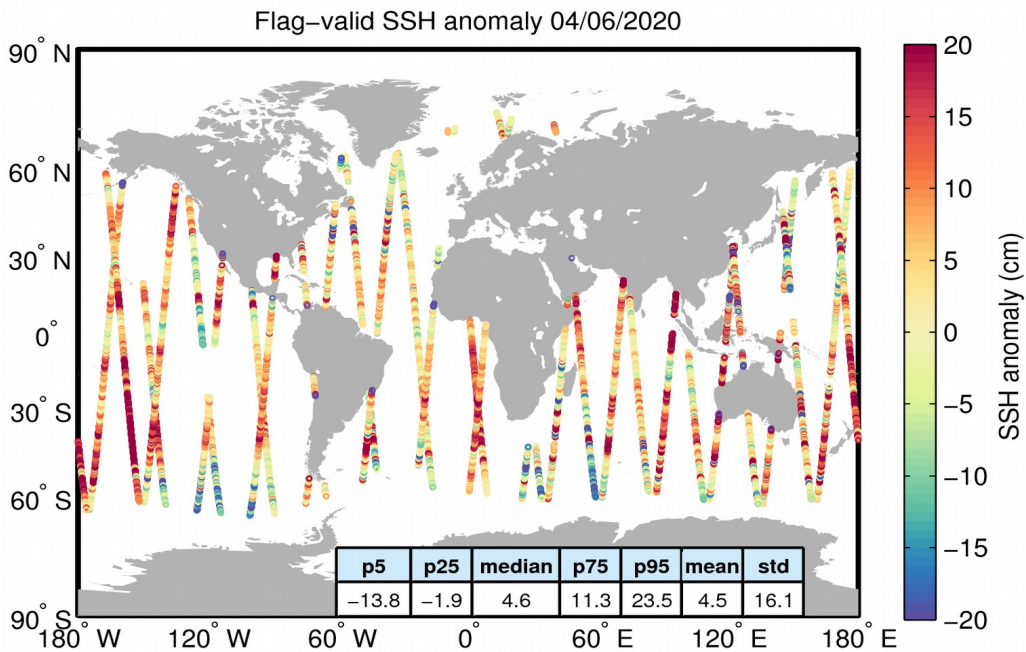
Figure 5. Geographical distribution of flag-valid 1-Hz SSH anomaly data over oceans and lakes for 04/06/2020. The statistical values shown in the table refer to the SSH anomaly in cm and are calculated over all measurements shown in the figure.
