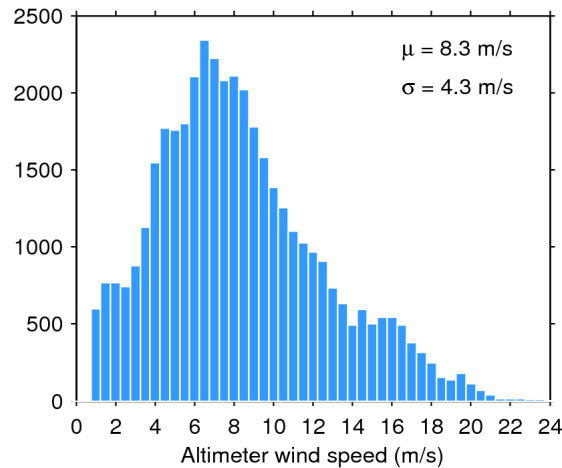
Figure 33. Histogram of flag-valid wind over oceans and lakes for 04/06/2020. The mean ( \mu ) and standard deviation ( \sigma ) are also shown. Note that values larger than 24 m/s are excluded from the histogram for the sake of readability but not from the computation of \mu and \sigma .
