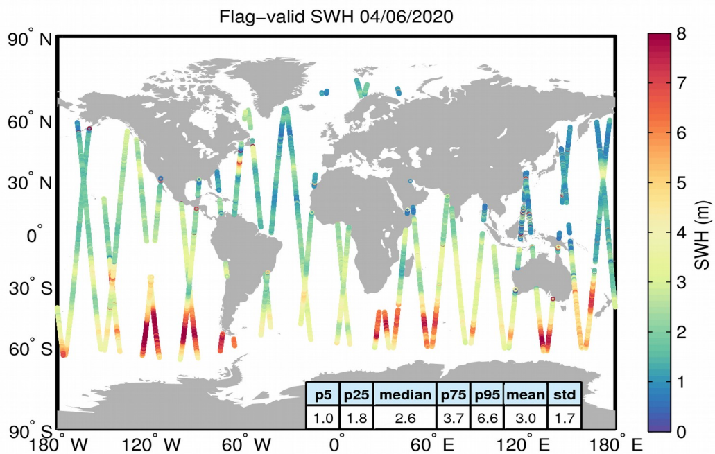
Figure 15. Geographical distribution of flag-valid SWH data over oceans and lakes for 04/06/2020. The statistical values shown in the table refer to the SWH in m and are calculated over all measurements shown in the figure.
