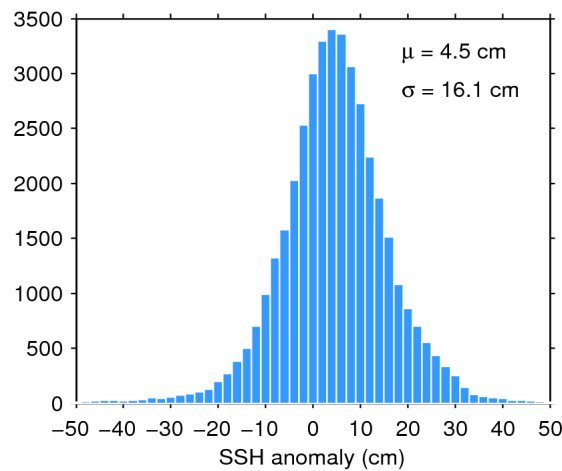
Figure 7. Histogram of flag-valid SSH anomaly over oceans and lakes for 04/06/2020. The mean ( \mu ) and standard deviation ( \sigma ) are also shown. Note that values outside [-50\ 50] cm are excluded from the histogram for the sake of readability but not from the computation of \mu and \sigma .
