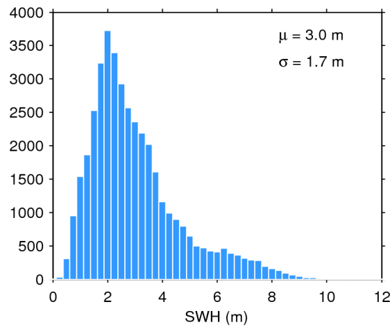
Figure 17. Histogram of flag-valid SWH over oceans and lakes for 04/06/2020. The mean ( \mu ) and standard deviation ( \sigma ) are also shown. Note that values larger than 12 m are excluded from the histogram for the sake of readability but not from the computation of \mu and \sigma .
