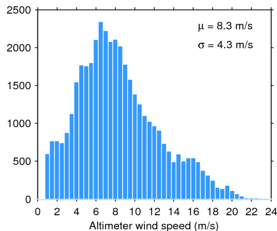
Figure 35. Histogram of science-valid wind over oceans and lakes for 04/06/2020. The mean ( \mu ) and standard deviation ( \sigma ) are also shown. Note that values larger than 24 m/s are excluded from the histogram for the sake of readability but not from the computation of \mu and \sigma .
