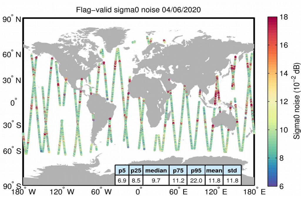
Figure 26. Geographical distribution of flag-valid 20-Hz sigma0 measurement noise over oceans and lakes for 04/06/2020. The statistical values shown in the figure refer to the sigma0 noise and are calculated over all measurements shown in the figure.
