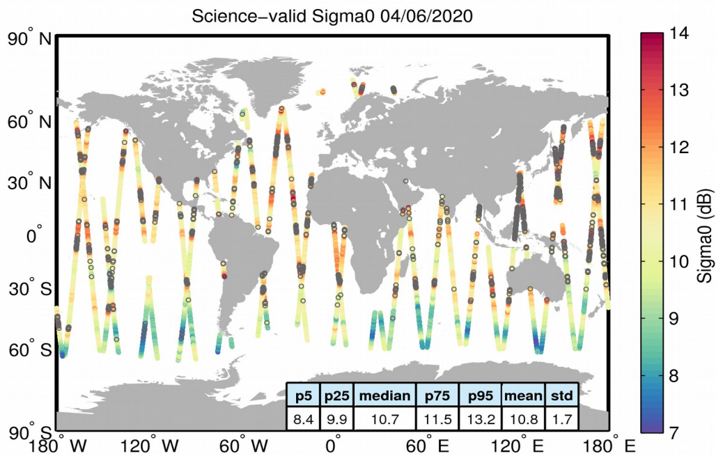
Figure 27. Geographical distribution of science-valid sigma0 data over oceans and lakes for 04/06/2020. The statistical values shown in the table refer to the sigma0 in dB and are calculated over all measurements shown in the figure. Gray circles denote records that have been rejected based on the editing criteria described in Table 4.
