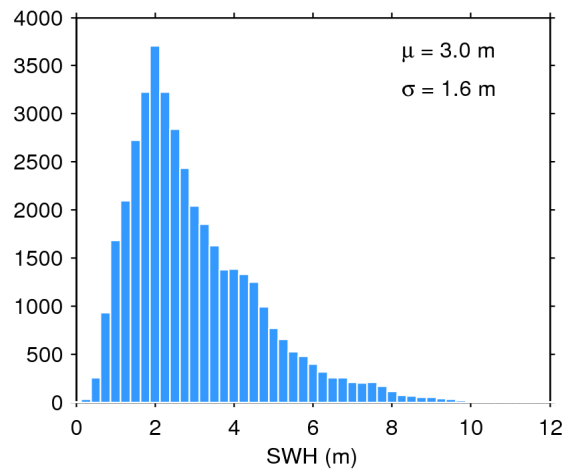
Figure 17. Histogram of flag-valid SWH over oceans and lakes for 03/06/2020. The mean ( \mu ) and standard deviation ( \sigma ) are also shown. Note that values larger than 12 m are excluded from the histogram for the sake of readability but not from the computation of \mu and \sigma .
