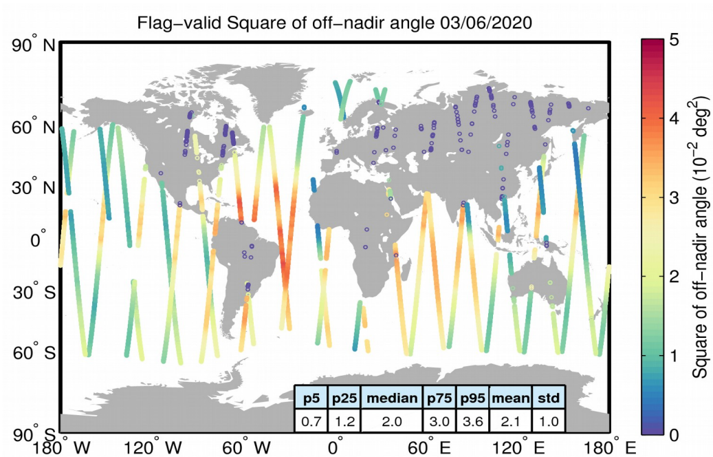
Figure 37. Geographical distribution of flag-valid mispointing data over oceans and lakes for 03/06/2020. The statistical values shown in the table refer to the mispointing in 10^{-2} deg 2 and are calculated over all measurements shown in the figure.
