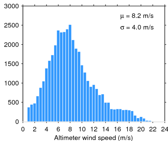
Figure 35. Histogram of science-valid wind over oceans and lakes for 03/06/2020. The mean ( \mu ) and standard deviation ( \sigma ) are also shown. Note that values larger than 24 m/s are excluded from the histogram for the sake of readability but not from the computation of \mu and \sigma .
