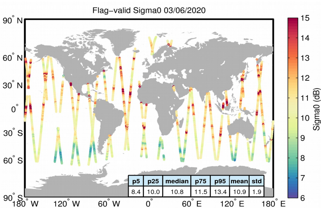
Figure 23. Geographical distribution of flag-valid sigma0 data over oceans and lakes for 03/06/2020. The statistical values shown in the table refer to the sigma0 in dB and are calculated over all measurements shown in the figure.
