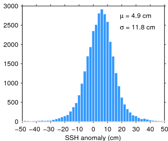
Figure 11. Histogram of science-valid SSH anomaly over oceans and lakes for 03/06/2020. The mean ( \mu ) and standard deviation ( \sigma ) are also shown. Note that values outside [-50 50] cm are excluded from the histogram for the sake of readability but not from the computation of \mu and \sigma .
