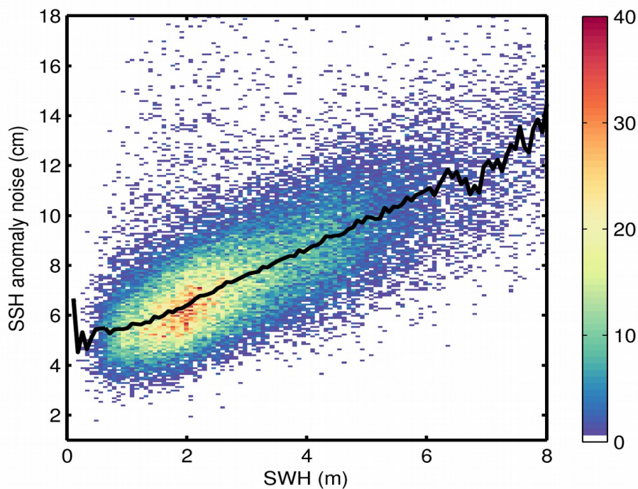
Figure 9. 2D histogram showing flag-valid SSH anomaly noise as a function of SWH for 03/06/2020. The black line denotes the median SSH anomaly noise as a function of SWH.
