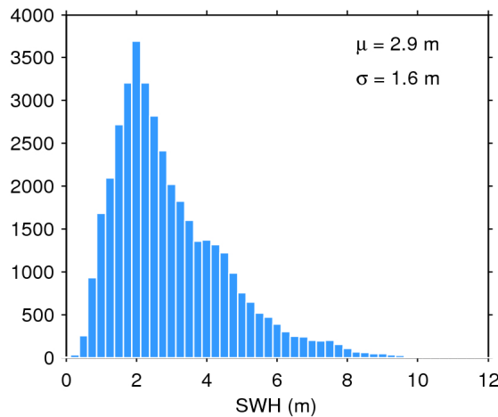
Figure 20. Histogram of science-valid SWH over oceans and lakes for 03/06/2020. The mean ( \mu ) and standard deviation ( \sigma ) are also shown. Note that values larger than 12 m are excluded from the histogram for the sake of readability but not from the computation of \mu and \sigma .
