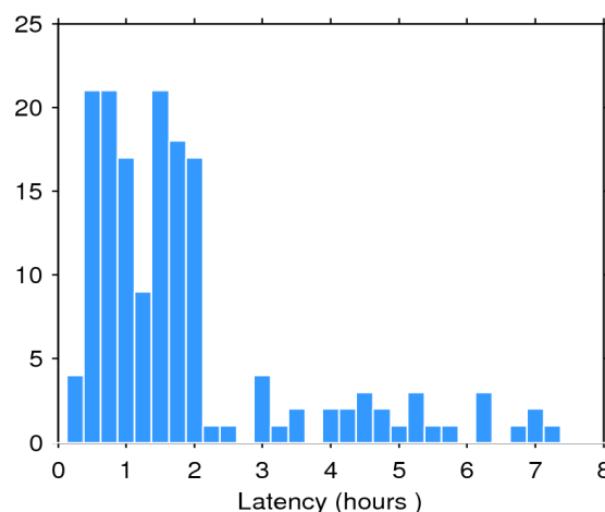
Figure 2. Histogram of the data latency for 03/06/2020. The y-axis denotes the number of files that are made available with a delay of x-hours with respect to the mean time of the records stored in the file.
