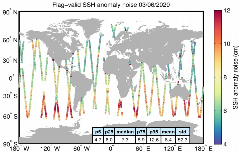
Figure 8. Geographical distribution of flag-valid 20-Hz SSH anomaly measurement noise over oceans and lakes for 03/06/2020. The statistical values shown in the table refer to the SSH anomaly noise and are calculated over all measurements shown in the figure.
