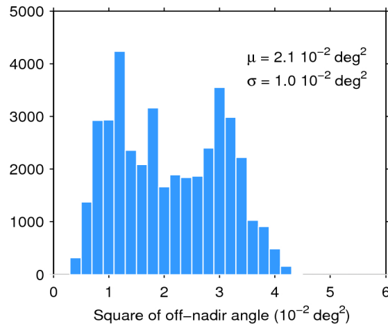
Figure 39. Histogram of flag-valid mispointing over oceans and lakes for 03/06/2020. The mean ( \mu ) and standard deviation ( \sigma ) are also shown. Note that values larger than 6 \cdot 10^{-2} \text{ deg}^2 are excluded from the histogram for the sake of readability but not from the computation of \mu and \sigma .
