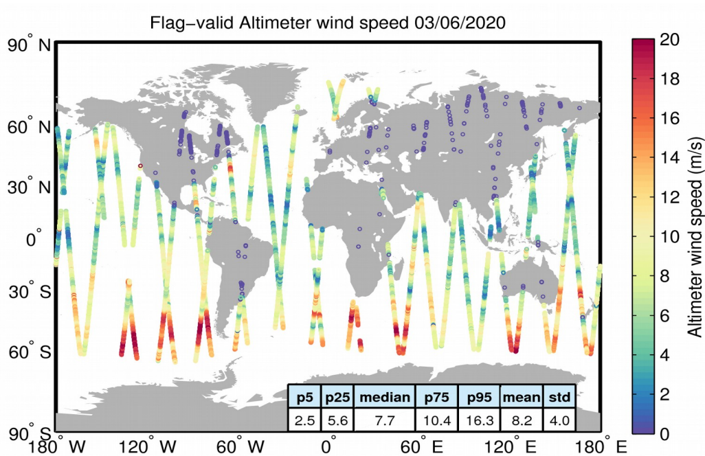
Figure 31. Geographical distribution of flag-valid wind data over oceans and lakes for 03/06/2020. The statistical values shown in the table refer to the wind in m/s and are calculated over all measurements shown in the figure.
