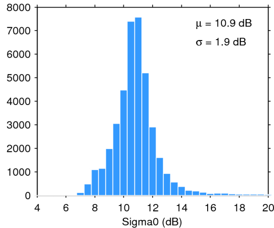
Figure 25. Histogram of flag-valid sigma0 over oceans and lakes for 03/06/2020. The mean ( \mu ) and standard deviation ( \sigma ) are also shown. Note that values outside [4 20] dB are excluded from the histogram for the sake of readability but not from the computation of \mu and \sigma .
