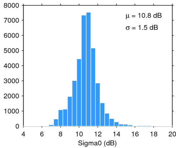
Figure 28. Histogram of science-valid sigma0 over oceans and lakes for 03/06/2020. The mean ( \mu ) and standard deviation ( \sigma ) are also shown. Note that values outside [4 20] dB are excluded from the histogram for the sake of readability but not from the computation of \mu and \sigma .
