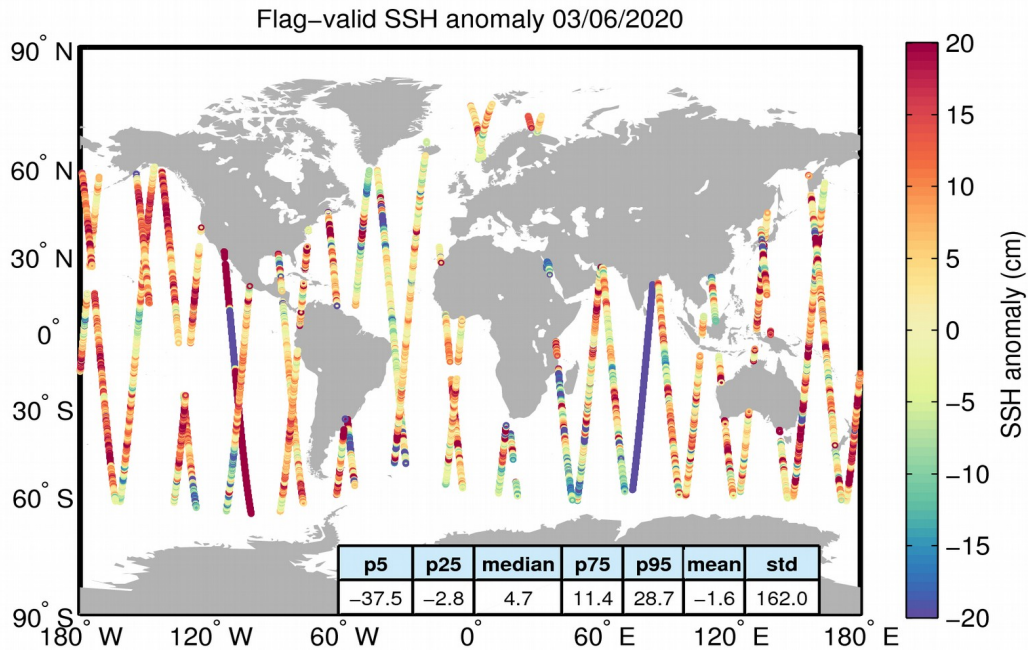
Figure 5. Geographical distribution of flag-valid 1-Hz SSH anomaly data over oceans and lakes for 03/06/2020. The statistical values shown in the table refer to the SSH anomaly in cm and are calculated over all measurements shown in the figure.
