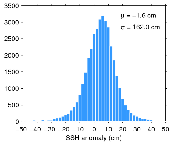
Figure 7. Histogram of flag-valid SSH anomaly over oceans and lakes for 03/06/2020. The mean ( \mu ) and standard deviation ( \sigma ) are also shown. Note that values outside [-50 50] cm are excluded from the histogram for the sake of readability but not from the computation of \mu and \sigma .
