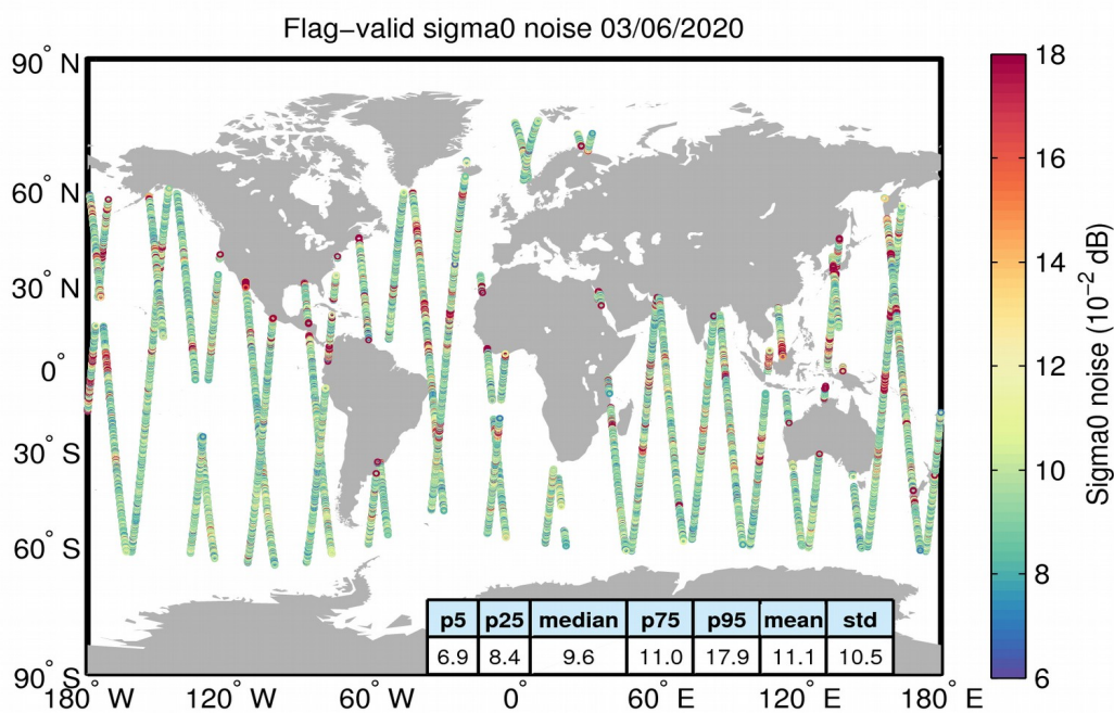
Figure 26. Geographical distribution of flag-valid 20-Hz sigma0 measurement noise over oceans and lakes for 03/06/2020. The statistical values shown in the figure refer to the sigma0 noise and are calculated over all measurements shown in the figure.
