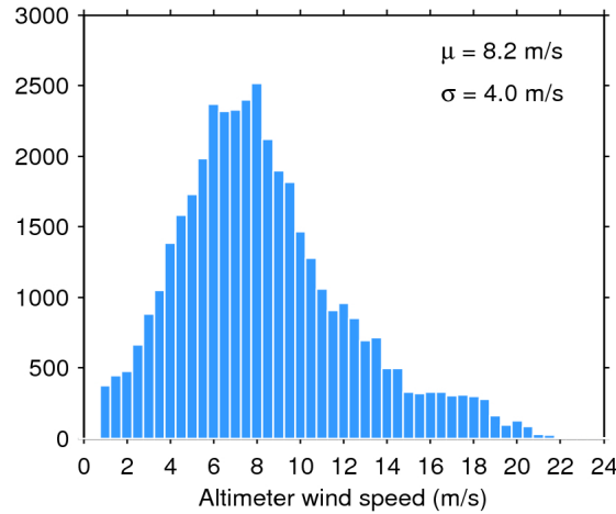
Figure 33. Histogram of flag-valid wind over oceans and lakes for 03/06/2020. The mean ( \mu ) and standard deviation ( \sigma ) are also shown. Note that values larger than 24 m/s are excluded from the histogram for the sake of readability but not from the computation of \mu and \sigma .
