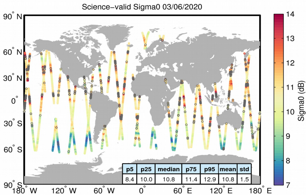
Figure 27. Geographical distribution of science-valid sigma0 data over oceans and lakes for 03/06/2020. The statistical values shown in the table refer to the sigma0 in dB and are calculated over all measurements shown in the figure. Gray circles denote records that have been rejected based on the editing criteria described in Table 4.
