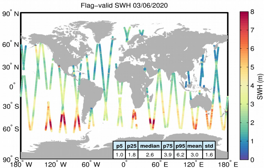
Figure 15. Geographical distribution of flag-valid SWH data over oceans and lakes for 03/06/2020. The statistical values shown in the table refer to the SWH in m and are calculated over all measurements shown in the figure.
