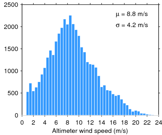
Figure 33. Histogram of flag-valid wind over oceans and lakes for 02/06/2020. The mean ( \mu ) and standard deviation ( \sigma ) are also shown. Note that values larger than 24 m/s are excluded from the histogram for the sake of readability but not from the computation of \mu and \sigma .
