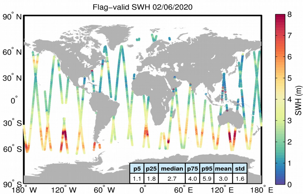
Figure 15. Geographical distribution of flag-valid SWH data over oceans and lakes for 02/06/2020. The statistical values shown in the table refer to the SWH in m and are calculated over all measurements shown in the figure.
