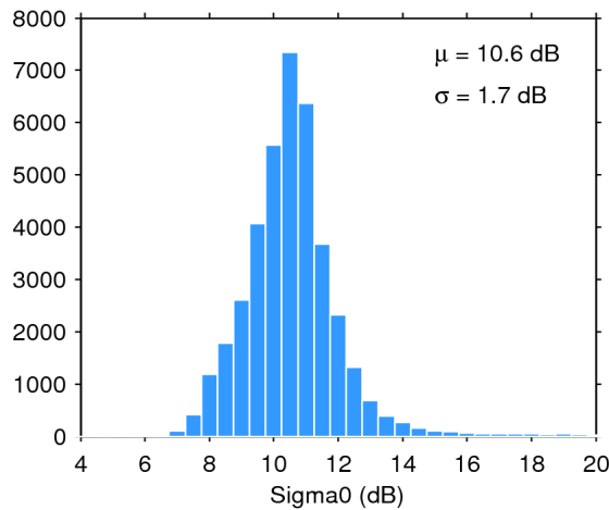
Figure 28. Histogram of science-valid sigma0 over oceans and lakes for 02/06/2020. The mean ( \mu ) and standard deviation ( \sigma ) are also shown. Note that values outside [4 20] dB are excluded from the histogram for the sake of readability but not from the computation of \mu and \sigma .
