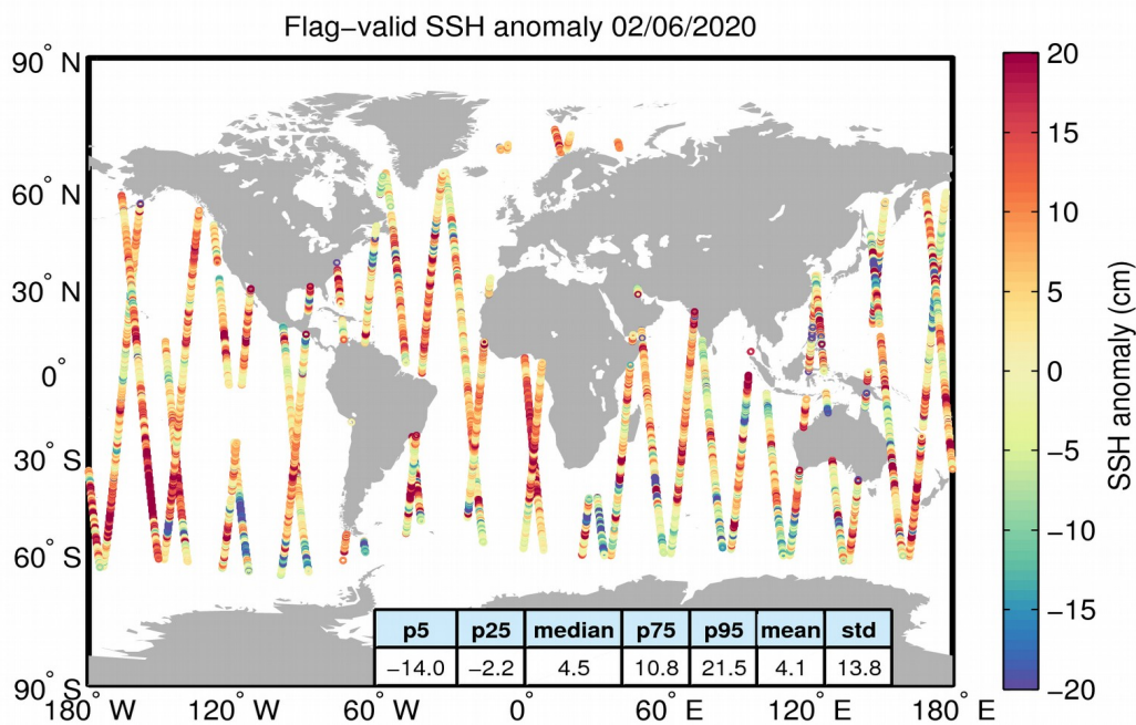
Figure 5. Geographical distribution of flag-valid 1-Hz SSH anomaly data over oceans and lakes for 02/06/2020. The statistical values shown in the table refer to the SSH anomaly in cm and are calculated over all measurements shown in the figure.
