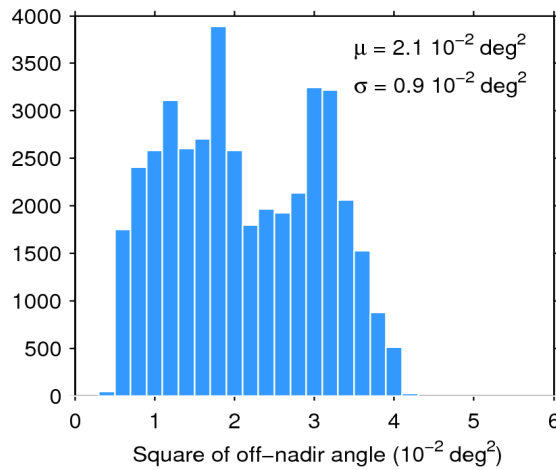
Figure 39. Histogram of flag-valid mispointing over oceans and lakes for 02/06/2020. The mean ( \mu ) and standard deviation ( \sigma ) are also shown. Note that values larger than 6 \cdot 10^{-2} \text{ deg}^2 are excluded from the histogram for the sake of readability but not from the computation of \mu and \sigma .
