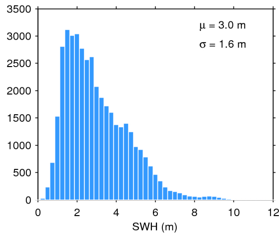
Figure 17. Histogram of flag-valid SWH over oceans and lakes for 02/06/2020. The mean ( \mu ) and standard deviation ( \sigma ) are also shown. Note that values larger than 12 m are excluded from the histogram for the sake of readability but not from the computation of \mu and \sigma .
