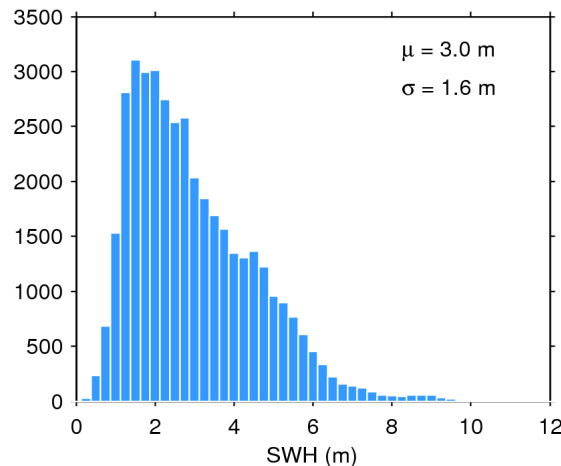
Figure 20. Histogram of science-valid SWH over oceans and lakes for 02/06/2020. The mean ( \mu ) and standard deviation ( \sigma ) are also shown. Note that values larger than 12 m are excluded from the histogram for the sake of readability but not from the computation of \mu and \sigma .
