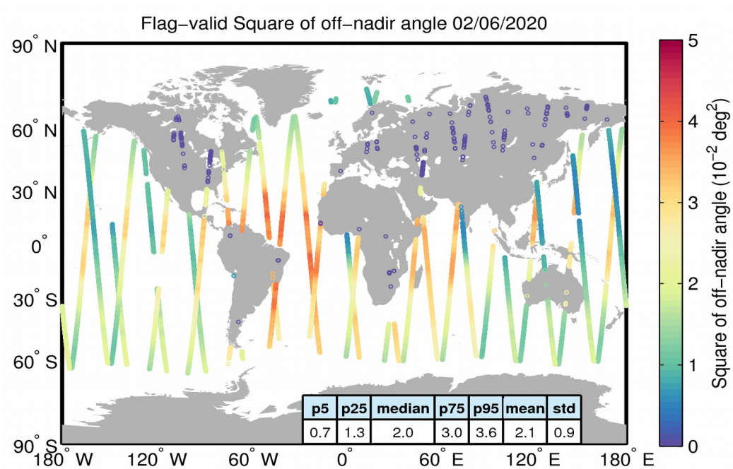
Figure 37. Geographical distribution of flag-valid mispointing data over oceans and lakes for 02/06/2020. The statistical values shown in the table refer to the mispointing in 10^{-2} \text{ deg}^2 and are calculated over all measurements shown in the figure.
