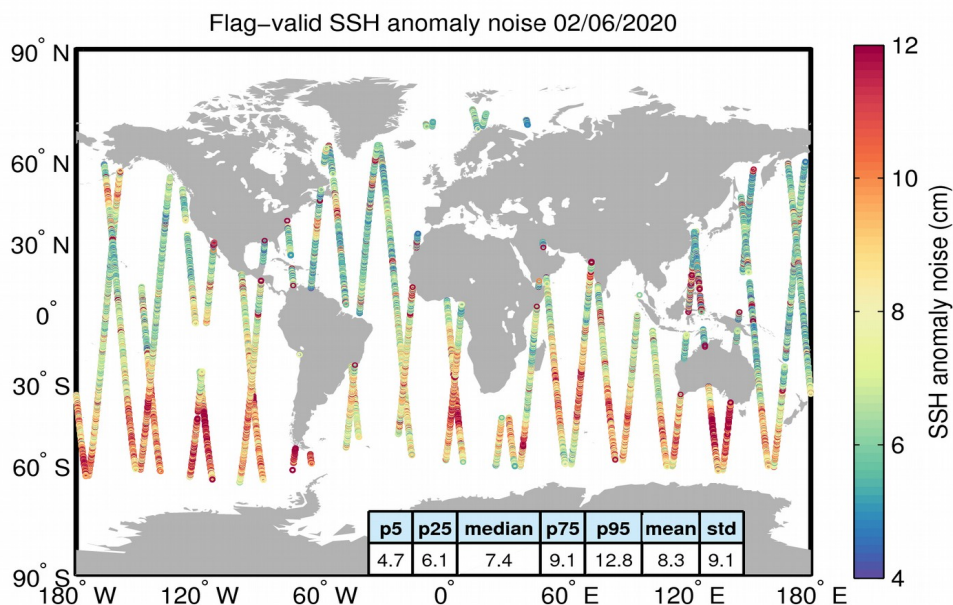
Figure 8. Geographical distribution of flag-valid 20-Hz SSH anomaly measurement noise over oceans and lakes for 02/06/2020. The statistical values shown in the table refer to the SSH anomaly noise and are calculated over all measurements shown in the figure.
