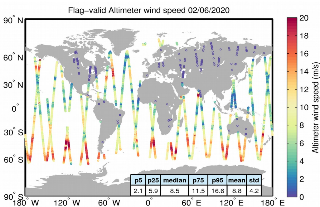
Figure 31. Geographical distribution of flag-valid wind data over oceans and lakes for 02/06/2020. The statistical values shown in the table refer to the wind in m/s and are calculated over all measurements shown in the figure.
