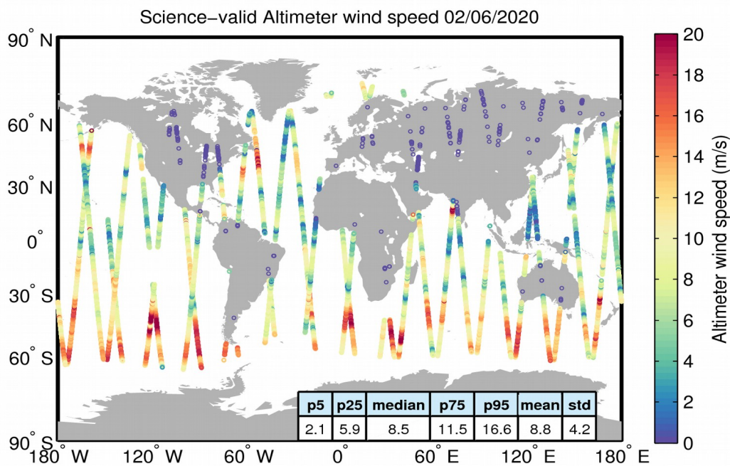
Figure 34. Geographical distribution of science-valid wind data over oceans and lakes for 02/06/2020. The statistical values shown in the table refer to the wind in m/s and are calculated over all measurements shown in the figure. Gray circles denote records that have been rejected based on the editing criteria described in Table 5.
