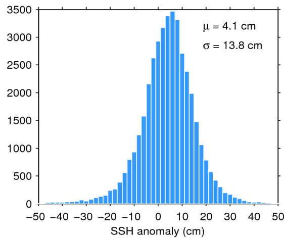
Figure 7. Histogram of flag-valid SSH anomaly over oceans and lakes for 02/06/2020. The mean ( \mu ) and standard deviation ( \sigma ) are also shown. Note that values outside [-50\ 50] cm are excluded from the histogram for the sake of readability but not from the computation of \mu and \sigma .
