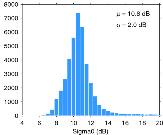
Figure 25. Histogram of flag-valid sigma0 over oceans and lakes for 02/06/2020. The mean ( \mu ) and standard deviation ( \sigma ) are also shown. Note that values outside [4 20] dB are excluded from the histogram for the sake of readability but not from the computation of \mu and \sigma .
