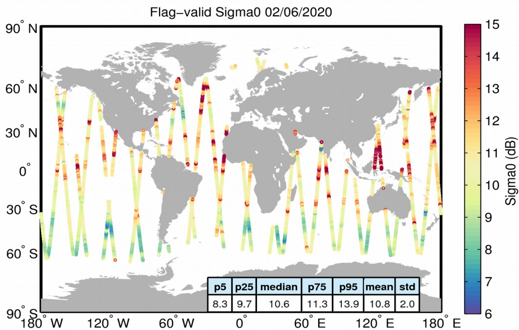
Figure 23. Geographical distribution of flag-valid sigma0 data over oceans and lakes for 02/06/2020. The statistical values shown in the table refer to the sigma0 in dB and are calculated over all measurements shown in the figure.
