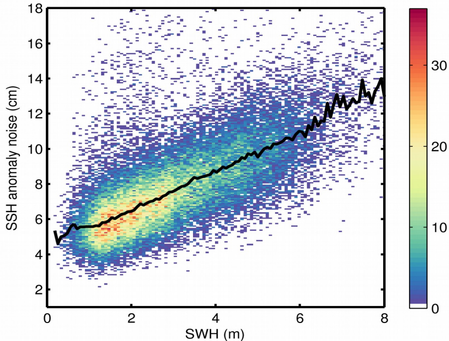
Figure 9. 2D histogram showing flag-valid SSH anomaly noise as a function of SWH for 02/06/2020. The black line denotes the median SSH anomaly noise as a function of SWH.
