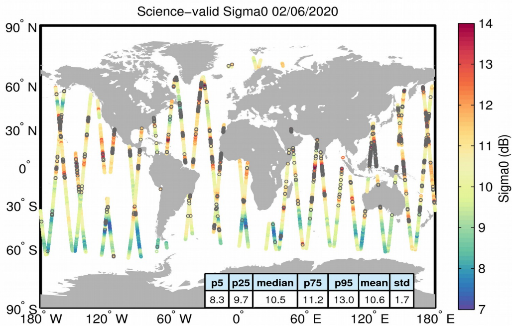
Figure 27. Geographical distribution of science-valid sigma0 data over oceans and lakes for 02/06/2020. The statistical values shown in the table refer to the sigma0 in dB and are calculated over all measurements shown in the figure. Gray circles denote records that have been rejected based on the editing criteria described in Table 4.
