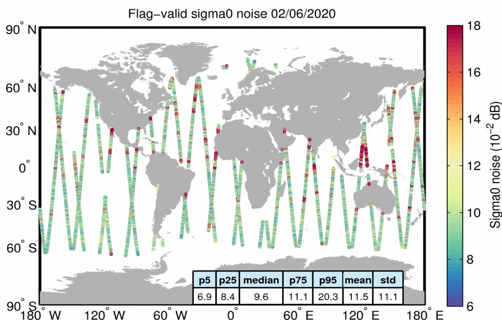
Figure 26. Geographical distribution of flag-valid 20-Hz sigma0 measurement noise over oceans and lakes for 02/06/2020. The statistical values shown in the table refer to the sigma0 noise and are calculated over all measurements shown in the figure.
