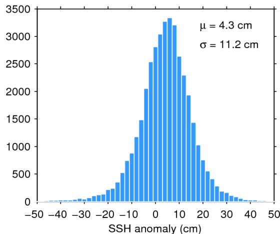
Figure 11. Histogram of science-valid SSH anomaly over oceans and lakes for 02/06/2020. The mean ( \mu ) and standard deviation ( \sigma ) are also shown. Note that values outside [-50 50] cm are excluded from the histogram for the sake of readability but not from the computation of \mu and \sigma .
