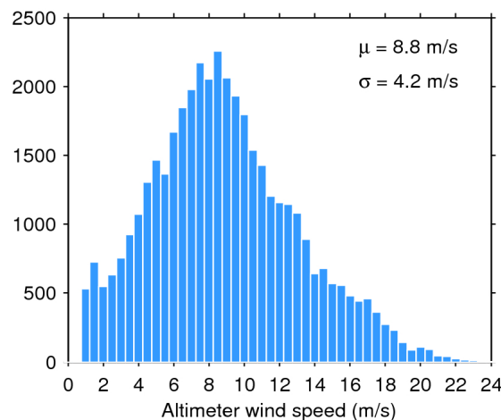
Figure 35. Histogram of science-valid wind over oceans and lakes for 02/06/2020. The mean ( \mu ) and standard deviation ( \sigma ) are also shown. Note that values larger than 24 m/s are excluded from the histogram for the sake of readability but not from the computation of \mu and \sigma .
