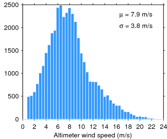
Figure 33. Histogram of flag-valid wind over oceans and lakes for 01/06/2020. The mean ( \mu ) and standard deviation ( \sigma ) are also shown. Note that values larger than 24 m/s are excluded from the histogram for the sake of readability but not from the computation of \mu and \sigma .
