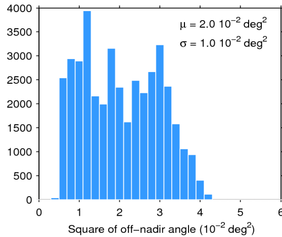
Figure 39. Histogram of flag-valid mispointing over oceans and lakes for 01/06/2020. The mean ( \mu ) and standard deviation ( \sigma ) are also shown. Note that values larger than 6 \cdot 10^{-2} \text{ deg}^2 are excluded from the histogram for the sake of readability but not from the computation of \mu and \sigma .
