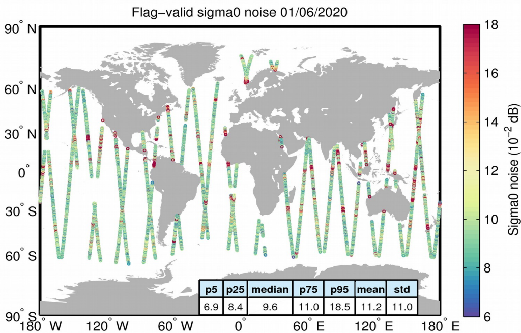
Figure 26. Geographical distribution of flag-valid 20-Hz sigma0 measurement noise over oceans and lakes for 01/06/2020. The statistical values shown in the table refer to the sigma0 noise and are calculated over all measurements shown in the figure.
