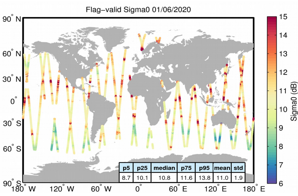
Figure 23. Geographical distribution of flag-valid sigma0 data over oceans and lakes for 01/06/2020. The statistical values shown in the table refer to the sigma0 in dB and are calculated over all measurements shown in the figure.
