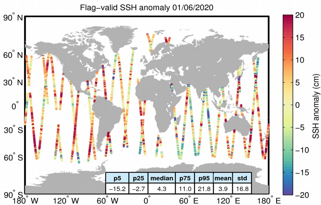
Figure 5. Geographical distribution of flag-valid 1-Hz SSH anomaly data over oceans and lakes for 01/06/2020. The statistical values shown in the table refer to the SSH anomaly in cm and are calculated over all measurements shown in the figure.
