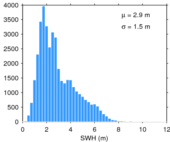
Figure 20. Histogram of science-valid SWH over oceans and lakes for 01/06/2020. The mean ( \mu ) and standard deviation ( \sigma ) are also shown. Note that values larger than 12 m are excluded from the histogram for the sake of readability but not from the computation of \mu and \sigma .
