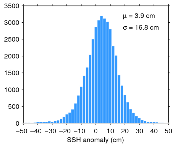
Figure 7. Histogram of flag-valid SSH anomaly over oceans and lakes for 01/06/2020. The mean ( \mu ) and standard deviation ( \sigma ) are also shown. Note that values outside [-50\ 50] cm are excluded from the histogram for the sake of readability but not from the computation of \mu and \sigma .
