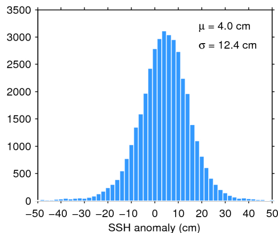
Figure 11. Histogram of science-valid SSH anomaly over oceans and lakes for 01/06/2020. The mean ( \mu ) and standard deviation ( \sigma ) are also shown. Note that values outside [-50 50] cm are excluded from the histogram for the sake of readability but not from the computation of \mu and \sigma .
