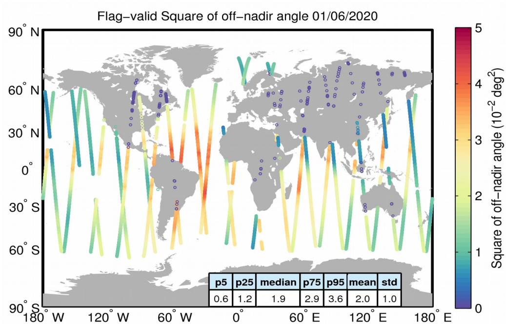
Figure 37. Geographical distribution of flag-valid mispointing data over oceans and lakes for 01/06/2020. The statistical values shown in the table refer to the mispointing in 10^{-2} \text{ deg}^2 and are calculated over all measurements shown in the figure.
