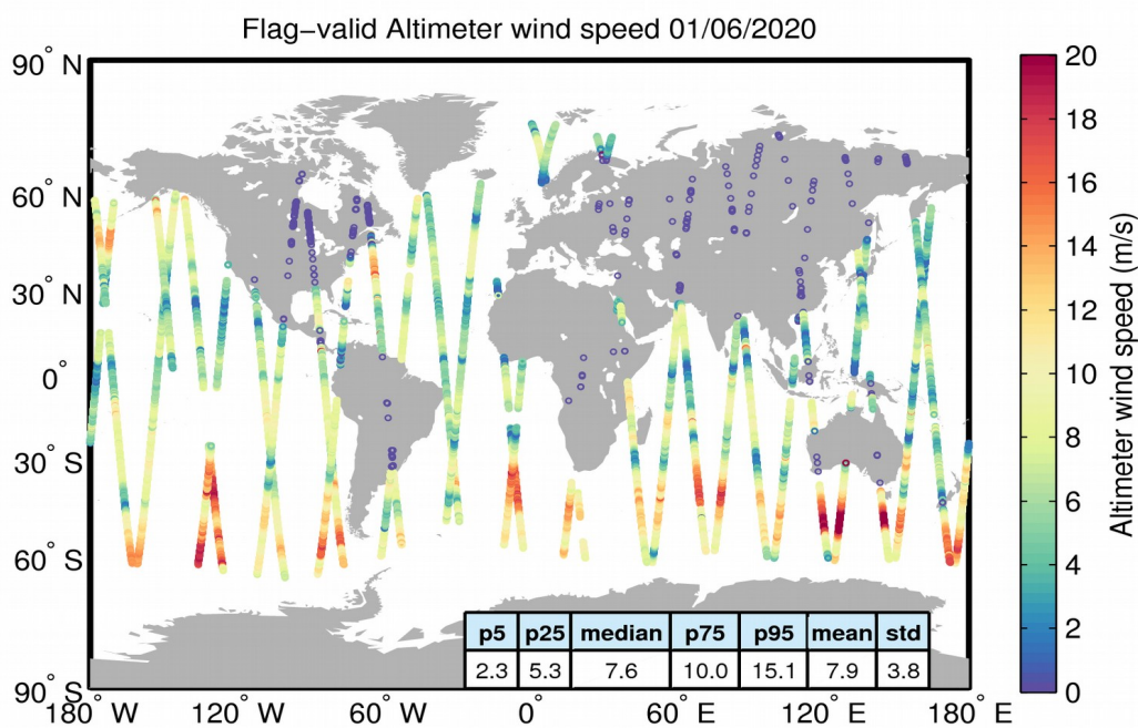
Figure 31. Geographical distribution of flag-valid wind data over oceans and lakes for 01/06/2020. The statistical values shown in the table refer to the wind in m/s and are calculated over all measurements shown in the figure.
