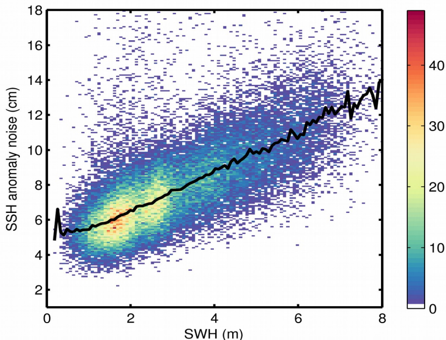
Figure 9. 2D histogram showing flag-valid SSH anomaly noise as a function of SWH for 01/06/2020. The black line denotes the median SSH anomaly noise as a function of SWH.
