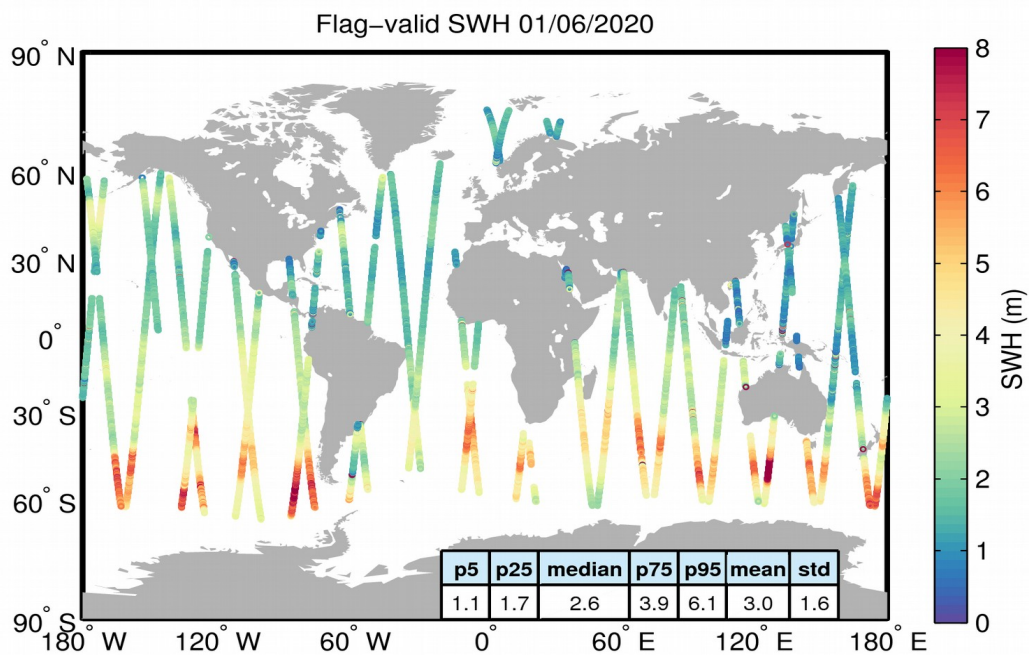
Figure 15. Geographical distribution of flag-valid SWH data over oceans and lakes for 01/06/2020. The statistical values shown in the table refer to the SWH in m and are calculated over all measurements shown in the figure.
