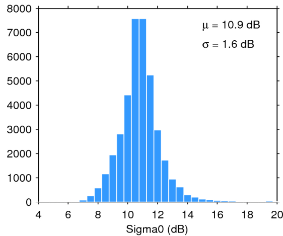
Figure 28. Histogram of science-valid sigma0 over oceans and lakes for 01/06/2020. The mean ( \mu ) and standard deviation ( \sigma ) are also shown. Note that values outside [4 20] dB are excluded from the histogram for the sake of readability but not from the computation of \mu and \sigma .
