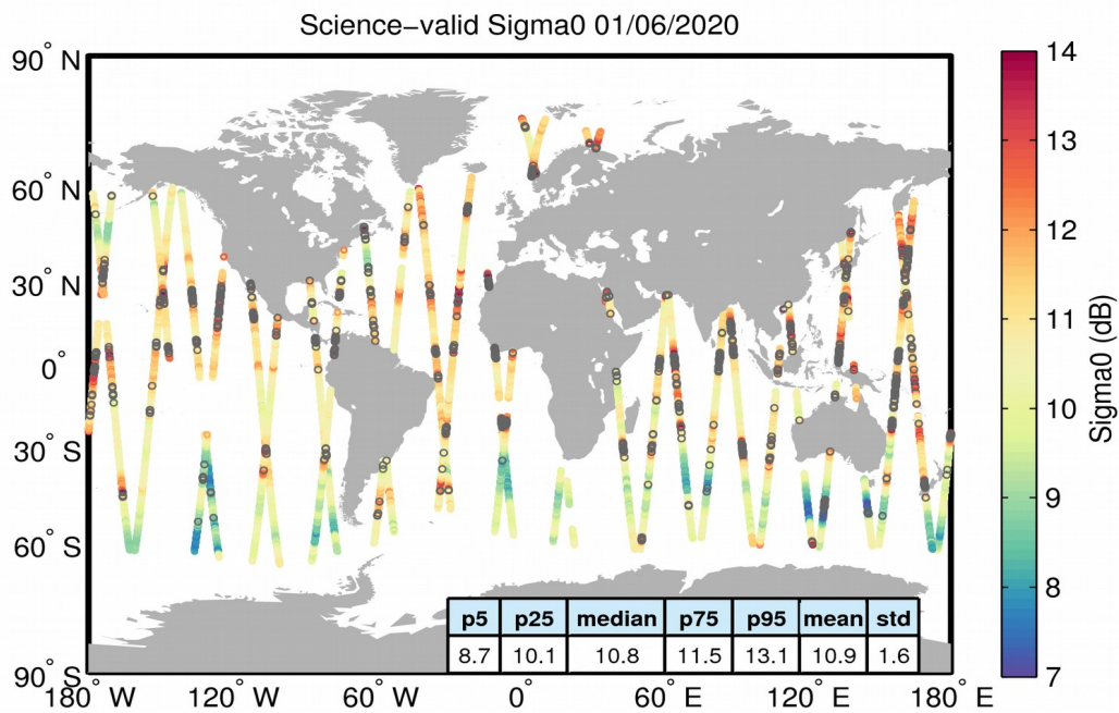
Figure 27. Geographical distribution of science-valid sigma0 data over oceans and lakes for 01/06/2020. The statistical values shown in the table refer to the sigma0 in dB and are calculated over all measurements shown in the figure. Gray circles denote records that have been rejected based on the editing criteria described in Table 4.
