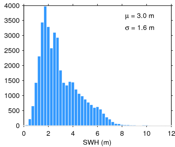
Figure 17. Histogram of flag-valid SWH over oceans and lakes for 01/06/2020. The mean ( \mu ) and standard deviation ( \sigma ) are also shown. Note that values larger than 12 m are excluded from the histogram for the sake of readability but not from the computation of \mu and \sigma .
