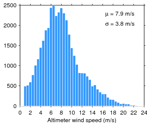
Figure 35. Histogram of science-valid wind over oceans and lakes for 01/06/2020. The mean ( \mu ) and standard deviation ( \sigma ) are also shown. Note that values larger than 24 m/s are excluded from the histogram for the sake of readability but not from the computation of \mu and \sigma .
