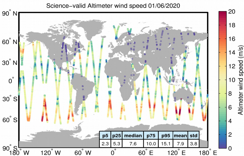
Figure 34. Geographical distribution of science-valid wind data over oceans and lakes for 01/06/2020. The statistical values shown in the table refer to the wind in m/s and are calculated over all measurements shown in the figure. Gray circles denote records that have been rejected based on the editing criteria described in Table 5.
