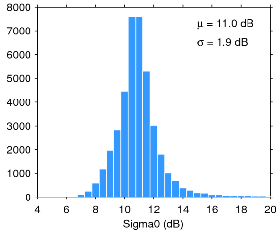
Figure 25. Histogram of flag-valid sigma0 over oceans and lakes for 01/06/2020. The mean ( \mu ) and standard deviation ( \sigma ) are also shown. Note that values outside [4 20] dB are excluded from the histogram for the sake of readability but not from the computation of \mu and \sigma .
