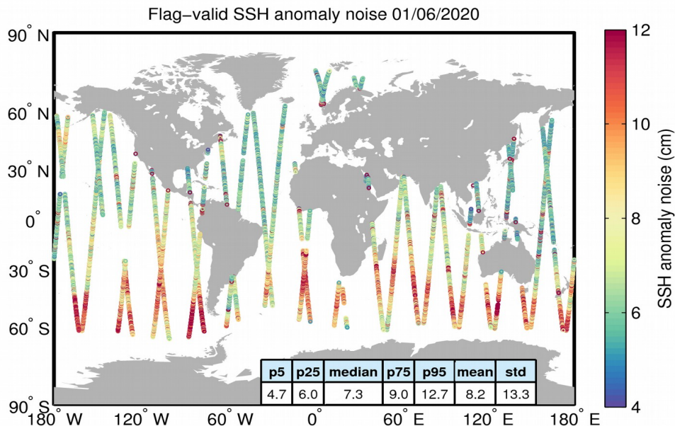
Figure 8. Geographical distribution of flag-valid 20-Hz SSH anomaly measurement noise over oceans and lakes for 01/06/2020. The statistical values shown in the table refer to the SSH anomaly noise and are calculated over all measurements shown in the figure.
