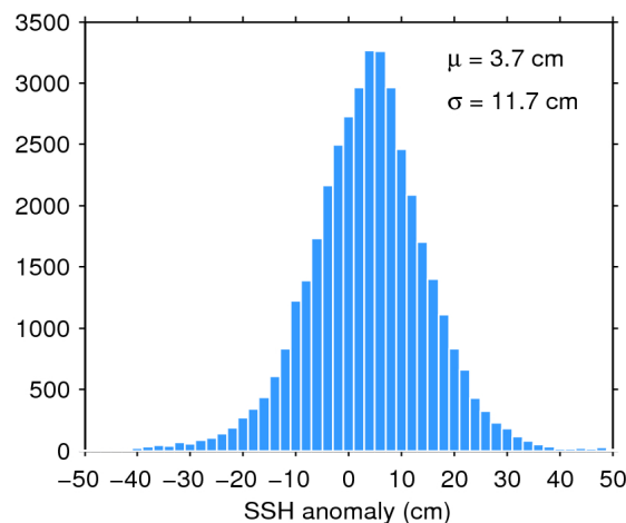
Figure 11. Histogram of science-valid SSH anomaly over oceans and lakes for 31/05/2020. The mean ( \mu ) and standard deviation ( \sigma ) are also shown. Note that values outside [-50 50] cm are excluded from the histogram for the sake of readability but not from the computation of \mu and \sigma .
