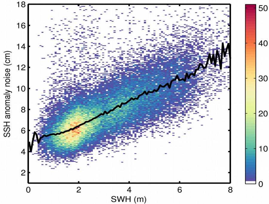
Figure 9. 2D histogram showing flag-valid SSH anomaly noise as a function of SWH for 31/05/2020. The black line denotes the median SSH anomaly noise as a function of SWH.
