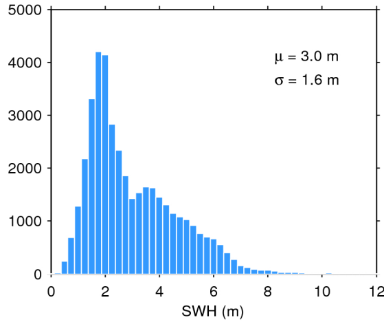
Figure 20. Histogram of science-valid SWH over oceans and lakes for 31/05/2020. The mean ( \mu ) and standard deviation ( \sigma ) are also shown. Note that values larger than 12 m are excluded from the histogram for the sake of readability but not from the computation of \mu and \sigma .
