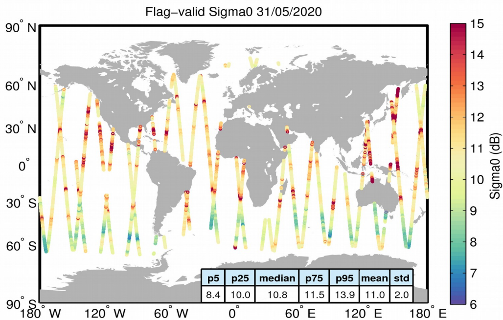
Figure 23. Geographical distribution of flag-valid sigma0 data over oceans and lakes for 31/05/2020. The statistical values shown in the table refer to the sigma0 in dB and are calculated over all measurements shown in the figure.
