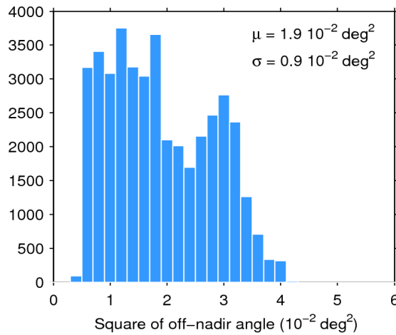
Figure 39. Histogram of flag-valid mispointing over oceans and lakes for 31/05/2020. The mean ( \mu ) and standard deviation ( \sigma ) are also shown. Note that values larger than 6 \cdot 10^{-2} \text{ deg}^2 are excluded from the histogram for the sake of readability but not from the computation of \mu and \sigma .
