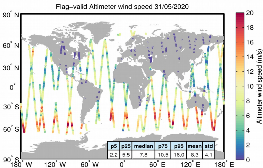
Figure 31. Geographical distribution of flag-valid wind data over oceans and lakes for 31/05/2020. The statistical values shown in the table refer to the wind in m/s and are calculated over all measurements shown in the figure.
