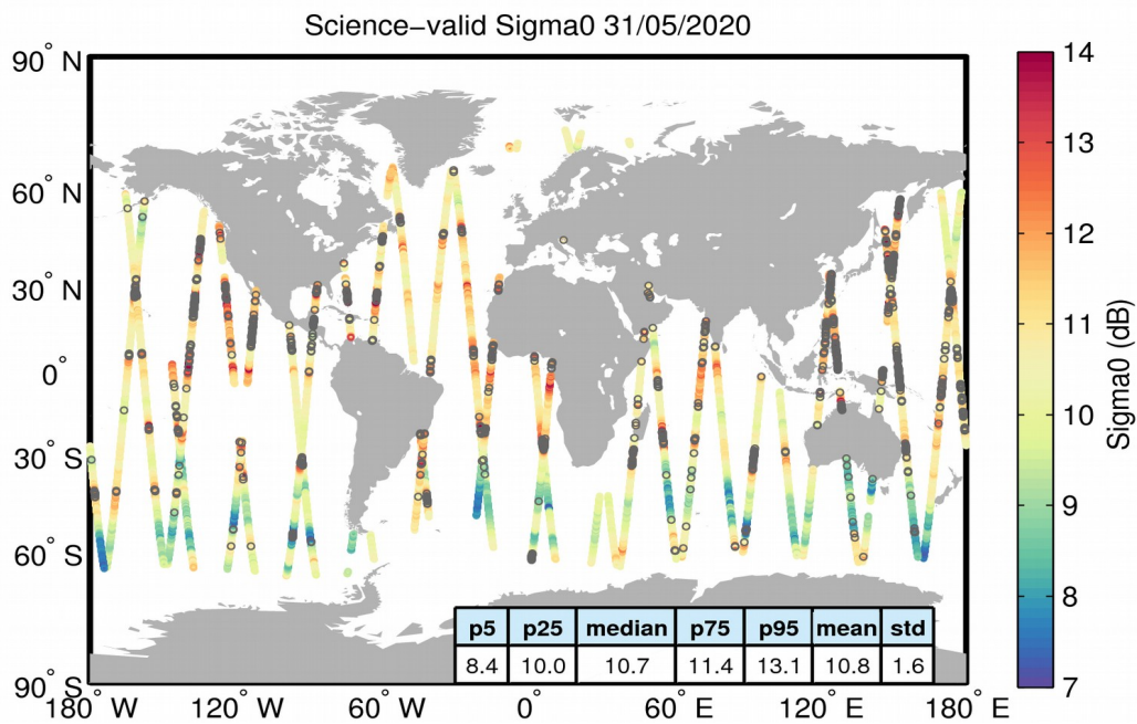
Figure 27. Geographical distribution of science-valid sigma0 data over oceans and lakes for 31/05/2020. The statistical values shown in the table refer to the sigma0 in dB and are calculated over all measurements shown in the figure. Gray circles denote records that have been rejected based on the editing criteria described in Table 4.
