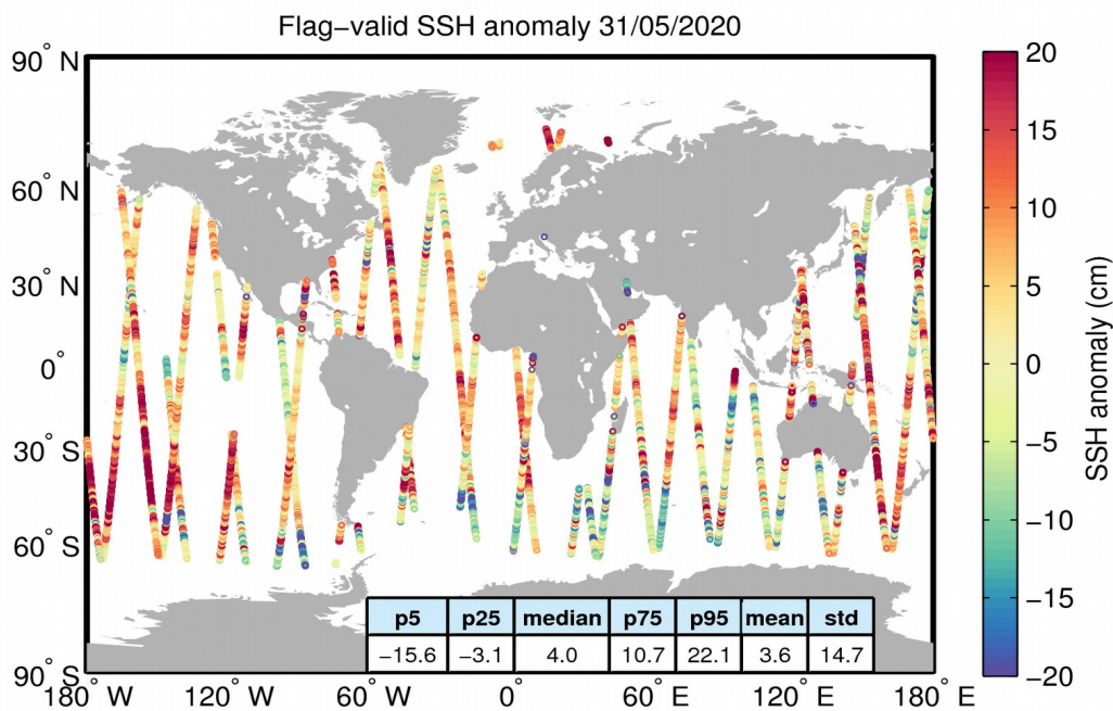
Figure 5. Geographical distribution of flag-valid 1-Hz SSH anomaly data over oceans and lakes for 31/05/2020. The statistical values shown in the table refer to the SSH anomaly in cm and are calculated over all measurements shown in the figure.
