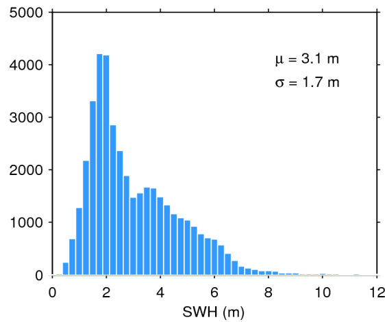
Figure 17. Histogram of flag-valid SWH over oceans and lakes for 31/05/2020. The mean ( \mu ) and standard deviation ( \sigma ) are also shown. Note that values larger than 12 m are excluded from the histogram for the sake of readability but not from the computation of \mu and \sigma .
