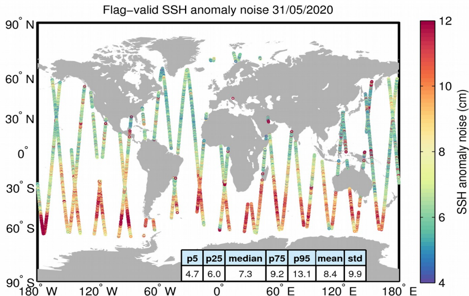
Figure 8. Geographical distribution of flag-valid 20-Hz SSH anomaly measurement noise over oceans and lakes for 31/05/2020. The statistical values shown in the table refer to the SSH anomaly noise and are calculated over all measurements shown in the figure.
