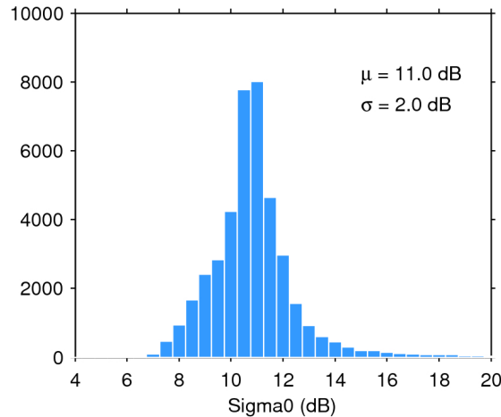
Figure 25. Histogram of flag-valid sigma0 over oceans and lakes for 31/05/2020. The mean ( \mu ) and standard deviation ( \sigma ) are also shown. Note that values outside [4 20] dB are excluded from the histogram for the sake of readability but not from the computation of \mu and \sigma .
