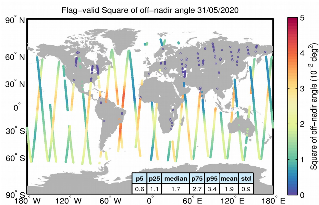
Figure 37. Geographical distribution of flag-valid mispointing data over oceans and lakes for 31/05/2020. The statistical values shown in the table refer to the mispointing in 10^{-2} deg 2 and are calculated over all measurements shown in the figure.
