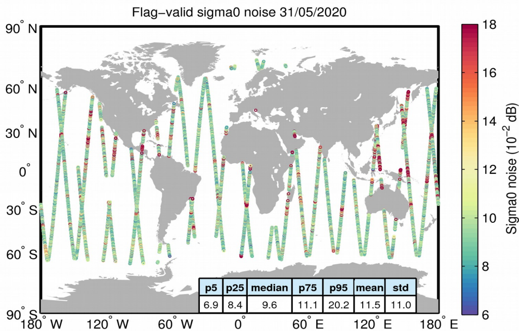
Figure 26. Geographical distribution of flag-valid 20-Hz sigma0 measurement noise over oceans and lakes for 31/05/2020. The statistical values shown in the table refer to the sigma0 noise and are calculated over all measurements shown in the figure.
