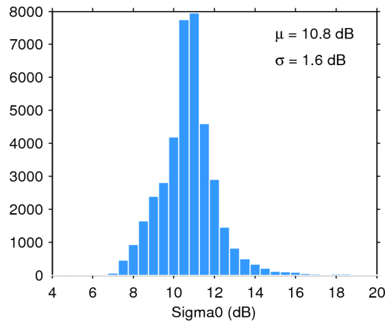
Figure 28. Histogram of science-valid sigma0 over oceans and lakes for 31/05/2020. The mean ( \mu ) and standard deviation ( \sigma ) are also shown. Note that values outside [4 20] dB are excluded from the histogram for the sake of readability but not from the computation of \mu and \sigma .
