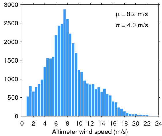
Figure 33. Histogram of flag-valid wind over oceans and lakes for 30/05/2020. The mean ( \mu ) and standard deviation ( \sigma ) are also shown. Note that values larger than 24 m/s are excluded from the histogram for the sake of readability but not from the computation of \mu and \sigma .
