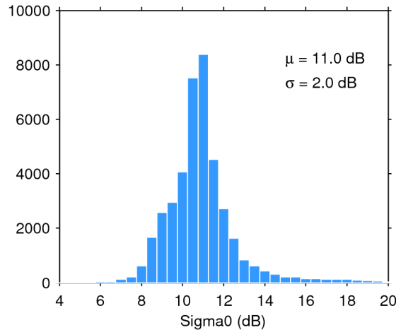
Figure 25. Histogram of flag-valid sigma0 over oceans and lakes for 30/05/2020. The mean ( \mu ) and standard deviation ( \sigma ) are also shown. Note that values outside [4 20] dB are excluded from the histogram for the sake of readability but not from the computation of \mu and \sigma .
