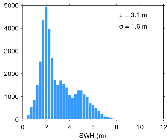
Figure 17. Histogram of flag-valid SWH over oceans and lakes for 30/05/2020. The mean ( \mu ) and standard deviation ( \sigma ) are also shown. Note that values larger than 12 m are excluded from the histogram for the sake of readability but not from the computation of \mu and \sigma .
