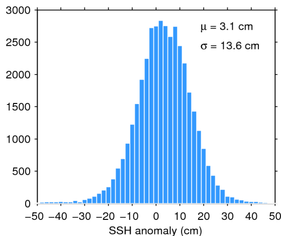
Figure 11. Histogram of science-valid SSH anomaly over oceans and lakes for 30/05/2020. The mean ( \mu ) and standard deviation ( \sigma ) are also shown. Note that values outside [-50 50] cm are excluded from the histogram for the sake of readability but not from the computation of \mu and \sigma .
