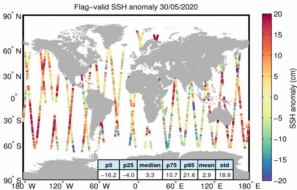
Figure 5. Geographical distribution of flag-valid 1-Hz SSH anomaly data over oceans and lakes for 30/05/2020. The statistical values shown in the table refer to the SSH anomaly in cm and are calculated over all measurements shown in the figure.
