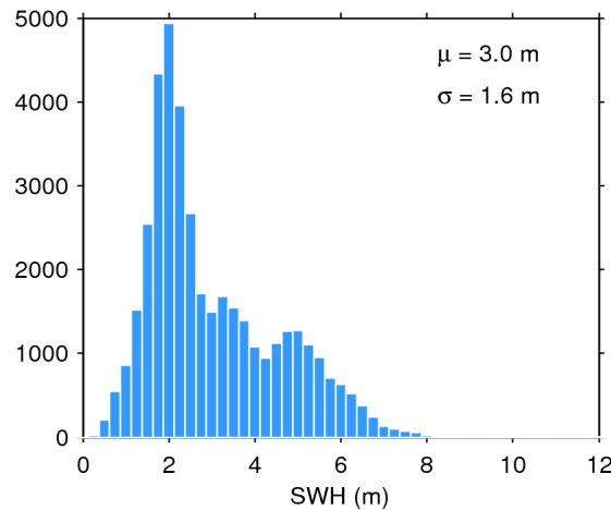
Figure 20. Histogram of science-valid SWH over oceans and lakes for 30/05/2020. The mean ( \mu ) and standard deviation ( \sigma ) are also shown. Note that values larger than 12 m are excluded from the histogram for the sake of readability but not from the computation of \mu and \sigma .
