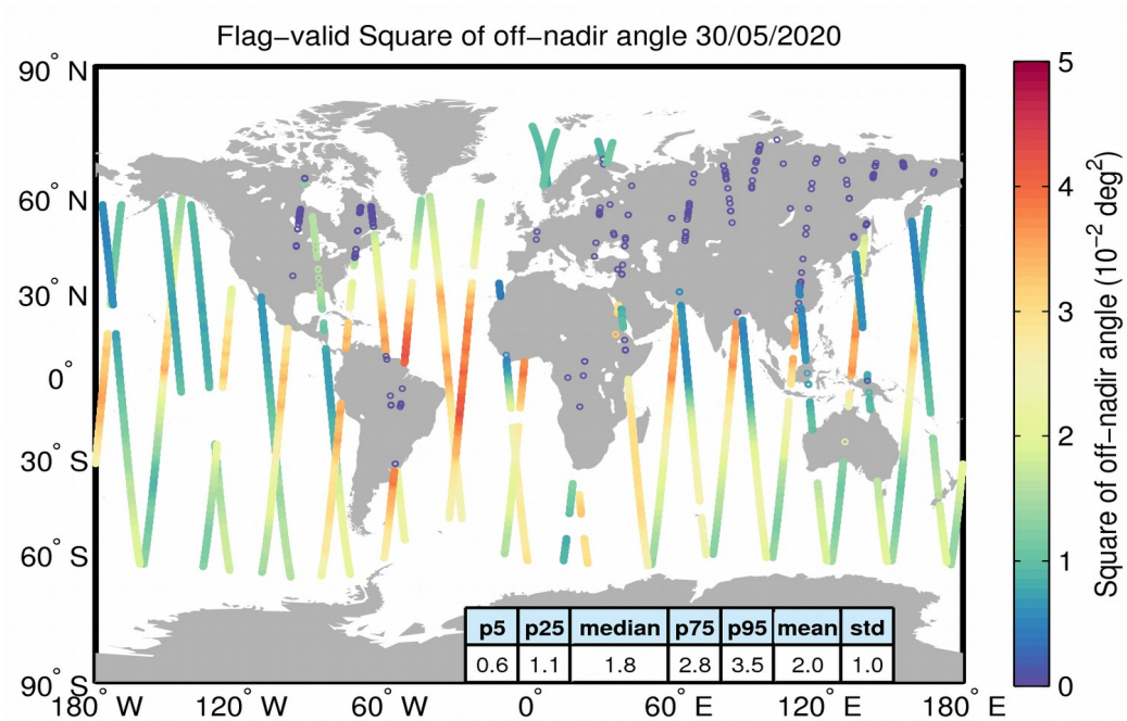
Figure 37. Geographical distribution of flag-valid mispointing data over oceans and lakes for 30/05/2020. The statistical values shown in the table refer to the mispointing in 10^{-2} deg 2 and are calculated over all measurements shown in the figure.
