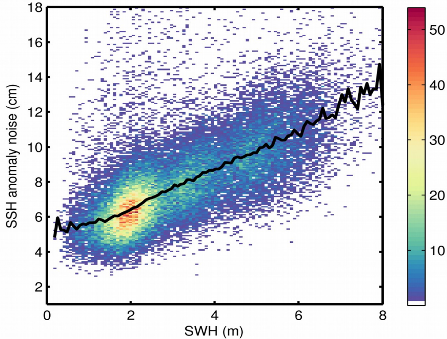
Figure 9. 2D histogram showing flag-valid SSH anomaly noise as a function of SWH for 30/05/2020. The black line denotes the median SSH anomaly noise as a function of SWH.
