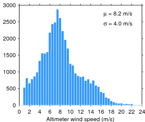
Figure 35. Histogram of science-valid wind over oceans and lakes for 30/05/2020. The mean ( \mu ) and standard deviation ( \sigma ) are also shown. Note that values larger than 24 m/s are excluded from the histogram for the sake of readability but not from the computation of \mu and \sigma .
