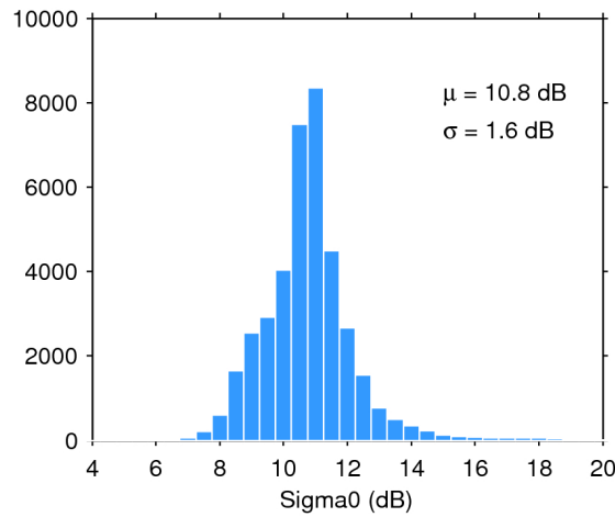
Figure 28. Histogram of science-valid sigma0 over oceans and lakes for 30/05/2020. The mean ( \mu ) and standard deviation ( \sigma ) are also shown. Note that values outside [4 20] dB are excluded from the histogram for the sake of readability but not from the computation of \mu and \sigma .
