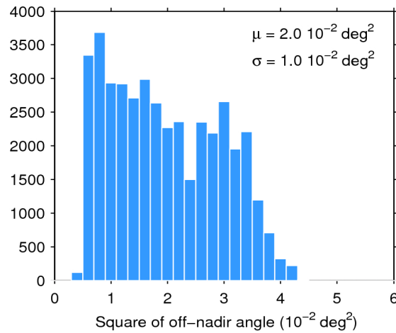
Figure 39. Histogram of flag-valid mispointing over oceans and lakes for 30/05/2020. The mean ( \mu ) and standard deviation ( \sigma ) are also shown. Note that values larger than 6 \cdot 10^{-2} \text{ deg}^2 are excluded from the histogram for the sake of readability but not from the computation of \mu and \sigma .
