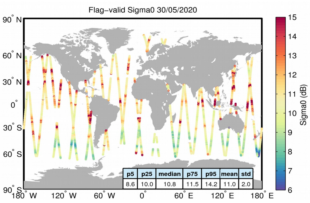
Figure 23. Geographical distribution of flag-valid sigma0 data over oceans and lakes for 30/05/2020. The statistical values shown in the table refer to the sigma0 in dB and are calculated over all measurements shown in the figure.
