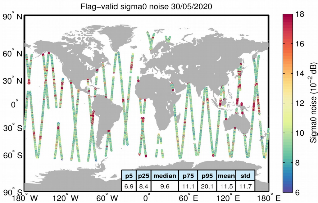
Figure 26. Geographical distribution of flag-valid 20-Hz sigma0 measurement noise over oceans and lakes for 30/05/2020. The statistical values shown in the table refer to the sigma0 noise and are calculated over all measurements shown in the figure.
