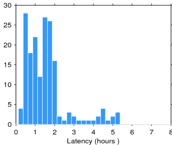
Figure 2. Histogram of the data latency for 30/05/2020. The y-axis denotes the number of files that are made available with a delay of x-hours with respect to the mean time of the records stored in the file.
