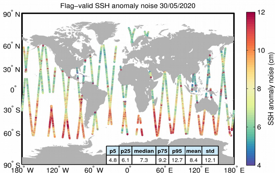
Figure 8. Geographical distribution of flag-valid 20-Hz SSH anomaly measurement noise over oceans and lakes for 30/05/2020. The statistical values shown in the table refer to the SSH anomaly noise and are calculated over all measurements shown in the figure.
