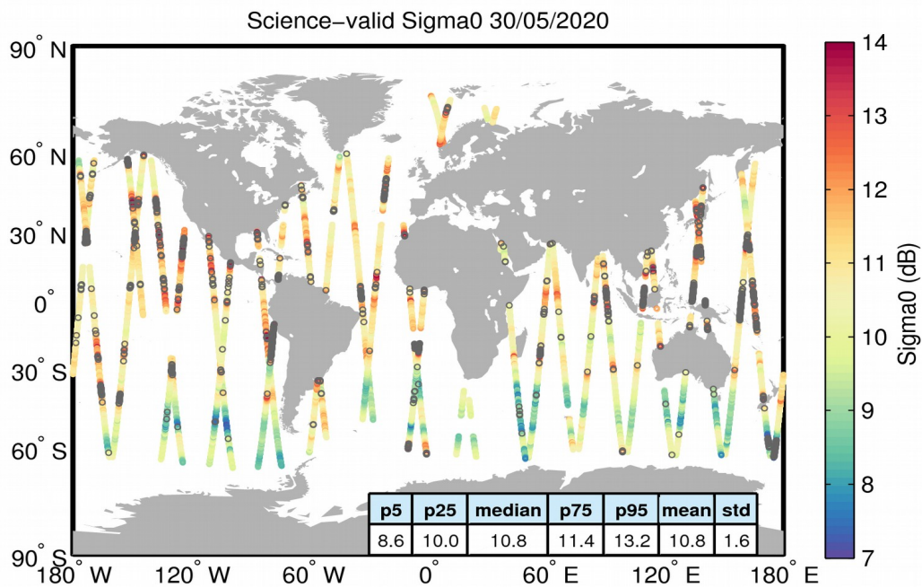
Figure 27. Geographical distribution of science-valid sigma0 data over oceans and lakes for 30/05/2020. The statistical values shown in the table refer to the sigma0 in dB and are calculated over all measurements shown in the figure. Gray circles denote records that have been rejected based on the editing criteria described in Table 4.
