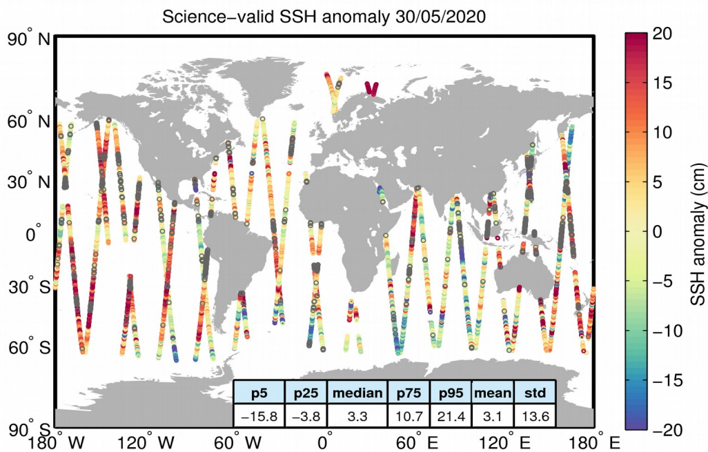
Figure 10. Geographical distribution of science-valid SSH anomaly data over oceans and lakes for 30/05/2020. The statistical values shown in the table refer to the SSH anomaly in cm and are calculated over all measurements shown in the figure. Gray circles denote records that have been rejected based on the editing criteria described in Table 2.
