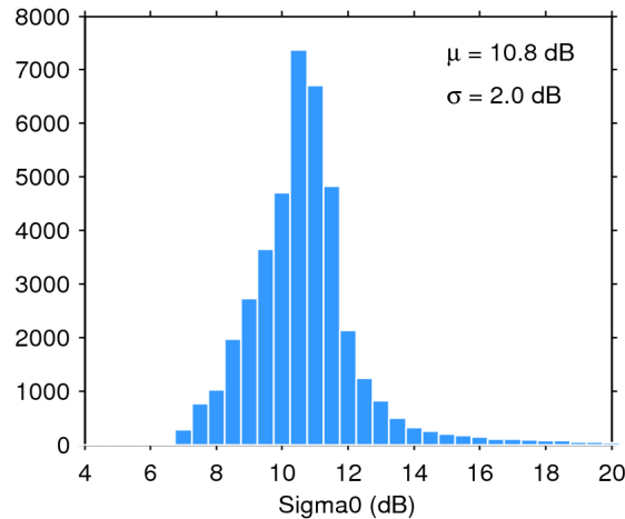
Figure 25. Histogram of flag-valid sigma0 over oceans and lakes for 27/05/2020. The mean ( \mu ) and standard deviation ( \sigma ) are also shown. Note that values outside [4 20] dB are excluded from the histogram for the sake of readability but not from the computation of \mu and \sigma .
