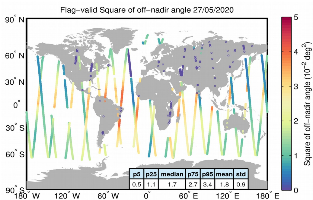
Figure 37. Geographical distribution of flag-valid mispointing data over oceans and lakes for 27/05/2020. The statistical values shown in the table refer to the mispointing in 10^{-2} \text{ deg}^2 and are calculated over all measurements shown in the figure.
