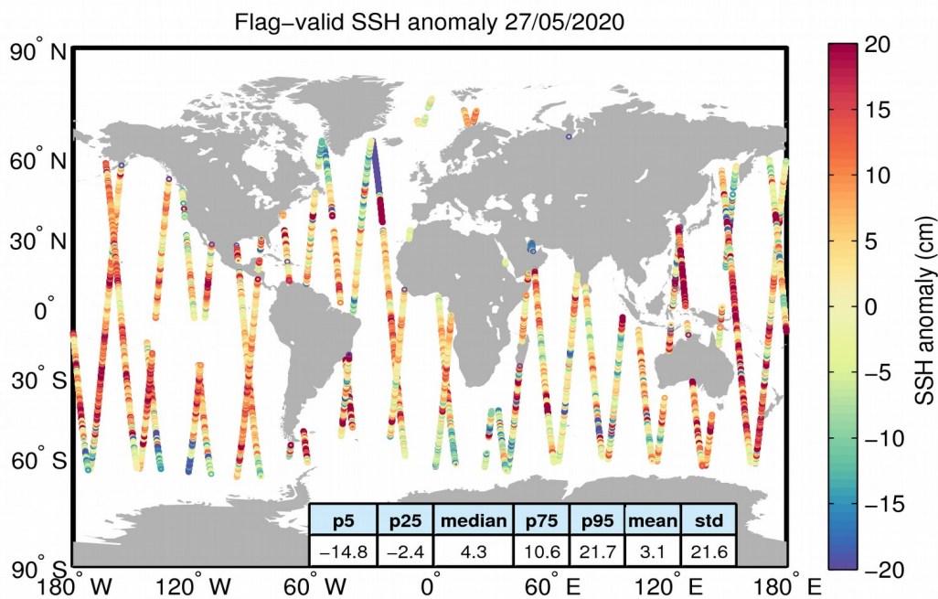
Figure 5. Geographical distribution of flag-valid 1-Hz SSH anomaly data over oceans and lakes for 27/05/2020. The statistical values shown in the table refer to the SSH anomaly in cm and are calculated over all measurements shown in the figure.
