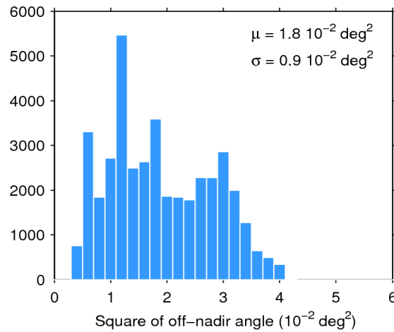
Figure 39. Histogram of flag-valid mispointing over oceans and lakes for 27/05/2020. The mean ( \mu ) and standard deviation ( \sigma ) are also shown. Note that values larger than 6 \cdot 10^{-2} \text{ deg}^2 are excluded from the histogram for the sake of readability but not from the computation of \mu and \sigma .
