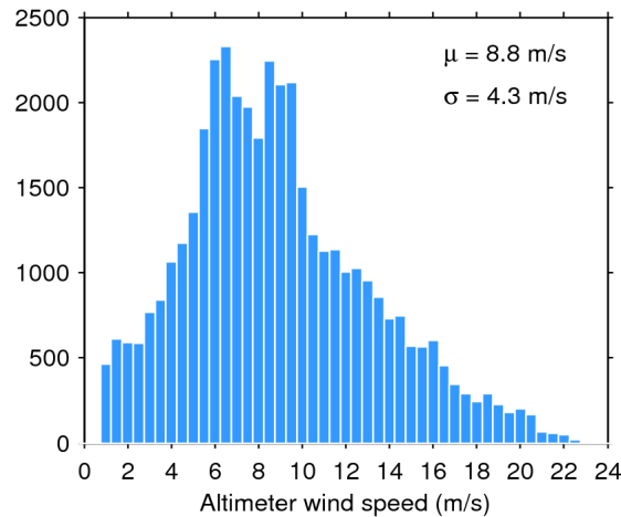
Figure 33. Histogram of flag-valid wind over oceans and lakes for 27/05/2020. The mean ( \mu ) and standard deviation ( \sigma ) are also shown. Note that values larger than 24 m/s are excluded from the histogram for the sake of readability but not from the computation of \mu and \sigma .
