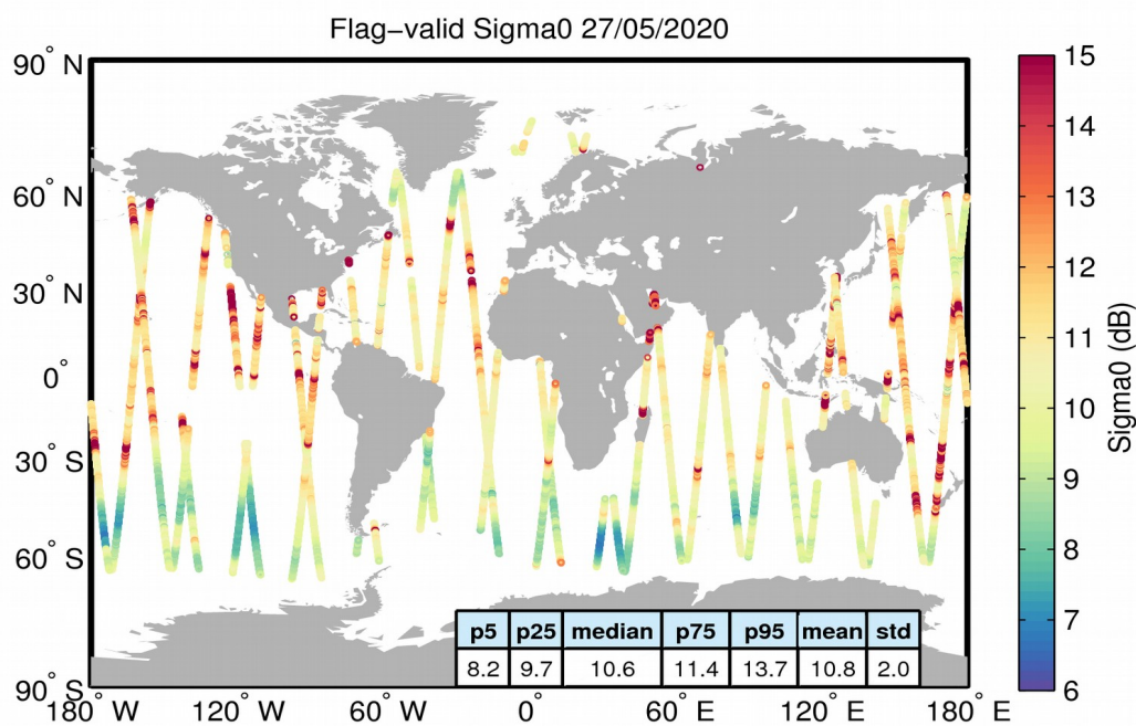
Figure 23. Geographical distribution of flag-valid sigma0 data over oceans and lakes for 27/05/2020. The statistical values shown in the table refer to the sigma0 in dB and are calculated over all measurements shown in the figure.
