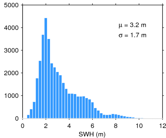
Figure 20. Histogram of science-valid SWH over oceans and lakes for 27/05/2020. The mean ( \mu ) and standard deviation ( \sigma ) are also shown. Note that values larger than 12 m are excluded from the histogram for the sake of readability but not from the computation of \mu and \sigma .
