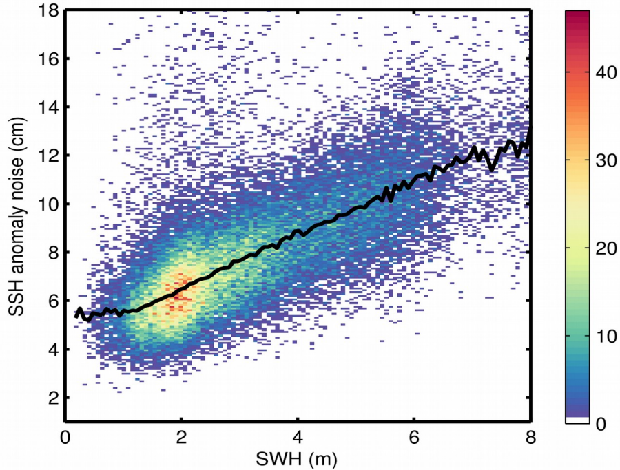
Figure 9. 2D histogram showing flag-valid SSH anomaly noise as a function of SWH for 27/05/2020. The black line denotes the median SSH anomaly noise as a function of SWH.
