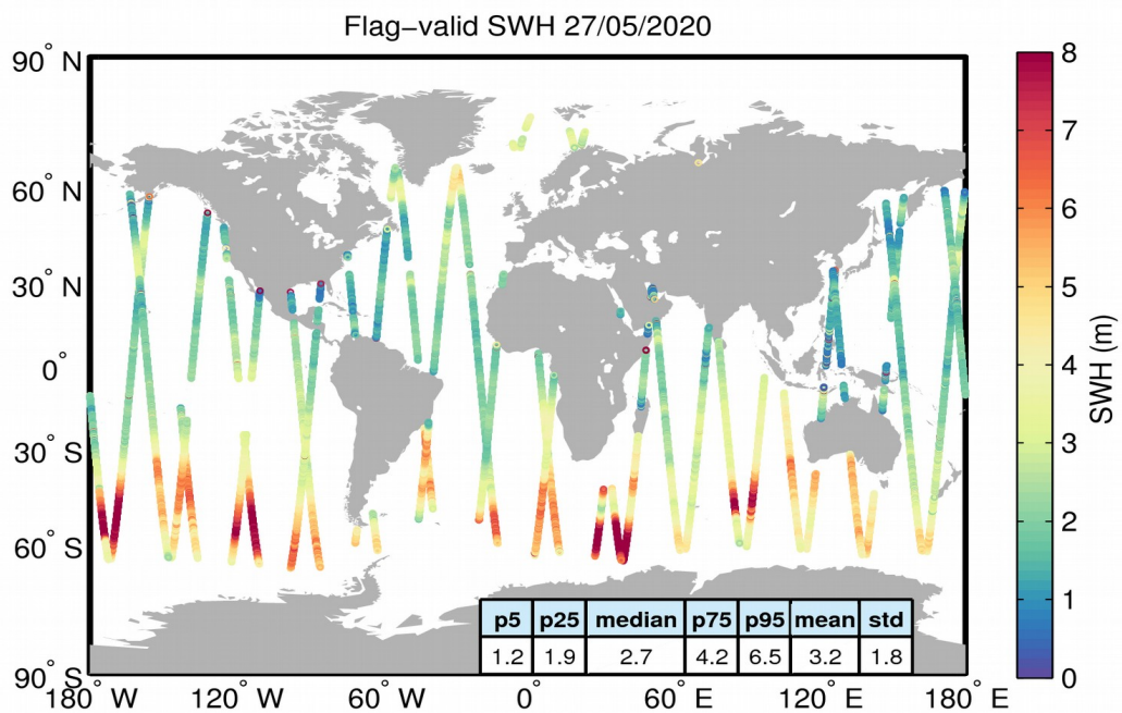
Figure 15. Geographical distribution of flag-valid SWH data over oceans and lakes for 27/05/2020. The statistical values shown in the table refer to the SWH in m and are calculated over all measurements shown in the figure.
