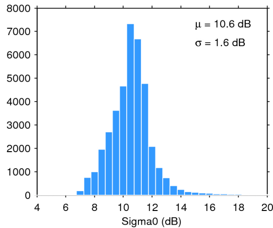
Figure 28. Histogram of science-valid sigma0 over oceans and lakes for 27/05/2020. The mean ( \mu ) and standard deviation ( \sigma ) are also shown. Note that values outside [4 20] dB are excluded from the histogram for the sake of readability but not from the computation of \mu and \sigma .
