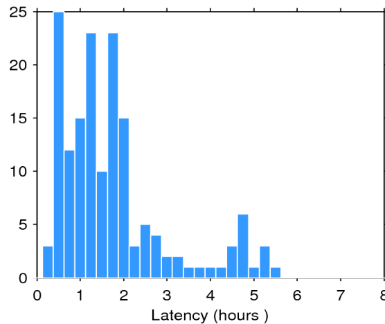
Figure 2. Histogram of the data latency for 27/05/2020. The y-axis denotes the number of files that are made available with a delay of x-hours with respect to the mean time of the records stored in the file.
