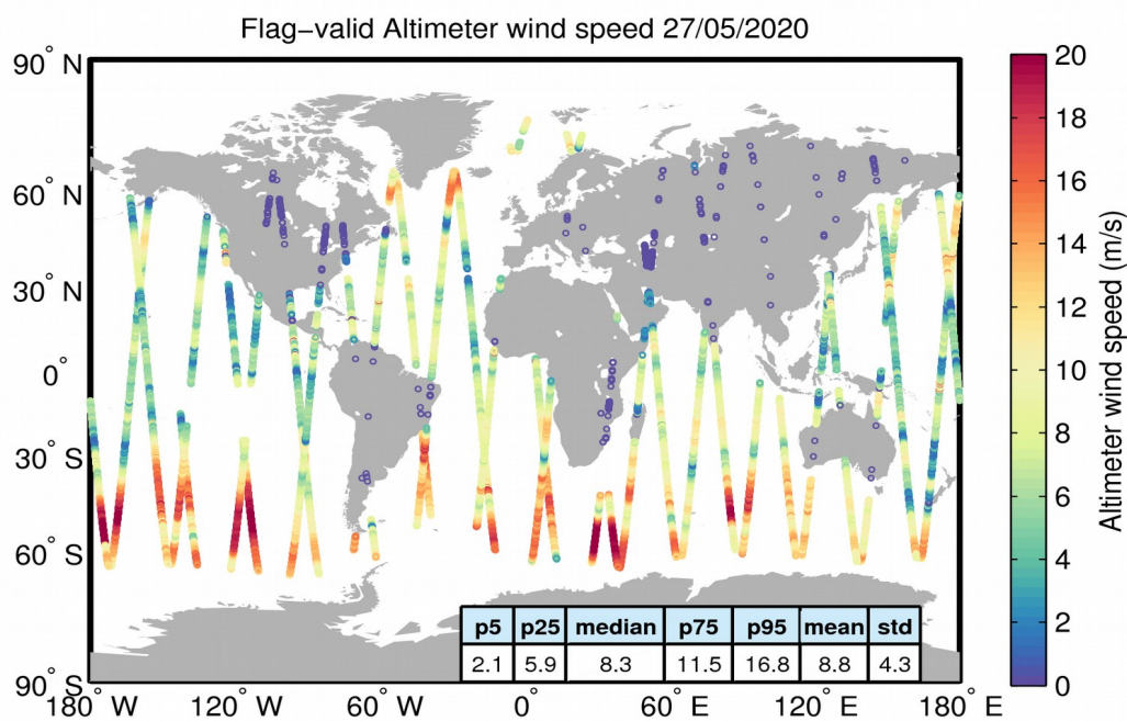
Figure 31. Geographical distribution of flag-valid wind data over oceans and lakes for 27/05/2020. The statistical values shown in the table refer to the wind in m/s and are calculated over all measurements shown in the figure.
