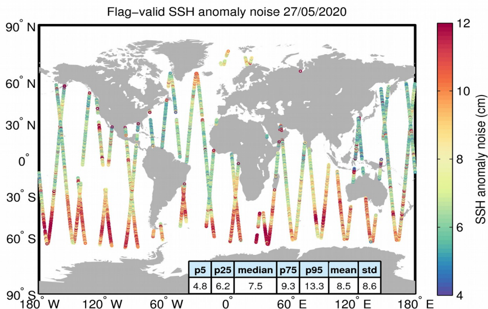
Figure 8. Geographical distribution of flag-valid 20-Hz SSH anomaly measurement noise over oceans and lakes for 27/05/2020. The statistical values shown in the table refer to the SSH anomaly noise and are calculated over all measurements shown in the figure.
