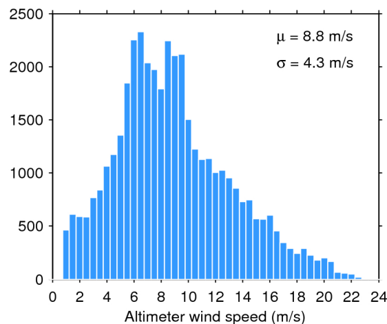
Figure 35. Histogram of science-valid wind over oceans and lakes for 27/05/2020. The mean ( \mu ) and standard deviation ( \sigma ) are also shown. Note that values larger than 24 m/s are excluded from the histogram for the sake of readability but not from the computation of \mu and \sigma .
