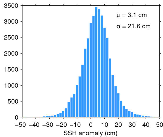
Figure 7. Histogram of flag-valid SSH anomaly over oceans and lakes for 27/05/2020. The mean ( \mu ) and standard deviation ( \sigma ) are also shown. Note that values outside [-50\ 50] cm are excluded from the histogram for the sake of readability but not from the computation of \mu and \sigma .
