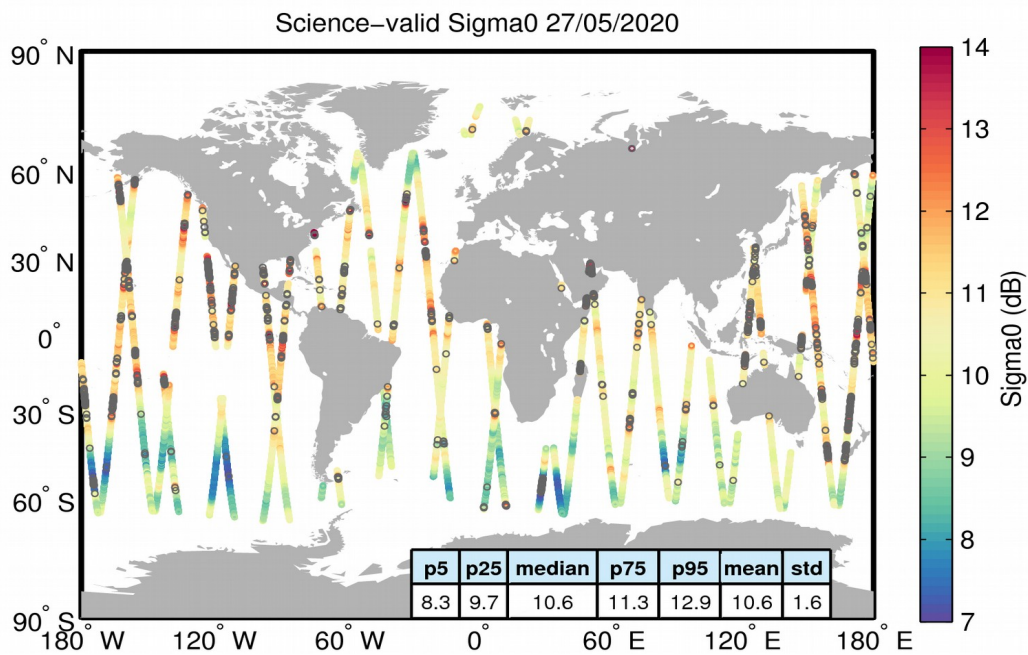
Figure 27. Geographical distribution of science-valid sigma0 data over oceans and lakes for 27/05/2020. The statistical values shown in the table refer to the sigma0 in dB and are calculated over all measurements shown in the figure. Gray circles denote records that have been rejected based on the editing criteria described in Table 4.
