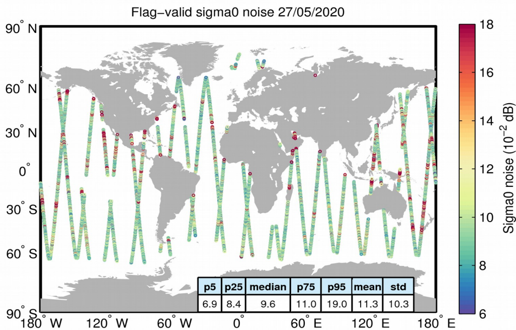
Figure 26. Geographical distribution of flag-valid 20-Hz sigma0 measurement noise over oceans and lakes for 27/05/2020. The statistical values shown in the table refer to the sigma0 noise and are calculated over all measurements shown in the figure.
