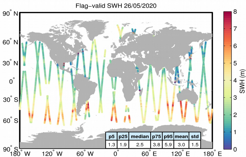
Figure 15. Geographical distribution of flag-valid SWH data over oceans and lakes for 26/05/2020. The statistical values shown in the table refer to the SWH in m and are calculated over all measurements shown in the figure.
