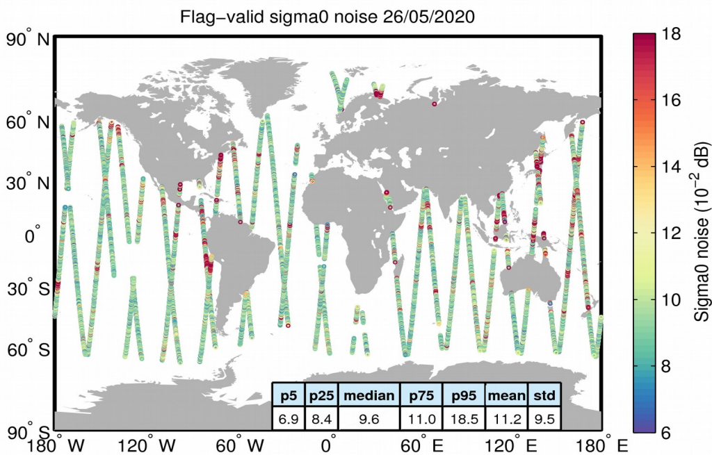
Figure 26. Geographical distribution of flag-valid 20-Hz sigma0 measurement noise over oceans and lakes for 26/05/2020. The statistical values shown in the table refer to the sigma0 noise and are calculated over all measurements shown in the figure.
