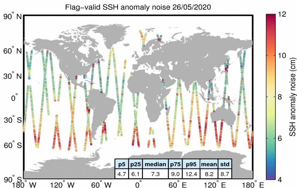
Figure 8. Geographical distribution of flag-valid 20-Hz SSH anomaly measurement noise over oceans and lakes for 26/05/2020. The statistical values shown in the table refer to the SSH anomaly noise and are calculated over all measurements shown in the figure.
