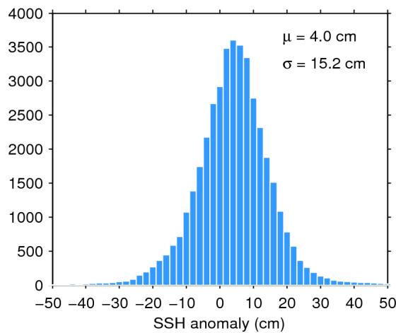
Figure 7. Histogram of flag-valid SSH anomaly over oceans and lakes for 26/05/2020. The mean ( \mu ) and standard deviation ( \sigma ) are also shown. Note that values outside [-50 50] cm are excluded from the histogram for the sake of readability but not from the computation of \mu and \sigma .
