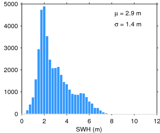
Figure 20. Histogram of science-valid SWH over oceans and lakes for 26/05/2020. The mean ( \mu ) and standard deviation ( \sigma ) are also shown. Note that values larger than 12 m are excluded from the histogram for the sake of readability but not from the computation of \mu and \sigma .
