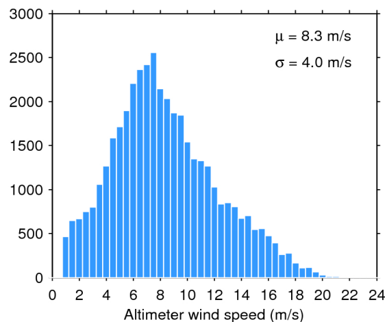
Figure 35. Histogram of science-valid wind over oceans and lakes for 26/05/2020. The mean ( \mu ) and standard deviation ( \sigma ) are also shown. Note that values larger than 24 m/s are excluded from the histogram for the sake of readability but not from the computation of \mu and \sigma .
