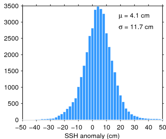
Figure 11. Histogram of science-valid SSH anomaly over oceans and lakes for 26/05/2020. The mean ( \mu ) and standard deviation ( \sigma ) are also shown. Note that values outside [-50 50] cm are excluded from the histogram for the sake of readability but not from the computation of \mu and \sigma .
