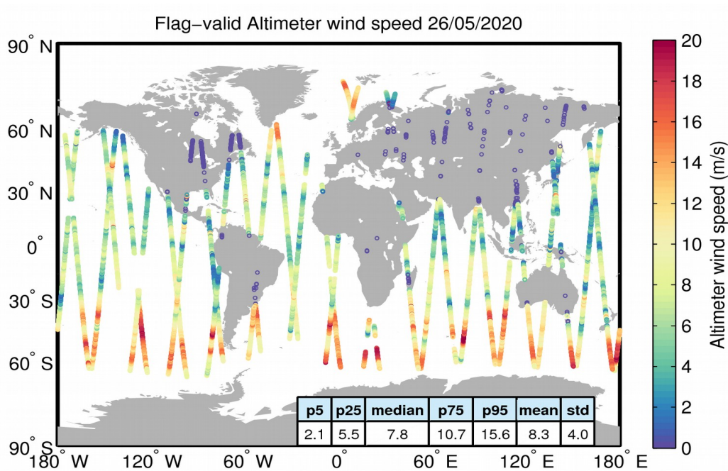
Figure 31. Geographical distribution of flag-valid wind data over oceans and lakes for 26/05/2020. The statistical values shown in the table refer to the wind in m/s and are calculated over all measurements shown in the figure.
