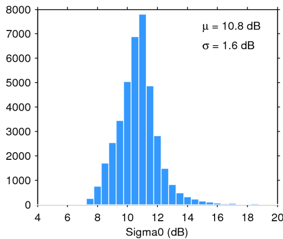
Figure 28. Histogram of science-valid sigma0 over oceans and lakes for 26/05/2020. The mean ( \mu ) and standard deviation ( \sigma ) are also shown. Note that values outside [4 20] dB are excluded from the histogram for the sake of readability but not from the computation of \mu and \sigma .
