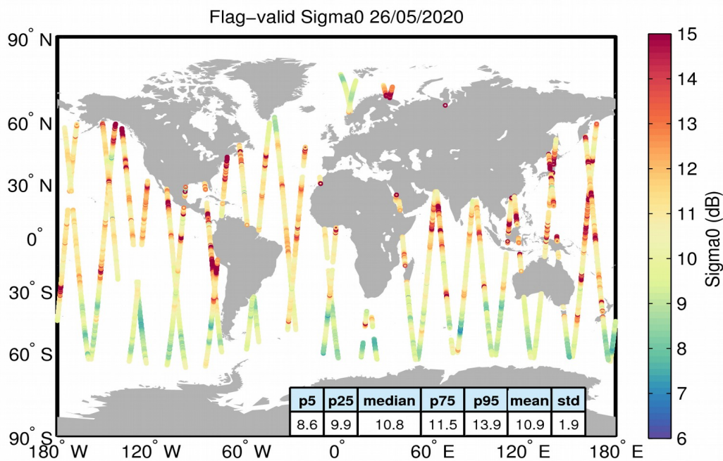
Figure 23. Geographical distribution of flag-valid sigma0 data over oceans and lakes for 26/05/2020. The statistical values shown in the table refer to the sigma0 in dB and are calculated over all measurements shown in the figure.
