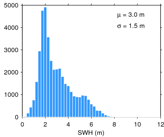
Figure 17. Histogram of flag-valid SWH over oceans and lakes for 26/05/2020. The mean ( \mu ) and standard deviation ( \sigma ) are also shown. Note that values larger than 12 m are excluded from the histogram for the sake of readability but not from the computation of \mu and \sigma .
