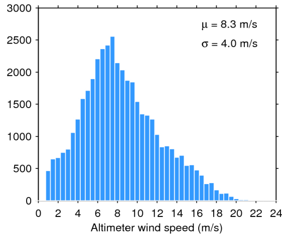
Figure 33. Histogram of flag-valid wind over oceans and lakes for 26/05/2020. The mean ( \mu ) and standard deviation ( \sigma ) are also shown. Note that values larger than 24 m/s are excluded from the histogram for the sake of readability but not from the computation of \mu and \sigma .
