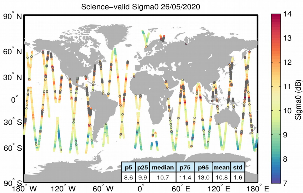
Figure 27. Geographical distribution of science-valid sigma0 data over oceans and lakes for 26/05/2020. The statistical values shown in the table refer to the sigma0 in dB and are calculated over all measurements shown in the figure. Gray circles denote records that have been rejected based on the editing criteria described in Table 4.
