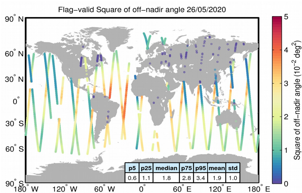
Figure 37. Geographical distribution of flag-valid mispointing data over oceans and lakes for 26/05/2020. The statistical values shown in the table refer to the mispointing in 10^{-2} \text{deg}^2 and are calculated over all measurements shown in the figure.
