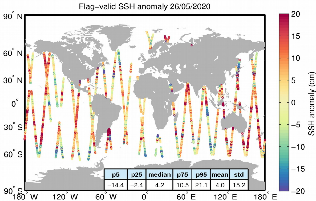
Figure 5. Geographical distribution of flag-valid 1-Hz SSH anomaly data over oceans and lakes for 26/05/2020. The statistical values shown in the table refer to the SSH anomaly in cm and are calculated over all measurements shown in the figure.
