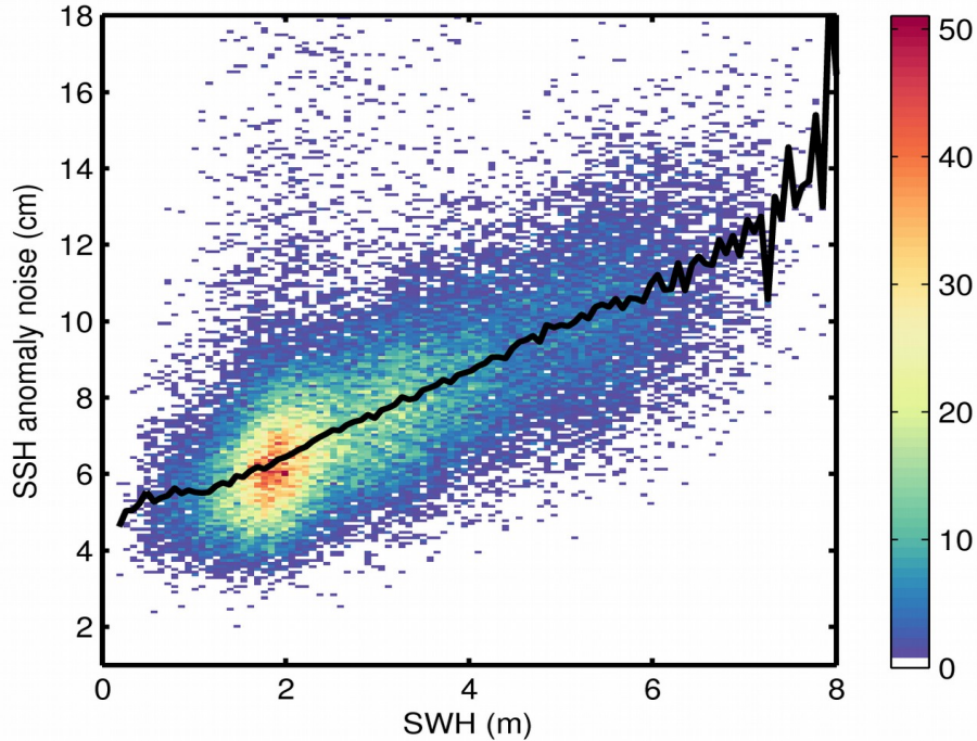
Figure 9. 2D histogram showing flag-valid SSH anomaly noise as a function of SWH for 26/05/2020. The black line denotes the median SSH anomaly noise as a function of SWH.
