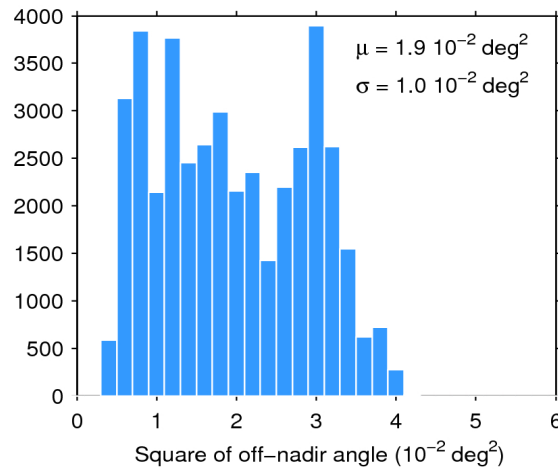
Figure 39. Histogram of flag-valid mispointing over oceans and lakes for 26/05/2020. The mean ( \mu ) and standard deviation ( \sigma ) are also shown. Note that values larger than 6 \cdot 10^{-2} \text{ deg}^2 are excluded from the histogram for the sake of readability but not from the computation of \mu and \sigma .
