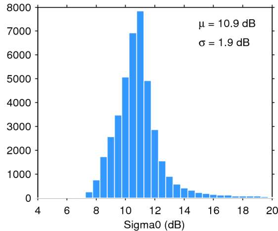
Figure 25. Histogram of flag-valid sigma0 over oceans and lakes for 26/05/2020. The mean ( \mu ) and standard deviation ( \sigma ) are also shown. Note that values outside [4 20] dB are excluded from the histogram for the sake of readability but not from the computation of \mu and \sigma .
