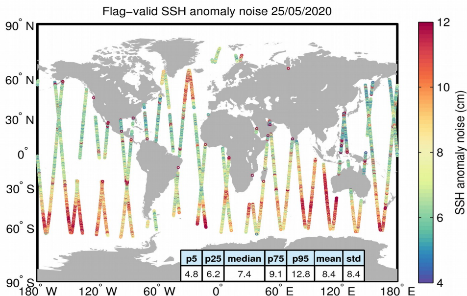
Figure 8. Geographical distribution of flag-valid 20-Hz SSH anomaly measurement noise over oceans and lakes for 25/05/2020. The statistical values shown in the table refer to the SSH anomaly noise and are calculated over all measurements shown in the figure.
