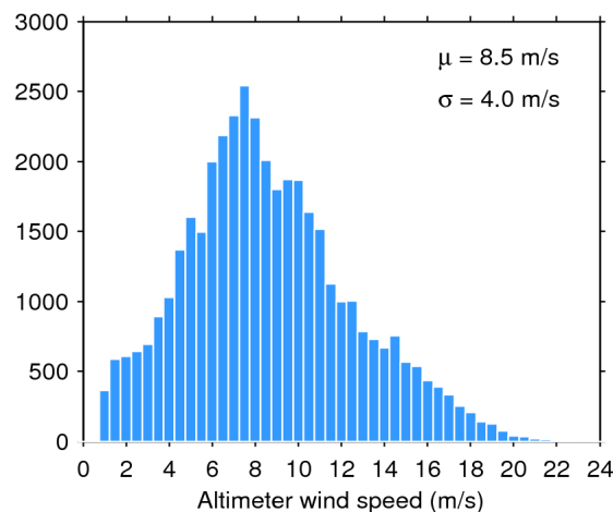
Figure 35. Histogram of science-valid wind over oceans and lakes for 25/05/2020. The mean ( \mu ) and standard deviation ( \sigma ) are also shown. Note that values larger than 24 m/s are excluded from the histogram for the sake of readability but not from the computation of \mu and \sigma .
