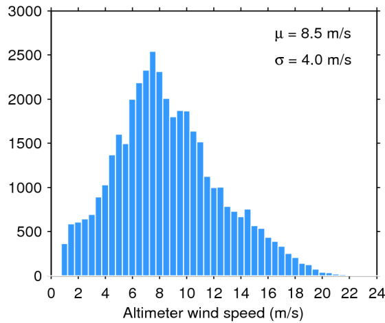
Figure 33. Histogram of flag-valid wind over oceans and lakes for 25/05/2020. The mean ( \mu ) and standard deviation ( \sigma ) are also shown. Note that values larger than 24 m/s are excluded from the histogram for the sake of readability but not from the computation of \mu and \sigma .
