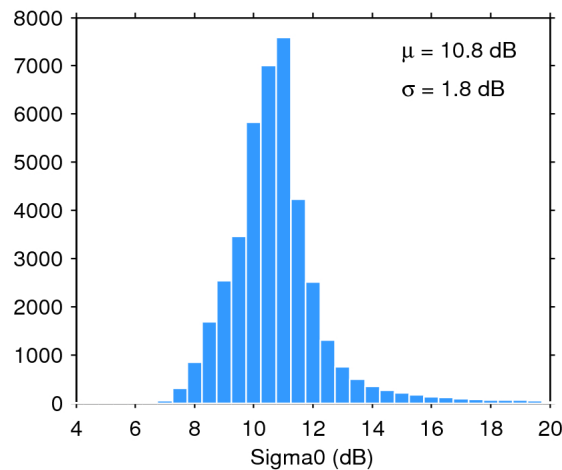
Figure 25. Histogram of flag-valid sigma0 over oceans and lakes for 25/05/2020. The mean ( \mu ) and standard deviation ( \sigma ) are also shown. Note that values outside [4 20] dB are excluded from the histogram for the sake of readability but not from the computation of \mu and \sigma .
