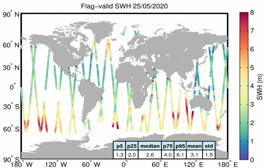
Figure 15. Geographical distribution of flag-valid SWH data over oceans and lakes for 25/05/2020. The statistical values shown in the table refer to the SWH in m and are calculated over all measurements shown in the figure.
