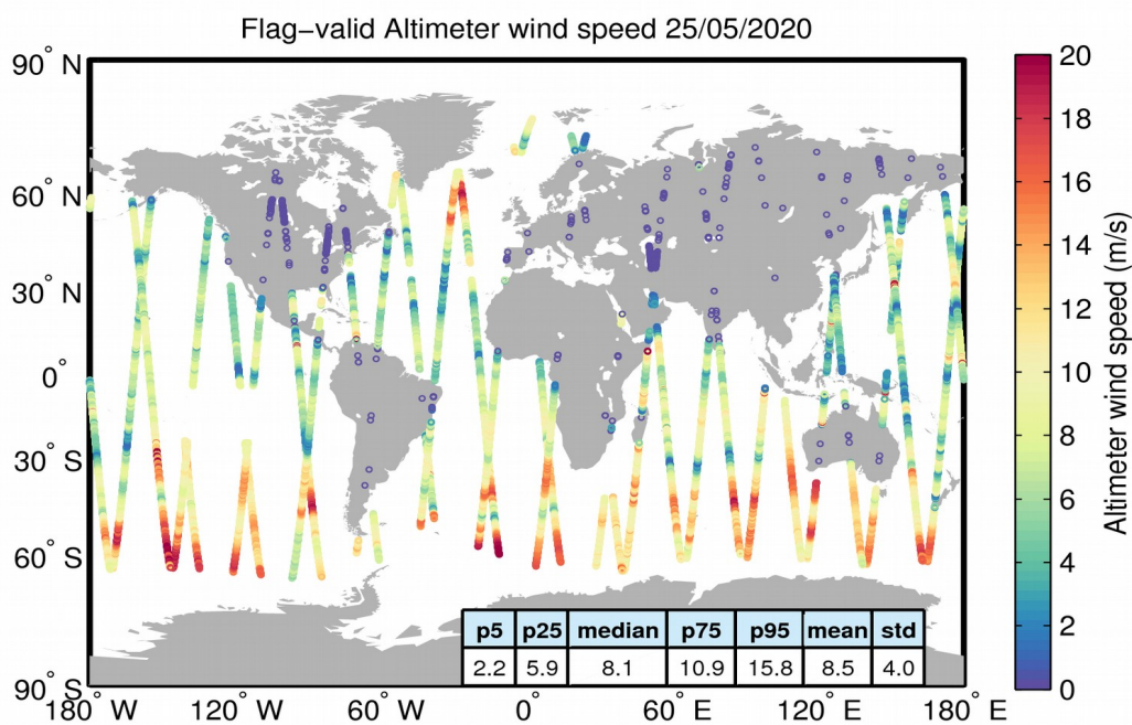
Figure 31. Geographical distribution of flag-valid wind data over oceans and lakes for 25/05/2020. The statistical values shown in the table refer to the wind in m/s and are calculated over all measurements shown in the figure.
