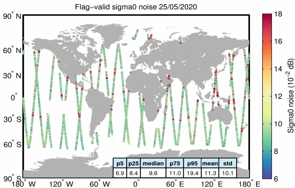
Figure 26. Geographical distribution of flag-valid 20-Hz sigma0 measurement noise over oceans and lakes for 25/05/2020. The statistical values shown in the table refer to the sigma0 noise and are calculated over all measurements shown in the figure.
