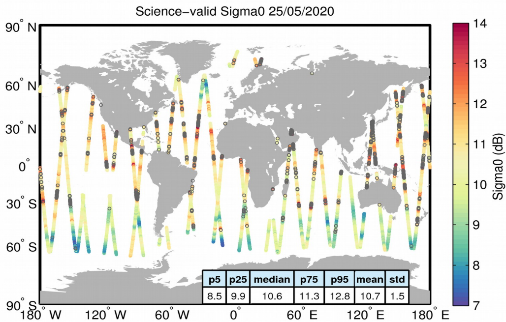
Figure 27. Geographical distribution of science-valid sigma0 data over oceans and lakes for 25/05/2020. The statistical values shown in the table refer to the sigma0 in dB and are calculated over all measurements shown in the figure. Gray circles denote records that have been rejected based on the editing criteria described in Table 4.
