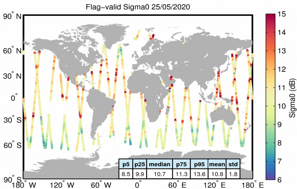
Figure 23. Geographical distribution of flag-valid sigma0 data over oceans and lakes for 25/05/2020. The statistical values shown in the table refer to the sigma0 in dB and are calculated over all measurements shown in the figure.
