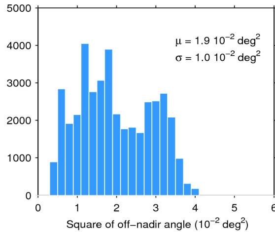
Figure 39. Histogram of flag-valid mispointing over oceans and lakes for 25/05/2020. The mean ( \mu ) and standard deviation ( \sigma ) are also shown. Note that values larger than 6 \cdot 10^{-2} \text{ deg}^2 are excluded from the histogram for the sake of readability but not from the computation of \mu and \sigma .
