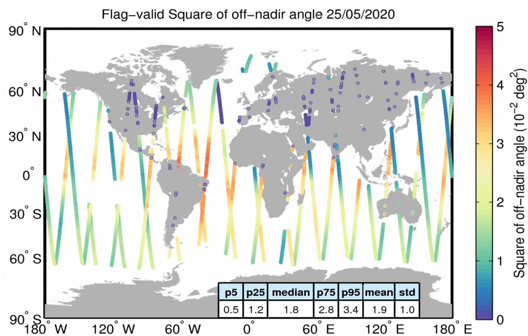
Figure 37. Geographical distribution of flag-valid mispointing data over oceans and lakes for 25/05/2020. The statistical values shown in the table refer to the mispointing in 10^{-2} \text{ deg}^2 and are calculated over all measurements shown in the figure.
