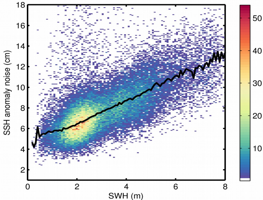
Figure 9. 2D histogram showing flag-valid SSH anomaly noise as a function of SWH for 25/05/2020. The black line denotes the median SSH anomaly noise as a function of SWH.
