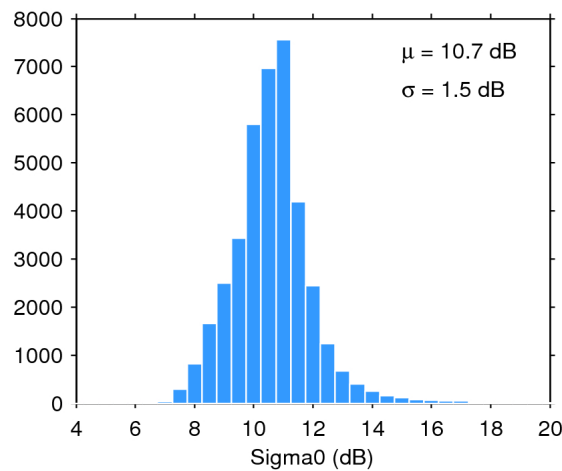
Figure 28. Histogram of science-valid sigma0 over oceans and lakes for 25/05/2020. The mean ( \mu ) and standard deviation ( \sigma ) are also shown. Note that values outside [4 20] dB are excluded from the histogram for the sake of readability but not from the computation of \mu and \sigma .
