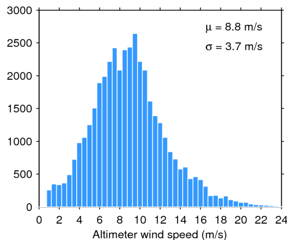
Figure 35. Histogram of science-valid wind over oceans and lakes for 23/05/2020. The mean ( \mu ) and standard deviation ( \sigma ) are also shown. Note that values larger than 24 m/s are excluded from the histogram for the sake of readability but not from the computation of \mu and \sigma .
