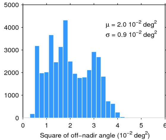
Figure 39. Histogram of flag-valid mispointing over oceans and lakes for 23/05/2020. The mean ( \mu ) and standard deviation ( \sigma ) are also shown. Note that values larger than 6 \cdot 10^{-2} \text{ deg}^2 are excluded from the histogram for the sake of readability but not from the computation of \mu and \sigma .
