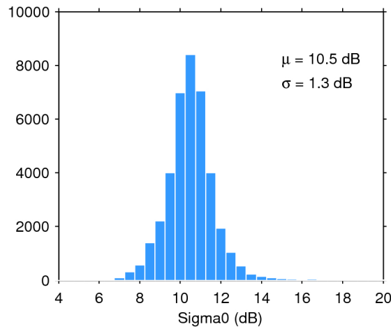
Figure 28. Histogram of science-valid sigma0 over oceans and lakes for 23/05/2020. The mean ( \mu ) and standard deviation ( \sigma ) are also shown. Note that values outside [4 20] dB are excluded from the histogram for the sake of readability but not from the computation of \mu and \sigma .
