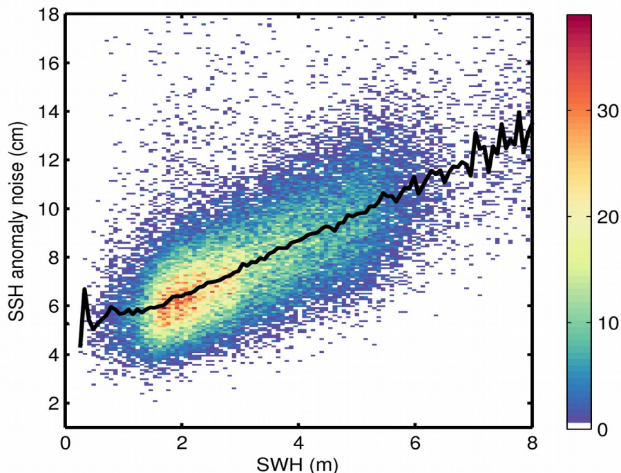
Figure 9. 2D histogram showing flag-valid SSH anomaly noise as a function of SWH for 23/05/2020. The black line denotes the median SSH anomaly noise as a function of SWH.
