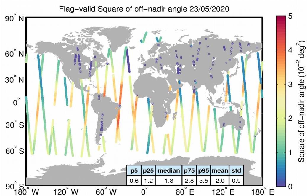
Figure 37. Geographical distribution of flag-valid mispointing data over oceans and lakes for 23/05/2020. The statistical values shown in the table refer to the mispointing in 10^{-2} \text{ deg}^2 and are calculated over all measurements shown in the figure.
