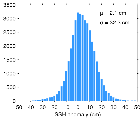
Figure 7. Histogram of flag-valid SSH anomaly over oceans and lakes for 23/05/2020. The mean ( \mu ) and standard deviation ( \sigma ) are also shown. Note that values outside [-50 50] cm are excluded from the histogram for the sake of readability but not from the computation of \mu and \sigma .
