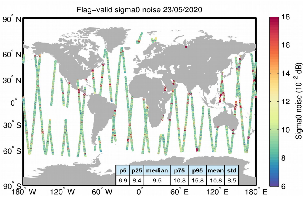
Figure 26. Geographical distribution of flag-valid 20-Hz sigma0 measurement noise over oceans and lakes for 23/05/2020. The statistical values shown in the table refer to the sigma0 noise and are calculated over all measurements shown in the figure.
