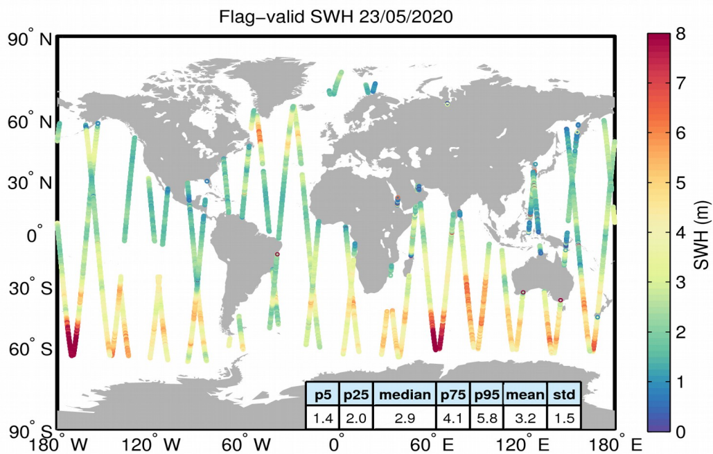
Figure 15. Geographical distribution of flag-valid SWH data over oceans and lakes for 23/05/2020. The statistical values shown in the table refer to the SWH in m and are calculated over all measurements shown in the figure.
