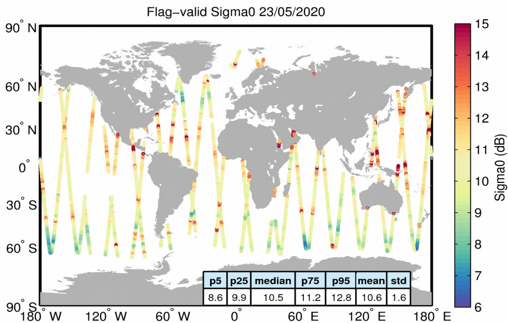
Figure 23. Geographical distribution of flag-valid sigma0 data over oceans and lakes for 23/05/2020. The statistical values shown in the table refer to the sigma0 in dB and are calculated over all measurements shown in the figure.
