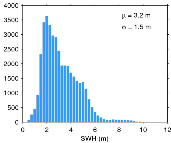
Figure 17. Histogram of flag-valid SWH over oceans and lakes for 23/05/2020. The mean ( \mu ) and standard deviation ( \sigma ) are also shown. Note that values larger than 12 m are excluded from the histogram for the sake of readability but not from the computation of \mu and \sigma .
