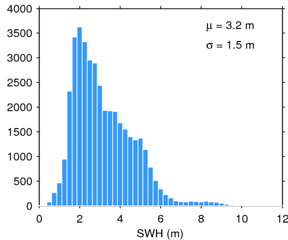
Figure 20. Histogram of science-valid SWH over oceans and lakes for 23/05/2020. The mean ( \mu ) and standard deviation ( \sigma ) are also shown. Note that values larger than 12 m are excluded from the histogram for the sake of readability but not from the computation of \mu and \sigma .
