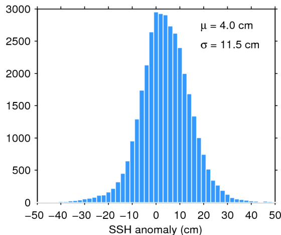
Figure 11. Histogram of science-valid SSH anomaly over oceans and lakes for 23/05/2020. The mean ( \mu ) and standard deviation ( \sigma ) are also shown. Note that values outside [-50 50] cm are excluded from the histogram for the sake of readability but not from the computation of \mu and \sigma .
