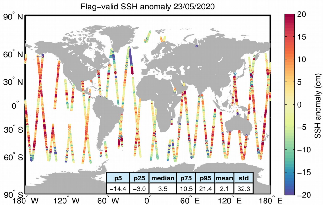
Figure 5. Geographical distribution of flag-valid 1-Hz SSH anomaly data over oceans and lakes for 23/05/2020. The statistical values shown in the table refer to the SSH anomaly in cm and are calculated over all measurements shown in the figure.
