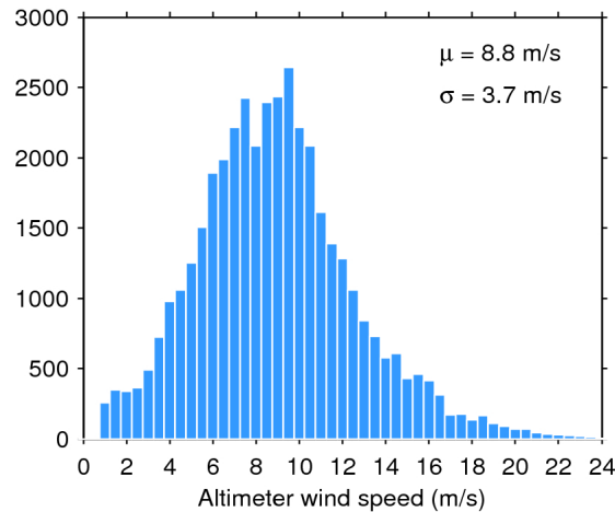
Figure 33. Histogram of flag-valid wind over oceans and lakes for 23/05/2020. The mean ( \mu ) and standard deviation ( \sigma ) are also shown. Note that values larger than 24 m/s are excluded from the histogram for the sake of readability but not from the computation of \mu and \sigma .
