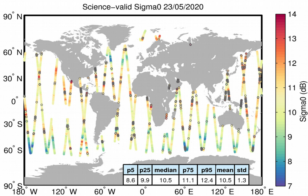
Figure 27. Geographical distribution of science-valid sigma0 data over oceans and lakes for 23/05/2020. The statistical values shown in the table refer to the sigma0 in dB and are calculated over all measurements shown in the figure. Gray circles denote records that have been rejected based on the editing criteria described in Table 4.
