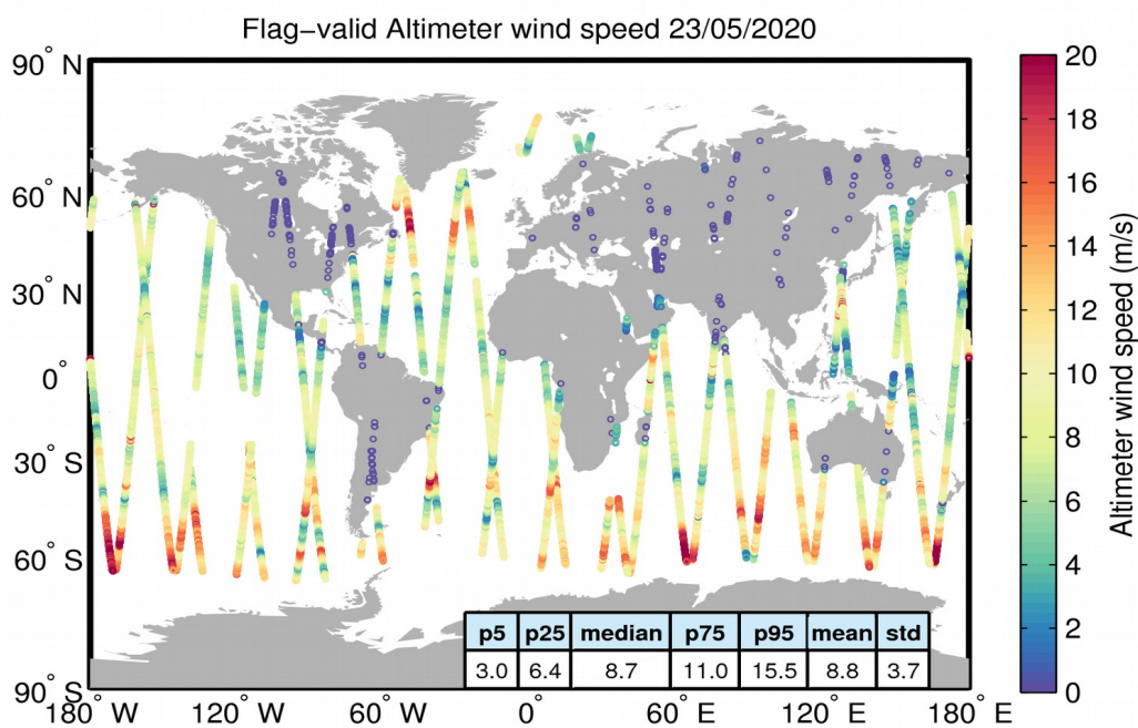
Figure 31. Geographical distribution of flag-valid wind data over oceans and lakes for 23/05/2020. The statistical values shown in the table refer to the wind in m/s and are calculated over all measurements shown in the figure.
