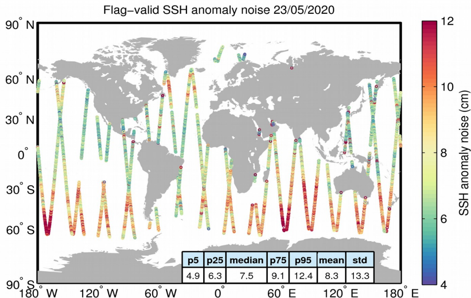
Figure 8. Geographical distribution of flag-valid 20-Hz SSH anomaly measurement noise over oceans and lakes for 23/05/2020. The statistical values shown in the table refer to the SSH anomaly noise and are calculated over all measurements shown in the figure.
