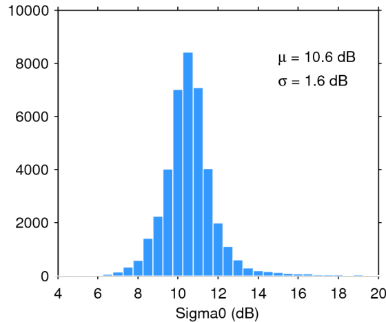
Figure 25. Histogram of flag-valid sigma0 over oceans and lakes for 23/05/2020. The mean ( \mu ) and standard deviation ( \sigma ) are also shown. Note that values outside [4 20] dB are excluded from the histogram for the sake of readability but not from the computation of \mu and \sigma .
