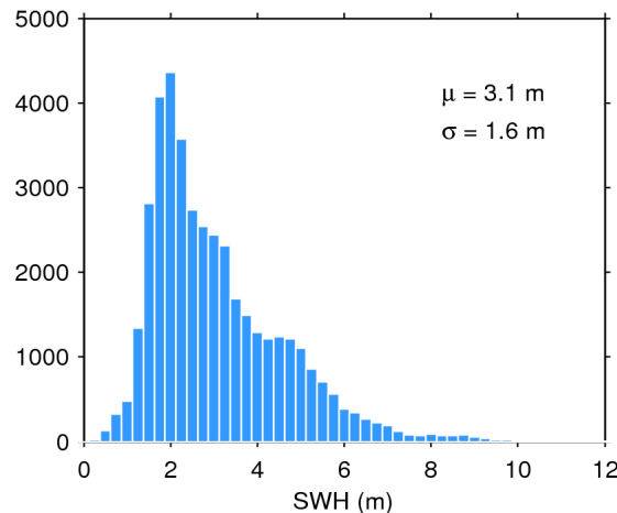
Figure 20. Histogram of science-valid SWH over oceans and lakes for 22/05/2020. The mean ( \mu ) and standard deviation ( \sigma ) are also shown. Note that values larger than 12 m are excluded from the histogram for the sake of readability but not from the computation of \mu and \sigma .
