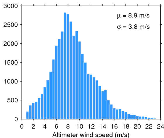
Figure 35. Histogram of science-valid wind over oceans and lakes for 22/05/2020. The mean ( \mu ) and standard deviation ( \sigma ) are also shown. Note that values larger than 24 m/s are excluded from the histogram for the sake of readability but not from the computation of \mu and \sigma .
