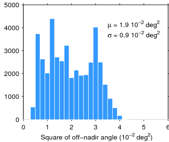
Figure 39. Histogram of flag-valid mispointing over oceans and lakes for 22/05/2020. The mean ( \mu ) and standard deviation ( \sigma ) are also shown. Note that values larger than 6 \cdot 10^{-2} \text{ deg}^2 are excluded from the histogram for the sake of readability but not from the computation of \mu and \sigma .
