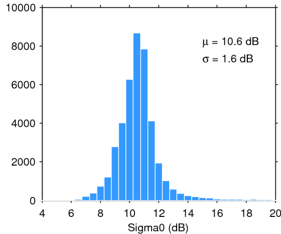
Figure 25. Histogram of flag-valid sigma0 over oceans and lakes for 22/05/2020. The mean ( \mu ) and standard deviation ( \sigma ) are also shown. Note that values outside [4 20] dB are excluded from the histogram for the sake of readability but not from the computation of \mu and \sigma .
