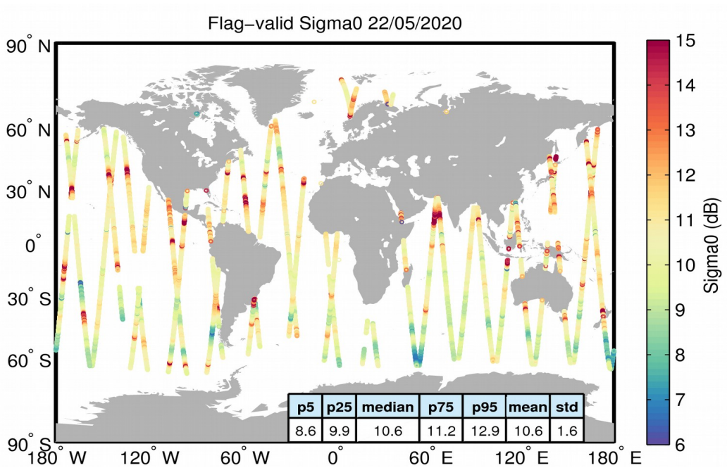
Figure 23. Geographical distribution of flag-valid sigma0 data over oceans and lakes for 22/05/2020. The statistical values shown in the table refer to the sigma0 in dB and are calculated over all measurements shown in the figure.
