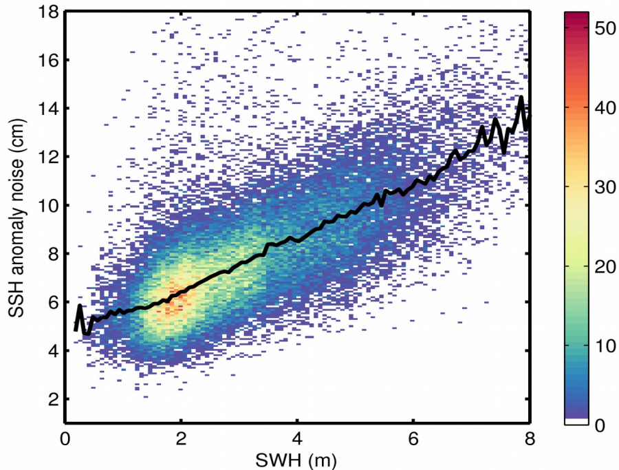
Figure 9. 2D histogram showing flag-valid SSH anomaly noise as a function of SWH for 22/05/2020. The black line denotes the median SSH anomaly noise as a function of SWH.
