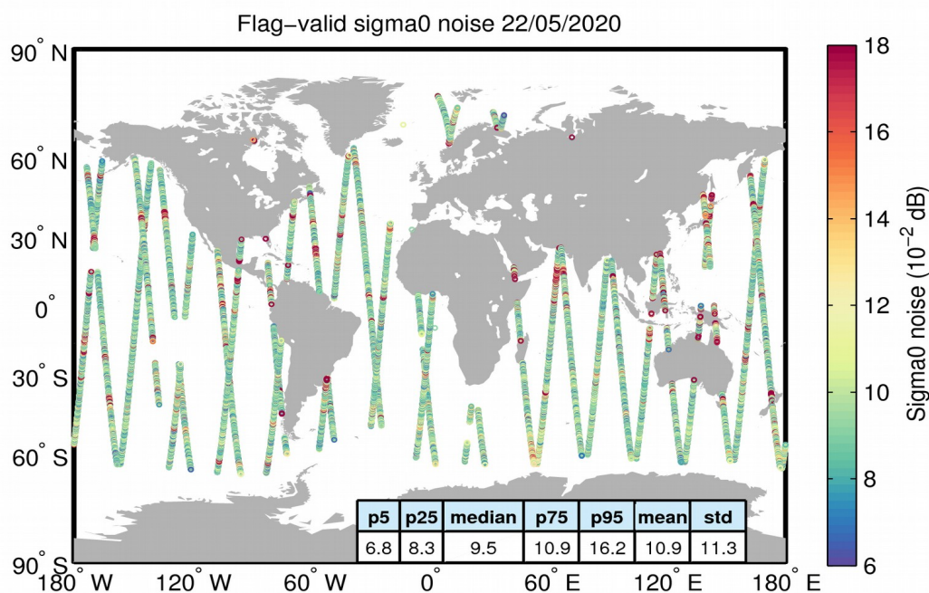
Figure 26. Geographical distribution of flag-valid 20-Hz sigma0 measurement noise over oceans and lakes for 22/05/2020. The statistical values shown in the table refer to the sigma0 noise and are calculated over all measurements shown in the figure.
