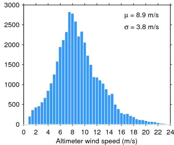
Figure 33. Histogram of flag-valid wind over oceans and lakes for 22/05/2020. The mean ( \mu ) and standard deviation ( \sigma ) are also shown. Note that values larger than 24 m/s are excluded from the histogram for the sake of readability but not from the computation of \mu and \sigma .
