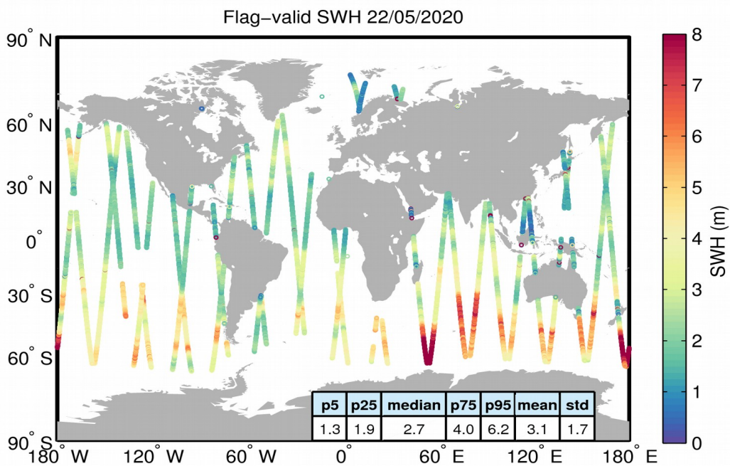
Figure 15. Geographical distribution of flag-valid SWH data over oceans and lakes for 22/05/2020. The statistical values shown in the table refer to the SWH in m and are calculated over all measurements shown in the figure.
