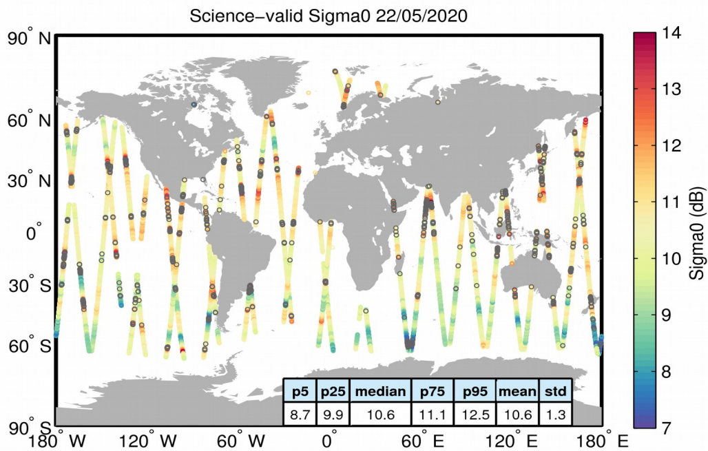
Figure 27. Geographical distribution of science-valid sigma0 data over oceans and lakes for 22/05/2020. The statistical values shown in the table refer to the sigma0 in dB and are calculated over all measurements shown in the figure. Gray circles denote records that have been rejected based on the editing criteria described in Table 4.
