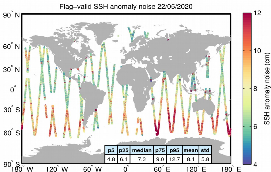
Figure 8. Geographical distribution of flag-valid 20-Hz SSH anomaly measurement noise over oceans and lakes for 22/05/2020. The statistical values shown in the table refer to the SSH anomaly noise and are calculated over all measurements shown in the figure.
