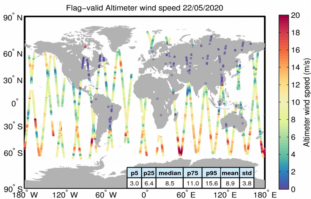
Figure 31. Geographical distribution of flag-valid wind data over oceans and lakes for 22/05/2020. The statistical values shown in the table refer to the wind in m/s and are calculated over all measurements shown in the figure.
