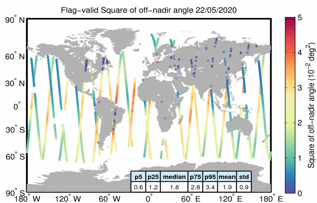
Figure 37. Geographical distribution of flag-valid mispointing data over oceans and lakes for 22/05/2020. The statistical values shown in the table refer to the mispointing in 10^{-2} \text{ deg}^2 and are calculated over all measurements shown in the figure.
