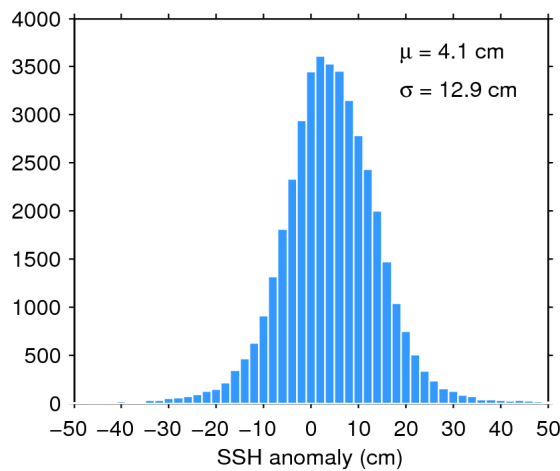
Figure 7. Histogram of flag-valid SSH anomaly over oceans and lakes for 22/05/2020. The mean ( \mu ) and standard deviation ( \sigma ) are also shown. Note that values outside [-50 50] cm are excluded from the histogram for the sake of readability but not from the computation of \mu and \sigma .
