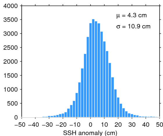
Figure 11. Histogram of science-valid SSH anomaly over oceans and lakes for 22/05/2020. The mean ( \mu ) and standard deviation ( \sigma ) are also shown. Note that values outside [-50 50] cm are excluded from the histogram for the sake of readability but not from the computation of \mu and \sigma .
