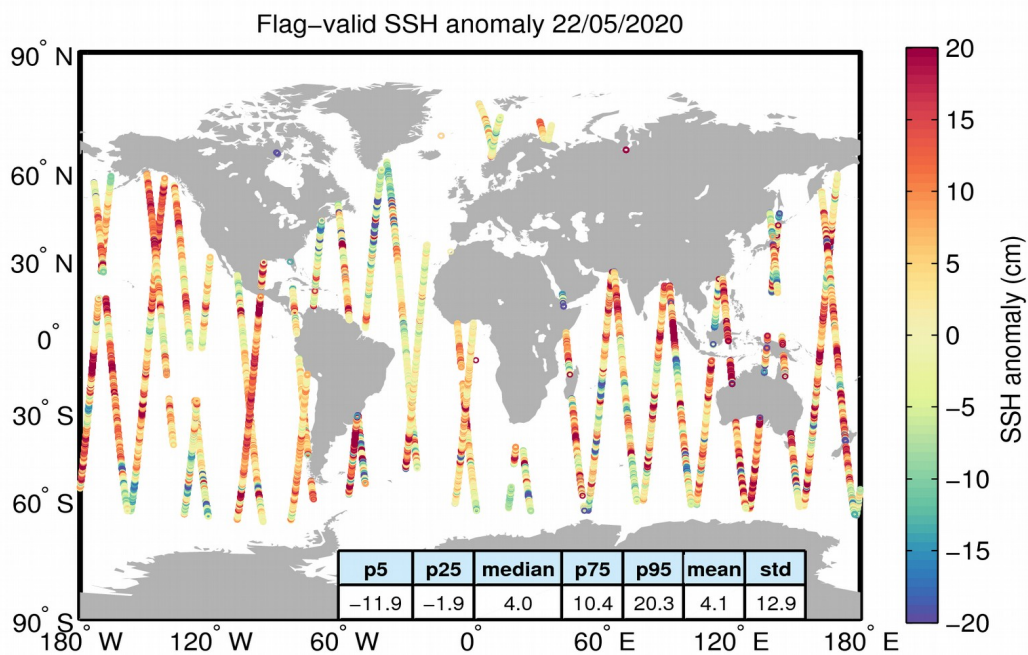
Figure 5. Geographical distribution of flag-valid 1-Hz SSH anomaly data over oceans and lakes for 22/05/2020. The statistical values shown in the table refer to the SSH anomaly in cm and are calculated over all measurements shown in the figure.
