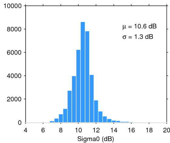
Figure 28. Histogram of science-valid sigma0 over oceans and lakes for 22/05/2020. The mean ( \mu ) and standard deviation ( \sigma ) are also shown. Note that values outside [4 20] dB are excluded from the histogram for the sake of readability but not from the computation of \mu and \sigma .
