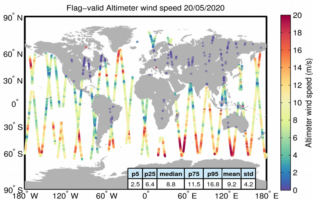
Figure 31. Geographical distribution of flag-valid wind data over oceans and lakes for 20/05/2020. The statistical values shown in the table refer to the wind in m/s and are calculated over all measurements shown in the figure.
