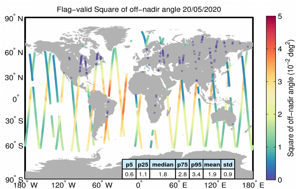
Figure 37. Geographical distribution of flag-valid mispointing data over oceans and lakes for 20/05/2020. The statistical values shown in the table refer to the mispointing in 10^{-2} \text{ deg}^2 and are calculated over all measurements shown in the figure.
