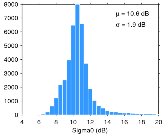
Figure 25. Histogram of flag-valid sigma0 over oceans and lakes for 20/05/2020. The mean ( \mu ) and standard deviation ( \sigma ) are also shown. Note that values outside [4 20] dB are excluded from the histogram for the sake of readability but not from the computation of \mu and \sigma .
