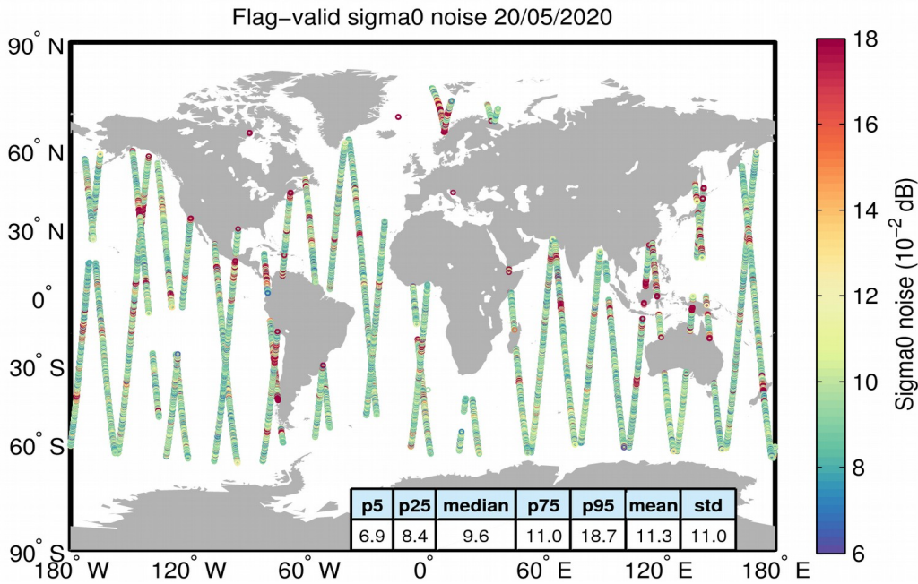
Figure 26. Geographical distribution of flag-valid 20-Hz sigma0 measurement noise over oceans and lakes for 20/05/2020. The statistical values shown in the table refer to the sigma0 noise and are calculated over all measurements shown in the figure.
