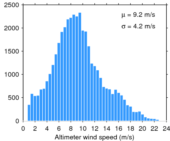
Figure 33. Histogram of flag-valid wind over oceans and lakes for 20/05/2020. The mean ( \mu ) and standard deviation ( \sigma ) are also shown. Note that values larger than 24 m/s are excluded from the histogram for the sake of readability but not from the computation of \mu and \sigma .
