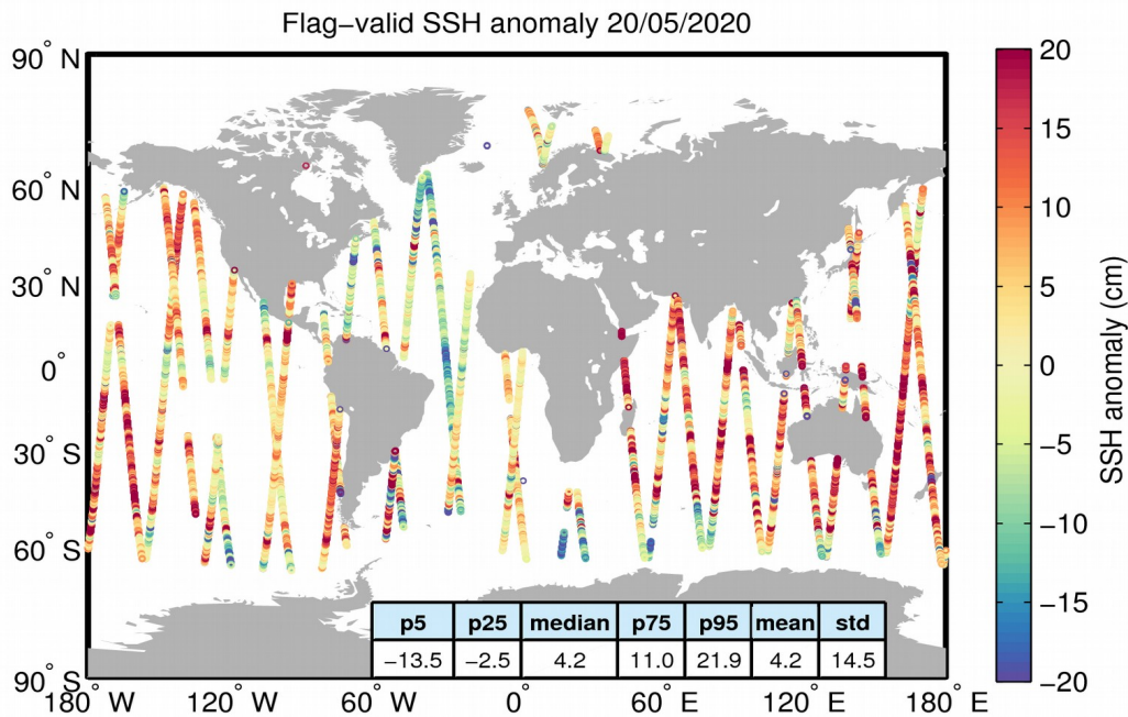
Figure 5. Geographical distribution of flag-valid 1-Hz SSH anomaly data over oceans and lakes for 20/05/2020. The statistical values shown in the table refer to the SSH anomaly in cm and are calculated over all measurements shown in the figure.
