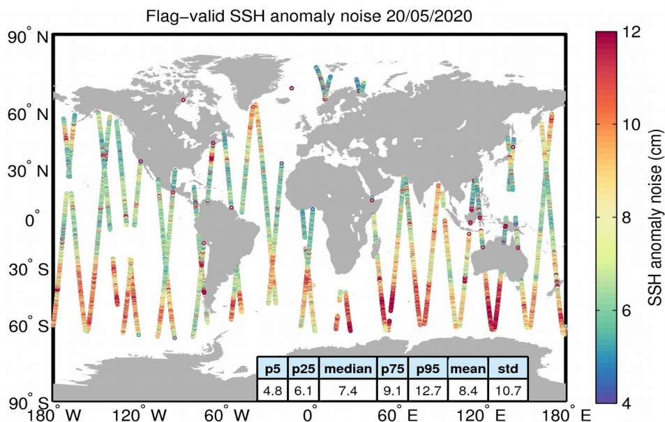
Figure 8. Geographical distribution of flag-valid 20-Hz SSH anomaly measurement noise over oceans and lakes for 20/05/2020. The statistical values shown in the table refer to the SSH anomaly noise and are calculated over all measurements shown in the figure.
