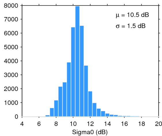
Figure 28. Histogram of science-valid sigma0 over oceans and lakes for 20/05/2020. The mean ( \mu ) and standard deviation ( \sigma ) are also shown. Note that values outside [4 20] dB are excluded from the histogram for the sake of readability but not from the computation of \mu and \sigma .
