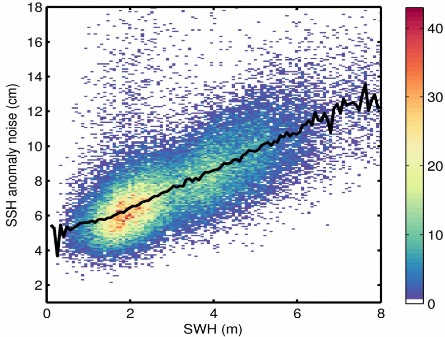
Figure 9. 2D histogram showing flag-valid SSH anomaly noise as a function of SWH for 20/05/2020. The black line denotes the median SSH anomaly noise as a function of SWH.
