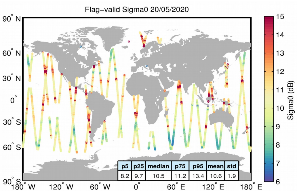
Figure 23. Geographical distribution of flag-valid sigma0 data over oceans and lakes for 20/05/2020. The statistical values shown in the table refer to the sigma0 in dB and are calculated over all measurements shown in the figure.
