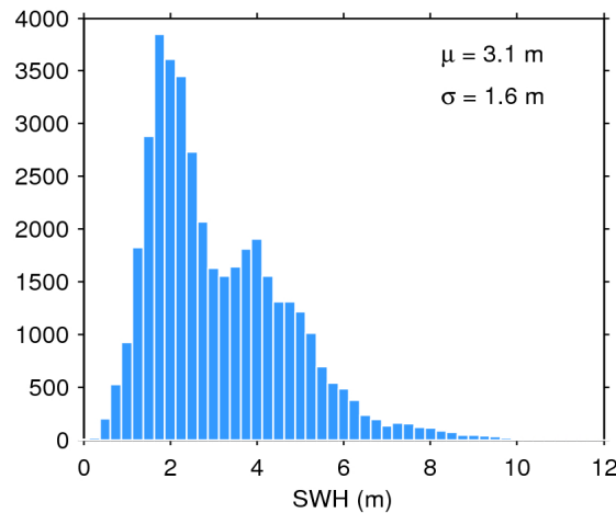
Figure 20. Histogram of science-valid SWH over oceans and lakes for 20/05/2020. The mean ( \mu ) and standard deviation ( \sigma ) are also shown. Note that values larger than 12 m are excluded from the histogram for the sake of readability but not from the computation of \mu and \sigma .
