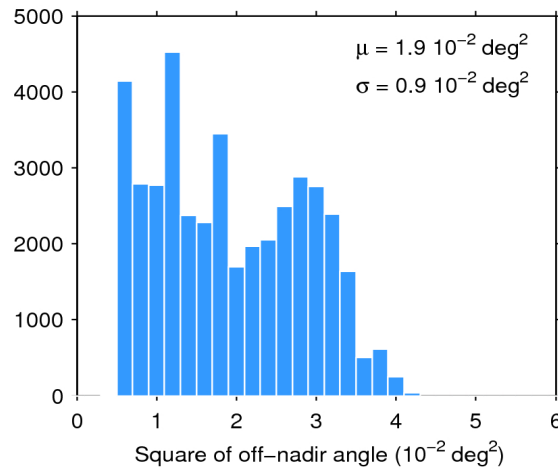
Figure 39. Histogram of flag-valid mispointing over oceans and lakes for 20/05/2020. The mean ( \mu ) and standard deviation ( \sigma ) are also shown. Note that values larger than 6 \cdot 10^{-2} \text{ deg}^2 are excluded from the histogram for the sake of readability but not from the computation of \mu and \sigma .
