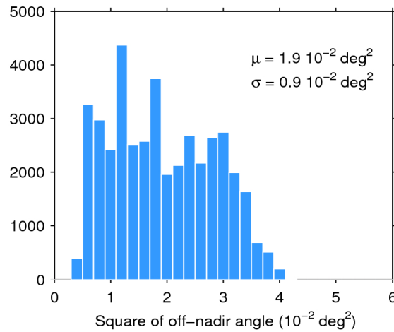
Figure 39. Histogram of flag-valid mispointing over oceans and lakes for 18/05/2020. The mean ( \mu ) and standard deviation ( \sigma ) are also shown. Note that values larger than 6 \cdot 10^{-2} \text{ deg}^2 are excluded from the histogram for the sake of readability but not from the computation of \mu and \sigma .
