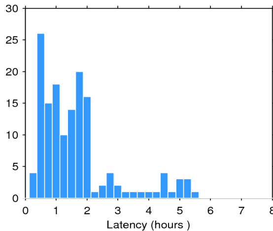
Figure 2. Histogram of the data latency for 18/05/2020. The y-axis denotes the number of files that are made available with a delay of x-hours with respect to the mean time of the records stored in the file.
