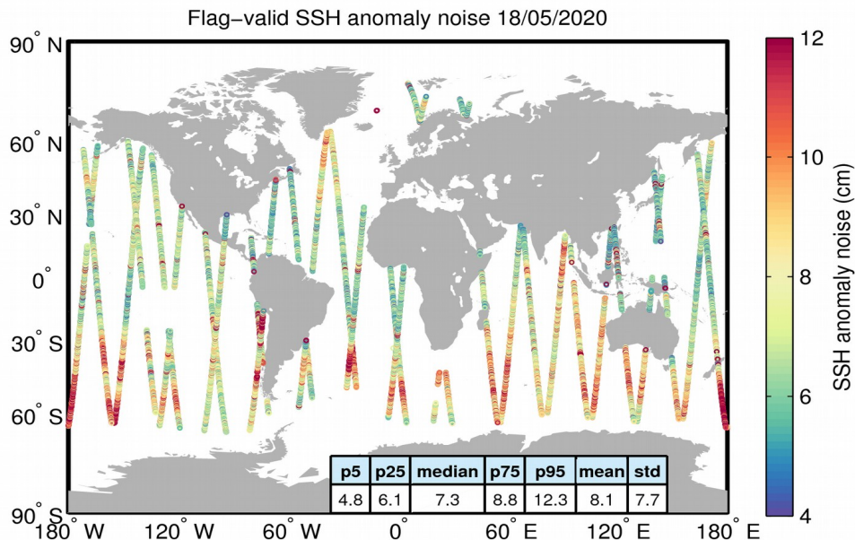
Figure 8. Geographical distribution of flag-valid 20-Hz SSH anomaly measurement noise over oceans and lakes for 18/05/2020. The statistical values shown in the table refer to the SSH anomaly noise and are calculated over all measurements shown in the figure.
