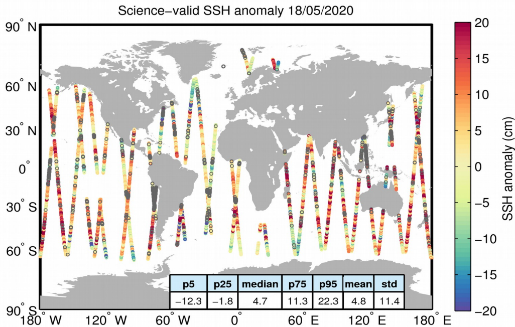
Figure 10. Geographical distribution of science-valid SSH anomaly data over oceans and lakes for 18/05/2020. The statistical values shown in the table refer to the SSH anomaly in cm and are calculated over all measurements shown in the figure. Gray circles denote records that have been rejected based on the editing criteria described in Table 2.
