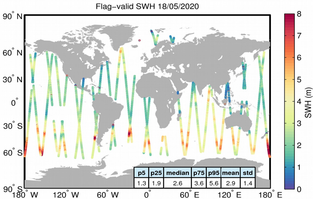
Figure 15. Geographical distribution of flag-valid SWH data over oceans and lakes for 18/05/2020. The statistical values shown in the table refer to the SWH in m and are calculated over all measurements shown in the figure.
