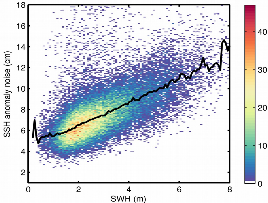
Figure 9. 2D histogram showing flag-valid SSH anomaly noise as a function of SWH for 18/05/2020. The black line denotes the median SSH anomaly noise as a function of SWH.
