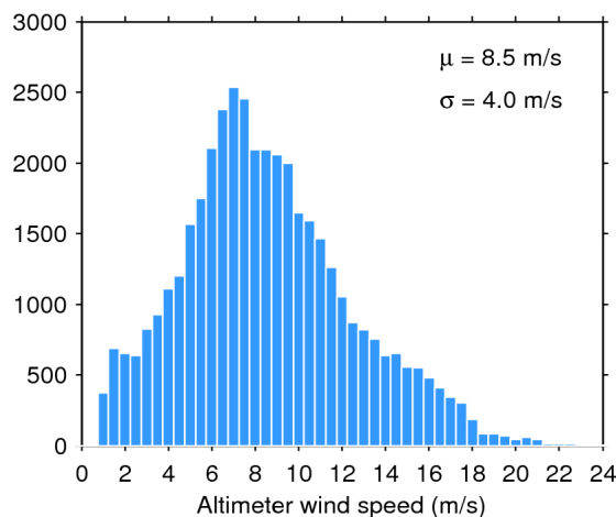
Figure 35. Histogram of science-valid wind over oceans and lakes for 18/05/2020. The mean ( \mu ) and standard deviation ( \sigma ) are also shown. Note that values larger than 24 m/s are excluded from the histogram for the sake of readability but not from the computation of \mu and \sigma .
