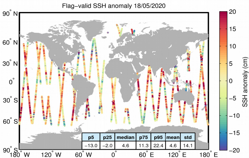
Figure 5. Geographical distribution of flag-valid 1-Hz SSH anomaly data over oceans and lakes for 18/05/2020. The statistical values shown in the table refer to the SSH anomaly in cm and are calculated over all measurements shown in the figure.
