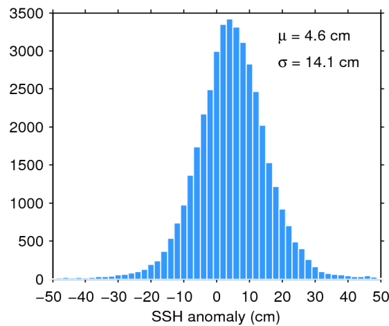
Figure 7. Histogram of flag-valid SSH anomaly over oceans and lakes for 18/05/2020. The mean ( \mu ) and standard deviation ( \sigma ) are also shown. Note that values outside [-50 50] cm are excluded from the histogram for the sake of readability but not from the computation of \mu and \sigma .
