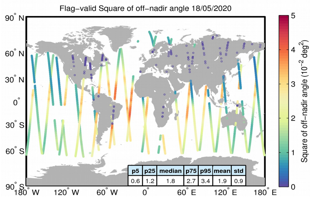
Figure 37. Geographical distribution of flag-valid mispointing data over oceans and lakes for 18/05/2020. The statistical values shown in the table refer to the mispointing in 10^{-2} \text{ deg}^2 and are calculated over all measurements shown in the figure.
