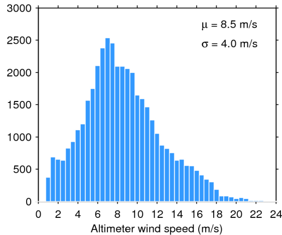
Figure 33. Histogram of flag-valid wind over oceans and lakes for 18/05/2020. The mean ( \mu ) and standard deviation ( \sigma ) are also shown. Note that values larger than 24 m/s are excluded from the histogram for the sake of readability but not from the computation of \mu and \sigma .
