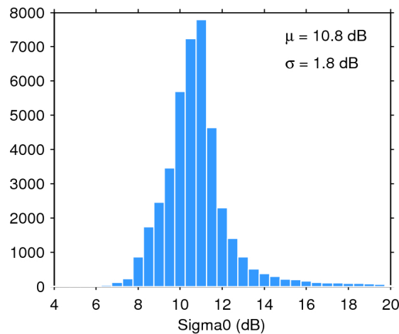
Figure 25. Histogram of flag-valid sigma0 over oceans and lakes for 18/05/2020. The mean ( \mu ) and standard deviation ( \sigma ) are also shown. Note that values outside [4 20] dB are excluded from the histogram for the sake of readability but not from the computation of \mu and \sigma .
