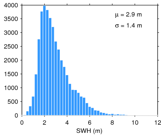
Figure 17. Histogram of flag-valid SWH over oceans and lakes for 18/05/2020. The mean ( \mu ) and standard deviation ( \sigma ) are also shown. Note that values larger than 12 m are excluded from the histogram for the sake of readability but not from the computation of \mu and \sigma .
