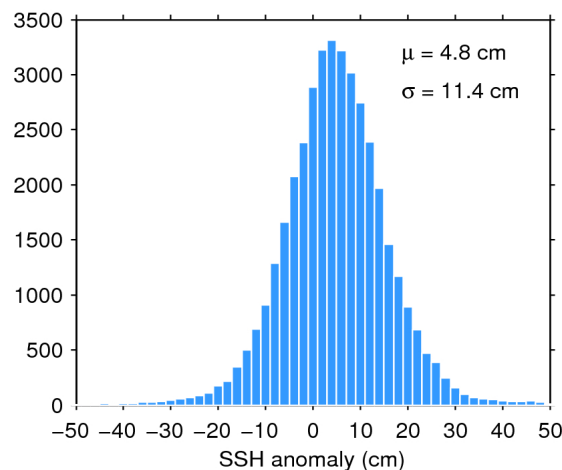
Figure 11. Histogram of science-valid SSH anomaly over oceans and lakes for 18/05/2020. The mean ( \mu ) and standard deviation ( \sigma ) are also shown. Note that values outside [-50 50] cm are excluded from the histogram for the sake of readability but not from the computation of \mu and \sigma .
