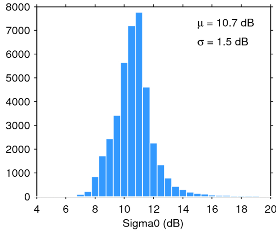
Figure 28. Histogram of science-valid sigma0 over oceans and lakes for 18/05/2020. The mean ( \mu ) and standard deviation ( \sigma ) are also shown. Note that values outside [4 20] dB are excluded from the histogram for the sake of readability but not from the computation of \mu and \sigma .
