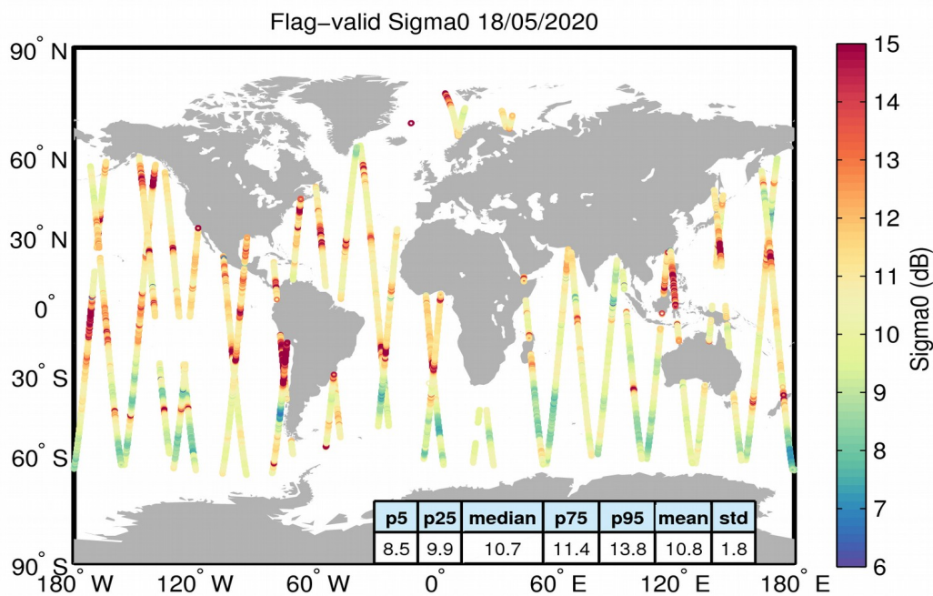
Figure 23. Geographical distribution of flag-valid sigma0 data over oceans and lakes for 18/05/2020. The statistical values shown in the table refer to the sigma0 in dB and are calculated over all measurements shown in the figure.
