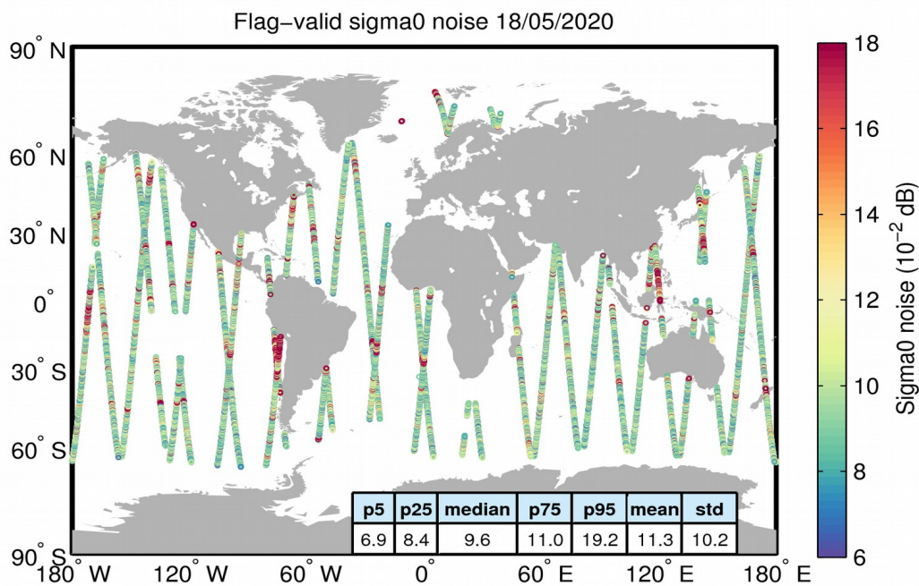
Figure 26. Geographical distribution of flag-valid 20-Hz sigma0 measurement noise over oceans and lakes for 18/05/2020. The statistical values shown in the table refer to the sigma0 noise and are calculated over all measurements shown in the figure.
