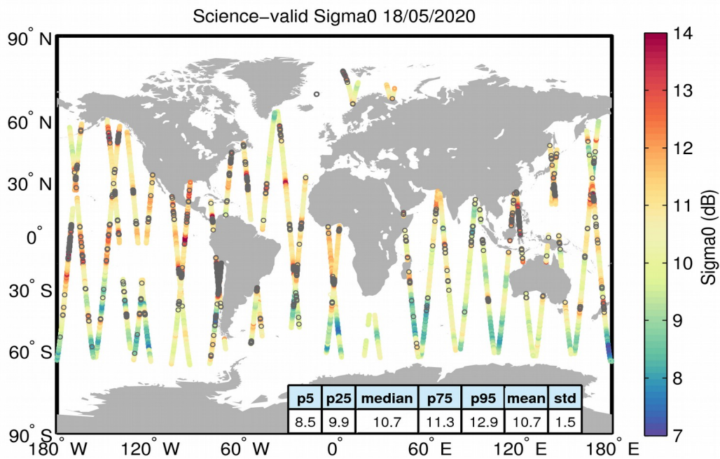
Figure 27. Geographical distribution of science-valid sigma0 data over oceans and lakes for 18/05/2020. The statistical values shown in the table refer to the sigma0 in dB and are calculated over all measurements shown in the figure. Gray circles denote records that have been rejected based on the editing criteria described in Table 4.
