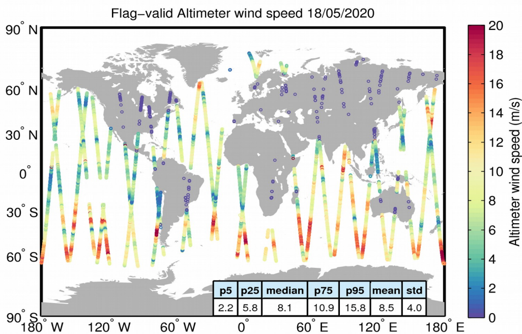
Figure 31. Geographical distribution of flag-valid wind data over oceans and lakes for 18/05/2020. The statistical values shown in the table refer to the wind in m/s and are calculated over all measurements shown in the figure.
