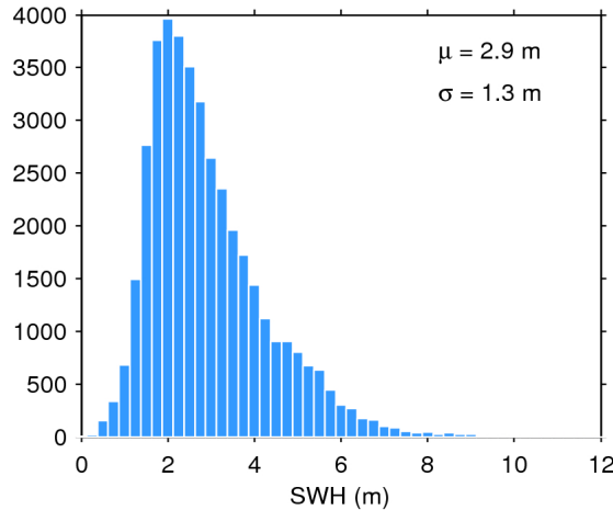
Figure 20. Histogram of science-valid SWH over oceans and lakes for 18/05/2020. The mean ( \mu ) and standard deviation ( \sigma ) are also shown. Note that values larger than 12 m are excluded from the histogram for the sake of readability but not from the computation of \mu and \sigma .
