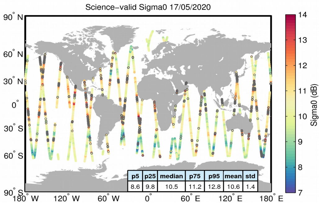
Figure 27. Geographical distribution of science-valid sigma0 data over oceans and lakes for 17/05/2020. The statistical values shown in the table refer to the sigma0 in dB and are calculated over all measurements shown in the figure. Gray circles denote records that have been rejected based on the editing criteria described in Table 4.
