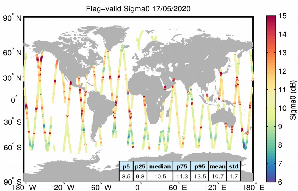
Figure 23. Geographical distribution of flag-valid sigma0 data over oceans and lakes for 17/05/2020. The statistical values shown in the table refer to the sigma0 in dB and are calculated over all measurements shown in the figure.
