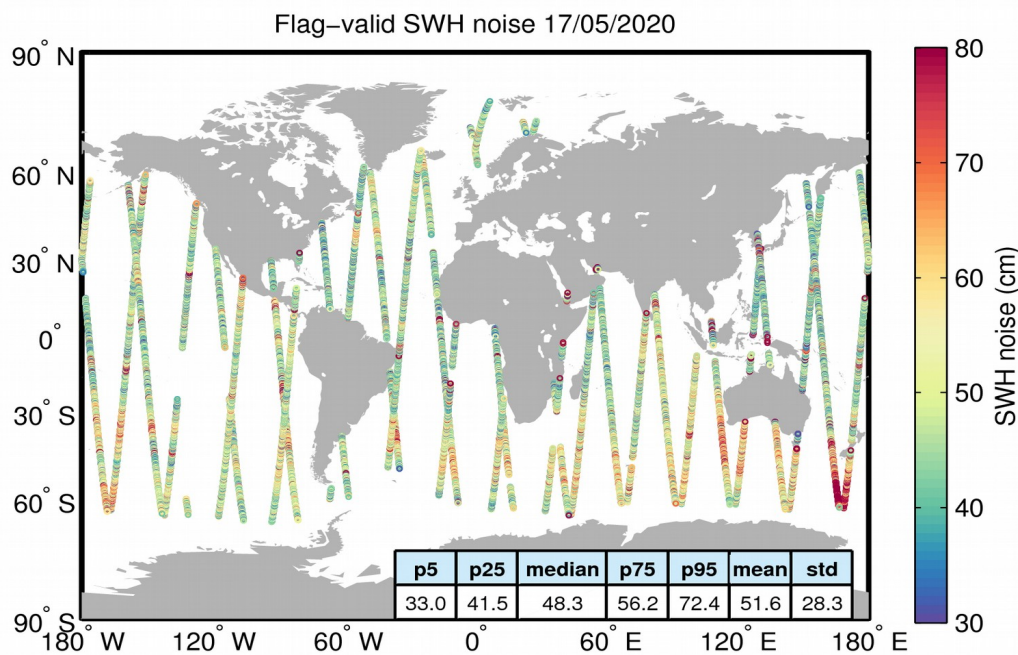
Figure 18. Geographical distribution of flag-valid 20-Hz SWH measurement noise over oceans and lakes for 17/05/2020. The statistical values shown in the figure refer to the SWH noise and are calculated over all measurements shown in the figure.
