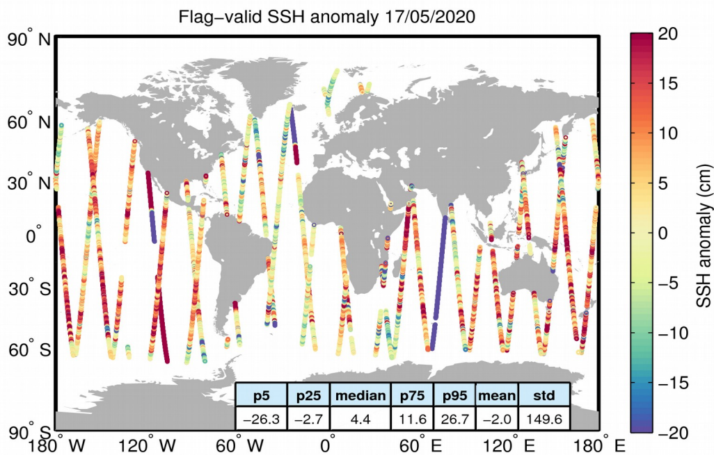
Figure 5. Geographical distribution of flag-valid 1-Hz SSH anomaly data over oceans and lakes for 17/05/2020. The statistical values shown in the table refer to the SSH anomaly in cm and are calculated over all measurements shown in the figure.
