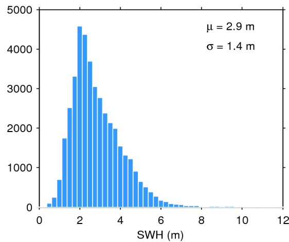
Figure 17. Histogram of flag-valid SWH over oceans and lakes for 17/05/2020. The mean ( \mu ) and standard deviation ( \sigma ) are also shown. Note that values larger than 12 m are excluded from the histogram for the sake of readability but not from the computation of \mu and \sigma .
