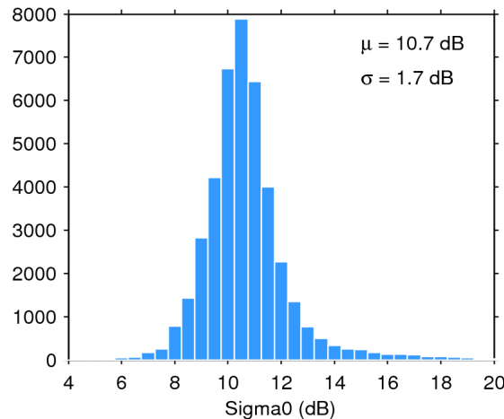
Figure 25. Histogram of flag-valid sigma0 over oceans and lakes for 17/05/2020. The mean ( \mu ) and standard deviation ( \sigma ) are also shown. Note that values outside [4 20] dB are excluded from the histogram for the sake of readability but not from the computation of \mu and \sigma .
