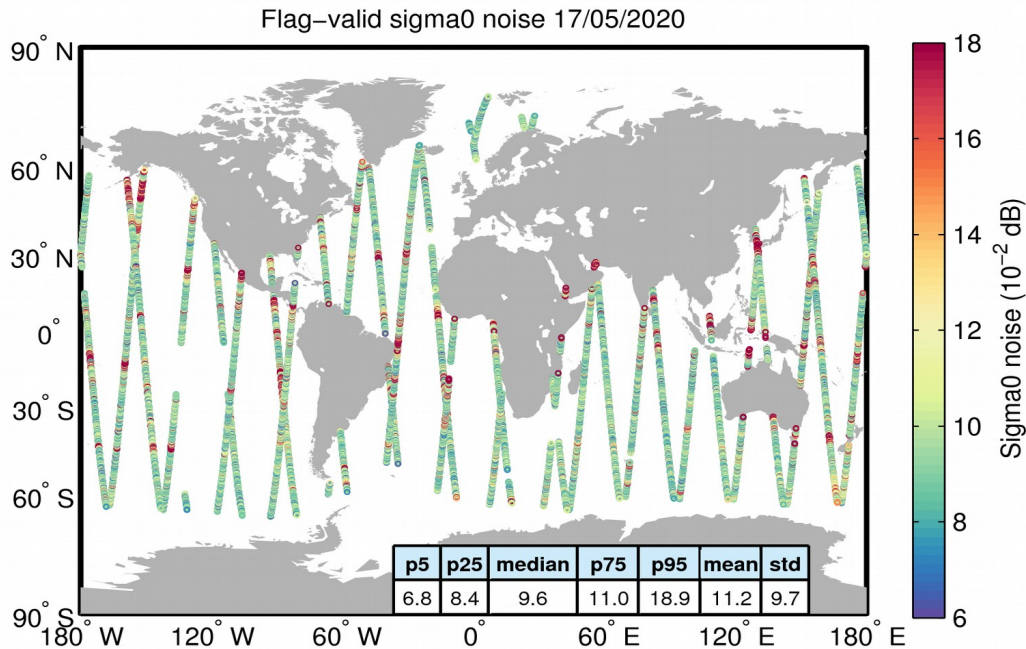
Figure 26. Geographical distribution of flag-valid 20-Hz sigma0 measurement noise over oceans and lakes for 17/05/2020. The statistical values shown in the table refer to the sigma0 noise and are calculated over all measurements shown in the figure.
