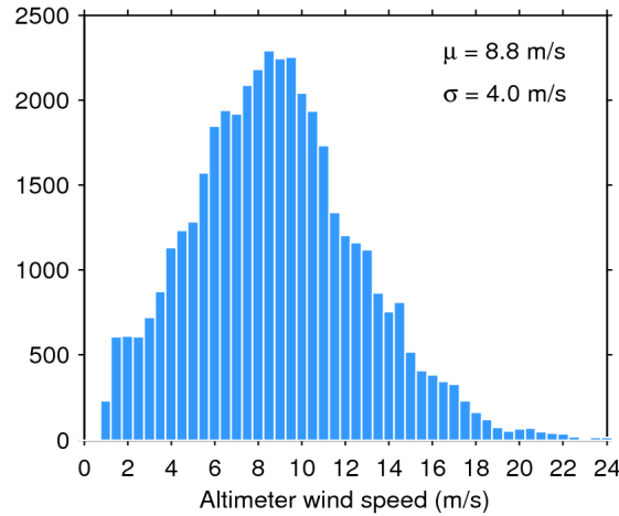
Figure 33. Histogram of flag-valid wind over oceans and lakes for 17/05/2020. The mean ( \mu ) and standard deviation ( \sigma ) are also shown. Note that values larger than 24 m/s are excluded from the histogram for the sake of readability but not from the computation of \mu and \sigma .
