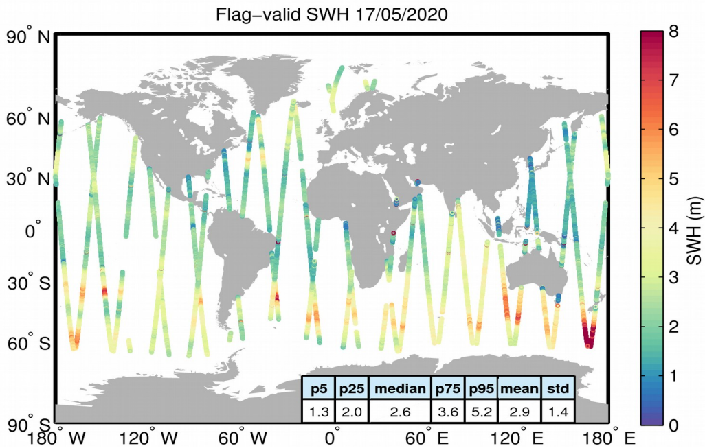
Figure 15. Geographical distribution of flag-valid SWH data over oceans and lakes for 17/05/2020. The statistical values shown in the table refer to the SWH in m and are calculated over all measurements shown in the figure.
