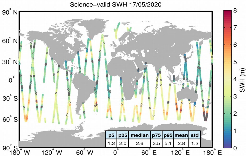
Figure 19. Geographical distribution of science-valid SWH data over oceans and lakes for 17/05/2020. The statistical values shown in the table refer to the SWH in m and are calculated over all measurements shown in the figure. Gray circles denote records that have been rejected based on the editing criteria described in Table 3.
