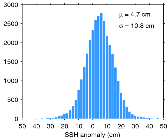
Figure 11. Histogram of science-valid SSH anomaly over oceans and lakes for 17/05/2020. The mean ( \mu ) and standard deviation ( \sigma ) are also shown. Note that values outside [-50 50] cm are excluded from the histogram for the sake of readability but not from the computation of \mu and \sigma .
