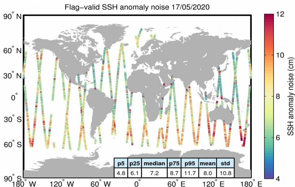
Figure 8. Geographical distribution of flag-valid 20-Hz SSH anomaly measurement noise over oceans and lakes for 17/05/2020. The statistical values shown in the table refer to the SSH anomaly noise and are calculated over all measurements shown in the figure.
