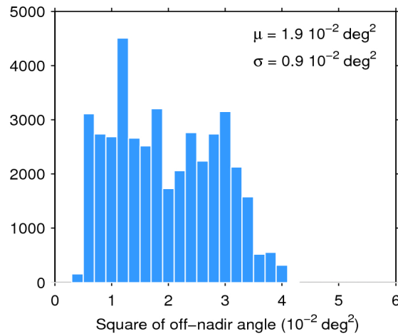
Figure 39. Histogram of flag-valid mispointing over oceans and lakes for 17/05/2020. The mean ( \mu ) and standard deviation ( \sigma ) are also shown. Note that values larger than 6 \cdot 10^{-2} \text{ deg}^2 are excluded from the histogram for the sake of readability but not from the computation of \mu and \sigma .
