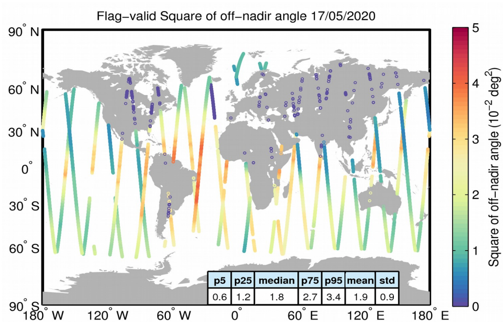
Figure 37. Geographical distribution of flag-valid mispointing data over oceans and lakes for 17/05/2020. The statistical values shown in the table refer to the mispointing in 10^{-2} \text{ deg}^2 and are calculated over all measurements shown in the figure.
