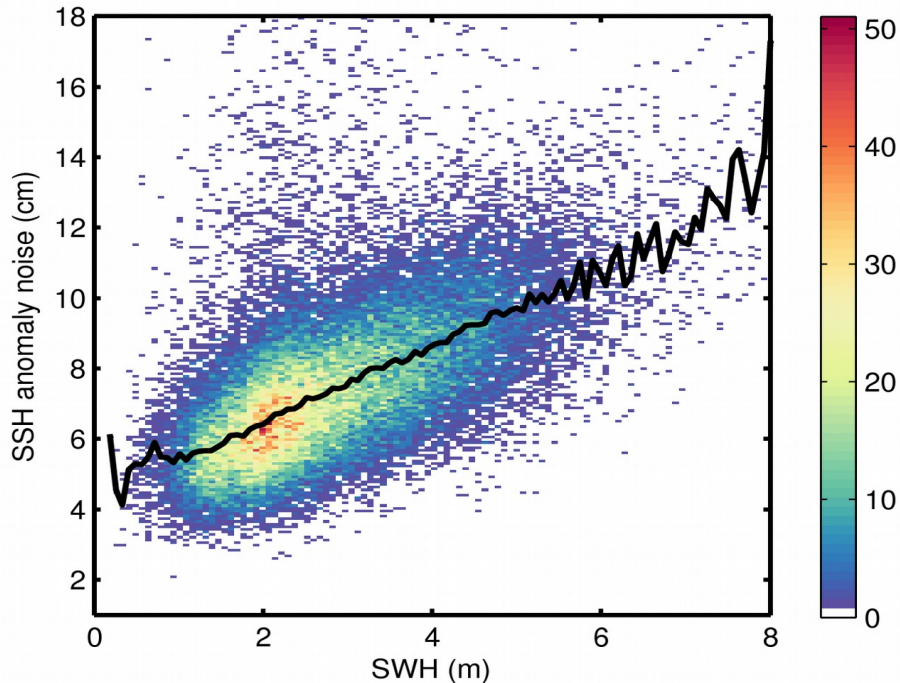
Figure 9. 2D histogram showing flag-valid SSH anomaly noise as a function of SWH for 17/05/2020. The black line denotes the median SSH anomaly noise as a function of SWH.
