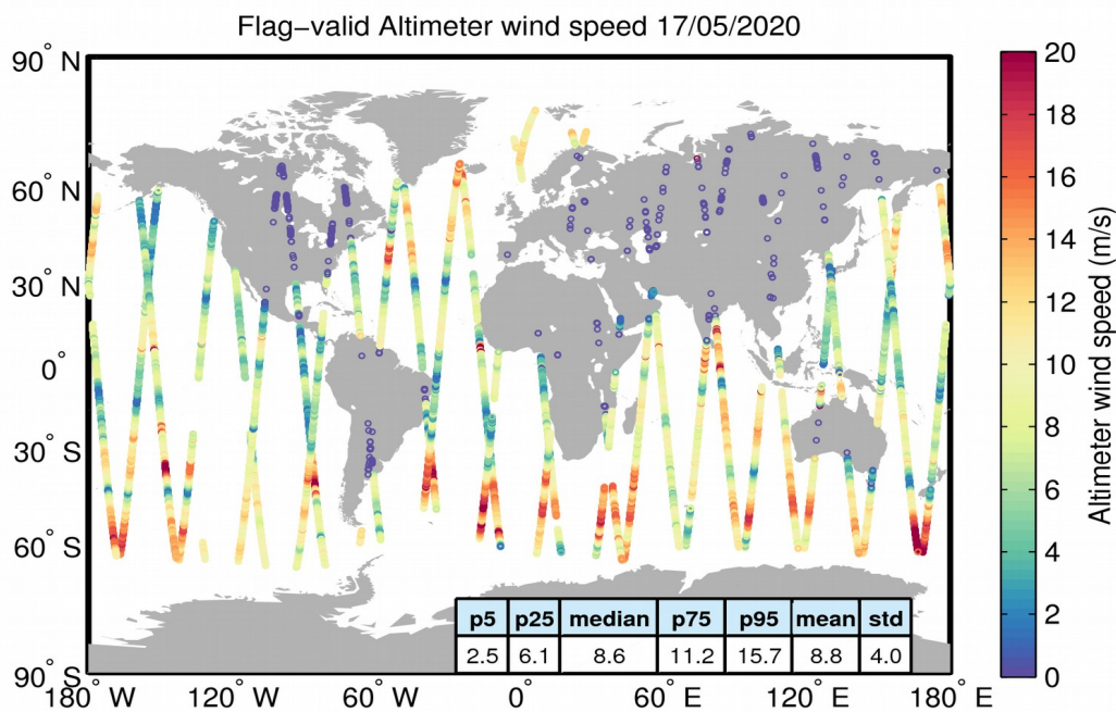
Figure 31. Geographical distribution of flag-valid wind data over oceans and lakes for 17/05/2020. The statistical values shown in the table refer to the wind in m/s and are calculated over all measurements shown in the figure.
