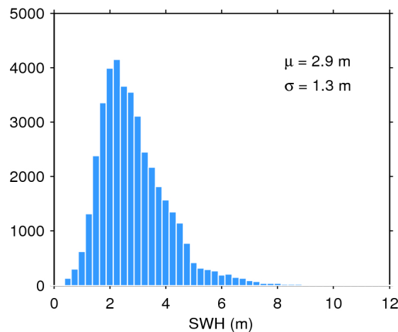
Figure 17. Histogram of flag-valid SWH over oceans and lakes for 16/05/2020. The mean ( \mu ) and standard deviation ( \sigma ) are also shown. Note that values larger than 12 m are excluded from the histogram for the sake of readability but not from the computation of \mu and \sigma .
