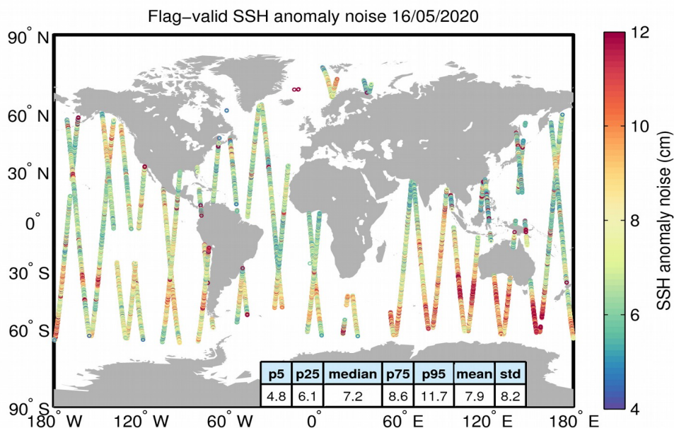
Figure 8. Geographical distribution of flag-valid 20-Hz SSH anomaly measurement noise over oceans and lakes for 16/05/2020. The statistical values shown in the table refer to the SSH anomaly noise and are calculated over all measurements shown in the figure.
