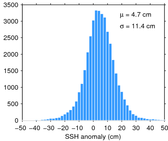
Figure 11. Histogram of science-valid SSH anomaly over oceans and lakes for 16/05/2020. The mean ( \mu ) and standard deviation ( \sigma ) are also shown. Note that values outside [-50 50] cm are excluded from the histogram for the sake of readability but not from the computation of \mu and \sigma .
