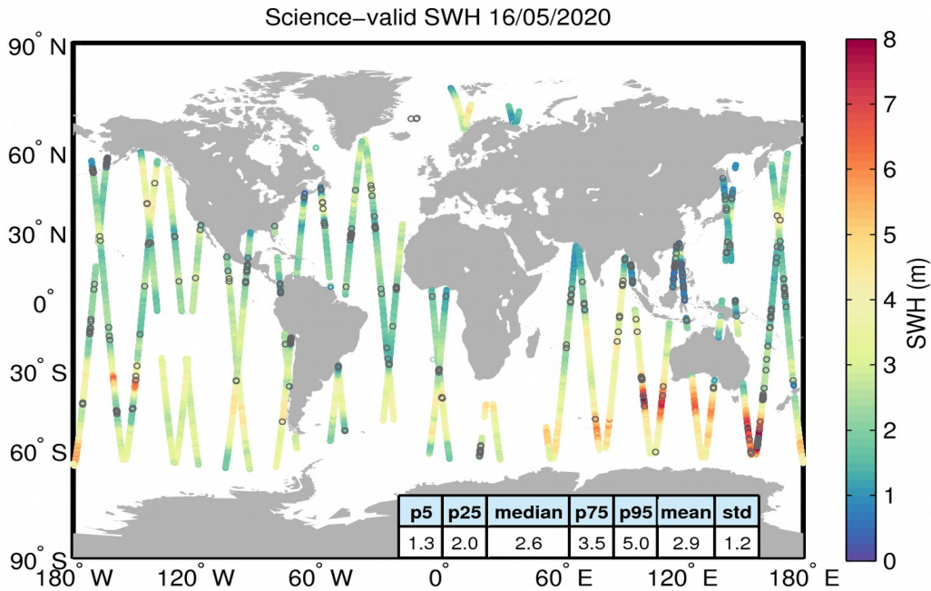
Figure 19. Geographical distribution of science-valid SWH data over oceans and lakes for 16/05/2020. The statistical values shown in the table refer to the SWH in m and are calculated over all measurements shown in the figure. Gray circles denote records that have been rejected based on the editing criteria described in Table 3.
