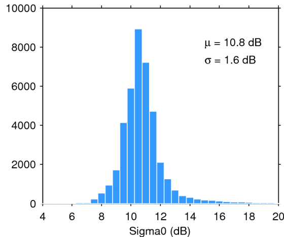
Figure 25. Histogram of flag-valid sigma0 over oceans and lakes for 16/05/2020. The mean ( \mu ) and standard deviation ( \sigma ) are also shown. Note that values outside [4 20] dB are excluded from the histogram for the sake of readability but not from the computation of \mu and \sigma .
