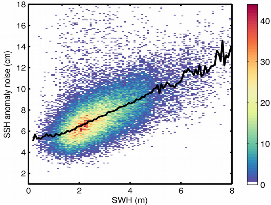
Figure 9. 2D histogram showing flag-valid SSH anomaly noise as a function of SWH for 16/05/2020. The black line denotes the median SSH anomaly noise as a function of SWH.
