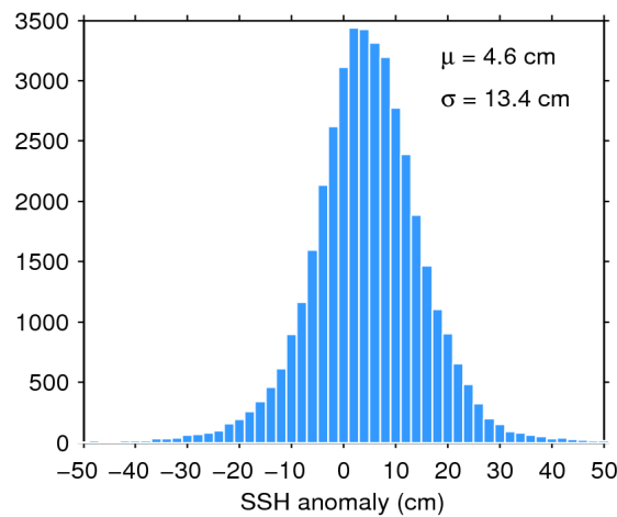
Figure 7. Histogram of flag-valid SSH anomaly over oceans and lakes for 16/05/2020. The mean ( \mu ) and standard deviation ( \sigma ) are also shown. Note that values outside [-50 50] cm are excluded from the histogram for the sake of readability but not from the computation of \mu and \sigma .
