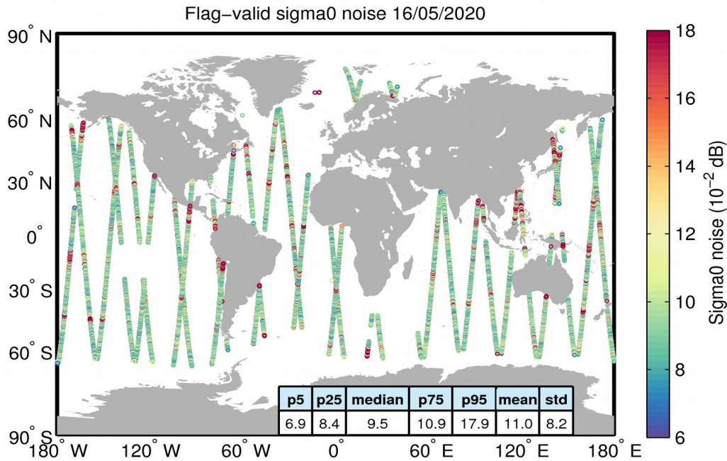
Figure 26. Geographical distribution of flag-valid 20-Hz sigma0 measurement noise over oceans and lakes for 16/05/2020. The statistical values shown in the table refer to the sigma0 noise and are calculated over all measurements shown in the figure.
