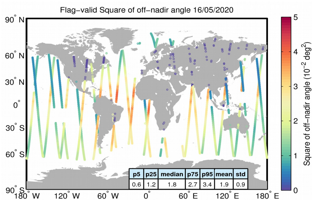
Figure 37. Geographical distribution of flag-valid mispointing data over oceans and lakes for 16/05/2020. The statistical values shown in the table refer to the mispointing in 10^{-2} \text{ deg}^2 and are calculated over all measurements shown in the figure.
