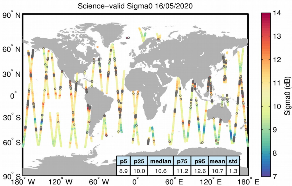
Figure 27. Geographical distribution of science-valid sigma0 data over oceans and lakes for 16/05/2020. The statistical values shown in the table refer to the sigma0 in dB and are calculated over all measurements shown in the figure. Gray circles denote records that have been rejected based on the editing criteria described in Table 4.
