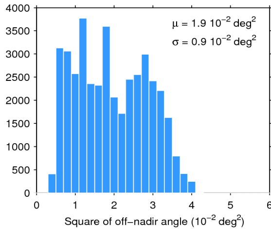
Figure 39. Histogram of flag-valid mispointing over oceans and lakes for 16/05/2020. The mean ( \mu ) and standard deviation ( \sigma ) are also shown. Note that values larger than 6 \cdot 10^{-2} \text{ deg}^2 are excluded from the histogram for the sake of readability but not from the computation of \mu and \sigma .
