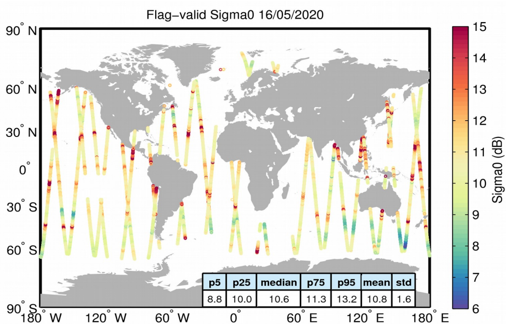
Figure 23. Geographical distribution of flag-valid sigma0 data over oceans and lakes for 16/05/2020. The statistical values shown in the table refer to the sigma0 in dB and are calculated over all measurements shown in the figure.
