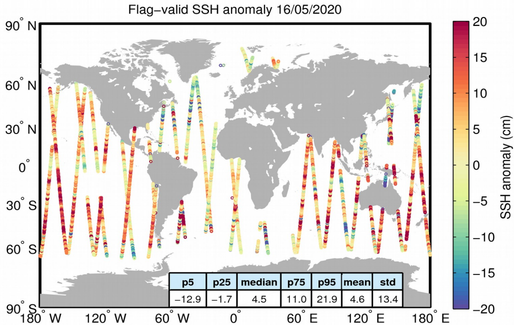
Figure 5. Geographical distribution of flag-valid 1-Hz SSH anomaly data over oceans and lakes for 16/05/2020. The statistical values shown in the table refer to the SSH anomaly in cm and are calculated over all measurements shown in the figure.
