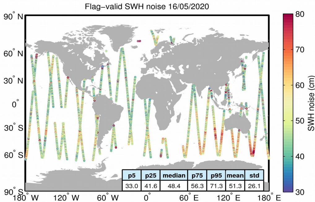
Figure 18. Geographical distribution of flag-valid 20-Hz SWH measurement noise over oceans and lakes for 16/05/2020. The statistical values shown in the figure refer to the SWH noise and are calculated over all measurements shown in the figure.
