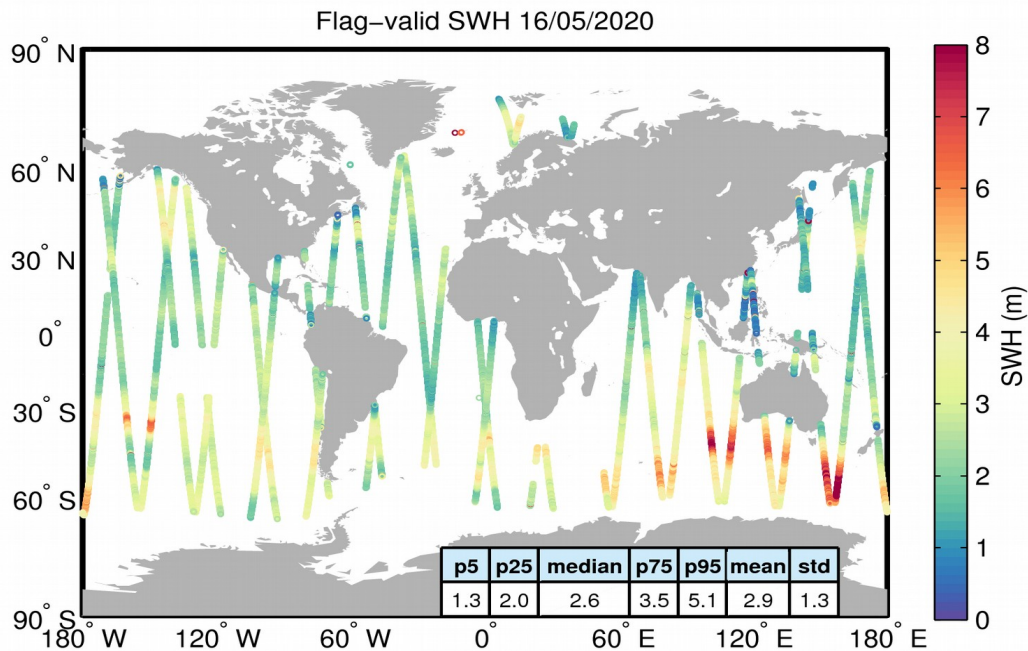
Figure 15. Geographical distribution of flag-valid SWH data over oceans and lakes for 16/05/2020. The statistical values shown in the table refer to the SWH in m and are calculated over all measurements shown in the figure.
