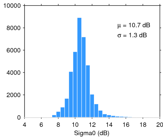
Figure 28. Histogram of science-valid sigma0 over oceans and lakes for 16/05/2020. The mean ( \mu ) and standard deviation ( \sigma ) are also shown. Note that values outside [4 20] dB are excluded from the histogram for the sake of readability but not from the computation of \mu and \sigma .
