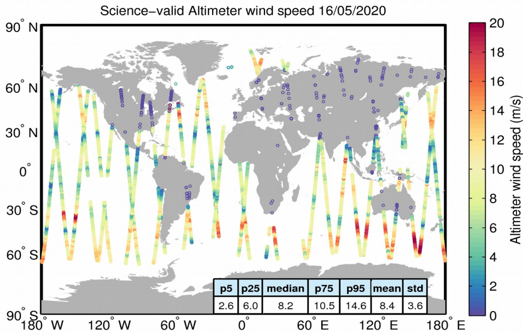
Figure 34. Geographical distribution of science-valid wind data over oceans and lakes for 16/05/2020. The statistical values shown in the table refer to the wind in m/s and are calculated over all measurements shown in the figure. Gray circles denote records that have been rejected based on the editing criteria described in Table 5.
