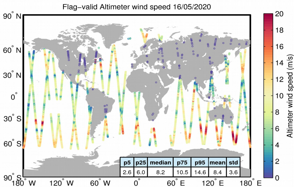
Figure 31. Geographical distribution of flag-valid wind data over oceans and lakes for 16/05/2020. The statistical values shown in the table refer to the wind in m/s and are calculated over all measurements shown in the figure.
