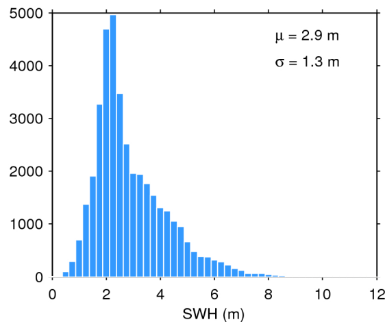
Figure 20. Histogram of science-valid SWH over oceans and lakes for 14/05/2020. The mean ( \mu ) and standard deviation ( \sigma ) are also shown. Note that values larger than 12 m are excluded from the histogram for the sake of readability but not from the computation of \mu and \sigma .
