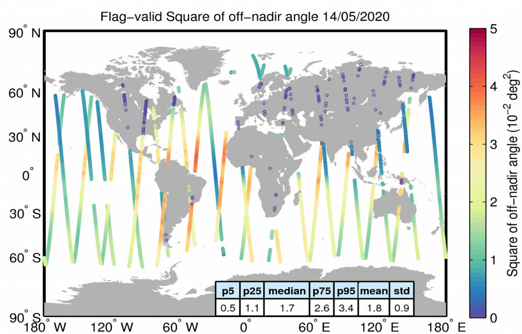
Figure 37. Geographical distribution of flag-valid mispointing data over oceans and lakes for 14/05/2020. The statistical values shown in the table refer to the mispointing in 10^{-2} deg 2 and are calculated over all measurements shown in the figure.
