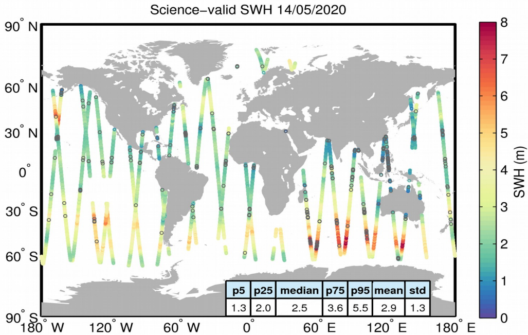
Figure 19. Geographical distribution of science-valid SWH data over oceans and lakes for 14/05/2020. The statistical values shown in the table refer to the SWH in m and are calculated over all measurements shown in the figure. Gray circles denote records that have been rejected based on the editing criteria described in Table 3.
