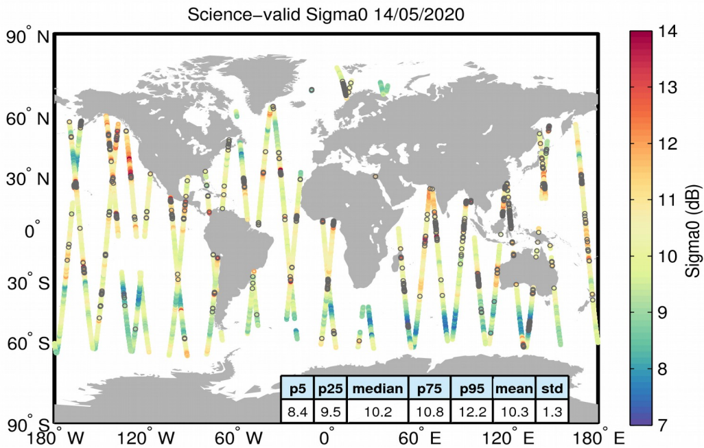
Figure 27. Geographical distribution of science-valid sigma0 data over oceans and lakes for 14/05/2020. The statistical values shown in the table refer to the sigma0 in dB and are calculated over all measurements shown in the figure. Gray circles denote records that have been rejected based on the editing criteria described in Table 4.
