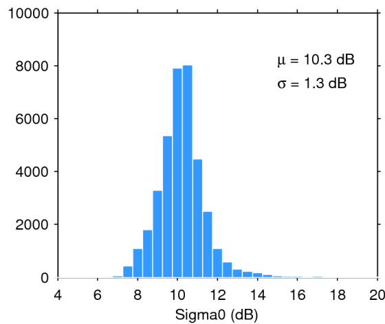
Figure 28. Histogram of science-valid sigma0 over oceans and lakes for 14/05/2020. The mean ( \mu ) and standard deviation ( \sigma ) are also shown. Note that values outside [4 20] dB are excluded from the histogram for the sake of readability but not from the computation of \mu and \sigma .
