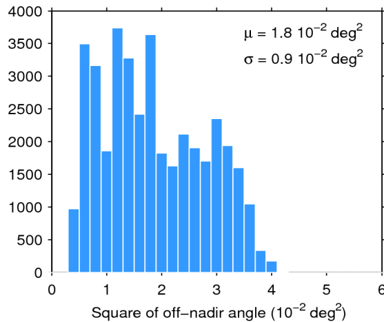
Figure 39. Histogram of flag-valid mispointing over oceans and lakes for 14/05/2020. The mean ( \mu ) and standard deviation ( \sigma ) are also shown. Note that values larger than 6 \cdot 10^{-2} \text{ deg}^2 are excluded from the histogram for the sake of readability but not from the computation of \mu and \sigma .
