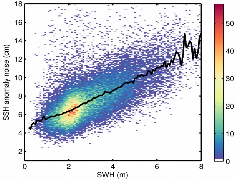
Figure 9. 2D histogram showing flag-valid SSH anomaly noise as a function of SWH for 14/05/2020. The black line denotes the median SSH anomaly noise as a function of SWH.
