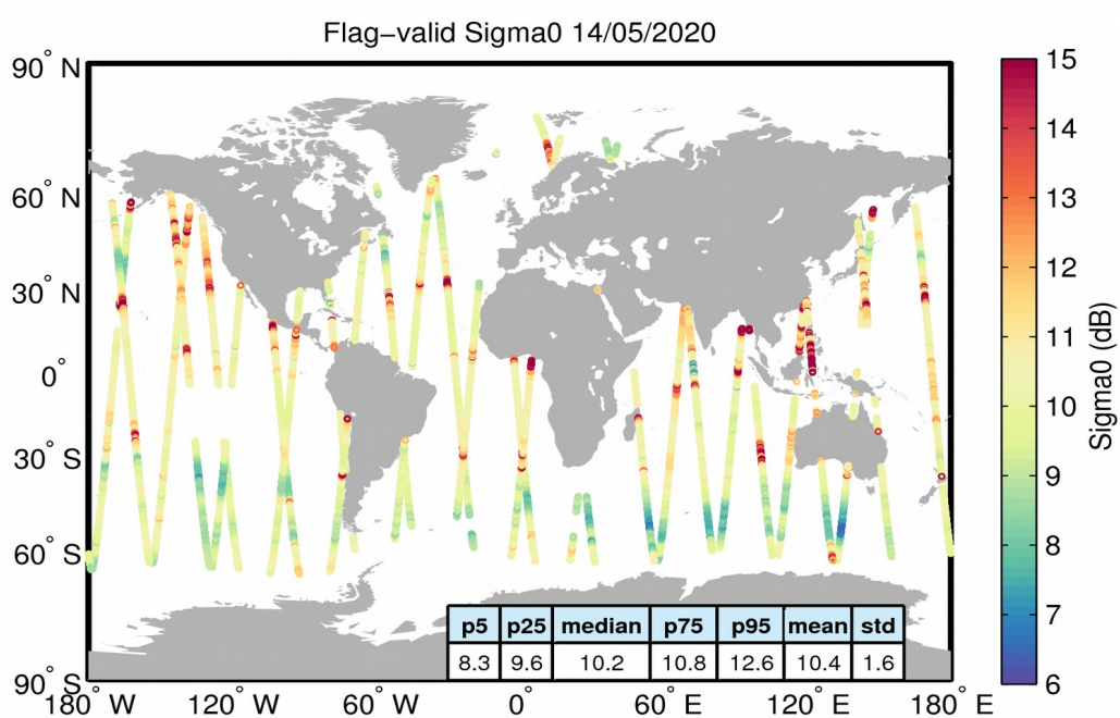
Figure 23. Geographical distribution of flag-valid sigma0 data over oceans and lakes for 14/05/2020. The statistical values shown in the table refer to the sigma0 in dB and are calculated over all measurements shown in the figure.
