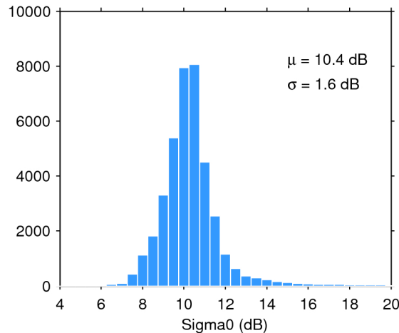
Figure 25. Histogram of flag-valid sigma0 over oceans and lakes for 14/05/2020. The mean ( \mu ) and standard deviation ( \sigma ) are also shown. Note that values outside [4 20] dB are excluded from the histogram for the sake of readability but not from the computation of \mu and \sigma .
