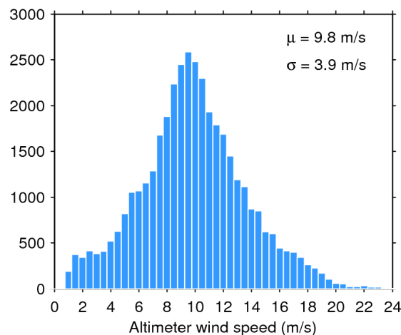
Figure 35. Histogram of science-valid wind over oceans and lakes for 14/05/2020. The mean ( \mu ) and standard deviation ( \sigma ) are also shown. Note that values larger than 24 m/s are excluded from the histogram for the sake of readability but not from the computation of \mu and \sigma .
