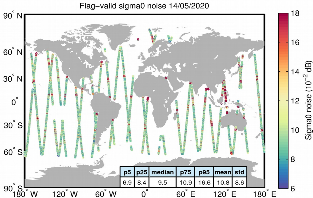
Figure 26. Geographical distribution of flag-valid 20-Hz sigma0 measurement noise over oceans and lakes for 14/05/2020. The statistical values shown in the table refer to the sigma0 noise and are calculated over all measurements shown in the figure.
