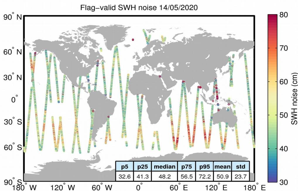
Figure 18. Geographical distribution of flag-valid 20-Hz SWH measurement noise over oceans and lakes for 14/05/2020. The statistical values shown in the table refer to the SWH noise and are calculated over all measurements shown in the figure.
