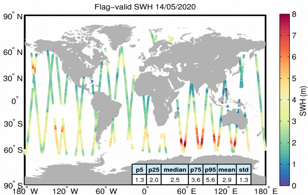
Figure 15. Geographical distribution of flag-valid SWH data over oceans and lakes for 14/05/2020. The statistical values shown in the table refer to the SWH in m and are calculated over all measurements shown in the figure.
