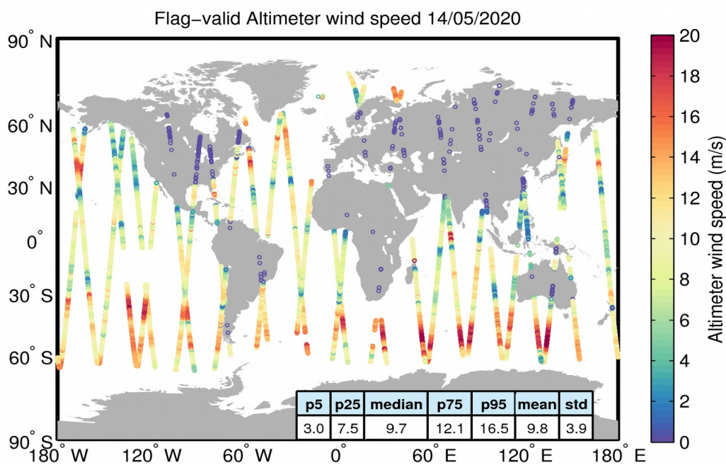
Figure 31. Geographical distribution of flag-valid wind data over oceans and lakes for 14/05/2020. The statistical values shown in the table refer to the wind in m/s and are calculated over all measurements shown in the figure.
