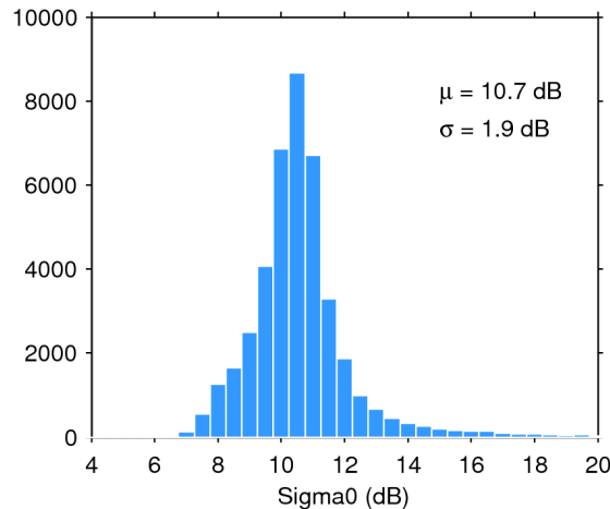
Figure 25. Histogram of flag-valid sigma0 over oceans and lakes for 13/05/2020. The mean ( \mu ) and standard deviation ( \sigma ) are also shown. Note that values outside [4 20] dB are excluded from the histogram for the sake of readability but not from the computation of \mu and \sigma .
