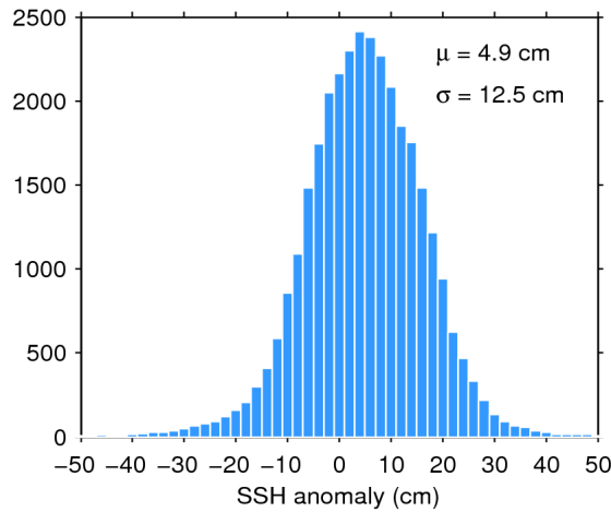
Figure 11. Histogram of science-valid SSH anomaly over oceans and lakes for 13/05/2020. The mean ( \mu ) and standard deviation ( \sigma ) are also shown. Note that values outside [-50 50] cm are excluded from the histogram for the sake of readability but not from the computation of \mu and \sigma .
