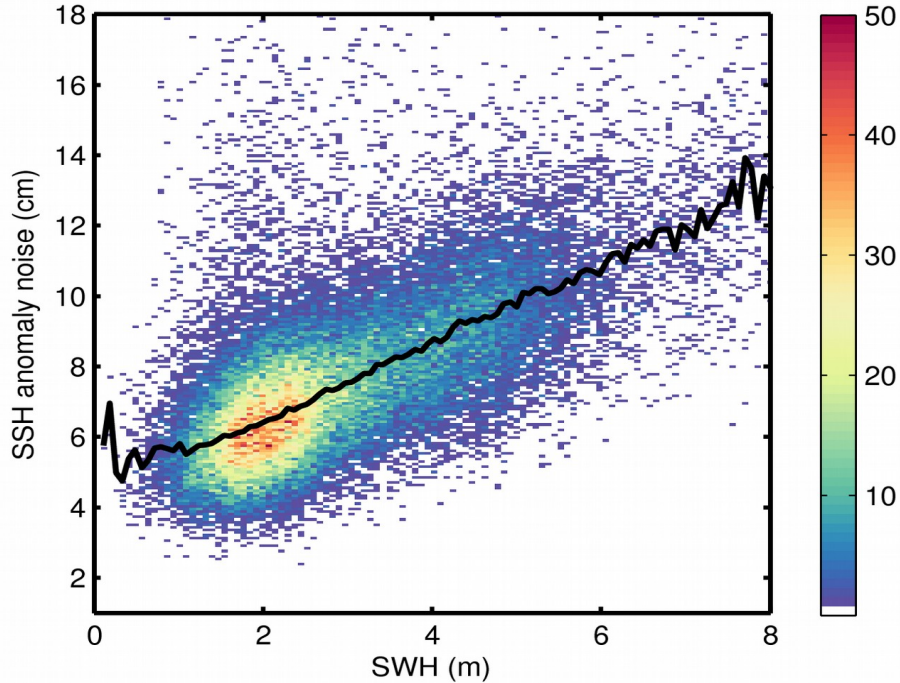
Figure 9. 2D histogram showing flag-valid SSH anomaly noise as a function of SWH for 13/05/2020. The black line denotes the median SSH anomaly noise as a function of SWH.
