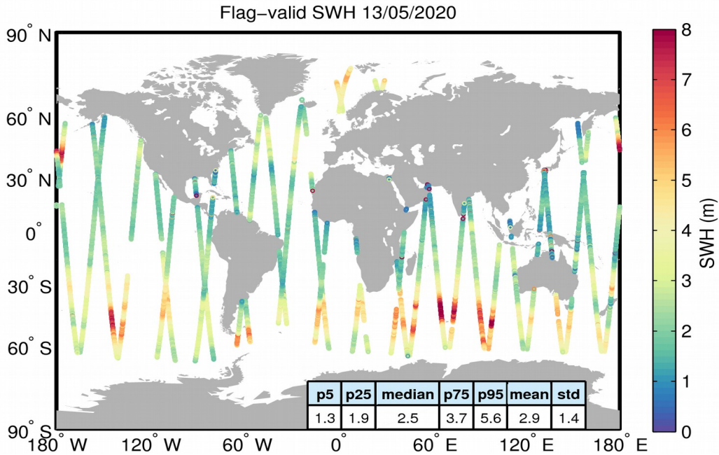
Figure 15. Geographical distribution of flag-valid SWH data over oceans and lakes for 13/05/2020. The statistical values shown in the table refer to the SWH in m and are calculated over all measurements shown in the figure.
