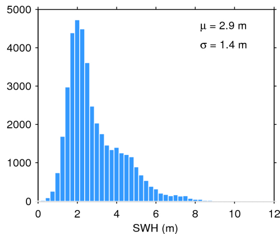
Figure 20. Histogram of science-valid SWH over oceans and lakes for 13/05/2020. The mean ( \mu ) and standard deviation ( \sigma ) are also shown. Note that values larger than 12 m are excluded from the histogram for the sake of readability but not from the computation of \mu and \sigma .
