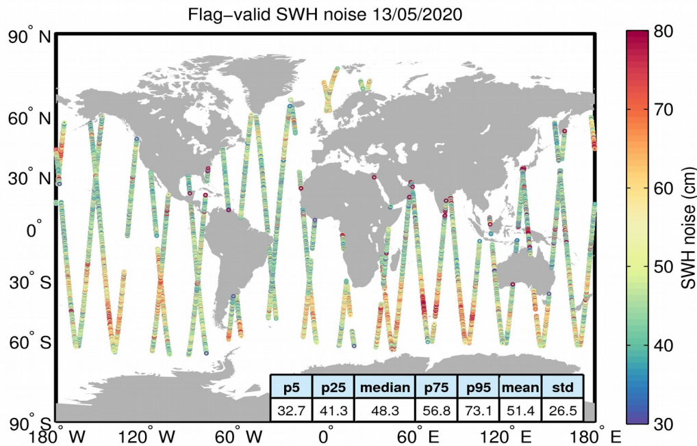
Figure 18. Geographical distribution of flag-valid 20-Hz SWH measurement noise over oceans and lakes for 13/05/2020. The statistical values shown in the figure refer to the SWH noise and are calculated over all measurements shown in the figure.
