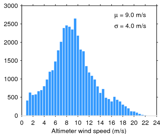
Figure 35. Histogram of science-valid wind over oceans and lakes for 13/05/2020. The mean ( \mu ) and standard deviation ( \sigma ) are also shown. Note that values larger than 24 m/s are excluded from the histogram for the sake of readability but not from the computation of \mu and \sigma .
