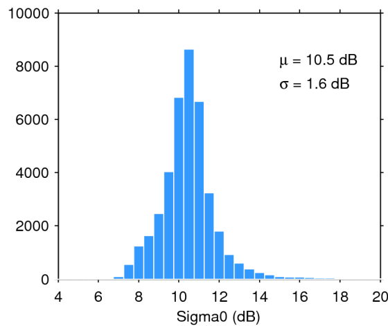
Figure 28. Histogram of science-valid sigma0 over oceans and lakes for 13/05/2020. The mean ( \mu ) and standard deviation ( \sigma ) are also shown. Note that values outside [4 20] dB are excluded from the histogram for the sake of readability but not from the computation of \mu and \sigma .
