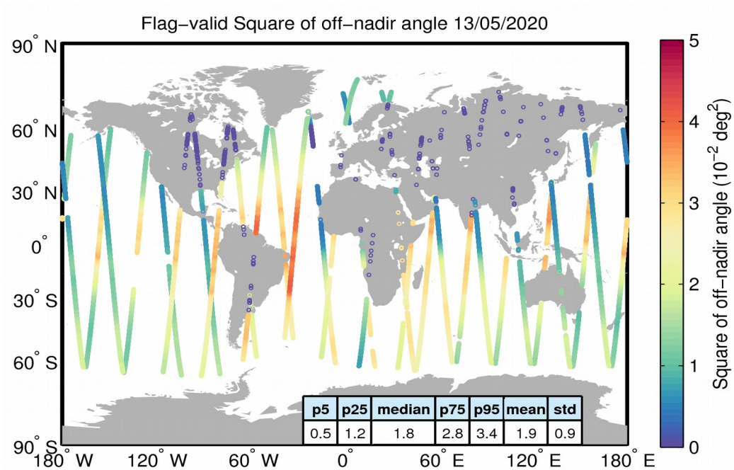
Figure 37. Geographical distribution of flag-valid mispointing data over oceans and lakes for 13/05/2020. The statistical values shown in the table refer to the mispointing in 10^{-2} \text{ deg}^2 and are calculated over all measurements shown in the figure.
