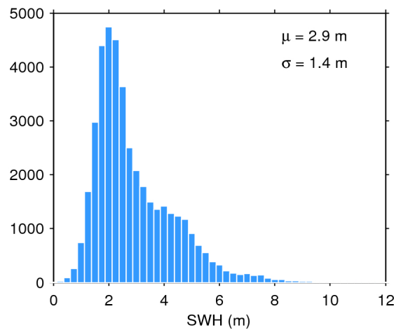
Figure 17. Histogram of flag-valid SWH over oceans and lakes for 13/05/2020. The mean ( \mu ) and standard deviation ( \sigma ) are also shown. Note that values larger than 12 m are excluded from the histogram for the sake of readability but not from the computation of \mu and \sigma .
