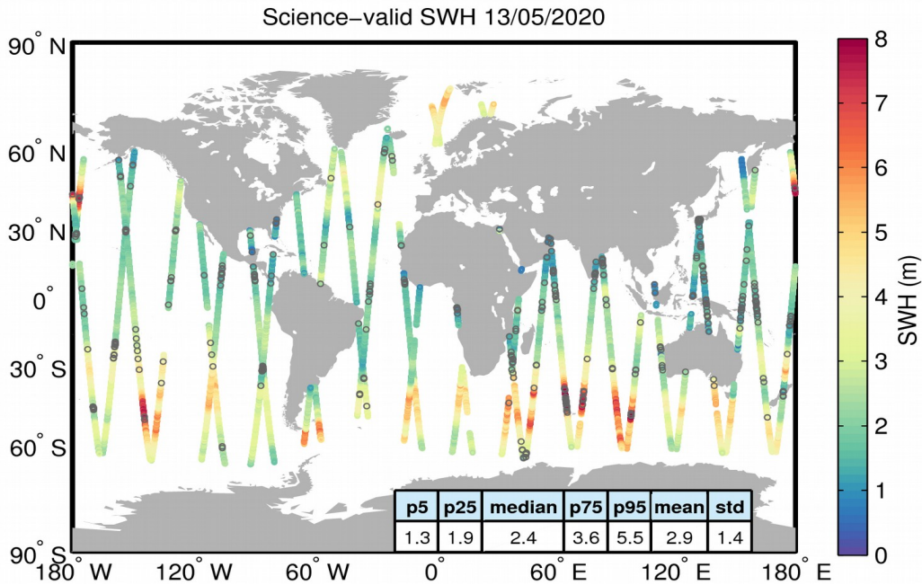
Figure 19. Geographical distribution of science-valid SWH data over oceans and lakes for 13/05/2020. The statistical values shown in the table refer to the SWH in m and are calculated over all measurements shown in the figure. Gray circles denote records that have been rejected based on the editing criteria described in Table 3.
