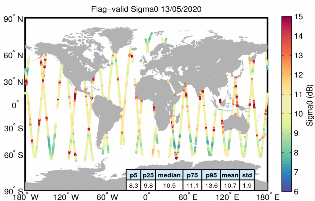
Figure 23. Geographical distribution of flag-valid sigma0 data over oceans and lakes for 13/05/2020. The statistical values shown in the table refer to the sigma0 in dB and are calculated over all measurements shown in the figure.
