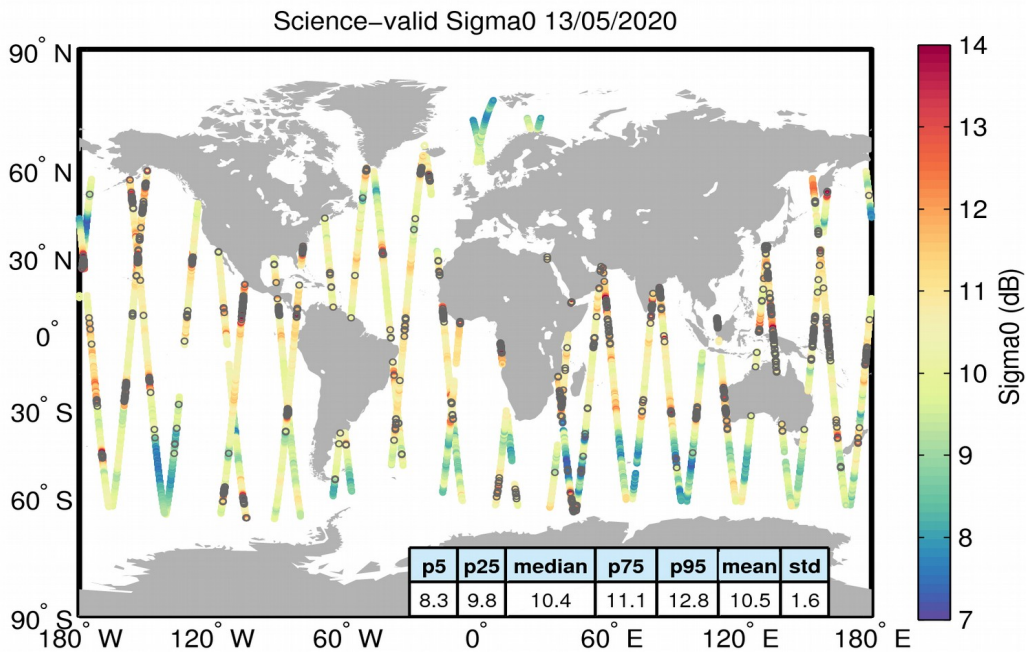
Figure 27. Geographical distribution of science-valid sigma0 data over oceans and lakes for 13/05/2020. The statistical values shown in the table refer to the sigma0 in dB and are calculated over all measurements shown in the figure. Gray circles denote records that have been rejected based on the editing criteria described in Table 4.
