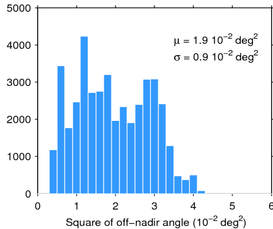
Figure 39. Histogram of flag-valid mispointing over oceans and lakes for 13/05/2020. The mean ( \mu ) and standard deviation ( \sigma ) are also shown. Note that values larger than 6 \cdot 10^{-2} \text{ deg}^2 are excluded from the histogram for the sake of readability but not from the computation of \mu and \sigma .
