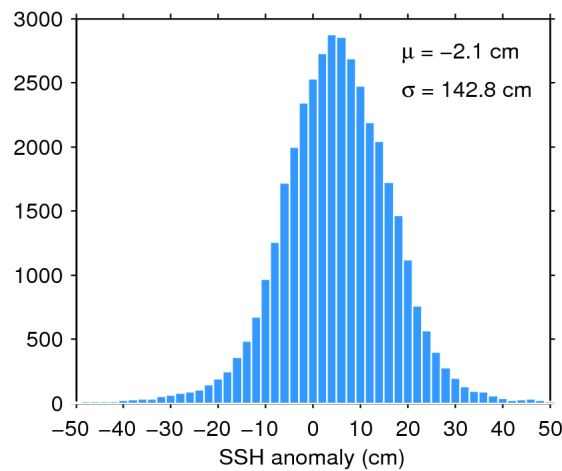
Figure 7. Histogram of flag-valid SSH anomaly over oceans and lakes for 13/05/2020. The mean ( \mu ) and standard deviation ( \sigma ) are also shown. Note that values outside [-50 50] cm are excluded from the histogram for the sake of readability but not from the computation of \mu and \sigma .
