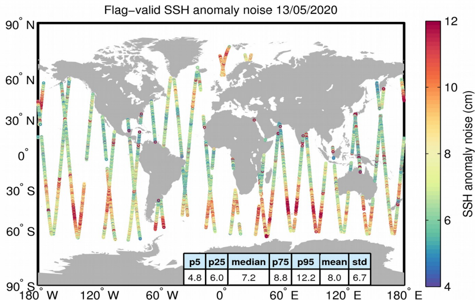
Figure 8. Geographical distribution of flag-valid 20-Hz SSH anomaly measurement noise over oceans and lakes for 13/05/2020. The statistical values shown in the table refer to the SSH anomaly noise and are calculated over all measurements shown in the figure.
