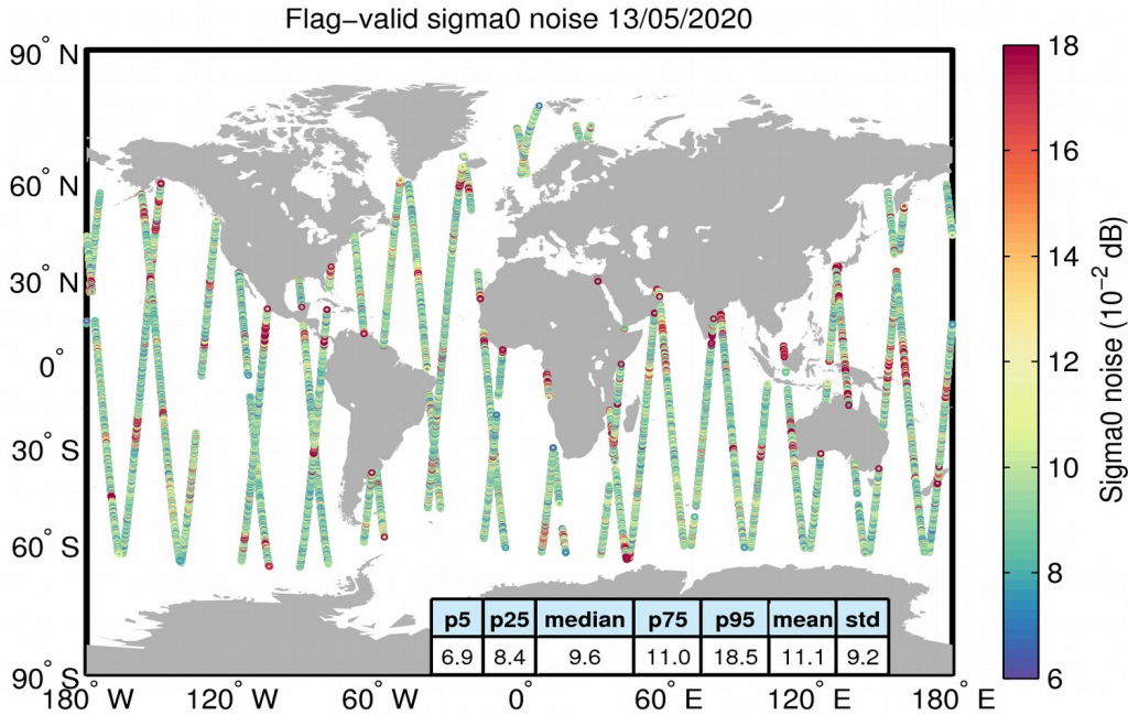
Figure 26. Geographical distribution of flag-valid 20-Hz sigma0 measurement noise over oceans and lakes for 13/05/2020. The statistical values shown in the table refer to the sigma0 noise and are calculated over all measurements shown in the figure.
