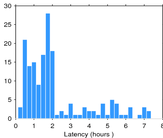
Figure 2. Histogram of the data latency for 13/05/2020. The y-axis denotes the number of files that are made available with a delay of x-hours with respect to the mean time of the records stored in the file.
