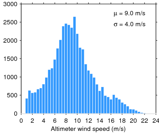
Figure 33. Histogram of flag-valid wind over oceans and lakes for 13/05/2020. The mean ( \mu ) and standard deviation ( \sigma ) are also shown. Note that values larger than 24 m/s are excluded from the histogram for the sake of readability but not from the computation of \mu and \sigma .
