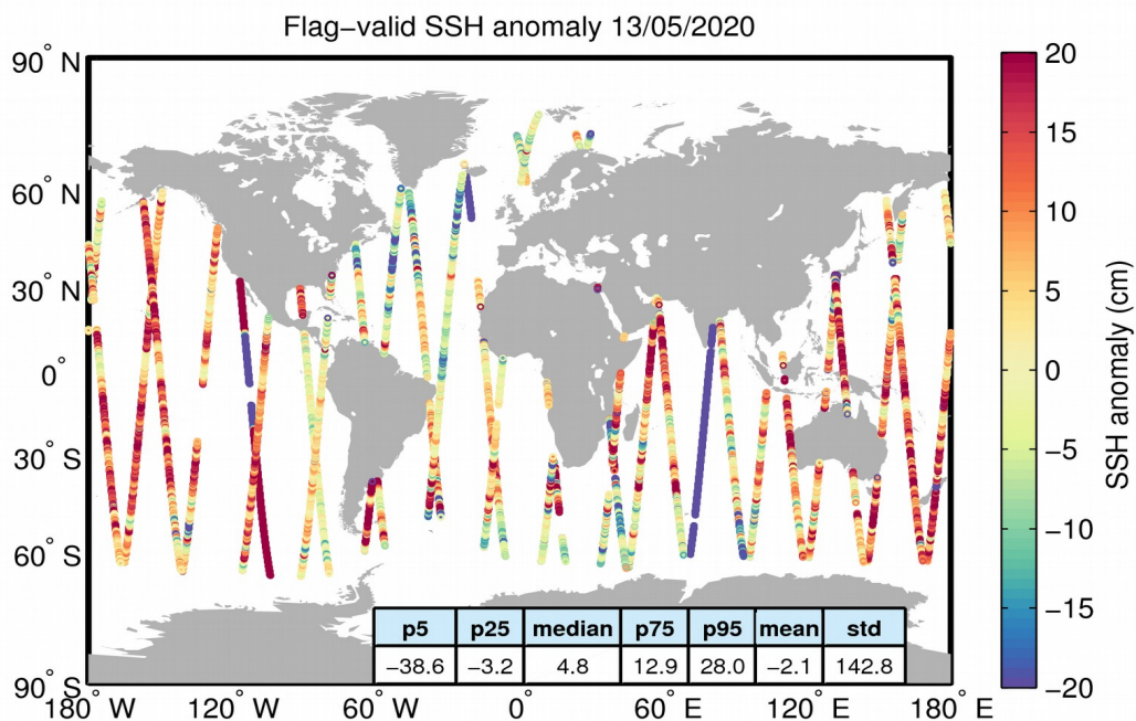
Figure 5. Geographical distribution of flag-valid 1-Hz SSH anomaly data over oceans and lakes for 13/05/2020. The statistical values shown in the table refer to the SSH anomaly in cm and are calculated over all measurements shown in the figure.
