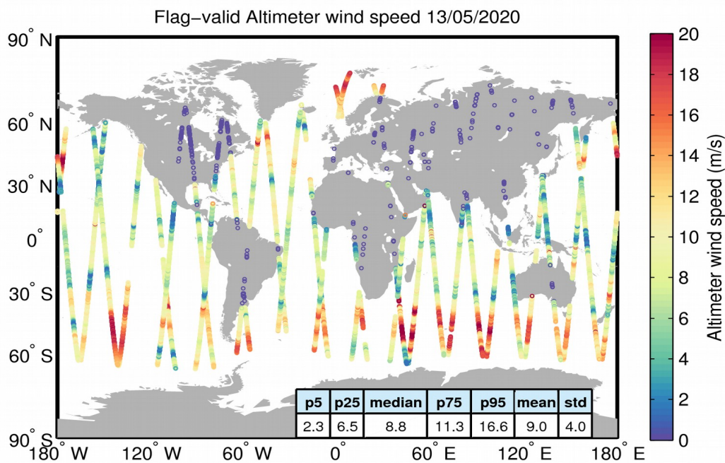
Figure 31. Geographical distribution of flag-valid wind data over oceans and lakes for 13/05/2020. The statistical values shown in the table refer to the wind in m/s and are calculated over all measurements shown in the figure.
