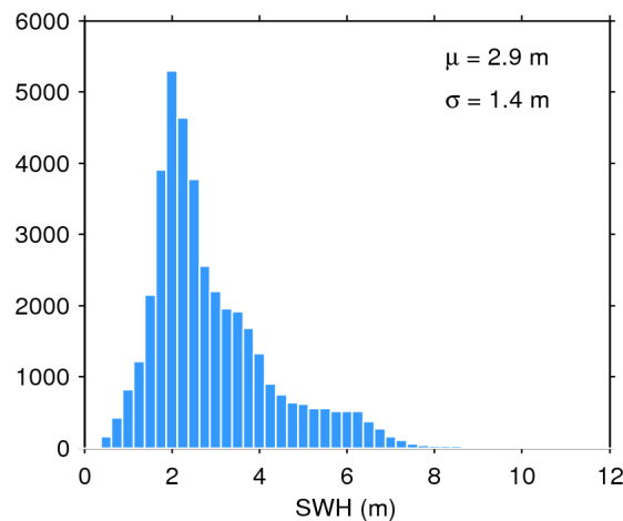
Figure 20. Histogram of science-valid SWH over oceans and lakes for 12/05/2020. The mean ( \mu ) and standard deviation ( \sigma ) are also shown. Note that values larger than 12 m are excluded from the histogram for the sake of readability but not from the computation of \mu and \sigma .
