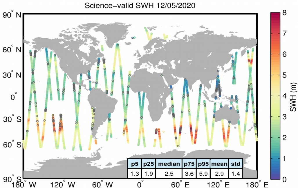
Figure 19. Geographical distribution of science-valid SWH data over oceans and lakes for 12/05/2020. The statistical values shown in the table refer to the SWH in m and are calculated over all measurements shown in the figure. Gray circles denote records that have been rejected based on the editing criteria described in Table 3.
