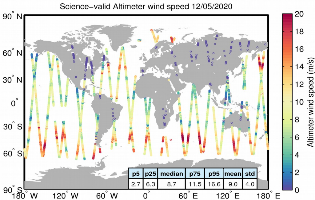
Figure 34. Geographical distribution of science-valid wind data over oceans and lakes for 12/05/2020. The statistical values shown in the table refer to the wind in m/s and are calculated over all measurements shown in the figure. Gray circles denote records that have been rejected based on the editing criteria described in Table 5.
