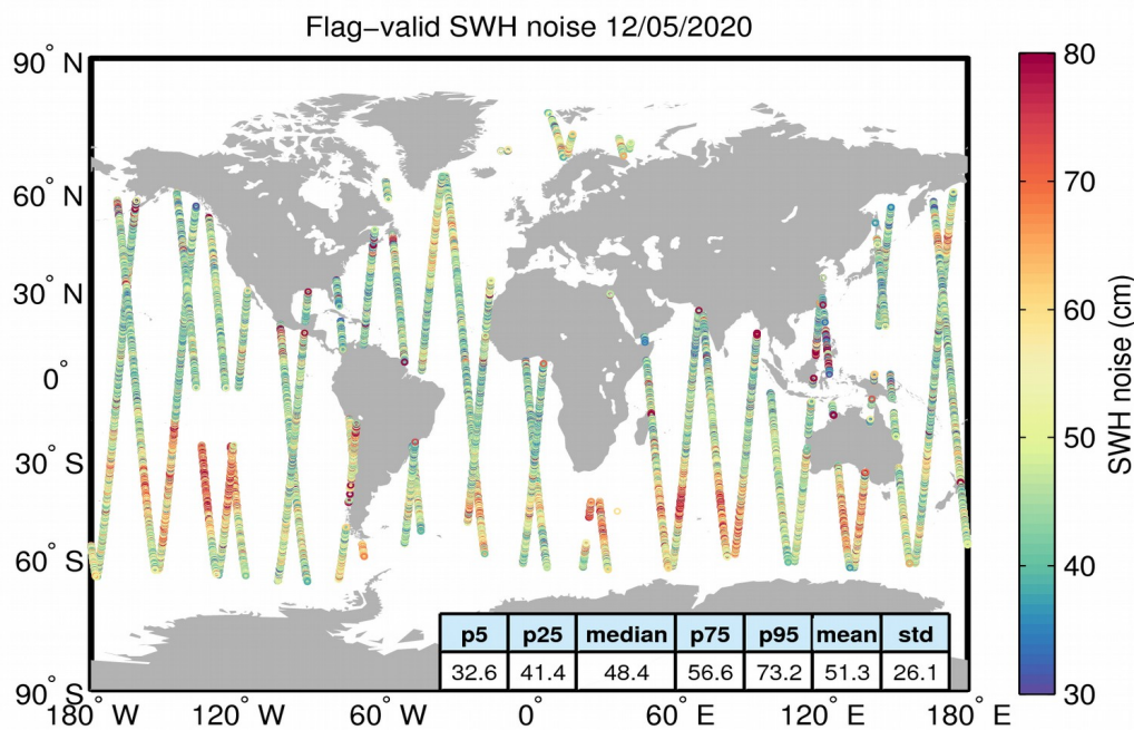
Figure 18. Geographical distribution of flag-valid 20-Hz SWH measurement noise over oceans and lakes for 12/05/2020. The statistical values shown in the table refer to the SWH noise and are calculated over all measurements shown in the figure.
