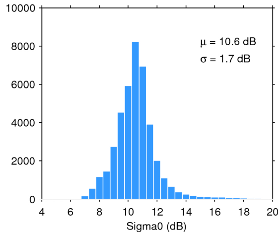
Figure 25. Histogram of flag-valid sigma0 over oceans and lakes for 12/05/2020. The mean ( \mu ) and standard deviation ( \sigma ) are also shown. Note that values outside [4 20] dB are excluded from the histogram for the sake of readability but not from the computation of \mu and \sigma .
