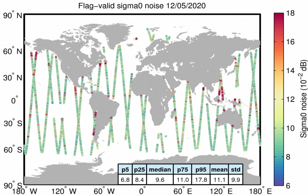
Figure 26. Geographical distribution of flag-valid 20-Hz sigma0 measurement noise over oceans and lakes for 12/05/2020. The statistical values shown in the table refer to the sigma0 noise and are calculated over all measurements shown in the figure.
