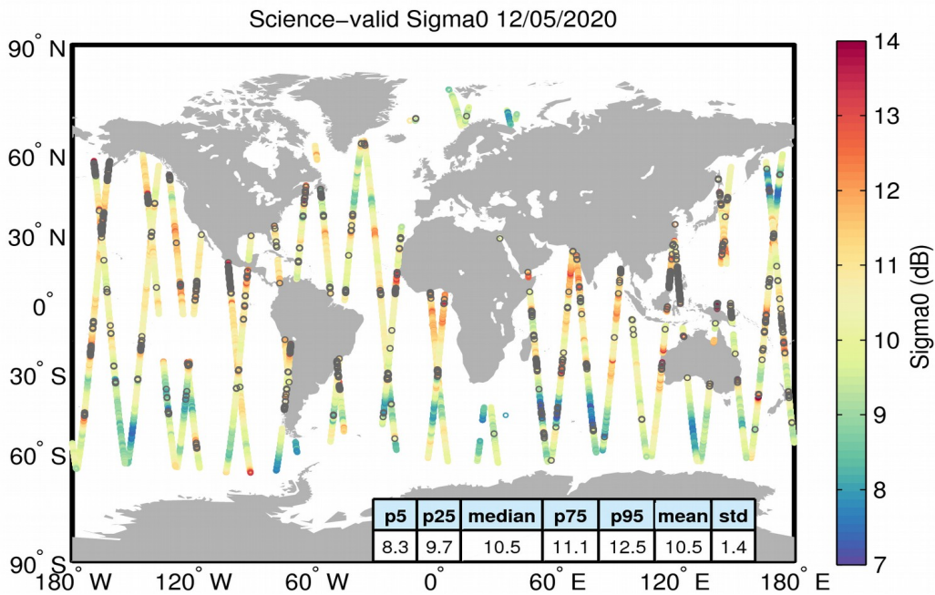
Figure 27. Geographical distribution of science-valid sigma0 data over oceans and lakes for 12/05/2020. The statistical values shown in the table refer to the sigma0 in dB and are calculated over all measurements shown in the figure. Gray circles denote records that have been rejected based on the editing criteria described in Table 4.
