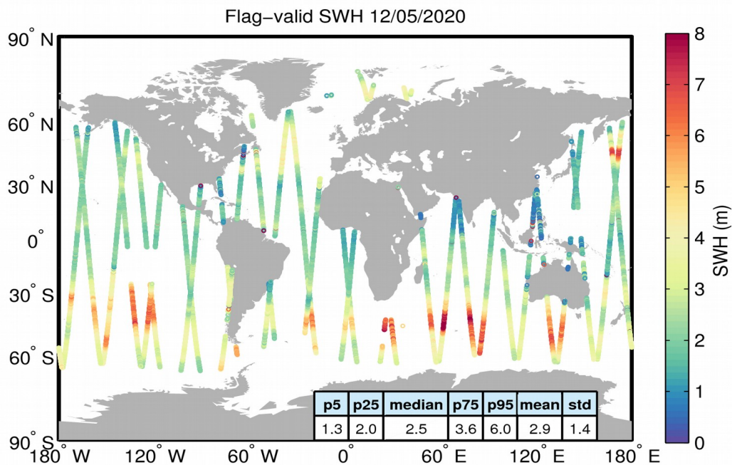
Figure 15. Geographical distribution of flag-valid SWH data over oceans and lakes for 12/05/2020. The statistical values shown in the table refer to the SWH in m and are calculated over all measurements shown in the figure.
