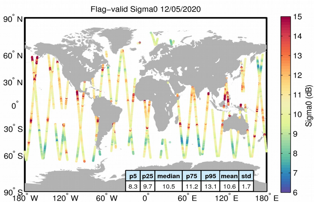
Figure 23. Geographical distribution of flag-valid sigma0 data over oceans and lakes for 12/05/2020. The statistical values shown in the table refer to the sigma0 in dB and are calculated over all measurements shown in the figure.
