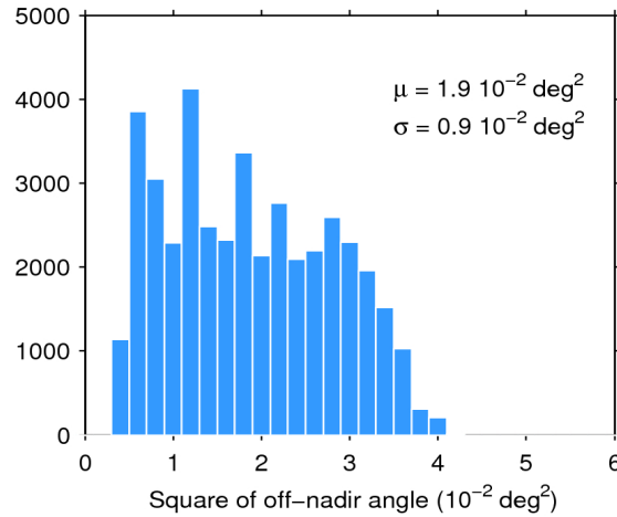
Figure 39. Histogram of flag-valid mispointing over oceans and lakes for 12/05/2020. The mean ( \mu ) and standard deviation ( \sigma ) are also shown. Note that values larger than 6 \cdot 10^{-2} \text{ deg}^2 are excluded from the histogram for the sake of readability but not from the computation of \mu and \sigma .
