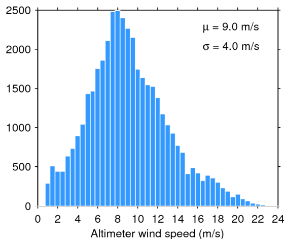
Figure 35. Histogram of science-valid wind over oceans and lakes for 12/05/2020. The mean ( \mu ) and standard deviation ( \sigma ) are also shown. Note that values larger than 24 m/s are excluded from the histogram for the sake of readability but not from the computation of \mu and \sigma .
