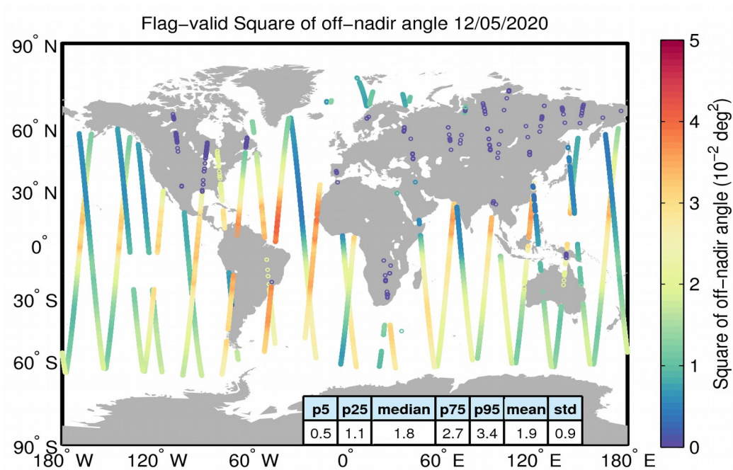
Figure 37. Geographical distribution of flag-valid mispointing data over oceans and lakes for 12/05/2020. The statistical values shown in the table refer to the mispointing in 10^{-2} \text{ deg}^2 and are calculated over all measurements shown in the figure.
