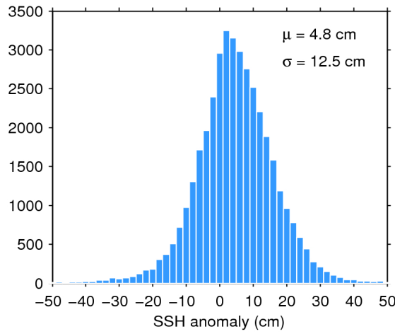
Figure 11. Histogram of science-valid SSH anomaly over oceans and lakes for 12/05/2020. The mean ( \mu ) and standard deviation ( \sigma ) are also shown. Note that values outside [-50 50] cm are excluded from the histogram for the sake of readability but not from the computation of \mu and \sigma .
