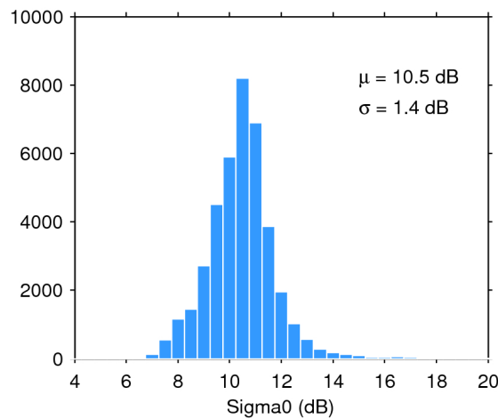
Figure 28. Histogram of science-valid sigma0 over oceans and lakes for 12/05/2020. The mean ( \mu ) and standard deviation ( \sigma ) are also shown. Note that values outside [4 20] dB are excluded from the histogram for the sake of readability but not from the computation of \mu and \sigma .
