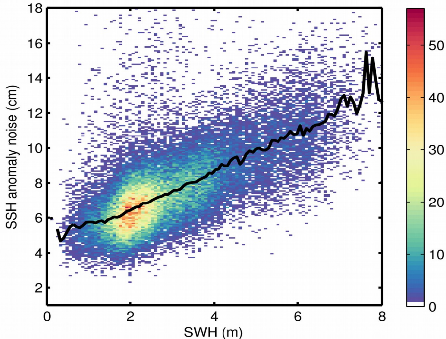
Figure 9. 2D histogram showing flag-valid SSH anomaly noise as a function of SWH for 12/05/2020. The black line denotes the median SSH anomaly noise as a function of SWH.
