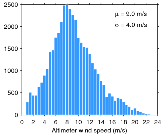
Figure 33. Histogram of flag-valid wind over oceans and lakes for 12/05/2020. The mean ( \mu ) and standard deviation ( \sigma ) are also shown. Note that values larger than 24 m/s are excluded from the histogram for the sake of readability but not from the computation of \mu and \sigma .
