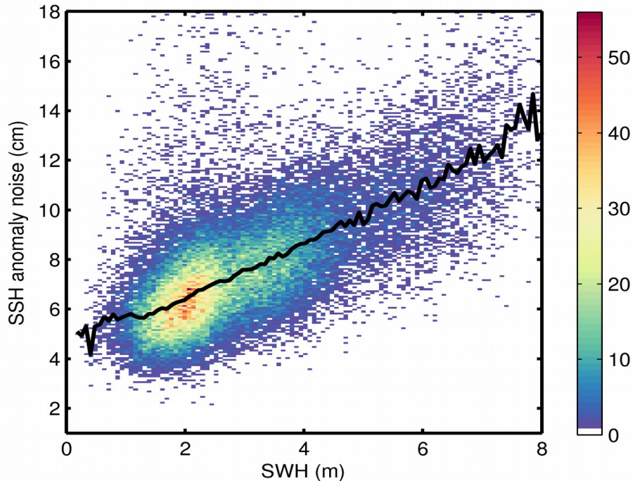
Figure 9. 2D histogram showing flag-valid SSH anomaly noise as a function of SWH for 11/05/2020. The black line denotes the median SSH anomaly noise as a function of SWH.
