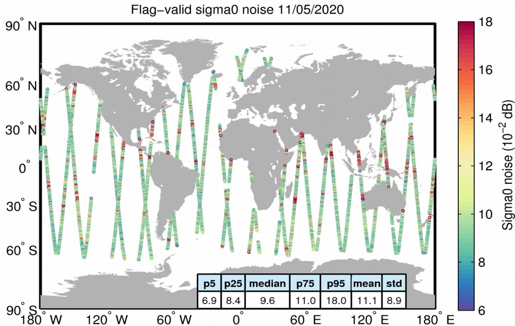
Figure 26. Geographical distribution of flag-valid 20-Hz sigma0 measurement noise over oceans and lakes for 11/05/2020. The statistical values shown in the table refer to the sigma0 noise and are calculated over all measurements shown in the figure.
