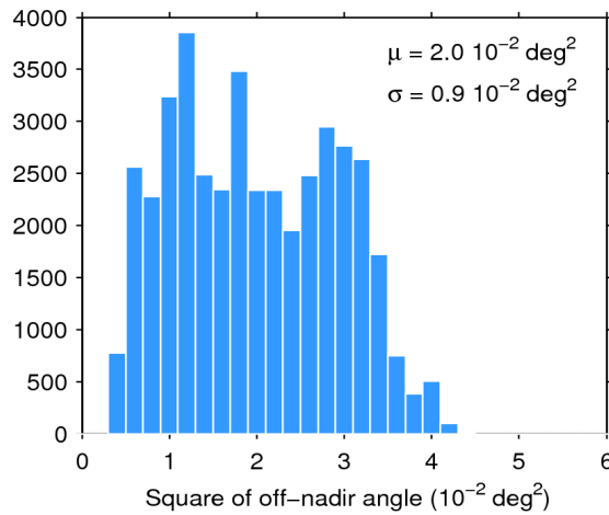
Figure 39. Histogram of flag-valid mispointing over oceans and lakes for 11/05/2020. The mean ( \mu ) and standard deviation ( \sigma ) are also shown. Note that values larger than 6 \cdot 10^{-2} \text{ deg}^2 are excluded from the histogram for the sake of readability but not from the computation of \mu and \sigma .
