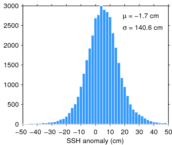
Figure 7. Histogram of flag-valid SSH anomaly over oceans and lakes for 11/05/2020. The mean ( \mu ) and standard deviation ( \sigma ) are also shown. Note that values outside [-50\ 50] cm are excluded from the histogram for the sake of readability but not from the computation of \mu and \sigma .
