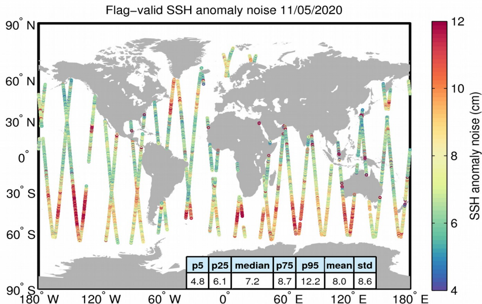
Figure 8. Geographical distribution of flag-valid 20-Hz SSH anomaly measurement noise over oceans and lakes for 11/05/2020. The statistical values shown in the table refer to the SSH anomaly noise and are calculated over all measurements shown in the figure.
