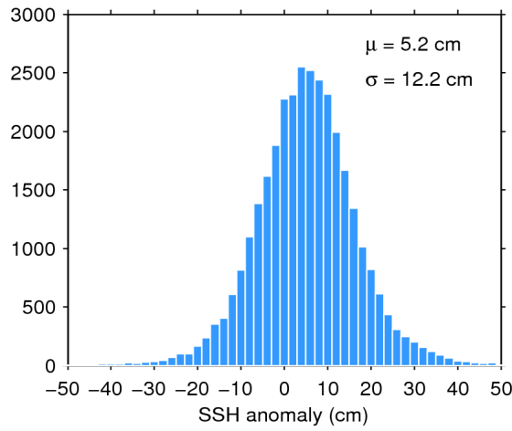
Figure 11. Histogram of science-valid SSH anomaly over oceans and lakes for 11/05/2020. The mean ( \mu ) and standard deviation ( \sigma ) are also shown. Note that values outside [-50 50] cm are excluded from the histogram for the sake of readability but not from the computation of \mu and \sigma .
