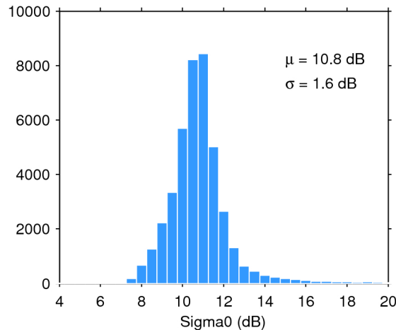
Figure 25. Histogram of flag-valid sigma0 over oceans and lakes for 11/05/2020. The mean ( \mu ) and standard deviation ( \sigma ) are also shown. Note that values outside [4 20] dB are excluded from the histogram for the sake of readability but not from the computation of \mu and \sigma .
