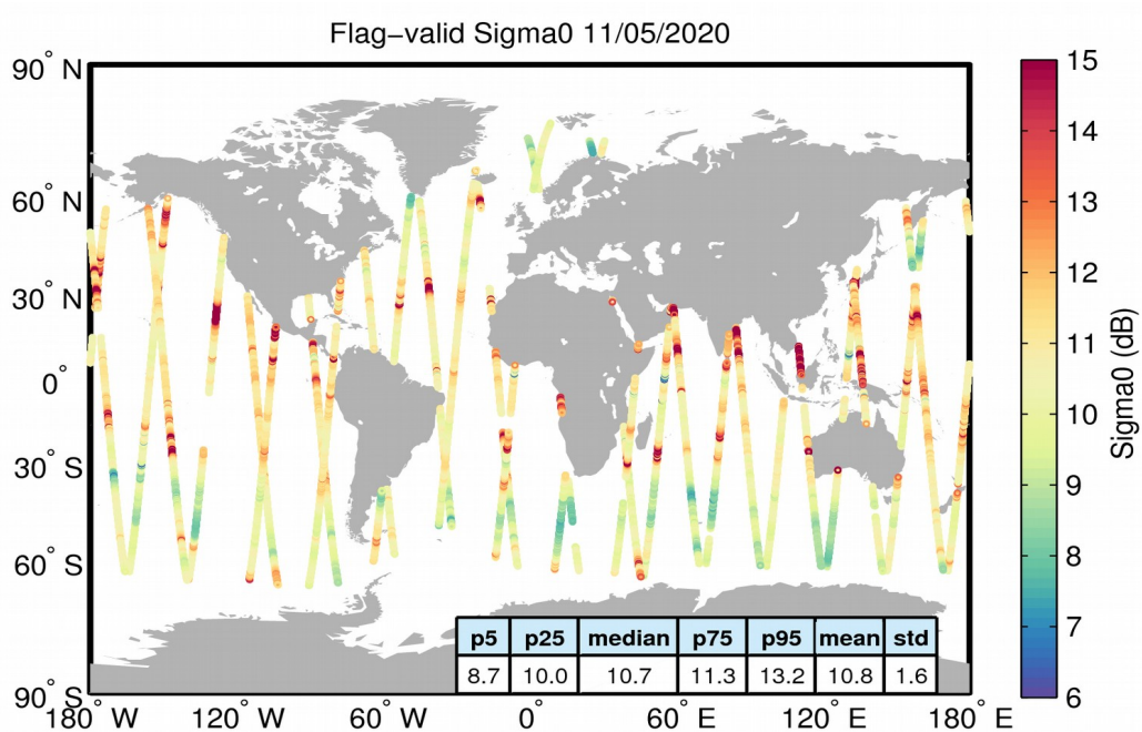
Figure 23. Geographical distribution of flag-valid sigma0 data over oceans and lakes for 11/05/2020. The statistical values shown in the table refer to the sigma0 in dB and are calculated over all measurements shown in the figure.
