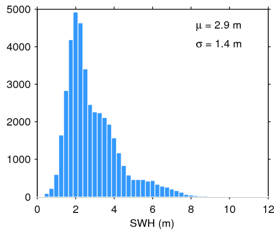
Figure 17. Histogram of flag-valid SWH over oceans and lakes for 11/05/2020. The mean ( \mu ) and standard deviation ( \sigma ) are also shown. Note that values larger than 12 m are excluded from the histogram for the sake of readability but not from the computation of \mu and \sigma .
