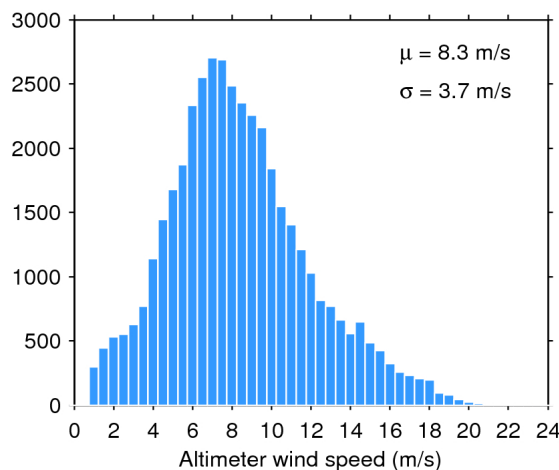
Figure 35. Histogram of science-valid wind over oceans and lakes for 11/05/2020. The mean ( \mu ) and standard deviation ( \sigma ) are also shown. Note that values larger than 24 m/s are excluded from the histogram for the sake of readability but not from the computation of \mu and \sigma .
