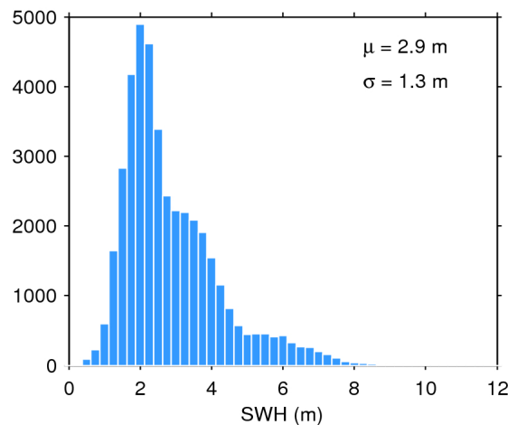
Figure 20. Histogram of science-valid SWH over oceans and lakes for 11/05/2020. The mean ( \mu ) and standard deviation ( \sigma ) are also shown. Note that values larger than 12 m are excluded from the histogram for the sake of readability but not from the computation of \mu and \sigma .
