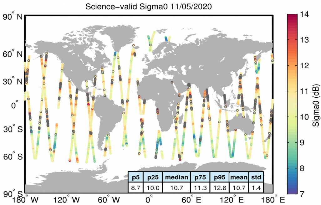
Figure 27. Geographical distribution of science-valid sigma0 data over oceans and lakes for 11/05/2020. The statistical values shown in the table refer to the sigma0 in dB and are calculated over all measurements shown in the figure. Gray circles denote records that have been rejected based on the editing criteria described in Table 4.
