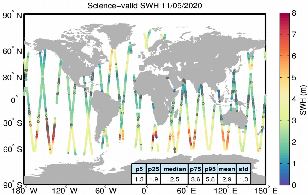
Figure 19. Geographical distribution of science-valid SWH data over oceans and lakes for 11/05/2020. The statistical values shown in the table refer to the SWH in m and are calculated over all measurements shown in the figure. Gray circles denote records that have been rejected based on the editing criteria described in Table 3.
