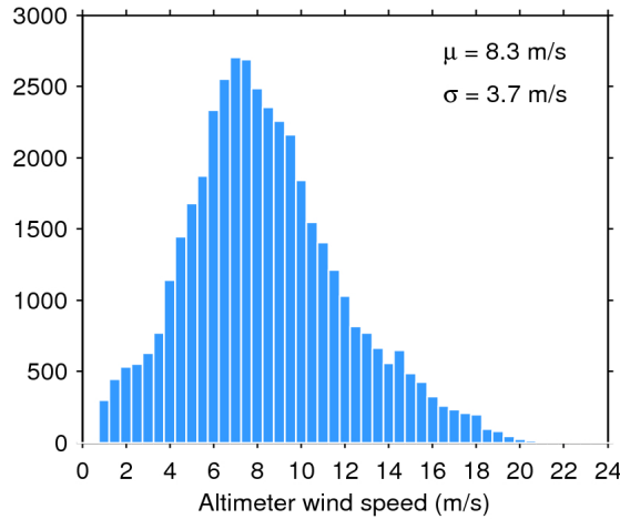
Figure 33. Histogram of flag-valid wind over oceans and lakes for 11/05/2020. The mean ( \mu ) and standard deviation ( \sigma ) are also shown. Note that values larger than 24 m/s are excluded from the histogram for the sake of readability but not from the computation of \mu and \sigma .
