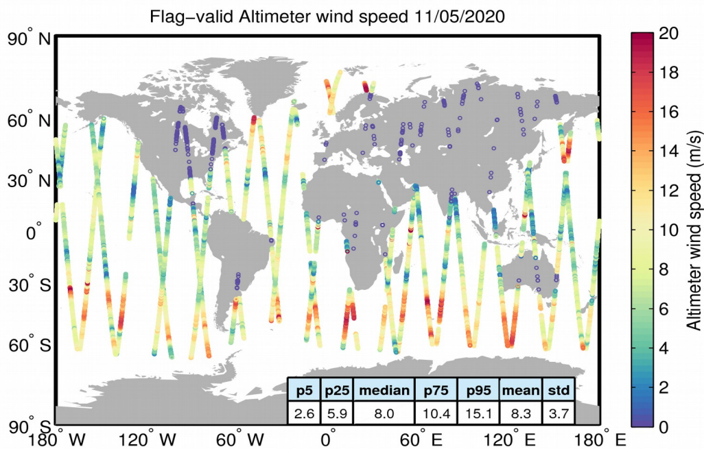
Figure 31. Geographical distribution of flag-valid wind data over oceans and lakes for 11/05/2020. The statistical values shown in the table refer to the wind in m/s and are calculated over all measurements shown in the figure.
