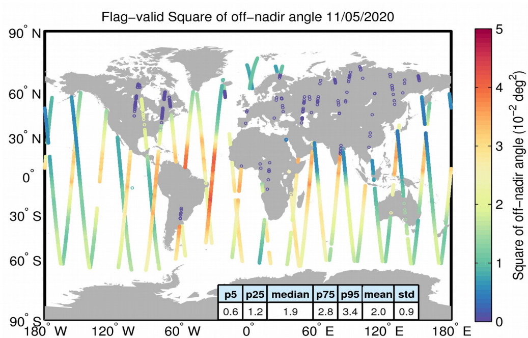
Figure 37. Geographical distribution of flag-valid mispointing data over oceans and lakes for 11/05/2020. The statistical values shown in the table refer to the mispointing in 10^{-2} \text{deg}^2 and are calculated over all measurements shown in the figure.
