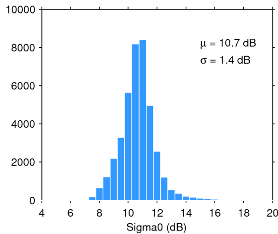
Figure 28. Histogram of science-valid sigma0 over oceans and lakes for 11/05/2020. The mean ( \mu ) and standard deviation ( \sigma ) are also shown. Note that values outside [4 20] dB are excluded from the histogram for the sake of readability but not from the computation of \mu and \sigma .
