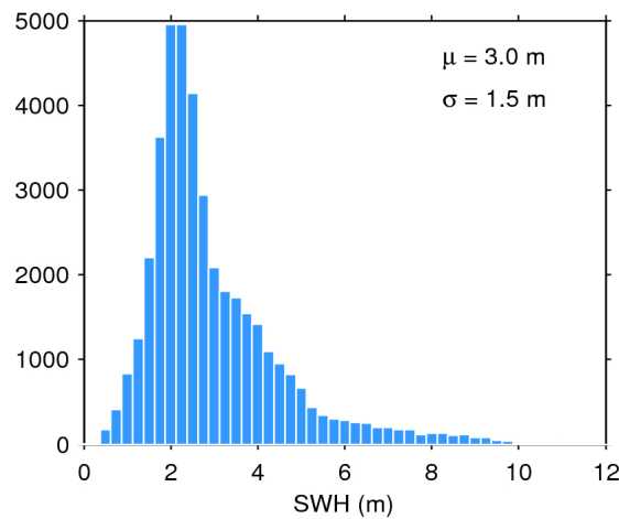
Figure 17. Histogram of flag-valid SWH over oceans and lakes for 10/05/2020. The mean ( \mu ) and standard deviation ( \sigma ) are also shown. Note that values larger than 12 m are excluded from the histogram for the sake of readability but not from the computation of \mu and \sigma .
