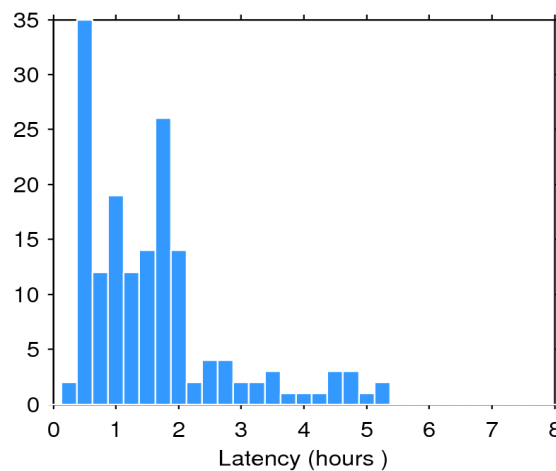
Figure 2. Histogram of the data latency for 10/05/2020. The y-axis denotes the number of files that are made available with a delay of x-hours with respect to the mean time of the records stored in the file.
