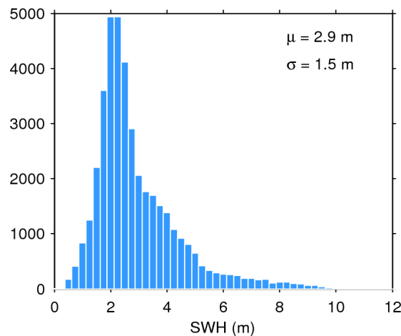
Figure 20. Histogram of science-valid SWH over oceans and lakes for 10/05/2020. The mean ( \mu ) and standard deviation ( \sigma ) are also shown. Note that values larger than 12 m are excluded from the histogram for the sake of readability but not from the computation of \mu and \sigma .
