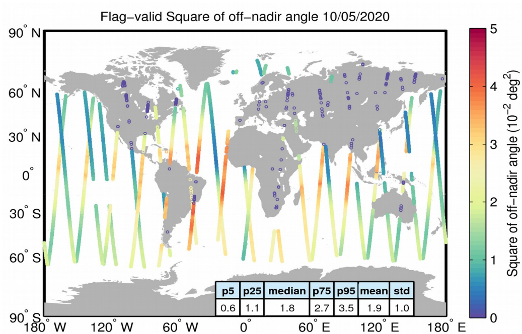
Figure 37. Geographical distribution of flag-valid mispointing data over oceans and lakes for 10/05/2020. The statistical values shown in the table refer to the mispointing in 10^{-2} \text{ deg}^2 and are calculated over all measurements shown in the figure.
