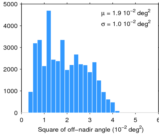
Figure 39. Histogram of flag-valid mispointing over oceans and lakes for 10/05/2020. The mean ( \mu ) and standard deviation ( \sigma ) are also shown. Note that values larger than 6 \cdot 10^{-2} \text{ deg}^2 are excluded from the histogram for the sake of readability but not from the computation of \mu and \sigma .
