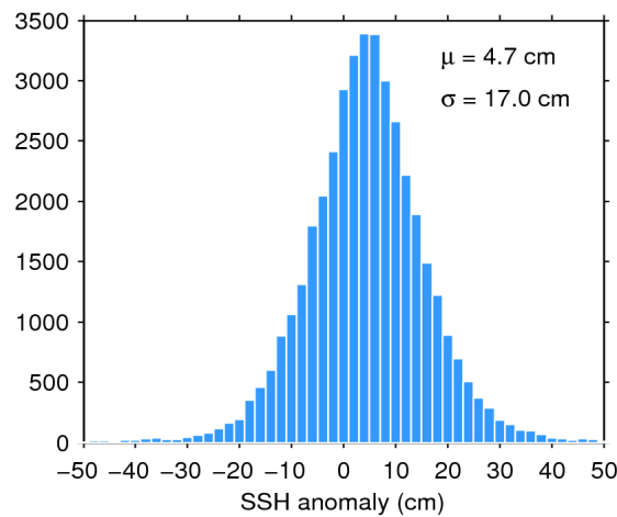
Figure 7. Histogram of flag-valid SSH anomaly over oceans and lakes for 10/05/2020. The mean ( \mu ) and standard deviation ( \sigma ) are also shown. Note that values outside [-50 50] cm are excluded from the histogram for the sake of readability but not from the computation of \mu and \sigma .
