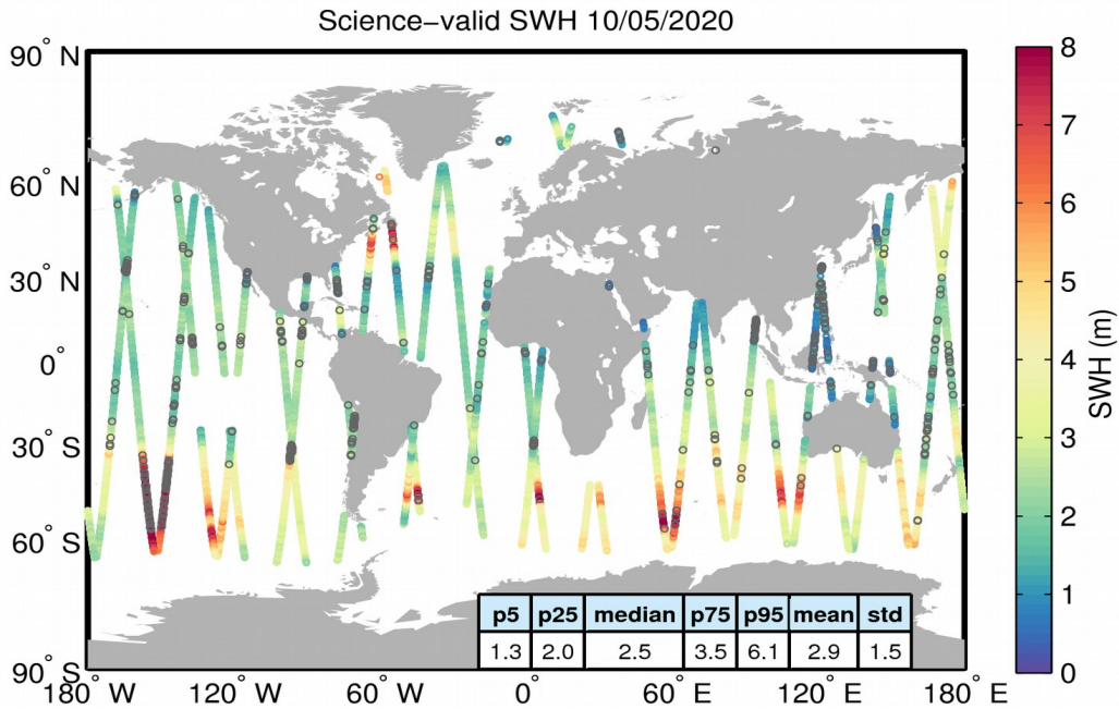
Figure 19. Geographical distribution of science-valid SWH data over oceans and lakes for 10/05/2020. The statistical values shown in the table refer to the SWH in m and are calculated over all measurements shown in the figure. Gray circles denote records that have been rejected based on the editing criteria described in Table 3.
