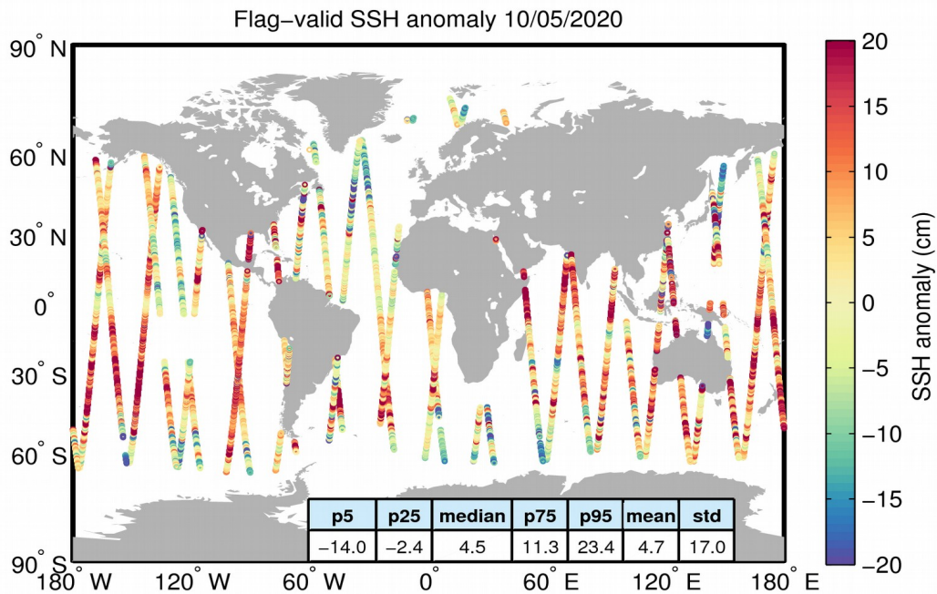
Figure 5. Geographical distribution of flag-valid 1-Hz SSH anomaly data over oceans and lakes for 10/05/2020. The statistical values shown in the table refer to the SSH anomaly in cm and are calculated over all measurements shown in the figure.
