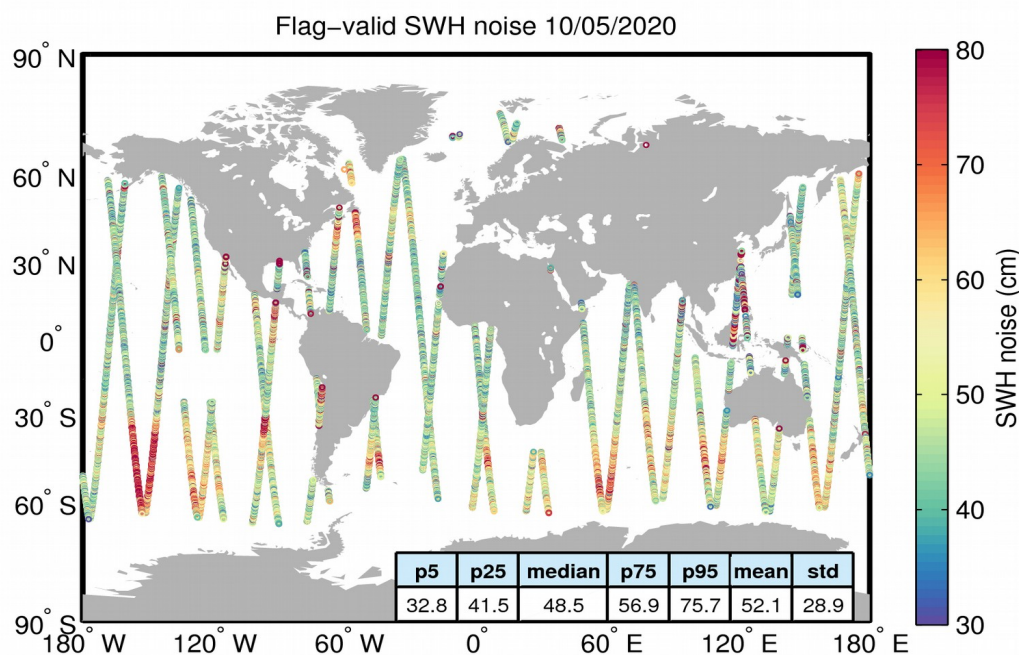
Figure 18. Geographical distribution of flag-valid 20-Hz SWH measurement noise over oceans and lakes for 10/05/2020. The statistical values shown in the figure refer to the SWH noise and are calculated over all measurements shown in the figure.
