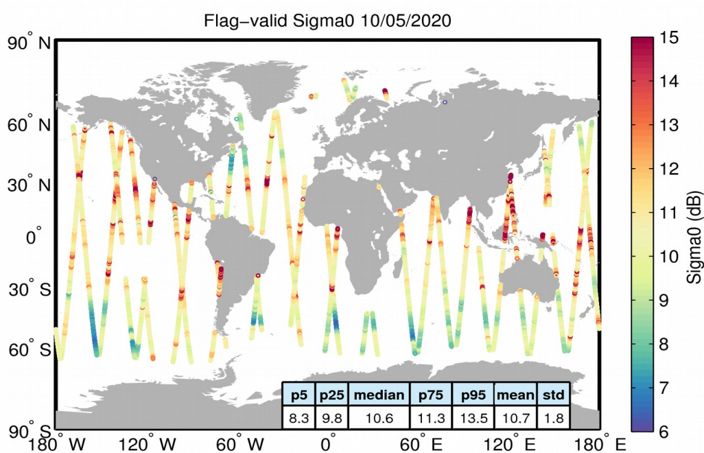
Figure 23. Geographical distribution of flag-valid sigma0 data over oceans and lakes for 10/05/2020. The statistical values shown in the table refer to the sigma0 in dB and are calculated over all measurements shown in the figure.
