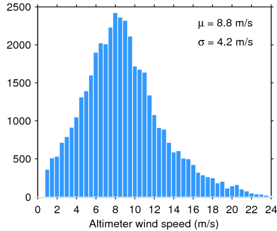
Figure 33. Histogram of flag-valid wind over oceans and lakes for 10/05/2020. The mean ( \mu ) and standard deviation ( \sigma ) are also shown. Note that values larger than 24 m/s are excluded from the histogram for the sake of readability but not from the computation of \mu and \sigma .
