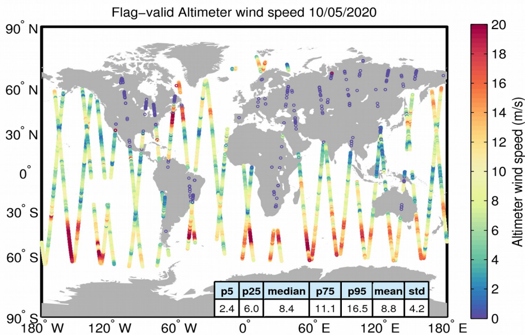
Figure 31. Geographical distribution of flag-valid wind data over oceans and lakes for 10/05/2020. The statistical values shown in the table refer to the wind in m/s and are calculated over all measurements shown in the figure.
