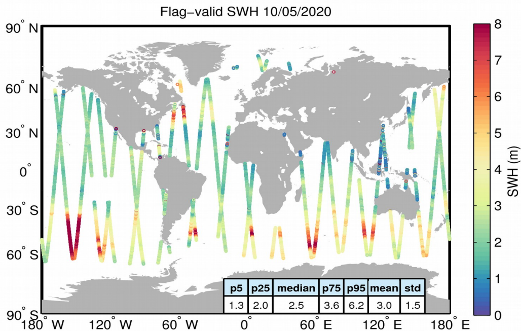
Figure 15. Geographical distribution of flag-valid SWH data over oceans and lakes for 10/05/2020. The statistical values shown in the table refer to the SWH in m and are calculated over all measurements shown in the figure.
