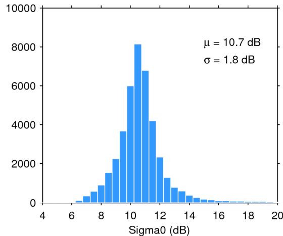
Figure 25. Histogram of flag-valid sigma0 over oceans and lakes for 10/05/2020. The mean ( \mu ) and standard deviation ( \sigma ) are also shown. Note that values outside [4 20] dB are excluded from the histogram for the sake of readability but not from the computation of \mu and \sigma .
