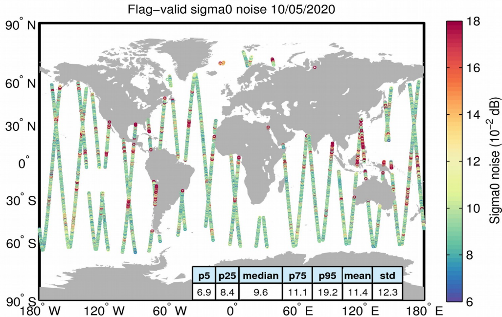
Figure 26. Geographical distribution of flag-valid 20-Hz sigma0 measurement noise over oceans and lakes for 10/05/2020. The statistical values shown in the table refer to the sigma0 noise and are calculated over all measurements shown in the figure.
