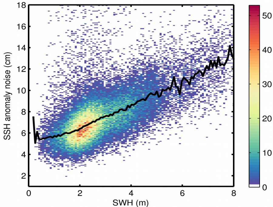
Figure 9. 2D histogram showing flag-valid SSH anomaly noise as a function of SWH for 10/05/2020. The black line denotes the median SSH anomaly noise as a function of SWH.
