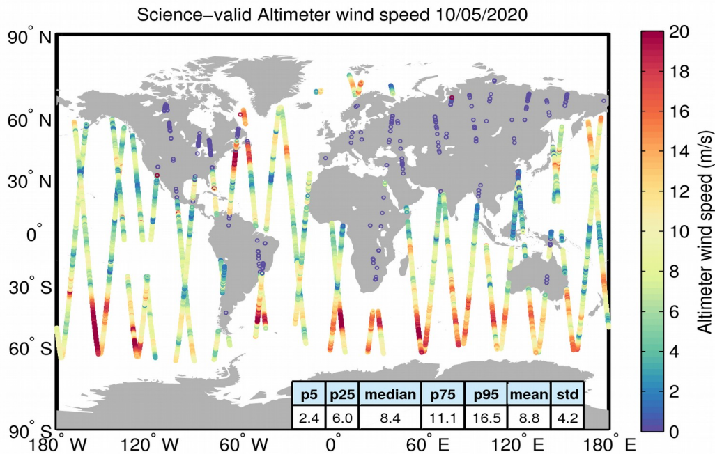
Figure 34. Geographical distribution of science-valid wind data over oceans and lakes for 10/05/2020. The statistical values shown in the table refer to the wind in m/s and are calculated over all measurements shown in the figure. Gray circles denote records that have been rejected based on the editing criteria described in Table 5.
