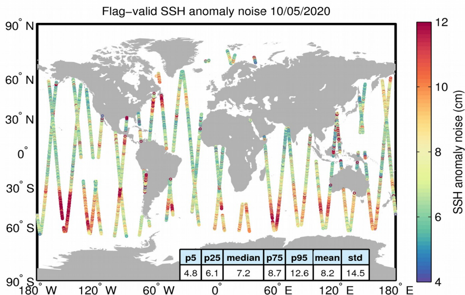
Figure 8. Geographical distribution of flag-valid 20-Hz SSH anomaly measurement noise over oceans and lakes for 10/05/2020. The statistical values shown in the table refer to the SSH anomaly noise and are calculated over all measurements shown in the figure.
