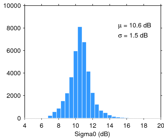
Figure 28. Histogram of science-valid sigma0 over oceans and lakes for 10/05/2020. The mean ( \mu ) and standard deviation ( \sigma ) are also shown. Note that values outside [4 20] dB are excluded from the histogram for the sake of readability but not from the computation of \mu and \sigma .
