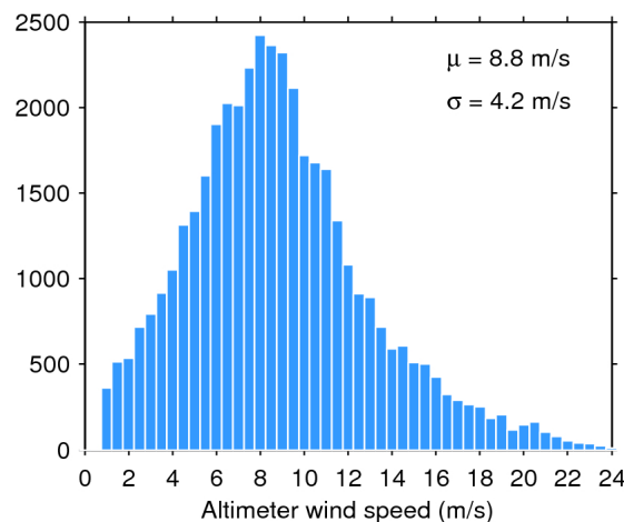
Figure 35. Histogram of science-valid wind over oceans and lakes for 10/05/2020. The mean ( \mu ) and standard deviation ( \sigma ) are also shown. Note that values larger than 24 m/s are excluded from the histogram for the sake of readability but not from the computation of \mu and \sigma .
