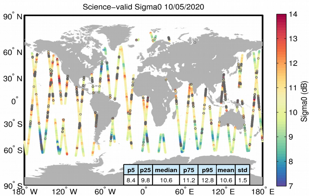
Figure 27. Geographical distribution of science-valid sigma0 data over oceans and lakes for 10/05/2020. The statistical values shown in the table refer to the sigma0 in dB and are calculated over all measurements shown in the figure. Gray circles denote records that have been rejected based on the editing criteria described in Table 4.
