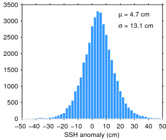
Figure 11. Histogram of science-valid SSH anomaly over oceans and lakes for 10/05/2020. The mean ( \mu ) and standard deviation ( \sigma ) are also shown. Note that values outside [-50 50] cm are excluded from the histogram for the sake of readability but not from the computation of \mu and \sigma .
