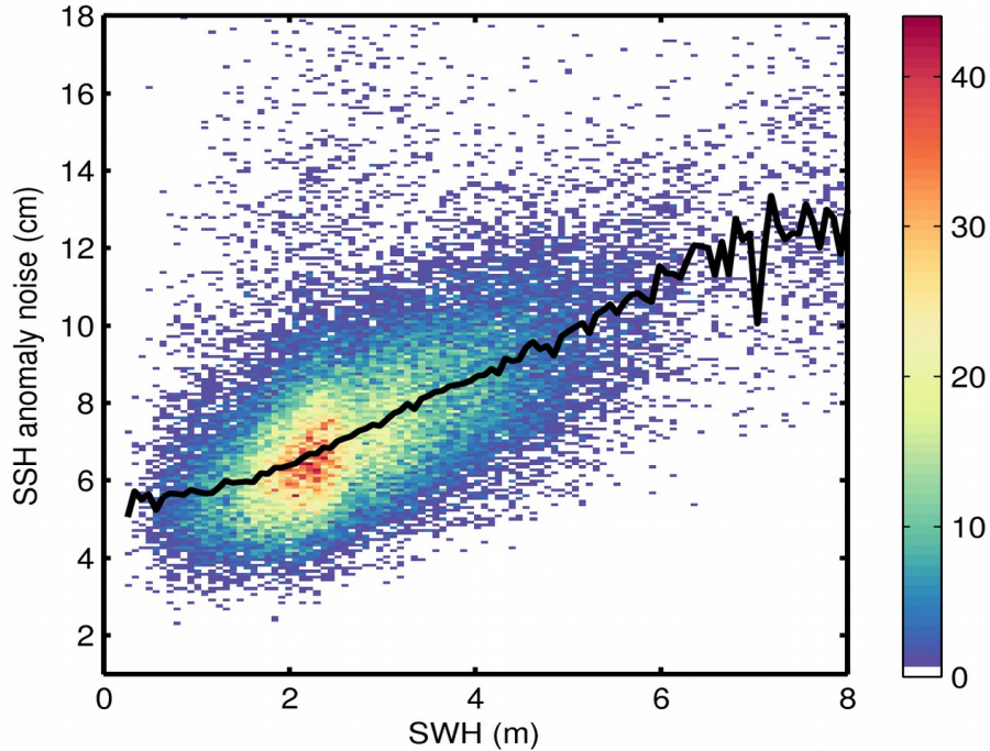
Figure 9. 2D histogram showing flag-valid SSH anomaly noise as a function of SWH for 08/05/2020. The black line denotes the median SSH anomaly noise as a function of SWH.
