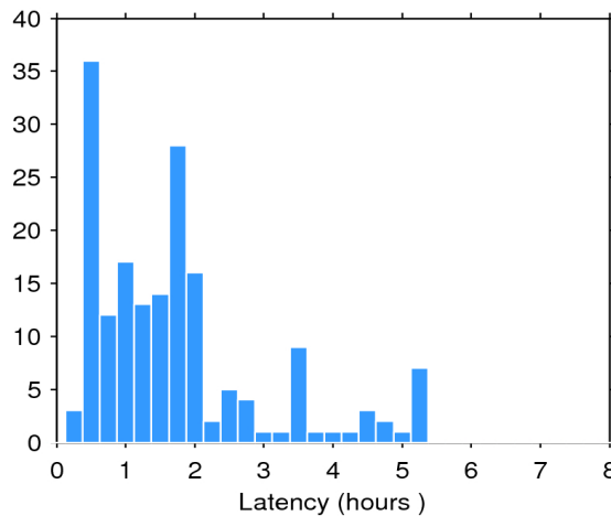
Figure 2. Histogram of the data latency for 08/05/2020. The y-axis denotes the number of files that are made available with a delay of x-hours with respect to the mean time of the records stored in the file.
