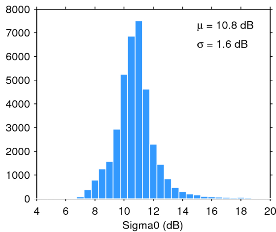
Figure 28. Histogram of science-valid sigma0 over oceans and lakes for 08/05/2020. The mean ( \mu ) and standard deviation ( \sigma ) are also shown. Note that values outside [4 20] dB are excluded from the histogram for the sake of readability but not from the computation of \mu and \sigma .
