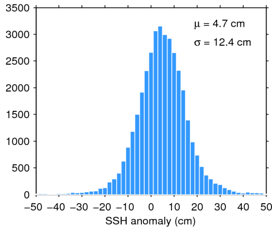
Figure 11. Histogram of science-valid SSH anomaly over oceans and lakes for 08/05/2020. The mean ( \mu ) and standard deviation ( \sigma ) are also shown. Note that values outside [-50 50] cm are excluded from the histogram for the sake of readability but not from the computation of \mu and \sigma .
