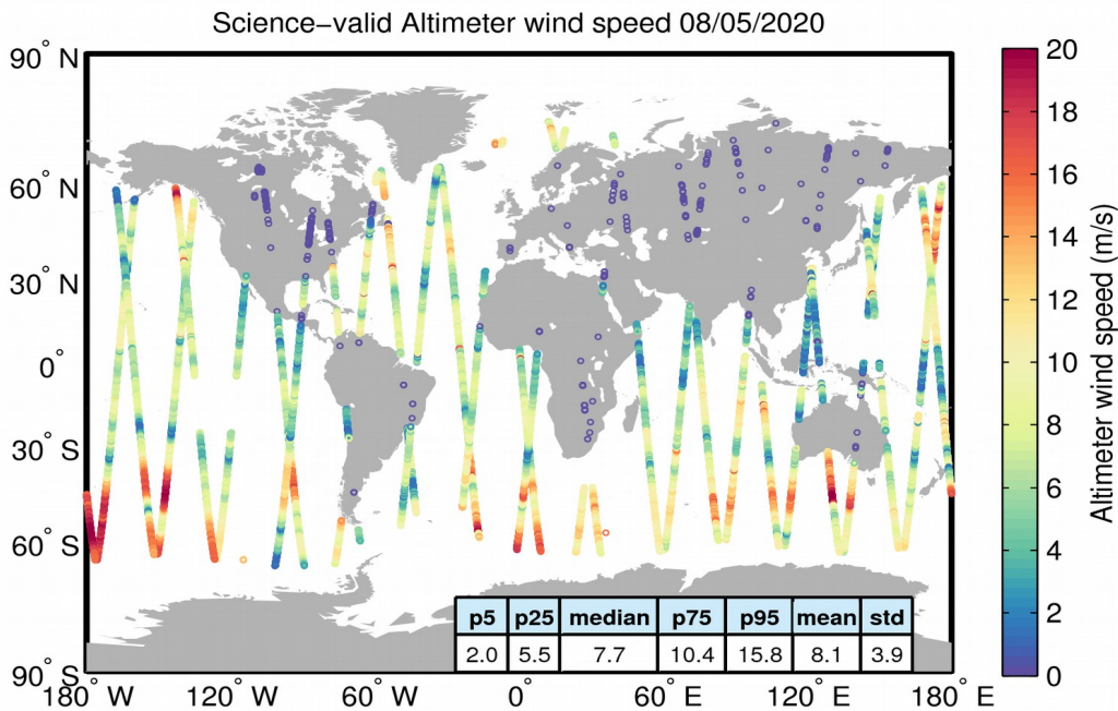
Figure 34. Geographical distribution of science-valid wind data over oceans and lakes for 08/05/2020. The statistical values shown in the table refer to the wind in m/s and are calculated over all measurements shown in the figure. Gray circles denote records that have been rejected based on the editing criteria described in Table 5.
