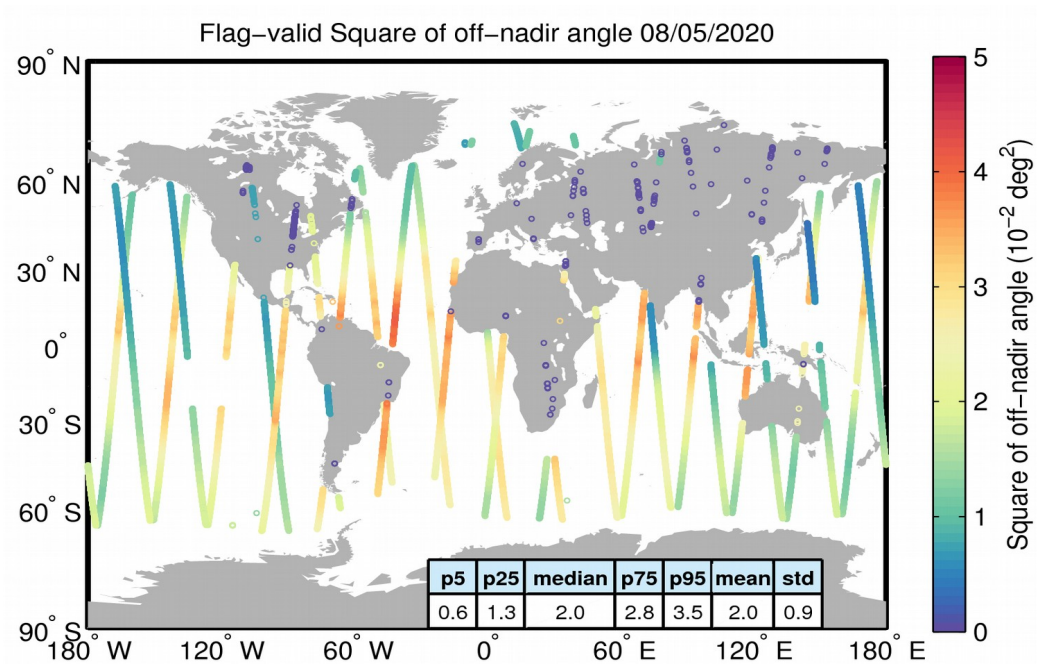
Figure 37. Geographical distribution of flag-valid mispointing data over oceans and lakes for 08/05/2020. The statistical values shown in the table refer to the mispointing in 10^{-2} deg 2 and are calculated over all measurements shown in the figure.
