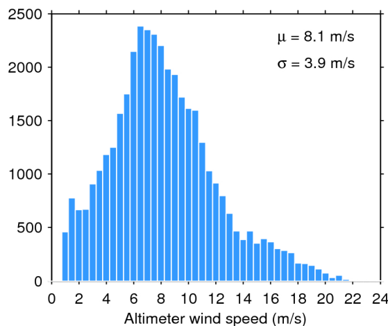
Figure 35. Histogram of science-valid wind over oceans and lakes for 08/05/2020. The mean ( \mu ) and standard deviation ( \sigma ) are also shown. Note that values larger than 24 m/s are excluded from the histogram for the sake of readability but not from the computation of \mu and \sigma .
