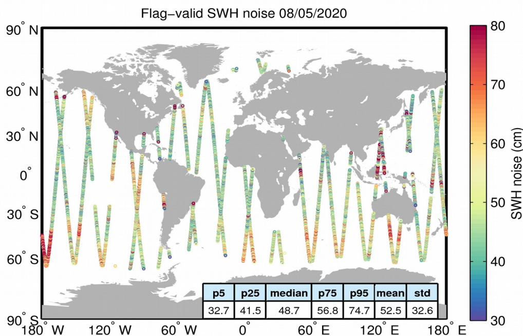
Figure 18. Geographical distribution of flag-valid 20-Hz SWH measurement noise over oceans and lakes for 08/05/2020. The statistical values shown in the table refer to the SWH noise and are calculated over all measurements shown in the figure.
