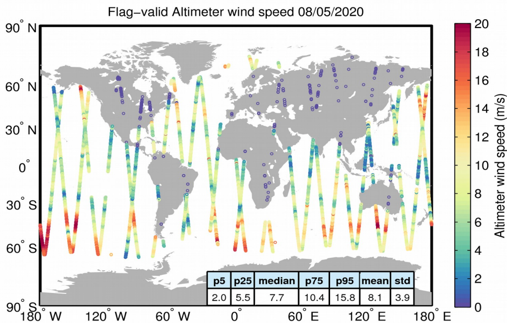
Figure 31. Geographical distribution of flag-valid wind data over oceans and lakes for 08/05/2020. The statistical values shown in the table refer to the wind in m/s and are calculated over all measurements shown in the figure.
