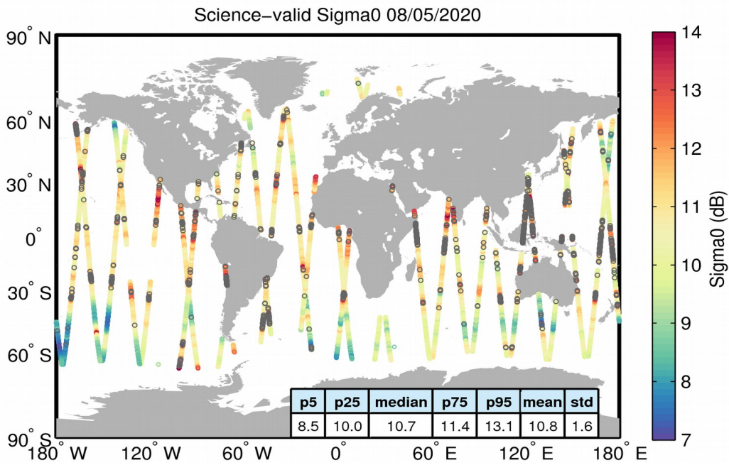
Figure 27. Geographical distribution of science-valid sigma0 data over oceans and lakes for 08/05/2020. The statistical values shown in the table refer to the sigma0 in dB and are calculated over all measurements shown in the figure. Gray circles denote records that have been rejected based on the editing criteria described in Table 4.
