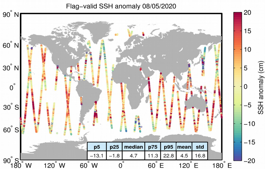
Figure 5. Geographical distribution of flag-valid 1-Hz SSH anomaly data over oceans and lakes for 08/05/2020. The statistical values shown in the table refer to the SSH anomaly in cm and are calculated over all measurements shown in the figure.
