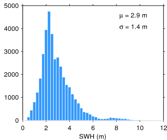
Figure 20. Histogram of science-valid SWH over oceans and lakes for 08/05/2020. The mean ( \mu ) and standard deviation ( \sigma ) are also shown. Note that values larger than 12 m are excluded from the histogram for the sake of readability but not from the computation of \mu and \sigma .
