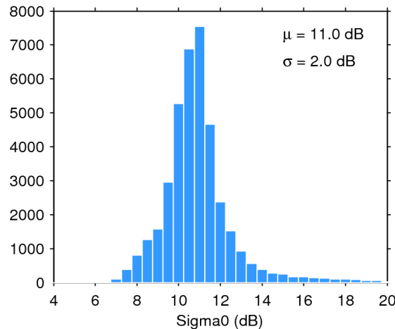
Figure 25. Histogram of flag-valid sigma0 over oceans and lakes for 08/05/2020. The mean ( \mu ) and standard deviation ( \sigma ) are also shown. Note that values outside [4 20] dB are excluded from the histogram for the sake of readability but not from the computation of \mu and \sigma .
