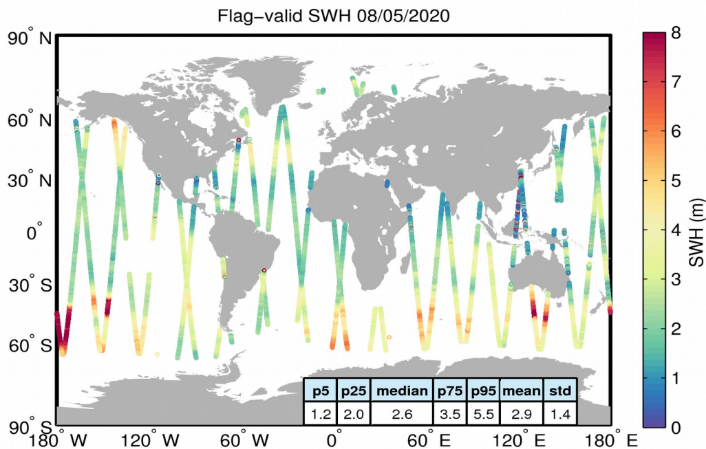
Figure 15. Geographical distribution of flag-valid SWH data over oceans and lakes for 08/05/2020. The statistical values shown in the table refer to the SWH in m and are calculated over all measurements shown in the figure.
