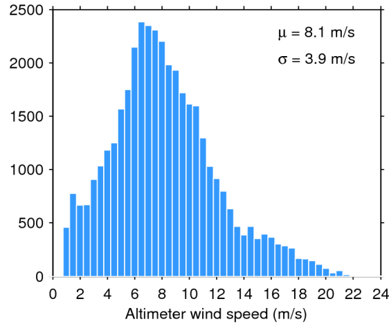
Figure 33. Histogram of flag-valid wind over oceans and lakes for 08/05/2020. The mean ( \mu ) and standard deviation ( \sigma ) are also shown. Note that values larger than 24 m/s are excluded from the histogram for the sake of readability but not from the computation of \mu and \sigma .
