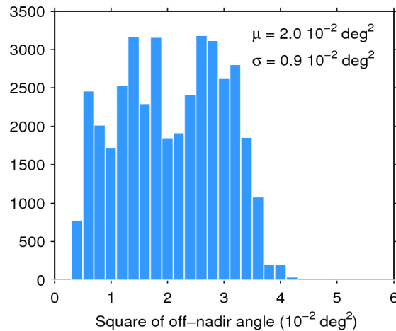
Figure 39. Histogram of flag-valid mispointing over oceans and lakes for 08/05/2020. The mean ( \mu ) and standard deviation ( \sigma ) are also shown. Note that values larger than 6 \cdot 10^{-2} \text{ deg}^2 are excluded from the histogram for the sake of readability but not from the computation of \mu and \sigma .
