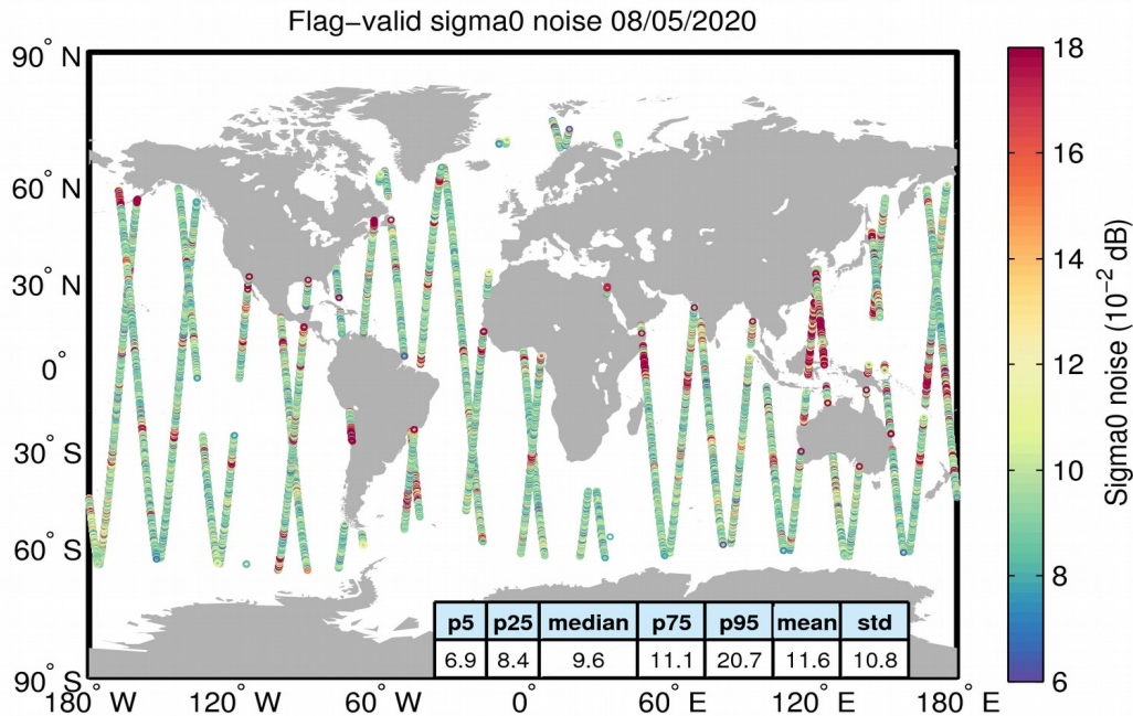
Figure 26. Geographical distribution of flag-valid 20-Hz sigma0 measurement noise over oceans and lakes for 08/05/2020. The statistical values shown in the table refer to the sigma0 noise and are calculated over all measurements shown in the figure.
