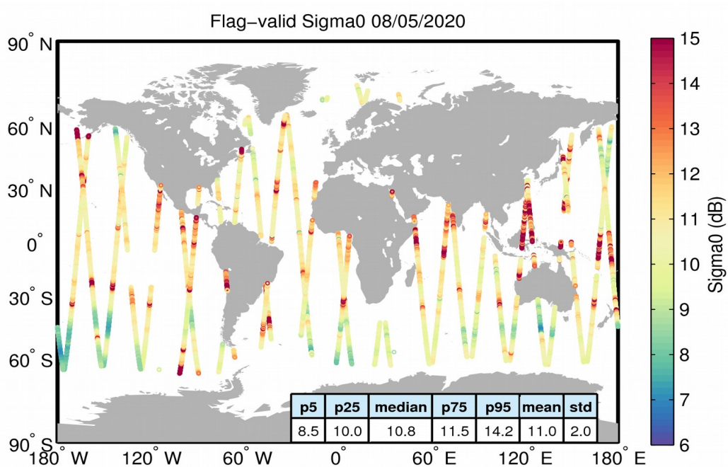
Figure 23. Geographical distribution of flag-valid sigma0 data over oceans and lakes for 08/05/2020. The statistical values shown in the table refer to the sigma0 in dB and are calculated over all measurements shown in the figure.
