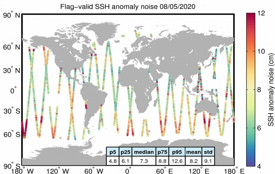
Figure 8. Geographical distribution of flag-valid 20-Hz SSH anomaly measurement noise over oceans and lakes for 08/05/2020. The statistical values shown in the table refer to the SSH anomaly noise and are calculated over all measurements shown in the figure.
