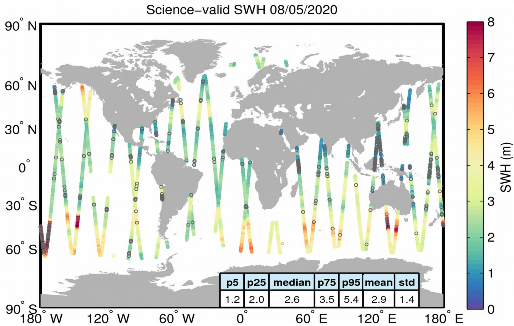
Figure 19. Geographical distribution of science-valid SWH data over oceans and lakes for 08/05/2020. The statistical values shown in the table refer to the SWH in m and are calculated over all measurements shown in the figure. Gray circles denote records that have been rejected based on the editing criteria described in Table 3.
