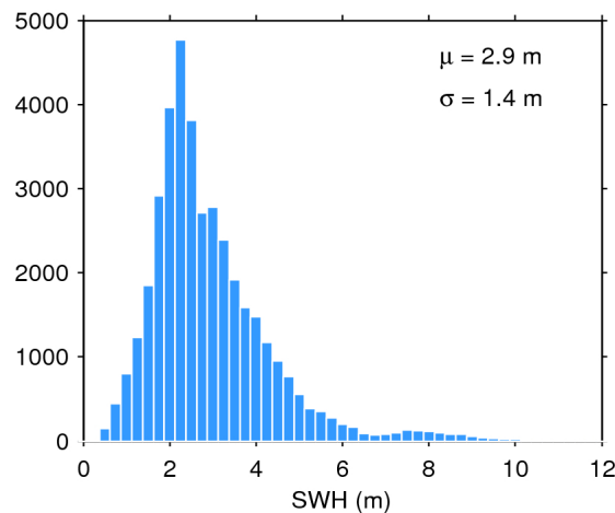
Figure 17. Histogram of flag-valid SWH over oceans and lakes for 08/05/2020. The mean ( \mu ) and standard deviation ( \sigma ) are also shown. Note that values larger than 12 m are excluded from the histogram for the sake of readability but not from the computation of \mu and \sigma .
