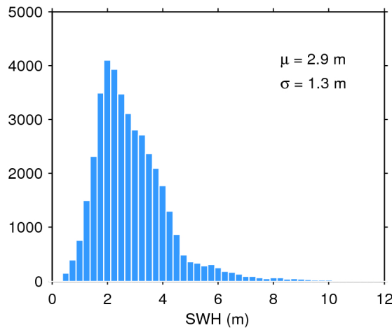
Figure 20. Histogram of science-valid SWH over oceans and lakes for 07/05/2020. The mean ( \mu ) and standard deviation ( \sigma ) are also shown. Note that values larger than 12 m are excluded from the histogram for the sake of readability but not from the computation of \mu and \sigma .
