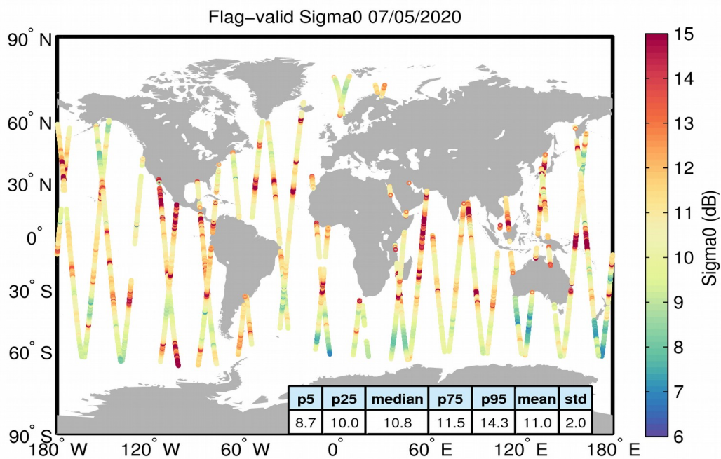
Figure 23. Geographical distribution of flag-valid sigma0 data over oceans and lakes for 07/05/2020. The statistical values shown in the table refer to the sigma0 in dB and are calculated over all measurements shown in the figure.
