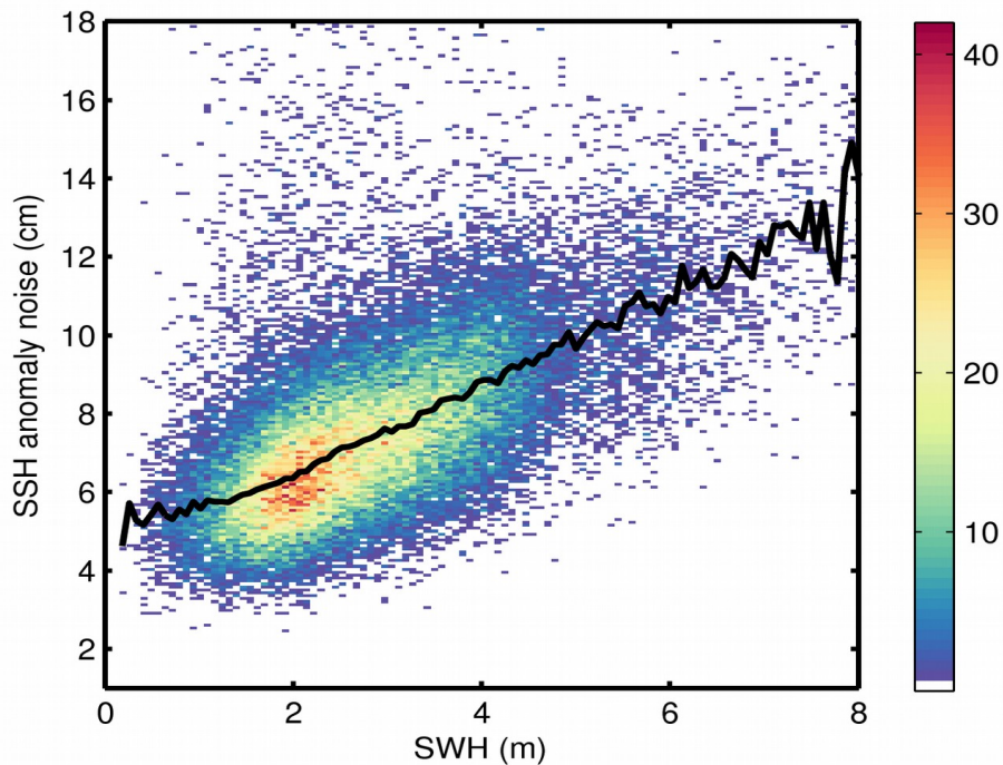
Figure 9. 2D histogram showing flag-valid SSH anomaly noise as a function of SWH for 07/05/2020. The black line denotes the median SSH anomaly noise as a function of SWH.
