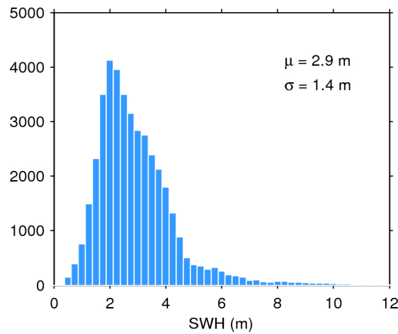
Figure 17. Histogram of flag-valid SWH over oceans and lakes for 07/05/2020. The mean ( \mu ) and standard deviation ( \sigma ) are also shown. Note that values larger than 12 m are excluded from the histogram for the sake of readability but not from the computation of \mu and \sigma .
