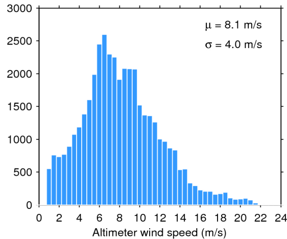
Figure 33. Histogram of flag-valid wind over oceans and lakes for 07/05/2020. The mean ( \mu ) and standard deviation ( \sigma ) are also shown. Note that values larger than 24 m/s are excluded from the histogram for the sake of readability but not from the computation of \mu and \sigma .
