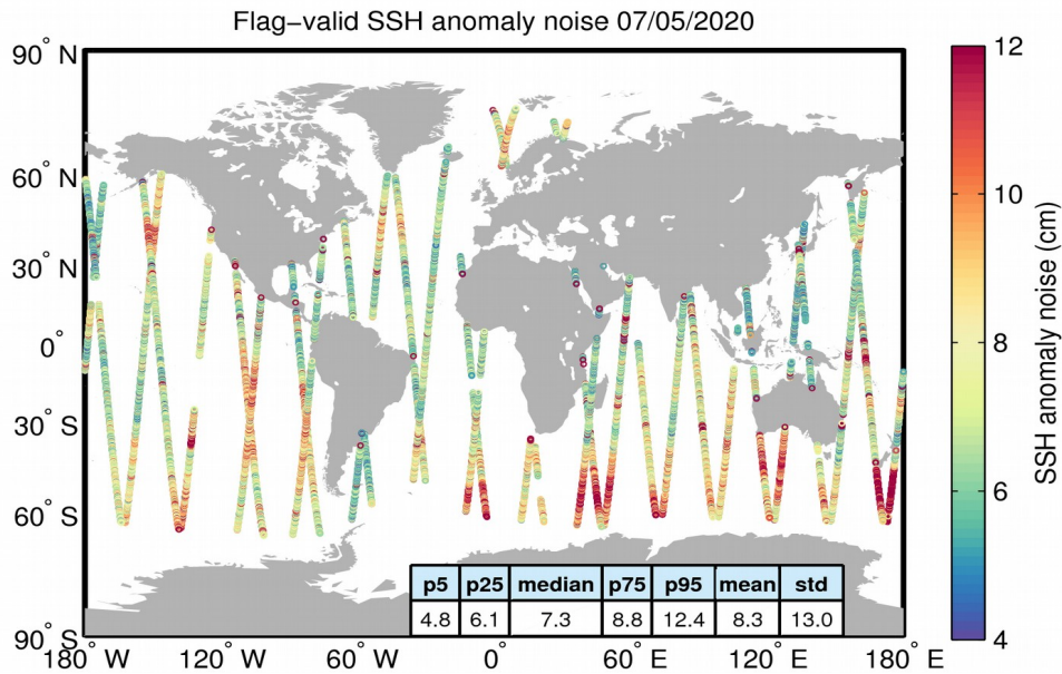
Figure 8. Geographical distribution of flag-valid 20-Hz SSH anomaly measurement noise over oceans and lakes for 07/05/2020. The statistical values shown in the table refer to the SSH anomaly noise and are calculated over all measurements shown in the figure.
