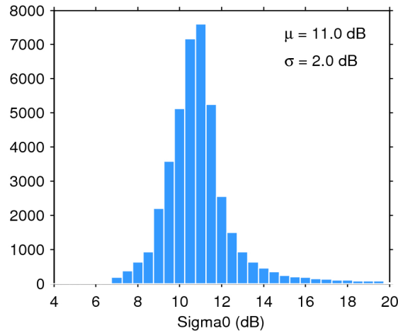
Figure 25. Histogram of flag-valid sigma0 over oceans and lakes for 07/05/2020. The mean ( \mu ) and standard deviation ( \sigma ) are also shown. Note that values outside [4 20] dB are excluded from the histogram for the sake of readability but not from the computation of \mu and \sigma .
