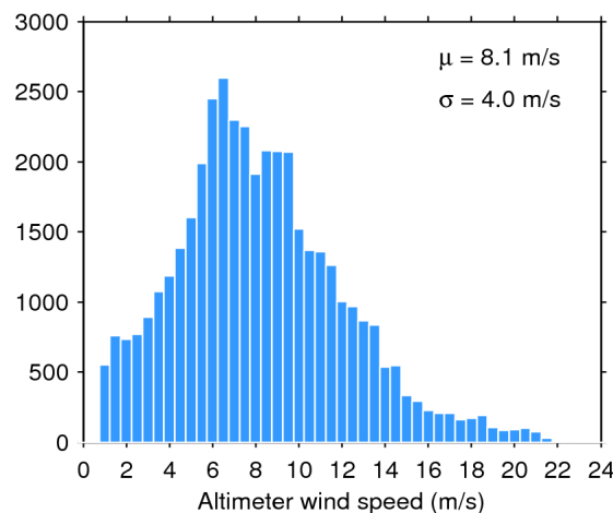
Figure 35. Histogram of science-valid wind over oceans and lakes for 07/05/2020. The mean ( \mu ) and standard deviation ( \sigma ) are also shown. Note that values larger than 24 m/s are excluded from the histogram for the sake of readability but not from the computation of \mu and \sigma .
