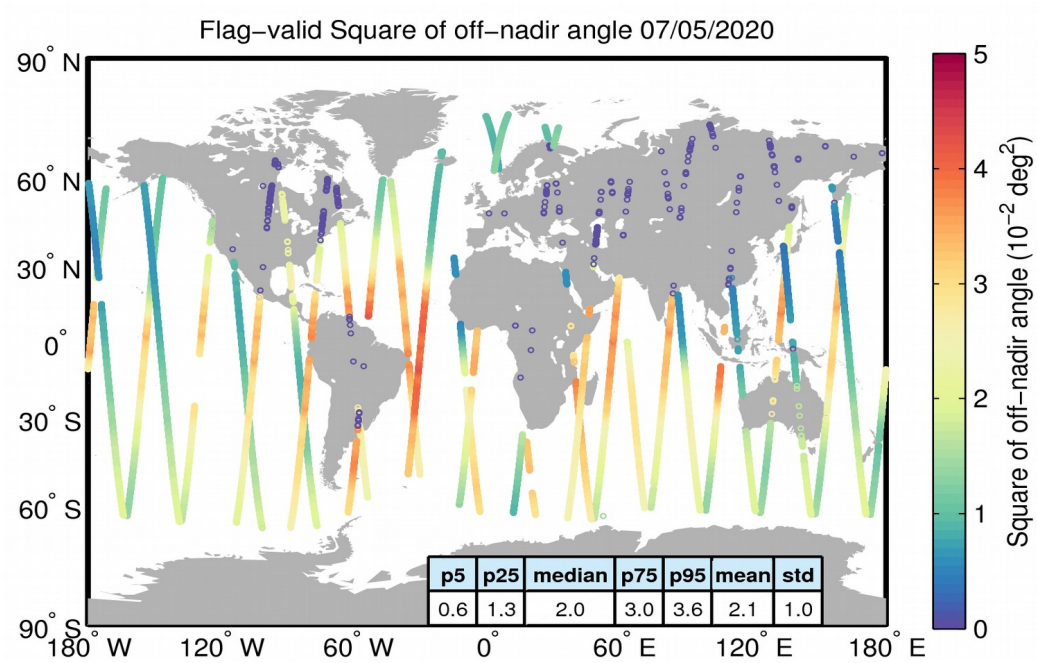
Figure 37. Geographical distribution of flag-valid mispointing data over oceans and lakes for 07/05/2020. The statistical values shown in the table refer to the mispointing in 10^{-2} deg 2 and are calculated over all measurements shown in the figure.
