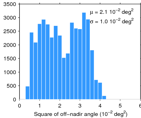
Figure 39. Histogram of flag-valid mispointing over oceans and lakes for 07/05/2020. The mean ( \mu ) and standard deviation ( \sigma ) are also shown. Note that values larger than 6 \cdot 10^{-2} \text{ deg}^2 are excluded from the histogram for the sake of readability but not from the computation of \mu and \sigma .
