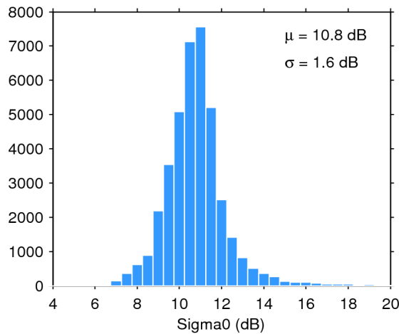
Figure 28. Histogram of science-valid sigma0 over oceans and lakes for 07/05/2020. The mean ( \mu ) and standard deviation ( \sigma ) are also shown. Note that values outside [4 20] dB are excluded from the histogram for the sake of readability but not from the computation of \mu and \sigma .
