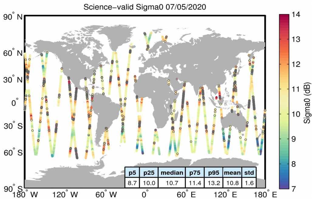
Figure 27. Geographical distribution of science-valid sigma0 data over oceans and lakes for 07/05/2020. The statistical values shown in the table refer to the sigma0 in dB and are calculated over all measurements shown in the figure. Gray circles denote records that have been rejected based on the editing criteria described in Table 4.
