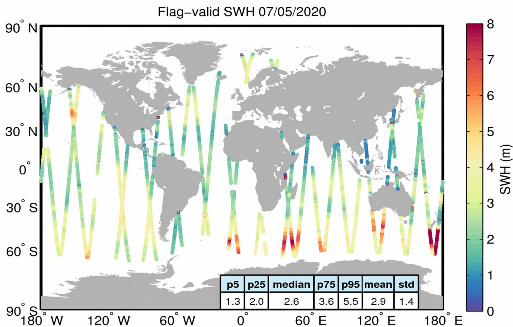
Figure 15. Geographical distribution of flag-valid SWH data over oceans and lakes for 07/05/2020. The statistical values shown in the table refer to the SWH in m and are calculated over all measurements shown in the figure.
