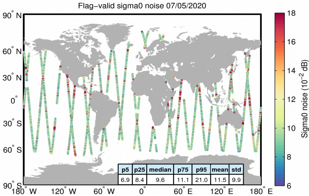
Figure 26. Geographical distribution of flag-valid 20-Hz sigma0 measurement noise over oceans and lakes for 07/05/2020. The statistical values shown in the table refer to the sigma0 noise and are calculated over all measurements shown in the figure.
