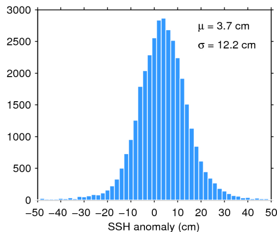
Figure 11. Histogram of science-valid SSH anomaly over oceans and lakes for 07/05/2020. The mean ( \mu ) and standard deviation ( \sigma ) are also shown. Note that values outside [-50 50] cm are excluded from the histogram for the sake of readability but not from the computation of \mu and \sigma .
