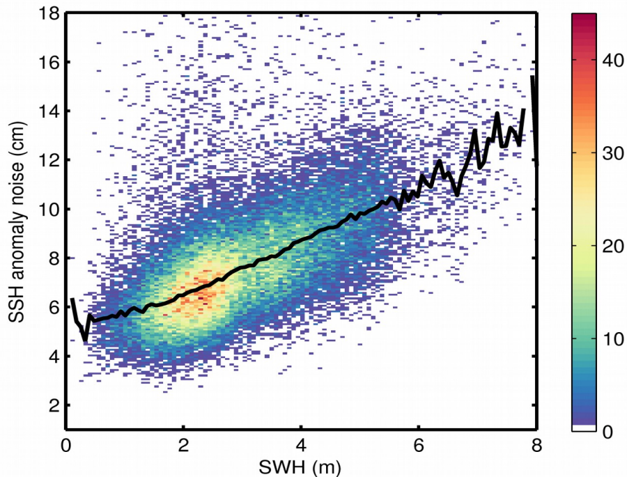
Figure 9. 2D histogram showing flag-valid SSH anomaly noise as a function of SWH for 06/05/2020. The black line denotes the median SSH anomaly noise as a function of SWH.
