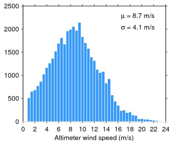
Figure 35. Histogram of science-valid wind over oceans and lakes for 06/05/2020. The mean ( \mu ) and standard deviation ( \sigma ) are also shown. Note that values larger than 24 m/s are excluded from the histogram for the sake of readability but not from the computation of \mu and \sigma .
