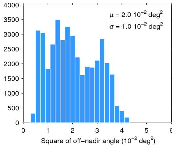
Figure 39. Histogram of flag-valid mispointing over oceans and lakes for 06/05/2020. The mean ( \mu ) and standard deviation ( \sigma ) are also shown. Note that values larger than 6 \cdot 10^{-2} \text{ deg}^2 are excluded from the histogram for the sake of readability but not from the computation of \mu and \sigma .
