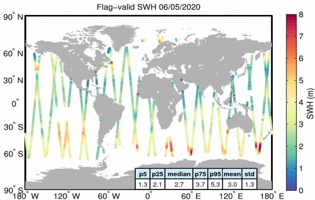
Figure 15. Geographical distribution of flag-valid SWH data over oceans and lakes for 06/05/2020. The statistical values shown in the table refer to the SWH in m and are calculated over all measurements shown in the figure.
