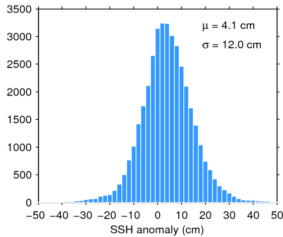
Figure 11. Histogram of science-valid SSH anomaly over oceans and lakes for 06/05/2020. The mean ( \mu ) and standard deviation ( \sigma ) are also shown. Note that values outside [-50 50] cm are excluded from the histogram for the sake of readability but not from the computation of \mu and \sigma .
