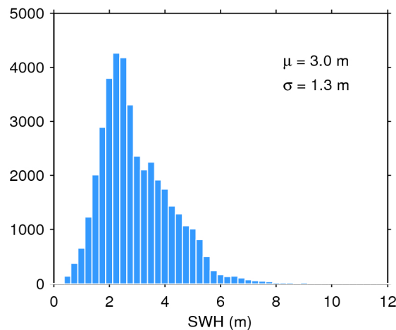
Figure 17. Histogram of flag-valid SWH over oceans and lakes for 06/05/2020. The mean ( \mu ) and standard deviation ( \sigma ) are also shown. Note that values larger than 12 m are excluded from the histogram for the sake of readability but not from the computation of \mu and \sigma .
