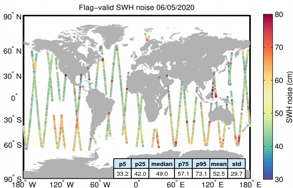
Figure 18. Geographical distribution of flag-valid 20-Hz SWH measurement noise over oceans and lakes for 06/05/2020. The statistical values shown in the figure refer to the SWH noise and are calculated over all measurements shown in the figure.
