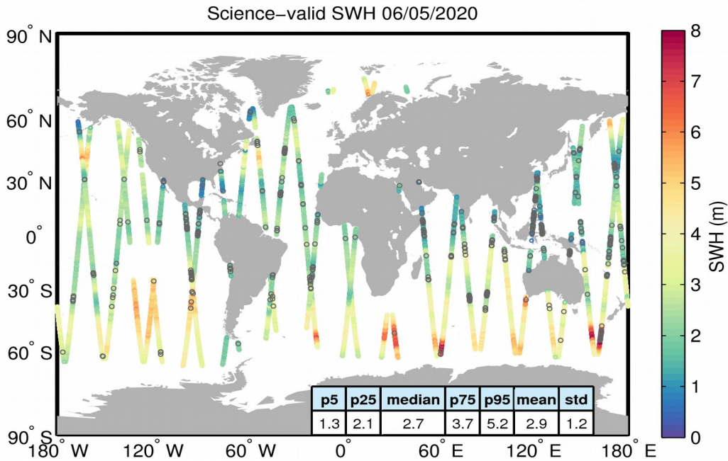
Figure 19. Geographical distribution of science-valid SWH data over oceans and lakes for 06/05/2020. The statistical values shown in the table refer to the SWH in m and are calculated over all measurements shown in the figure. Gray circles denote records that have been rejected based on the editing criteria described in Table 3.
