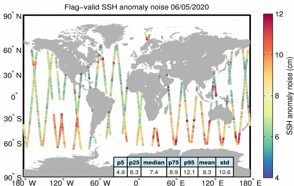
Figure 8. Geographical distribution of flag-valid 20-Hz SSH anomaly measurement noise over oceans and lakes for 06/05/2020. The statistical values shown in the table refer to the SSH anomaly noise and are calculated over all measurements shown in the figure.
