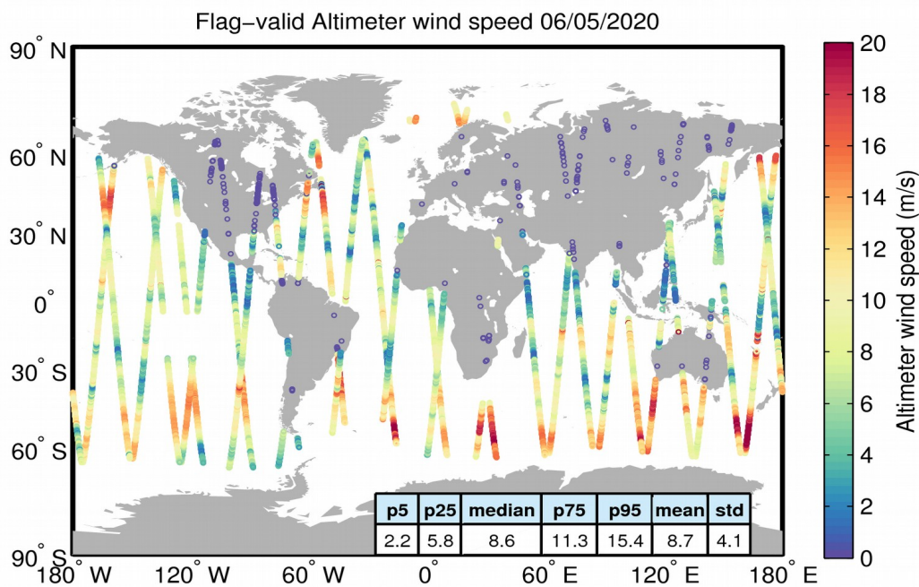
Figure 31. Geographical distribution of flag-valid wind data over oceans and lakes for 06/05/2020. The statistical values shown in the table refer to the wind in m/s and are calculated over all measurements shown in the figure.
