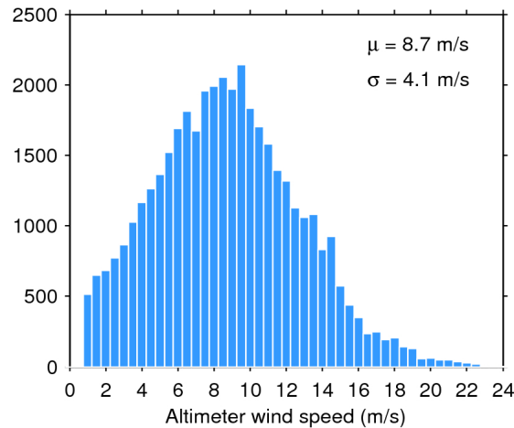
Figure 33. Histogram of flag-valid wind over oceans and lakes for 06/05/2020. The mean ( \mu ) and standard deviation ( \sigma ) are also shown. Note that values larger than 24 m/s are excluded from the histogram for the sake of readability but not from the computation of \mu and \sigma .
