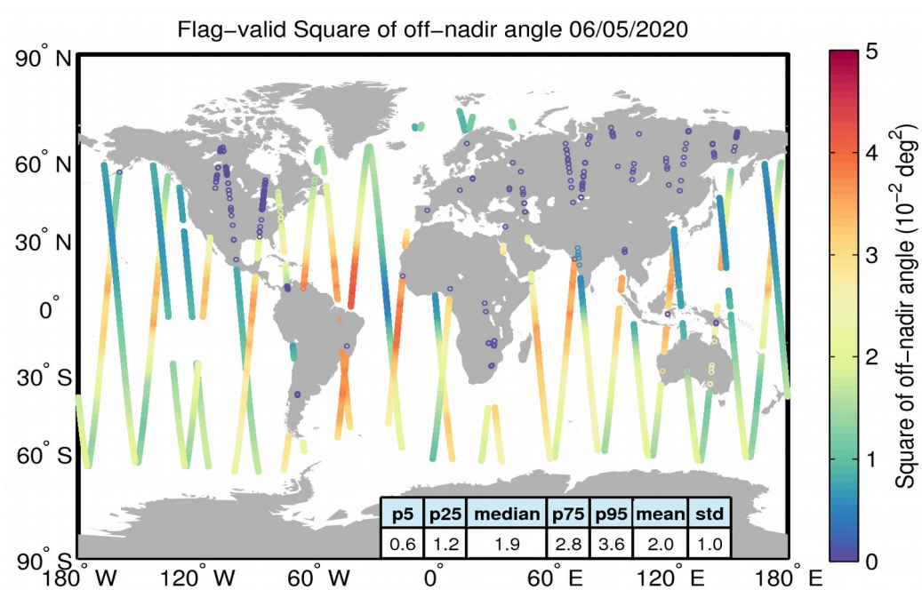
Figure 37. Geographical distribution of flag-valid mispointing data over oceans and lakes for 06/05/2020. The statistical values shown in the table refer to the mispointing in 10^{-2} \text{ deg}^2 and are calculated over all measurements shown in the figure.
