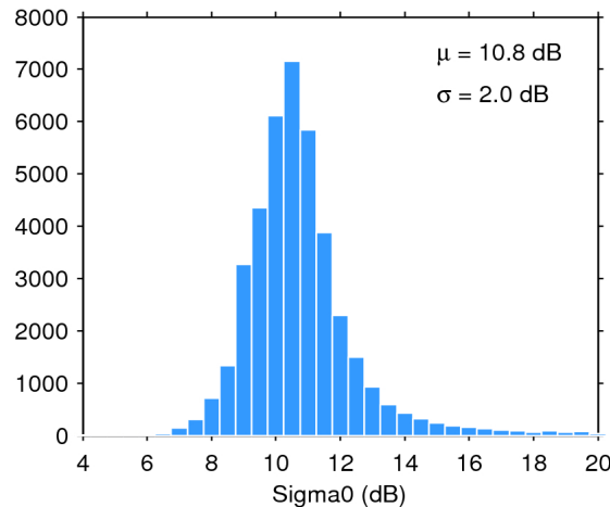
Figure 25. Histogram of flag-valid sigma0 over oceans and lakes for 06/05/2020. The mean ( \mu ) and standard deviation ( \sigma ) are also shown. Note that values outside [4 20] dB are excluded from the histogram for the sake of readability but not from the computation of \mu and \sigma .
