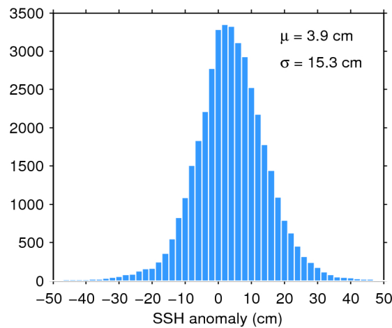
Figure 7. Histogram of flag-valid SSH anomaly over oceans and lakes for 06/05/2020. The mean ( \mu ) and standard deviation ( \sigma ) are also shown. Note that values outside [-50\ 50] cm are excluded from the histogram for the sake of readability but not from the computation of \mu and \sigma .
