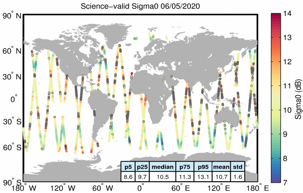
Figure 27. Geographical distribution of science-valid sigma0 data over oceans and lakes for 06/05/2020. The statistical values shown in the table refer to the sigma0 in dB and are calculated over all measurements shown in the figure. Gray circles denote records that have been rejected based on the editing criteria described in Table 4.
