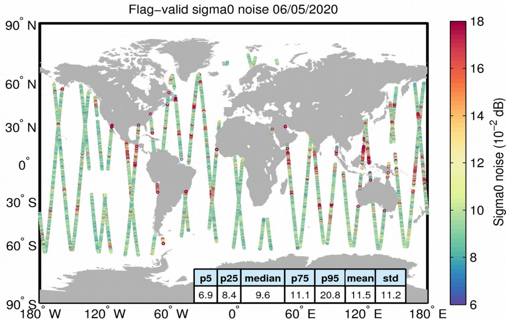
Figure 26. Geographical distribution of flag-valid 20-Hz sigma0 measurement noise over oceans and lakes for 06/05/2020. The statistical values shown in the table refer to the sigma0 noise and are calculated over all measurements shown in the figure.
