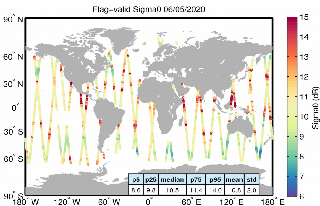
Figure 23. Geographical distribution of flag-valid sigma0 data over oceans and lakes for 06/05/2020. The statistical values shown in the table refer to the sigma0 in dB and are calculated over all measurements shown in the figure.
