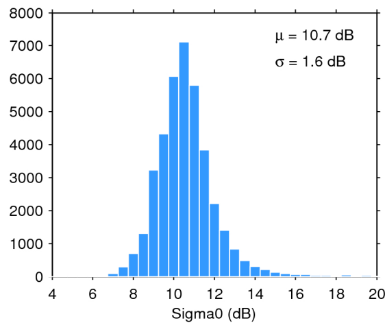
Figure 28. Histogram of science-valid sigma0 over oceans and lakes for 06/05/2020. The mean ( \mu ) and standard deviation ( \sigma ) are also shown. Note that values outside [4 20] dB are excluded from the histogram for the sake of readability but not from the computation of \mu and \sigma .
