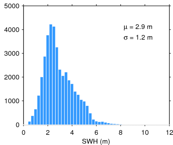
Figure 20. Histogram of science-valid SWH over oceans and lakes for 06/05/2020. The mean ( \mu ) and standard deviation ( \sigma ) are also shown. Note that values larger than 12 m are excluded from the histogram for the sake of readability but not from the computation of \mu and \sigma .
