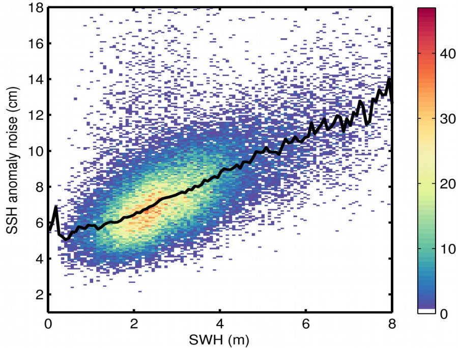
Figure 9. 2D histogram showing flag-valid SSH anomaly noise as a function of SWH for 03/05/2020. The black line denotes the median SSH anomaly noise as a function of SWH.
