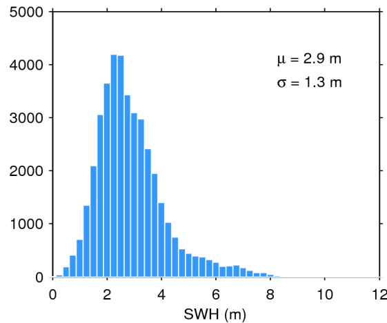
Figure 20. Histogram of science-valid SWH over oceans and lakes for 03/05/2020. The mean ( \mu ) and standard deviation ( \sigma ) are also shown. Note that values larger than 12 m are excluded from the histogram for the sake of readability but not from the computation of \mu and \sigma .
