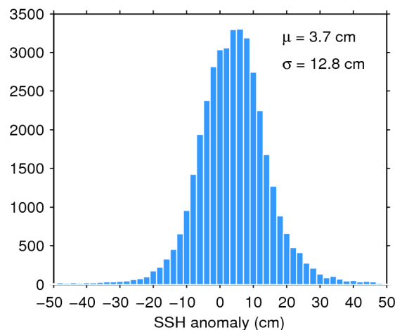
Figure 11. Histogram of science-valid SSH anomaly over oceans and lakes for 03/05/2020. The mean ( \mu ) and standard deviation ( \sigma ) are also shown. Note that values outside [-50 50] cm are excluded from the histogram for the sake of readability but not from the computation of \mu and \sigma .
