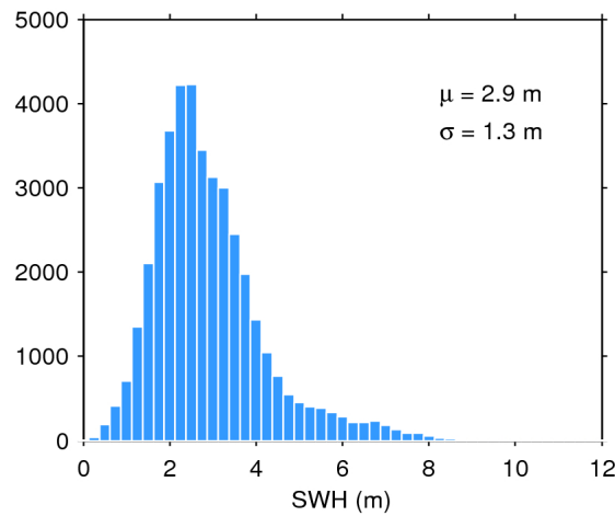
Figure 17. Histogram of flag-valid SWH over oceans and lakes for 03/05/2020. The mean ( \mu ) and standard deviation ( \sigma ) are also shown. Note that values larger than 12 m are excluded from the histogram for the sake of readability but not from the computation of \mu and \sigma .
