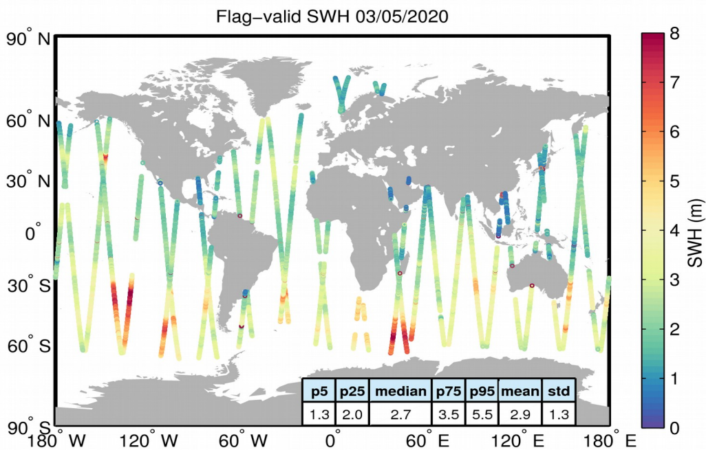
Figure 15. Geographical distribution of flag-valid SWH data over oceans and lakes for 03/05/2020. The statistical values shown in the table refer to the SWH in m and are calculated over all measurements shown in the figure.
