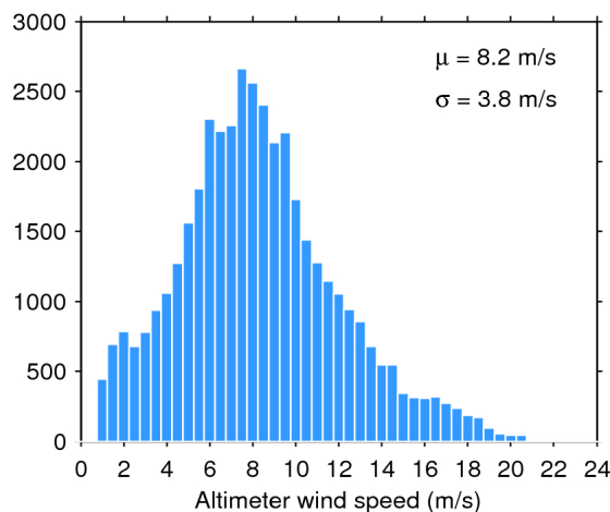
Figure 35. Histogram of science-valid wind over oceans and lakes for 03/05/2020. The mean ( \mu ) and standard deviation ( \sigma ) are also shown. Note that values larger than 24 m/s are excluded from the histogram for the sake of readability but not from the computation of \mu and \sigma .
