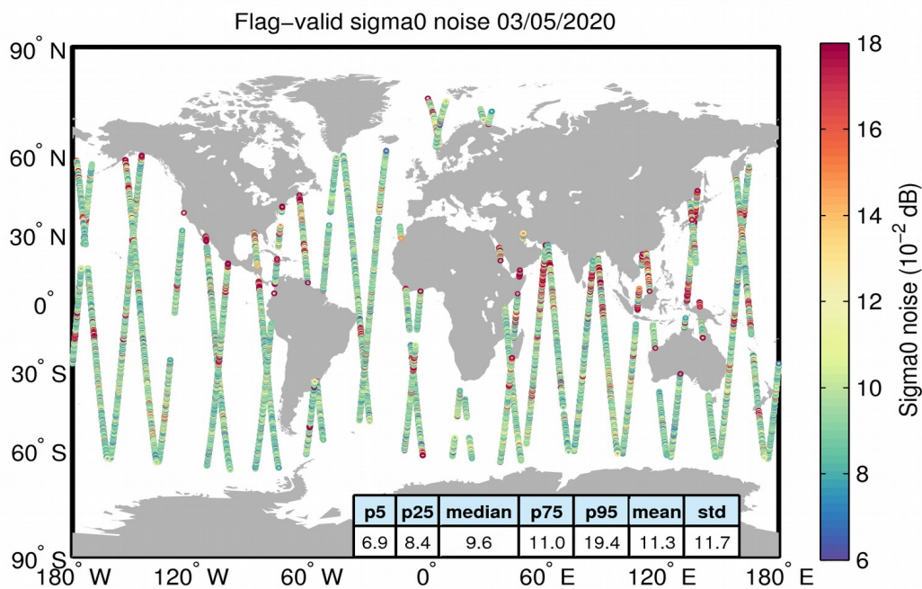
Figure 26. Geographical distribution of flag-valid 20-Hz sigma0 measurement noise over oceans and lakes for 03/05/2020. The statistical values shown in the table refer to the sigma0 noise and are calculated over all measurements shown in the figure.
