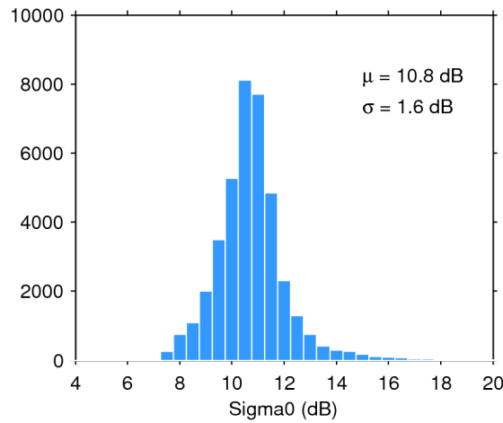
Figure 28. Histogram of science-valid sigma0 over oceans and lakes for 03/05/2020. The mean ( \mu ) and standard deviation ( \sigma ) are also shown. Note that values outside [4 20] dB are excluded from the histogram for the sake of readability but not from the computation of \mu and \sigma .
