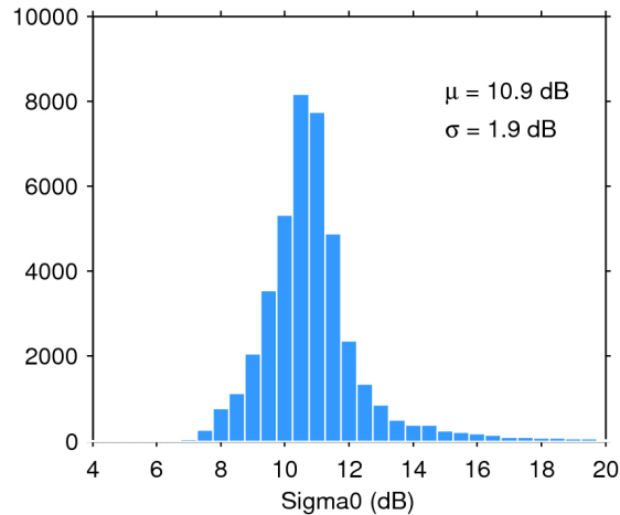
Figure 25. Histogram of flag-valid sigma0 over oceans and lakes for 03/05/2020. The mean ( \mu ) and standard deviation ( \sigma ) are also shown. Note that values outside [4 20] dB are excluded from the histogram for the sake of readability but not from the computation of \mu and \sigma .
