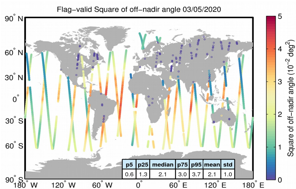
Figure 37. Geographical distribution of flag-valid mispointing data over oceans and lakes for 03/05/2020. The statistical values shown in the table refer to the mispointing in 10^{-2} deg 2 and are calculated over all measurements shown in the figure.
