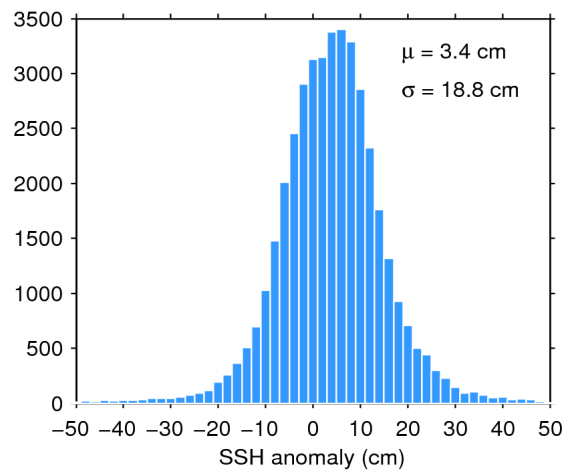
Figure 7. Histogram of flag-valid SSH anomaly over oceans and lakes for 03/05/2020. The mean ( \mu ) and standard deviation ( \sigma ) are also shown. Note that values outside [-50 50] cm are excluded from the histogram for the sake of readability but not from the computation of \mu and \sigma .
