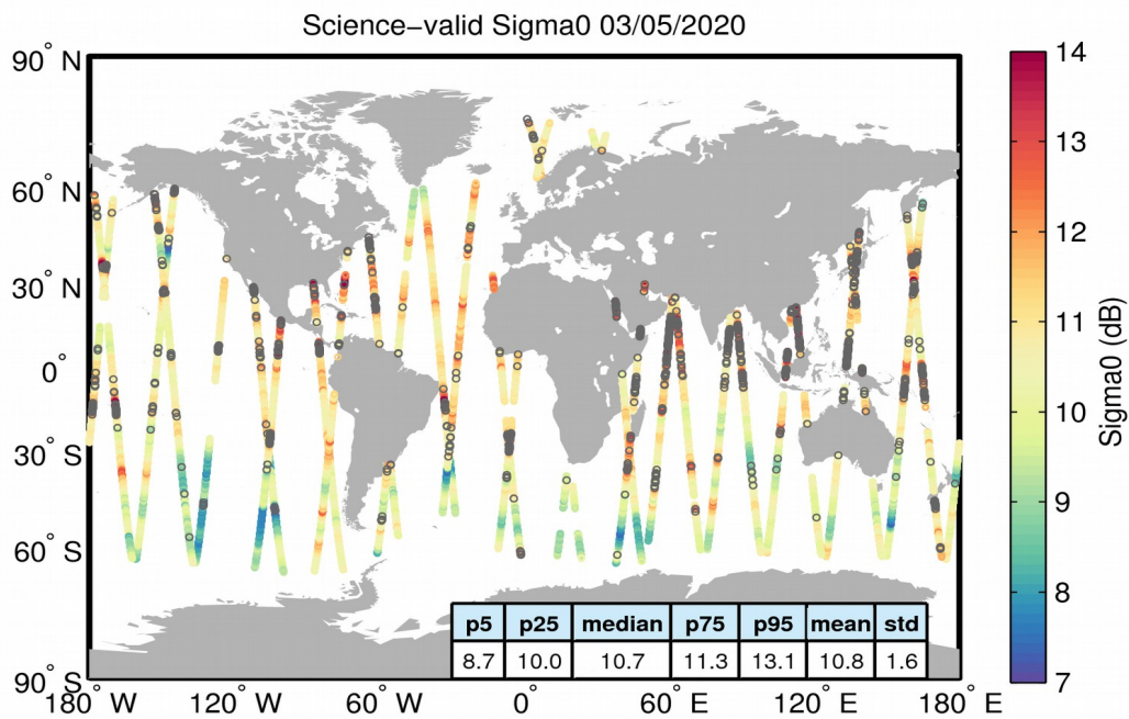
Figure 27. Geographical distribution of science-valid sigma0 data over oceans and lakes for 03/05/2020. The statistical values shown in the table refer to the sigma0 in dB and are calculated over all measurements shown in the figure. Gray circles denote records that have been rejected based on the editing criteria described in Table 4.
