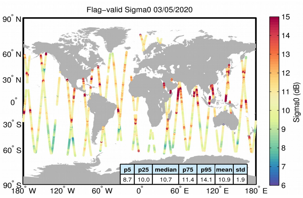
Figure 23. Geographical distribution of flag-valid sigma0 data over oceans and lakes for 03/05/2020. The statistical values shown in the table refer to the sigma0 in dB and are calculated over all measurements shown in the figure.
