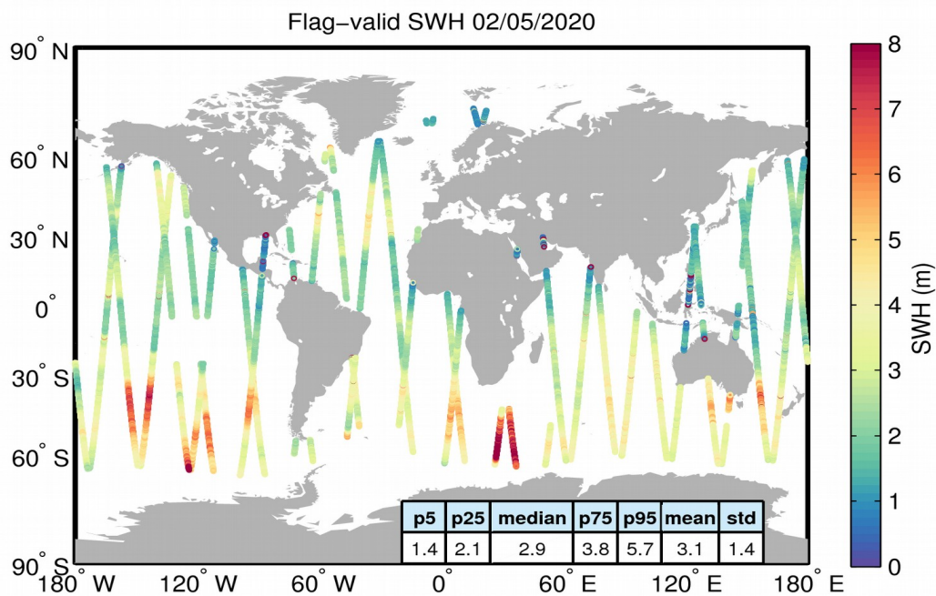
Figure 15. Geographical distribution of flag-valid SWH data over oceans and lakes for 02/05/2020. The statistical values shown in the table refer to the SWH in m and are calculated over all measurements shown in the figure.
