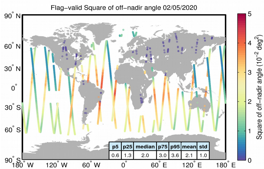
Figure 37. Geographical distribution of flag-valid mispointing data over oceans and lakes for 02/05/2020. The statistical values shown in the table refer to the mispointing in 10^{-2} deg 2 and are calculated over all measurements shown in the figure.
