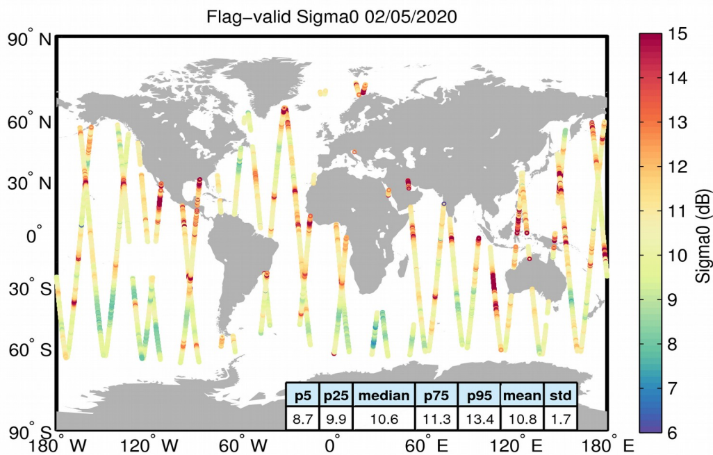
Figure 23. Geographical distribution of flag-valid sigma0 data over oceans and lakes for 02/05/2020. The statistical values shown in the table refer to the sigma0 in dB and are calculated over all measurements shown in the figure.
