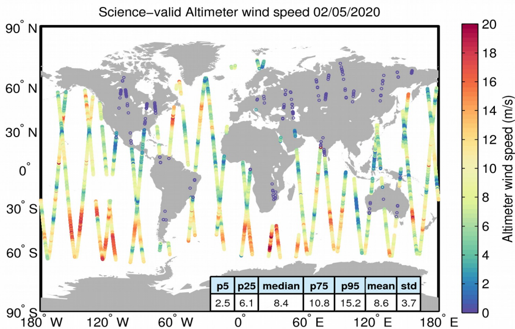
Figure 34. Geographical distribution of science-valid wind data over oceans and lakes for 02/05/2020. The statistical values shown in the table refer to the wind in m/s and are calculated over all measurements shown in the figure. Gray circles denote records that have been rejected based on the editing criteria described in Table 5.
