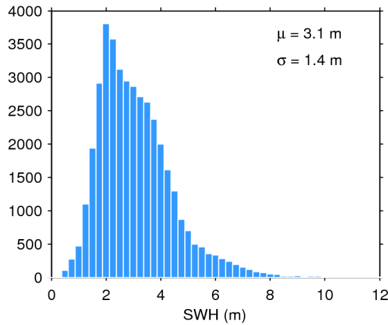
Figure 17. Histogram of flag-valid SWH over oceans and lakes for 02/05/2020. The mean ( \mu ) and standard deviation ( \sigma ) are also shown. Note that values larger than 12 m are excluded from the histogram for the sake of readability but not from the computation of \mu and \sigma .
