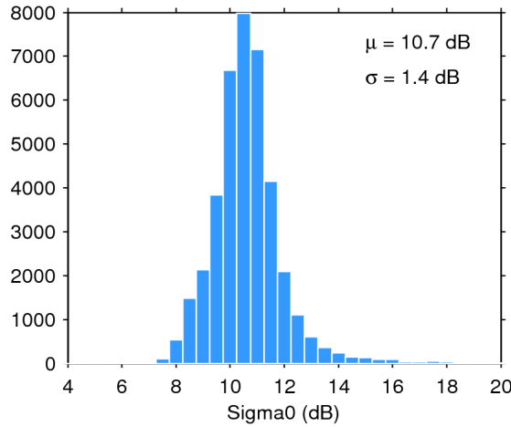
Figure 28. Histogram of science-valid sigma0 over oceans and lakes for 02/05/2020. The mean ( \mu ) and standard deviation ( \sigma ) are also shown. Note that values outside [4 20] dB are excluded from the histogram for the sake of readability but not from the computation of \mu and \sigma .
