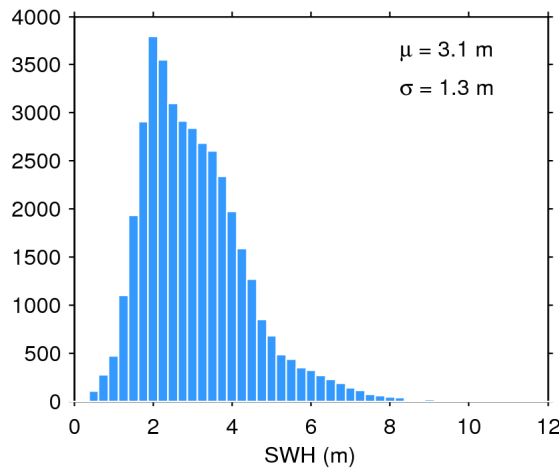
Figure 20. Histogram of science-valid SWH over oceans and lakes for 02/05/2020. The mean ( \mu ) and standard deviation ( \sigma ) are also shown. Note that values larger than 12 m are excluded from the histogram for the sake of readability but not from the computation of \mu and \sigma .
