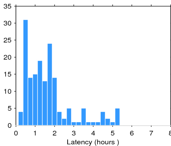
Figure 2. Histogram of the data latency for 02/05/2020. The y-axis denotes the number of files that are made available with a delay of x-hours with respect to the mean time of the records stored in the file.
