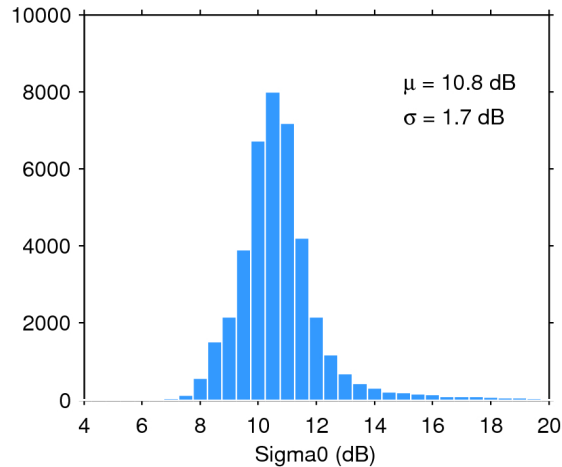
Figure 25. Histogram of flag-valid sigma0 over oceans and lakes for 02/05/2020. The mean ( \mu ) and standard deviation ( \sigma ) are also shown. Note that values outside [4 20] dB are excluded from the histogram for the sake of readability but not from the computation of \mu and \sigma .
