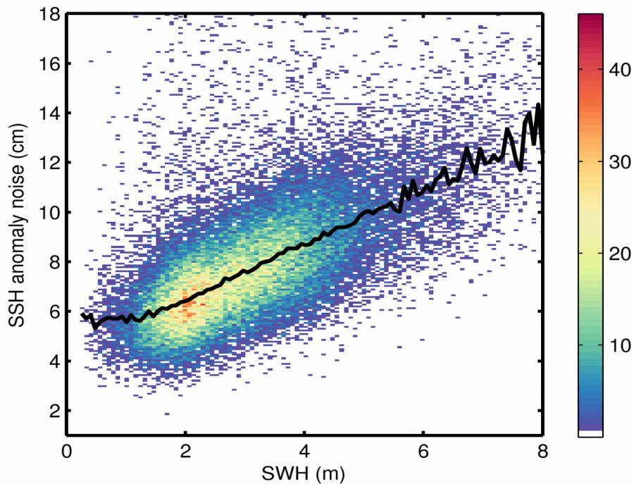
Figure 9. 2D histogram showing flag-valid SSH anomaly noise as a function of SWH for 02/05/2020. The black line denotes the median SSH anomaly noise as a function of SWH.
