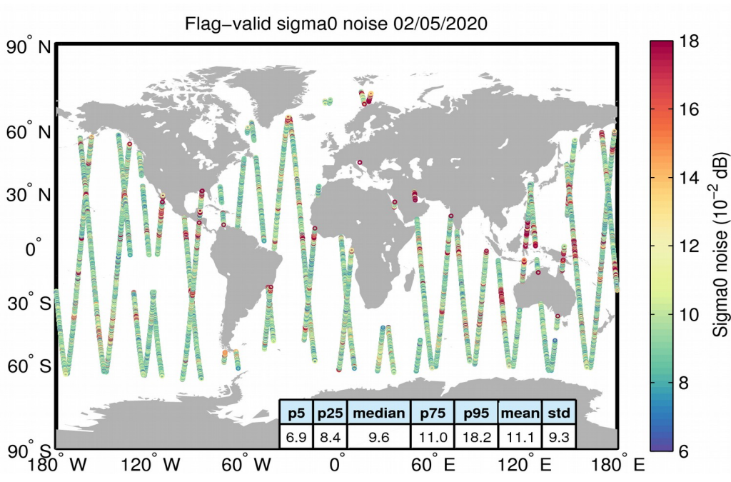
Figure 26. Geographical distribution of flag-valid 20-Hz sigma0 measurement noise over oceans and lakes for 02/05/2020. The statistical values shown in the table refer to the sigma0 noise and are calculated over all measurements shown in the figure.
