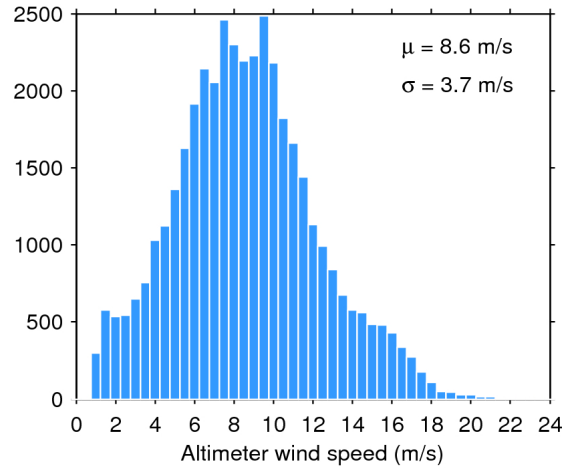
Figure 33. Histogram of flag-valid wind over oceans and lakes for 02/05/2020. The mean ( \mu ) and standard deviation ( \sigma ) are also shown. Note that values larger than 24 m/s are excluded from the histogram for the sake of readability but not from the computation of \mu and \sigma .
