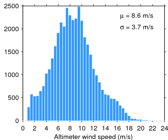
Figure 35. Histogram of science-valid wind over oceans and lakes for 02/05/2020. The mean ( \mu ) and standard deviation ( \sigma ) are also shown. Note that values larger than 24 m/s are excluded from the histogram for the sake of readability but not from the computation of \mu and \sigma .
