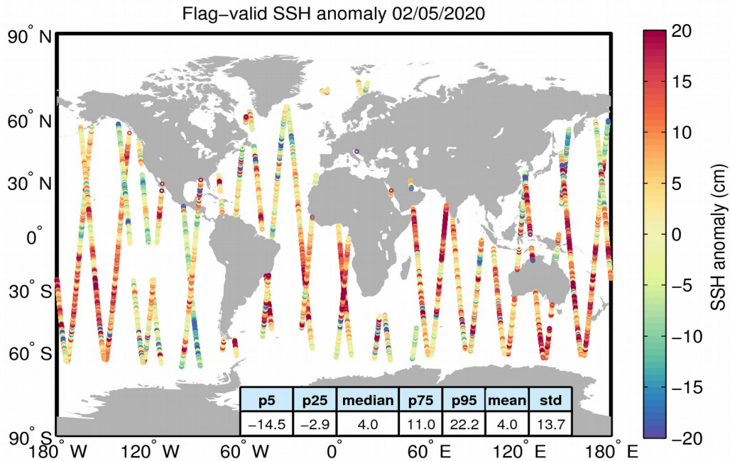
Figure 5. Geographical distribution of flag-valid 1-Hz SSH anomaly data over oceans and lakes for 02/05/2020. The statistical values shown in the table refer to the SSH anomaly in cm and are calculated over all measurements shown in the figure.
