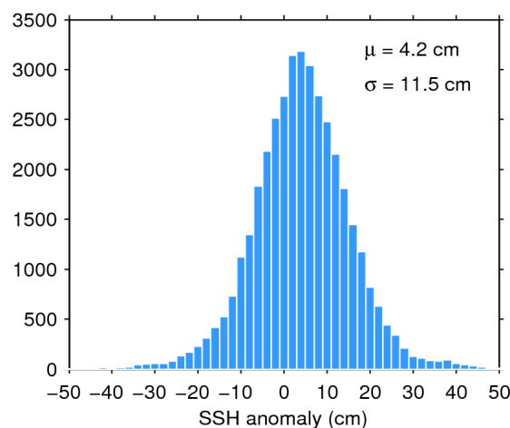
Figure 11. Histogram of science-valid SSH anomaly over oceans and lakes for 02/05/2020. The mean ( \mu ) and standard deviation ( \sigma ) are also shown. Note that values outside [-50 50] cm are excluded from the histogram for the sake of readability but not from the computation of \mu and \sigma .
