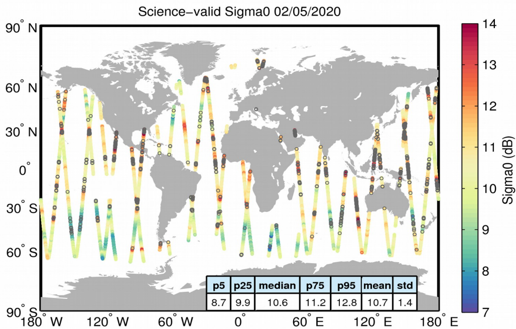
Figure 27. Geographical distribution of science-valid sigma0 data over oceans and lakes for 02/05/2020. The statistical values shown in the table refer to the sigma0 in dB and are calculated over all measurements shown in the figure. Gray circles denote records that have been rejected based on the editing criteria described in Table 4.
