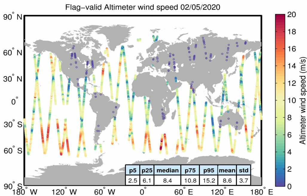
Figure 31. Geographical distribution of flag-valid wind data over oceans and lakes for 02/05/2020. The statistical values shown in the table refer to the wind in m/s and are calculated over all measurements shown in the figure.
