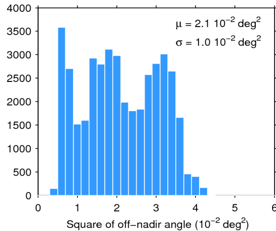
Figure 39. Histogram of flag-valid mispointing over oceans and lakes for 02/05/2020. The mean ( \mu ) and standard deviation ( \sigma ) are also shown. Note that values larger than 6 \cdot 10^{-2} \text{ deg}^2 are excluded from the histogram for the sake of readability but not from the computation of \mu and \sigma .
