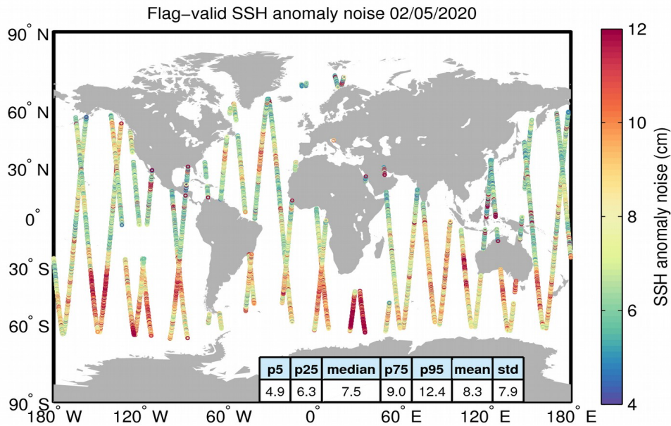
Figure 8. Geographical distribution of flag-valid 20-Hz SSH anomaly measurement noise over oceans and lakes for 02/05/2020. The statistical values shown in the table refer to the SSH anomaly noise and are calculated over all measurements shown in the figure.
