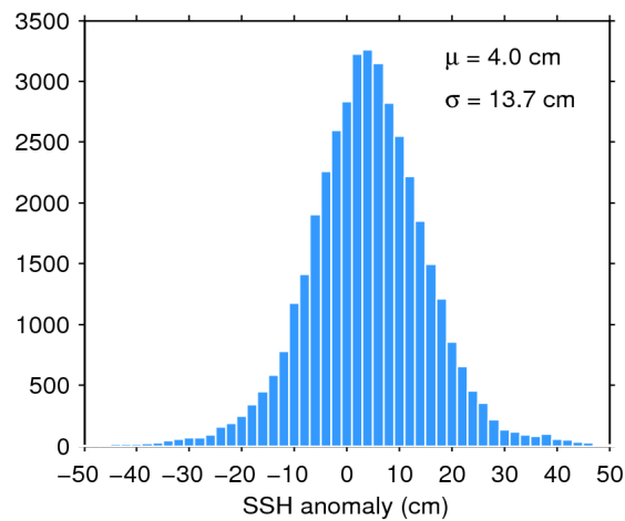
Figure 7. Histogram of flag-valid SSH anomaly over oceans and lakes for 02/05/2020. The mean ( \mu ) and standard deviation ( \sigma ) are also shown. Note that values outside [-50 50] cm are excluded from the histogram for the sake of readability but not from the computation of \mu and \sigma .
