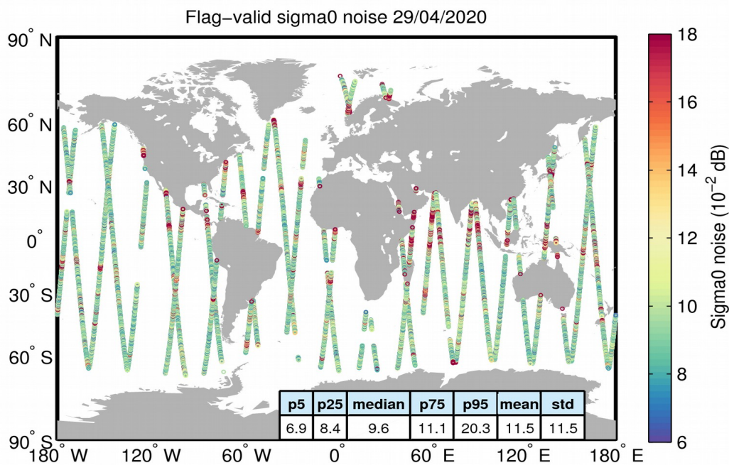
Figure 26. Geographical distribution of flag-valid 20-Hz sigma0 measurement noise over oceans and lakes for 29/04/2020. The statistical values shown in the table refer to the sigma0 noise and are calculated over all measurements shown in the figure.
