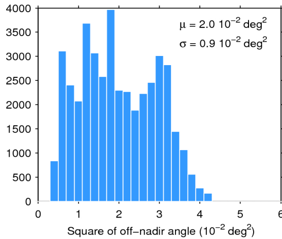
Figure 39. Histogram of flag-valid mispointing over oceans and lakes for 29/04/2020. The mean ( \mu ) and standard deviation ( \sigma ) are also shown. Note that values larger than 6 \cdot 10^{-2} \text{ deg}^2 are excluded from the histogram for the sake of readability but not from the computation of \mu and \sigma .
