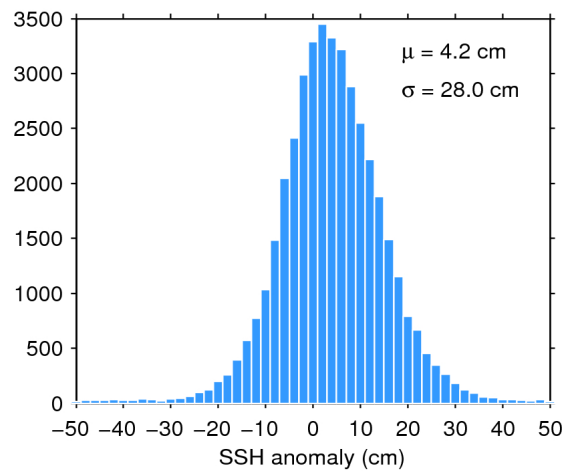
Figure 7. Histogram of flag-valid SSH anomaly over oceans and lakes for 29/04/2020. The mean ( \mu ) and standard deviation ( \sigma ) are also shown. Note that values outside [-50\ 50] cm are excluded from the histogram for the sake of readability but not from the computation of \mu and \sigma .
