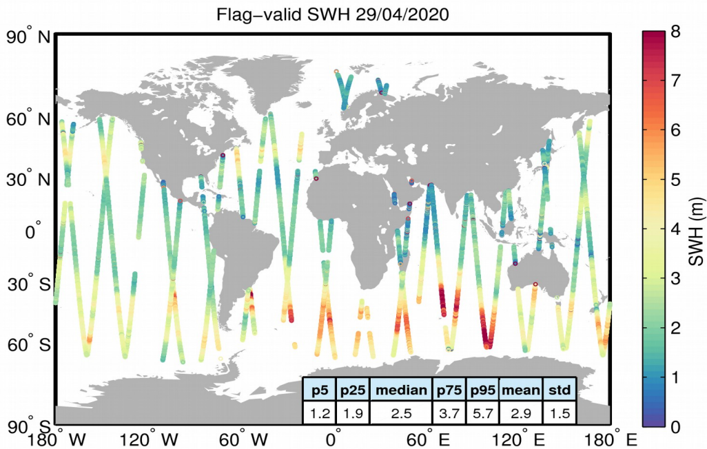
Figure 15. Geographical distribution of flag-valid SWH data over oceans and lakes for 29/04/2020. The statistical values shown in the table refer to the SWH in m and are calculated over all measurements shown in the figure.
