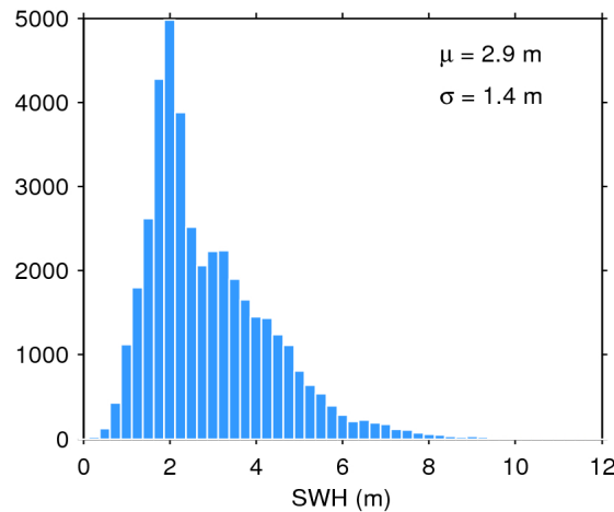
Figure 20. Histogram of science-valid SWH over oceans and lakes for 29/04/2020. The mean ( \mu ) and standard deviation ( \sigma ) are also shown. Note that values larger than 12 m are excluded from the histogram for the sake of readability but not from the computation of \mu and \sigma .
