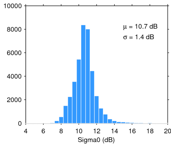
Figure 28. Histogram of science-valid sigma0 over oceans and lakes for 29/04/2020. The mean ( \mu ) and standard deviation ( \sigma ) are also shown. Note that values outside [4 20] dB are excluded from the histogram for the sake of readability but not from the computation of \mu and \sigma .
