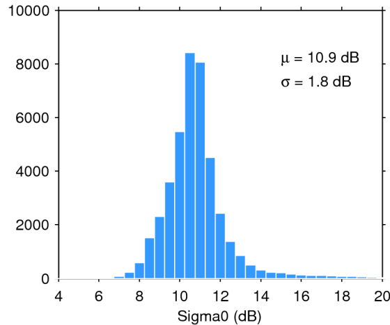
Figure 25. Histogram of flag-valid sigma0 over oceans and lakes for 29/04/2020. The mean ( \mu ) and standard deviation ( \sigma ) are also shown. Note that values outside [4 20] dB are excluded from the histogram for the sake of readability but not from the computation of \mu and \sigma .
