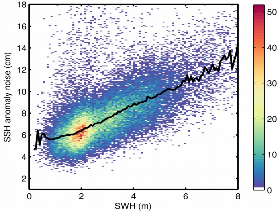
Figure 9. 2D histogram showing flag-valid SSH anomaly noise as a function of SWH for 29/04/2020. The black line denotes the median SSH anomaly noise as a function of SWH.
