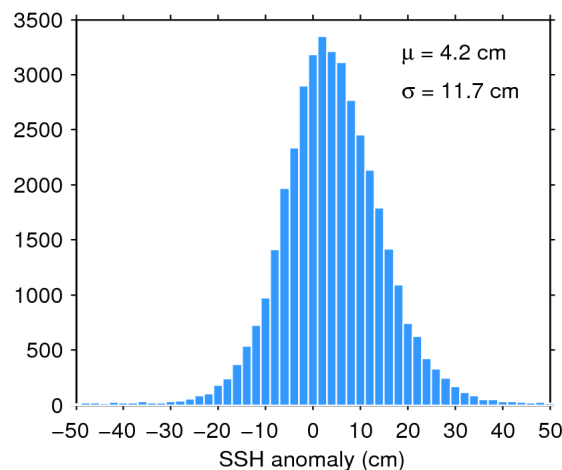
Figure 11. Histogram of science-valid SSH anomaly over oceans and lakes for 29/04/2020. The mean ( \mu ) and standard deviation ( \sigma ) are also shown. Note that values outside [-50 50] cm are excluded from the histogram for the sake of readability but not from the computation of \mu and \sigma .
