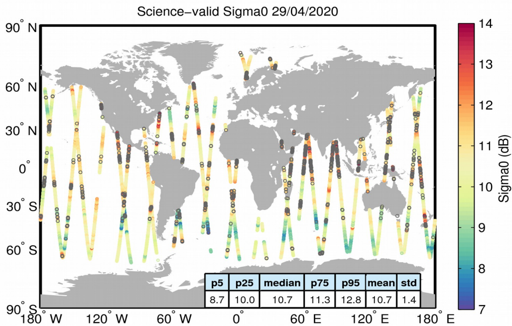
Figure 27. Geographical distribution of science-valid sigma0 data over oceans and lakes for 29/04/2020. The statistical values shown in the table refer to the sigma0 in dB and are calculated over all measurements shown in the figure. Gray circles denote records that have been rejected based on the editing criteria described in Table 4.
