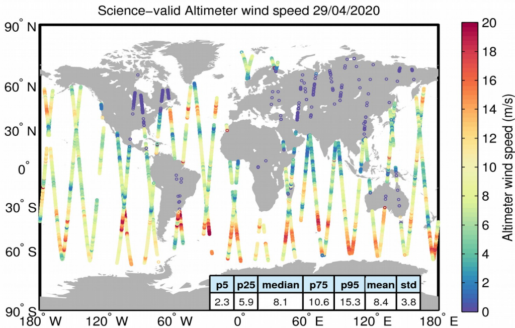
Figure 34. Geographical distribution of science-valid wind data over oceans and lakes for 29/04/2020. The statistical values shown in the table refer to the wind in m/s and are calculated over all measurements shown in the figure. Gray circles denote records that have been rejected based on the editing criteria described in Table 5.
