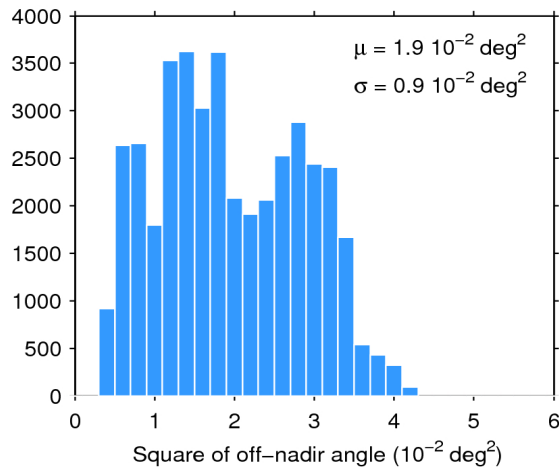
Figure 39. Histogram of flag-valid mispointing over oceans and lakes for 28/04/2020. The mean ( \mu ) and standard deviation ( \sigma ) are also shown. Note that values larger than 6 \cdot 10^{-2} \text{ deg}^2 are excluded from the histogram for the sake of readability but not from the computation of \mu and \sigma .
