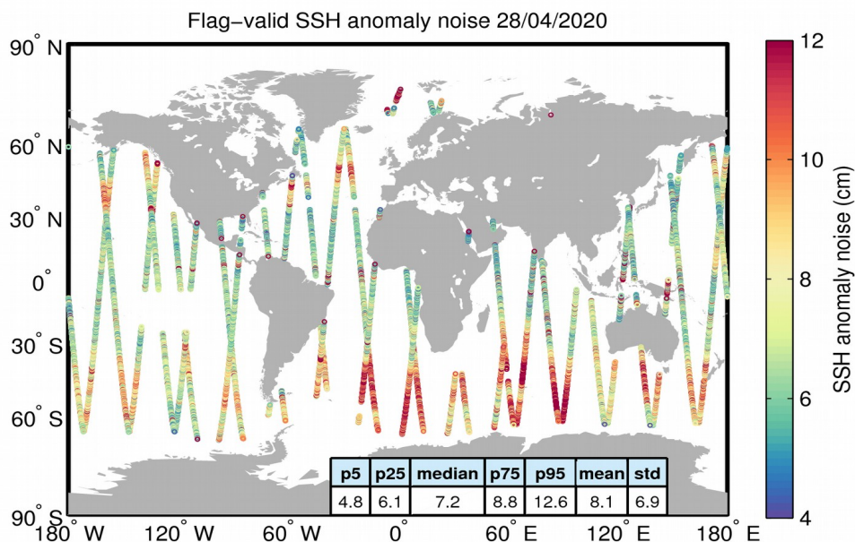
Figure 8. Geographical distribution of flag-valid 20-Hz SSH anomaly measurement noise over oceans and lakes for 28/04/2020. The statistical values shown in the table refer to the SSH anomaly noise and are calculated over all measurements shown in the figure.
