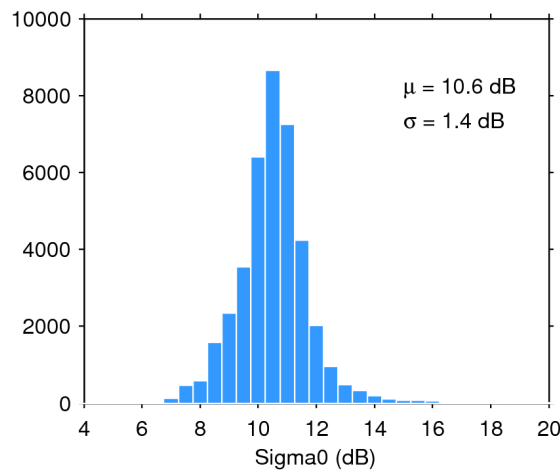
Figure 28. Histogram of science-valid sigma0 over oceans and lakes for 28/04/2020. The mean ( \mu ) and standard deviation ( \sigma ) are also shown. Note that values outside [4 20] dB are excluded from the histogram for the sake of readability but not from the computation of \mu and \sigma .
