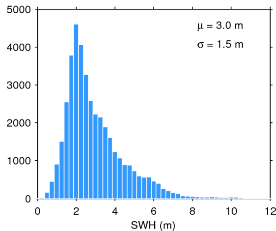
Figure 20. Histogram of science-valid SWH over oceans and lakes for 28/04/2020. The mean ( \mu ) and standard deviation ( \sigma ) are also shown. Note that values larger than 12 m are excluded from the histogram for the sake of readability but not from the computation of \mu and \sigma .
