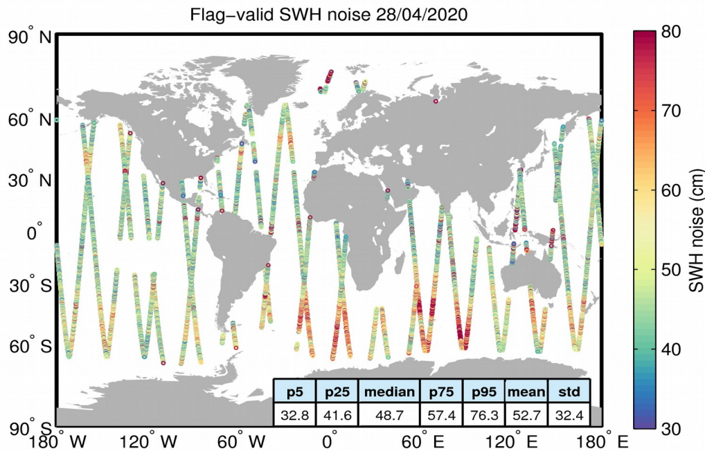
Figure 18. Geographical distribution of flag-valid 20-Hz SWH measurement noise over oceans and lakes for 28/04/2020. The statistical values shown in the figure refer to the SWH noise and are calculated over all measurements shown in the figure.
