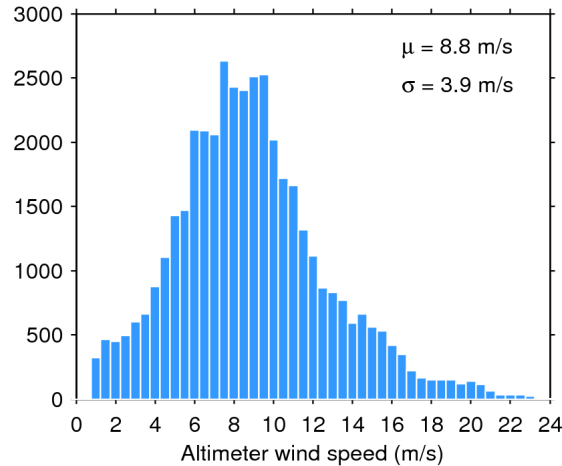
Figure 33. Histogram of flag-valid wind over oceans and lakes for 28/04/2020. The mean ( \mu ) and standard deviation ( \sigma ) are also shown. Note that values larger than 24 m/s are excluded from the histogram for the sake of readability but not from the computation of \mu and \sigma .
