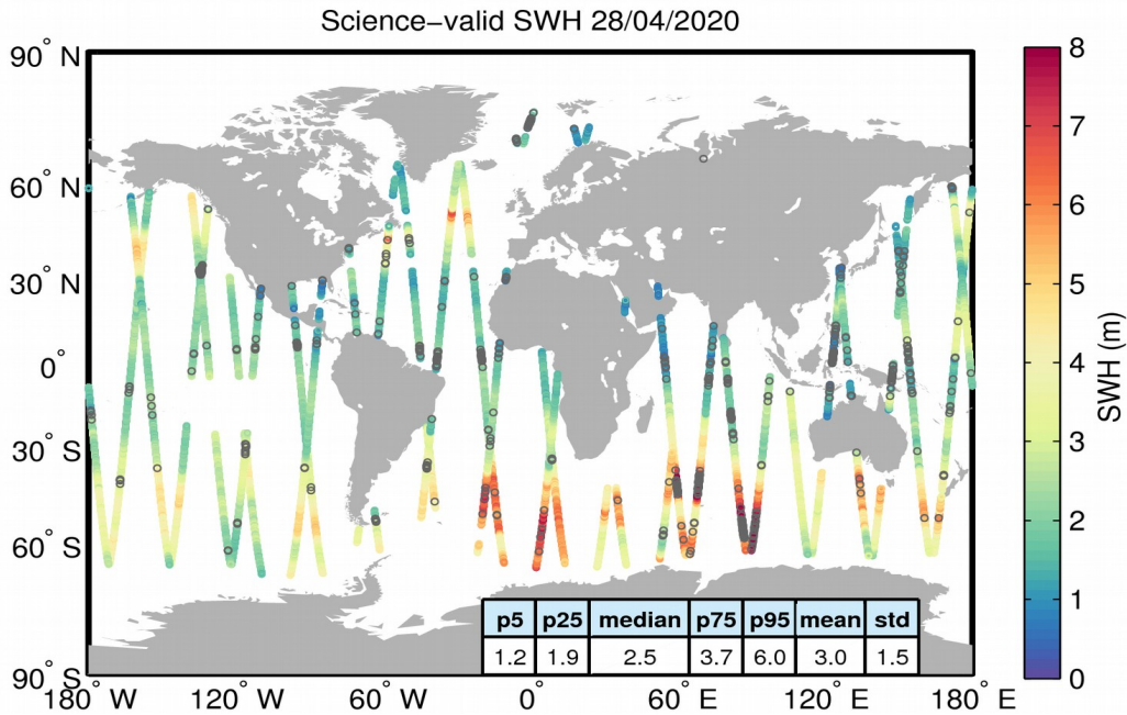
Figure 19. Geographical distribution of science-valid SWH data over oceans and lakes for 28/04/2020. The statistical values shown in the table refer to the SWH in m and are calculated over all measurements shown in the figure. Gray circles denote records that have been rejected based on the editing criteria described in Table 3.
