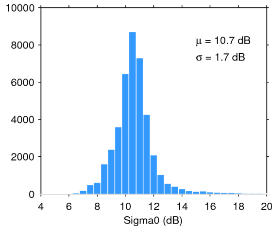
Figure 25. Histogram of flag-valid sigma0 over oceans and lakes for 28/04/2020. The mean ( \mu ) and standard deviation ( \sigma ) are also shown. Note that values outside [4 20] dB are excluded from the histogram for the sake of readability but not from the computation of \mu and \sigma .
