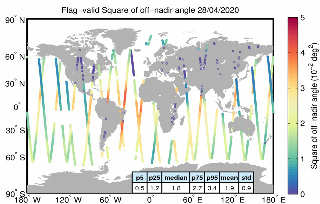
Figure 37. Geographical distribution of flag-valid mispointing data over oceans and lakes for 28/04/2020. The statistical values shown in the table refer to the mispointing in 10^{-2} \text{ deg}^2 and are calculated over all measurements shown in the figure.
