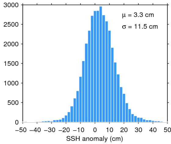
Figure 11. Histogram of science-valid SSH anomaly over oceans and lakes for 28/04/2020. The mean ( \mu ) and standard deviation ( \sigma ) are also shown. Note that values outside [-50 50] cm are excluded from the histogram for the sake of readability but not from the computation of \mu and \sigma .
