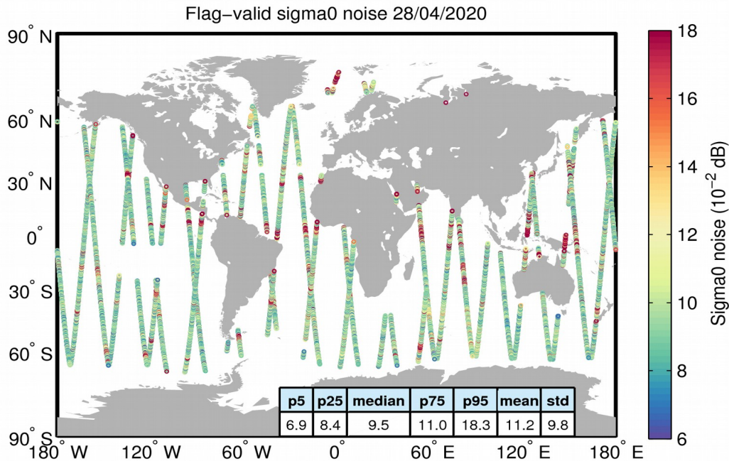
Figure 26. Geographical distribution of flag-valid 20-Hz sigma0 measurement noise over oceans and lakes for 28/04/2020. The statistical values shown in the table refer to the sigma0 noise and are calculated over all measurements shown in the figure.
