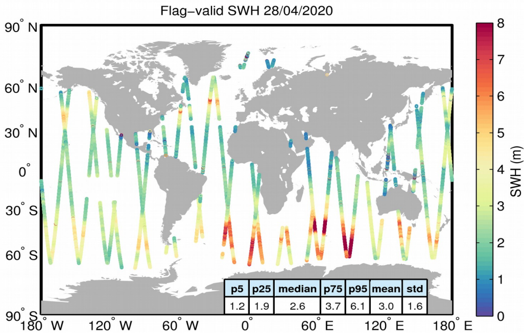
Figure 15. Geographical distribution of flag-valid SWH data over oceans and lakes for 28/04/2020. The statistical values shown in the table refer to the SWH in m and are calculated over all measurements shown in the figure.
