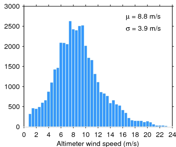
Figure 35. Histogram of science-valid wind over oceans and lakes for 28/04/2020. The mean ( \mu ) and standard deviation ( \sigma ) are also shown. Note that values larger than 24 m/s are excluded from the histogram for the sake of readability but not from the computation of \mu and \sigma .
