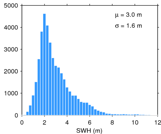
Figure 17. Histogram of flag-valid SWH over oceans and lakes for 28/04/2020. The mean ( \mu ) and standard deviation ( \sigma ) are also shown. Note that values larger than 12 m are excluded from the histogram for the sake of readability but not from the computation of \mu and \sigma .
