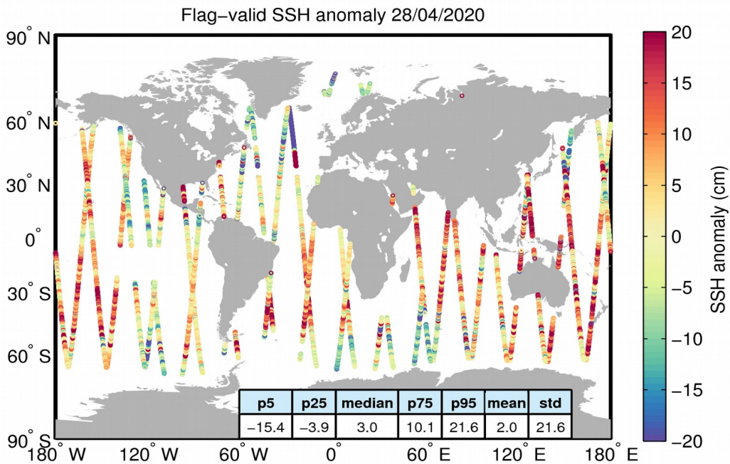
Figure 5. Geographical distribution of flag-valid 1-Hz SSH anomaly data over oceans and lakes for 28/04/2020. The statistical values shown in the table refer to the SSH anomaly in cm and are calculated over all measurements shown in the figure.
