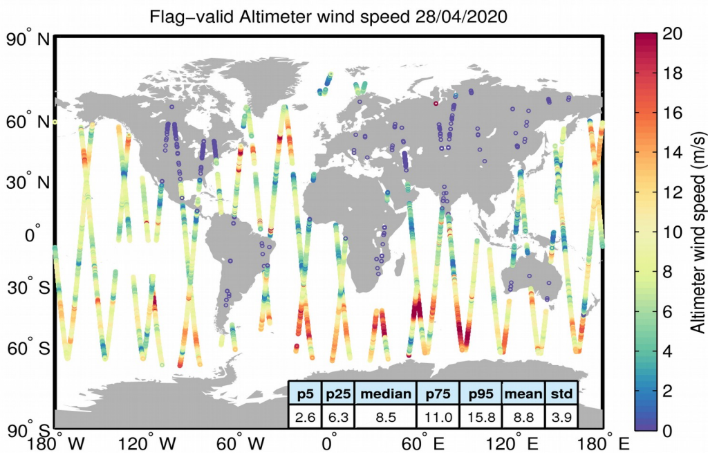
Figure 31. Geographical distribution of flag-valid wind data over oceans and lakes for 28/04/2020. The statistical values shown in the table refer to the wind in m/s and are calculated over all measurements shown in the figure.
