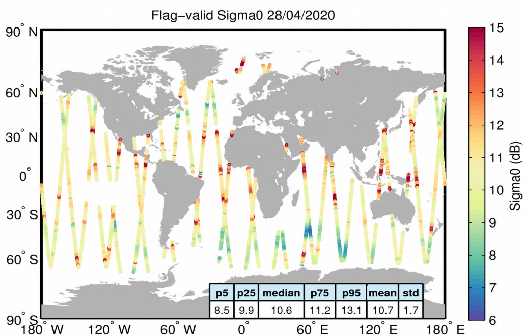
Figure 23. Geographical distribution of flag-valid sigma0 data over oceans and lakes for 28/04/2020. The statistical values shown in the table refer to the sigma0 in dB and are calculated over all measurements shown in the figure.
