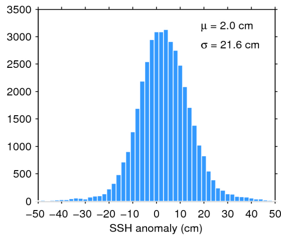
Figure 7. Histogram of flag-valid SSH anomaly over oceans and lakes for 28/04/2020. The mean ( \mu ) and standard deviation ( \sigma ) are also shown. Note that values outside [-50\ 50] cm are excluded from the histogram for the sake of readability but not from the computation of \mu and \sigma .
