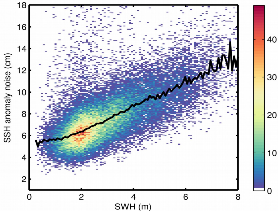
Figure 9. 2D histogram showing flag-valid SSH anomaly noise as a function of SWH for 28/04/2020. The black line denotes the median SSH anomaly noise as a function of SWH.
