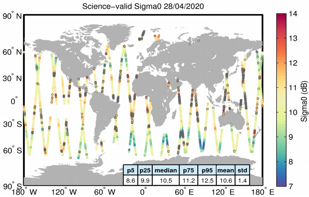
Figure 27. Geographical distribution of science-valid sigma0 data over oceans and lakes for 28/04/2020. The statistical values shown in the table refer to the sigma0 in dB and are calculated over all measurements shown in the figure. Gray circles denote records that have been rejected based on the editing criteria described in Table 4.
