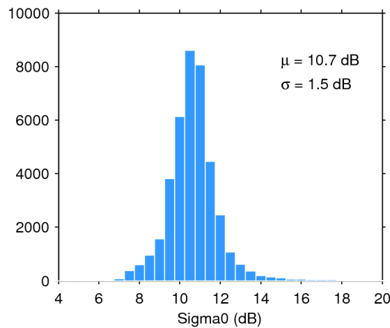
Figure 28. Histogram of science-valid sigma0 over oceans and lakes for 27/04/2020. The mean ( \mu ) and standard deviation ( \sigma ) are also shown. Note that values outside [4 20] dB are excluded from the histogram for the sake of readability but not from the computation of \mu and \sigma .
