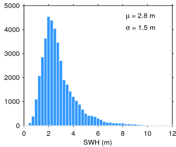
Figure 17. Histogram of flag-valid SWH over oceans and lakes for 27/04/2020. The mean ( \mu ) and standard deviation ( \sigma ) are also shown. Note that values larger than 12 m are excluded from the histogram for the sake of readability but not from the computation of \mu and \sigma .
