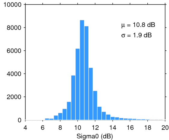
Figure 25. Histogram of flag-valid sigma0 over oceans and lakes for 27/04/2020. The mean ( \mu ) and standard deviation ( \sigma ) are also shown. Note that values outside [4 20] dB are excluded from the histogram for the sake of readability but not from the computation of \mu and \sigma .
