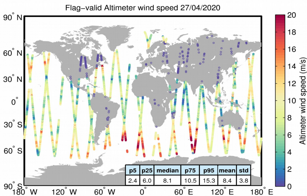
Figure 31. Geographical distribution of flag-valid wind data over oceans and lakes for 27/04/2020. The statistical values shown in the table refer to the wind in m/s and are calculated over all measurements shown in the figure.
