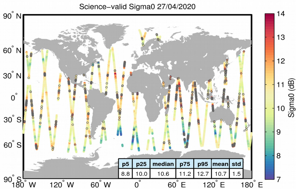
Figure 27. Geographical distribution of science-valid sigma0 data over oceans and lakes for 27/04/2020. The statistical values shown in the table refer to the sigma0 in dB and are calculated over all measurements shown in the figure. Gray circles denote records that have been rejected based on the editing criteria described in Table 4.
