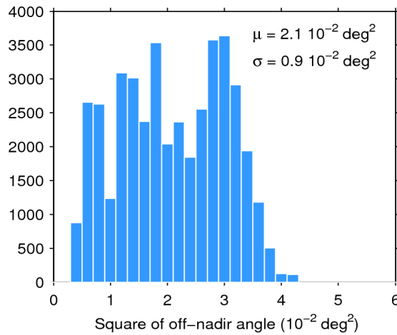
Figure 39. Histogram of flag-valid mispointing over oceans and lakes for 27/04/2020. The mean ( \mu ) and standard deviation ( \sigma ) are also shown. Note that values larger than 6 \cdot 10^{-2} \text{ deg}^2 are excluded from the histogram for the sake of readability but not from the computation of \mu and \sigma .
