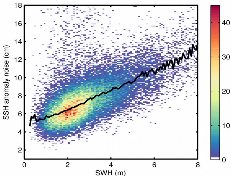
Figure 9. 2D histogram showing flag-valid SSH anomaly noise as a function of SWH for 27/04/2020. The black line denotes the median SSH anomaly noise as a function of SWH.
