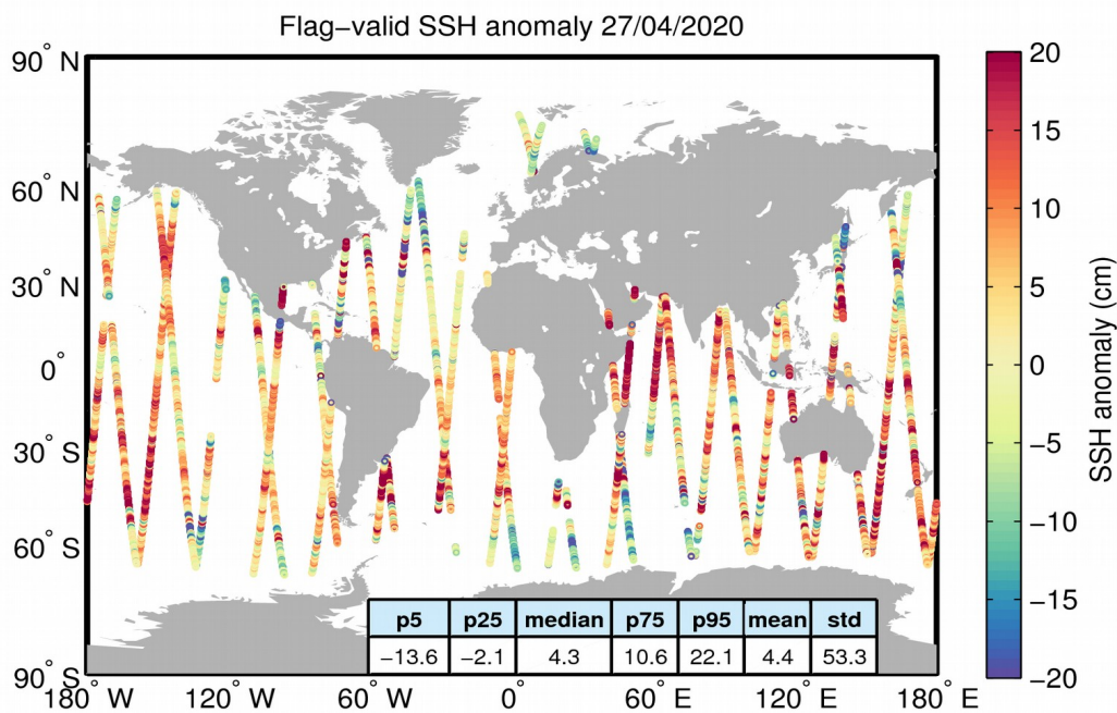
Figure 5. Geographical distribution of flag-valid 1-Hz SSH anomaly data over oceans and lakes for 27/04/2020. The statistical values shown in the table refer to the SSH anomaly in cm and are calculated over all measurements shown in the figure.
