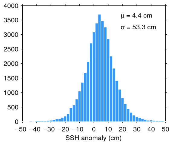
Figure 7. Histogram of flag-valid SSH anomaly over oceans and lakes for 27/04/2020. The mean ( \mu ) and standard deviation ( \sigma ) are also shown. Note that values outside [-50 50] cm are excluded from the histogram for the sake of readability but not from the computation of \mu and \sigma .
