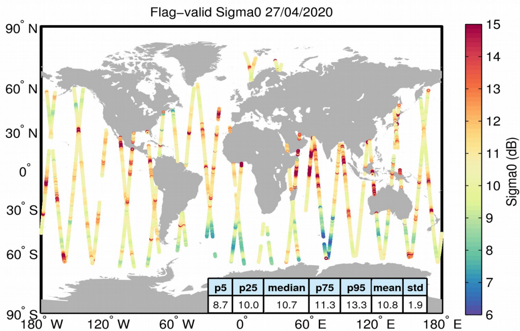
Figure 23. Geographical distribution of flag-valid sigma0 data over oceans and lakes for 27/04/2020. The statistical values shown in the table refer to the sigma0 in dB and are calculated over all measurements shown in the figure.
