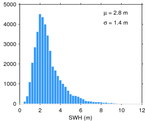
Figure 20. Histogram of science-valid SWH over oceans and lakes for 27/04/2020. The mean ( \mu ) and standard deviation ( \sigma ) are also shown. Note that values larger than 12 m are excluded from the histogram for the sake of readability but not from the computation of \mu and \sigma .
