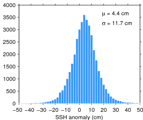
Figure 11. Histogram of science-valid SSH anomaly over oceans and lakes for 27/04/2020. The mean ( \mu ) and standard deviation ( \sigma ) are also shown. Note that values outside [-50 50] cm are excluded from the histogram for the sake of readability but not from the computation of \mu and \sigma .
