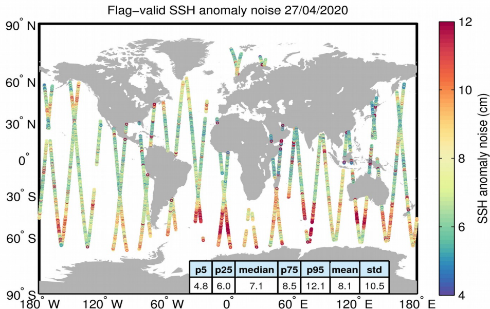
Figure 8. Geographical distribution of flag-valid 20-Hz SSH anomaly measurement noise over oceans and lakes for 27/04/2020. The statistical values shown in the table refer to the SSH anomaly noise and are calculated over all measurements shown in the figure.
