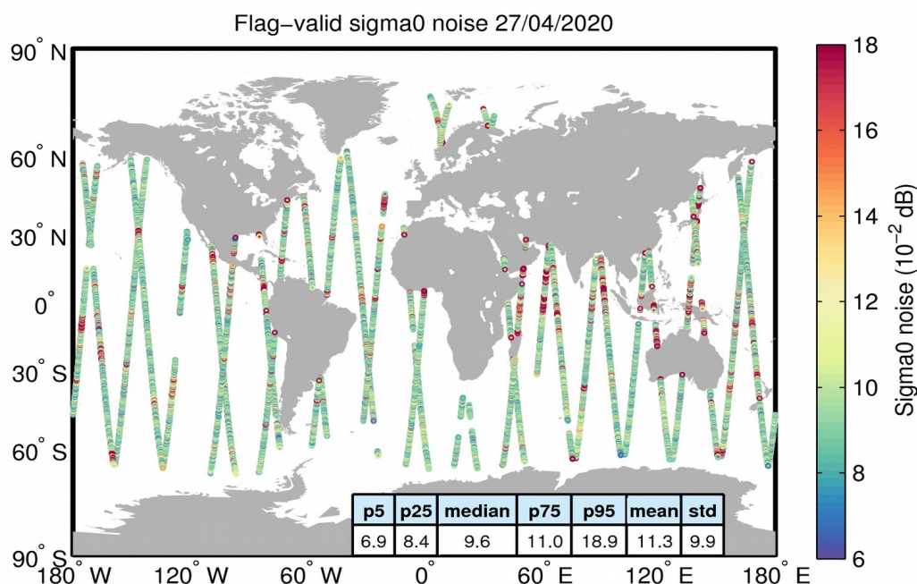
Figure 26. Geographical distribution of flag-valid 20-Hz sigma0 measurement noise over oceans and lakes for 27/04/2020. The statistical values shown in the table refer to the sigma0 noise and are calculated over all measurements shown in the figure.
