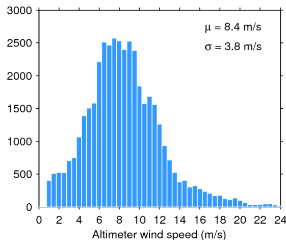
Figure 35. Histogram of science-valid wind over oceans and lakes for 27/04/2020. The mean ( \mu ) and standard deviation ( \sigma ) are also shown. Note that values larger than 24 m/s are excluded from the histogram for the sake of readability but not from the computation of \mu and \sigma .
