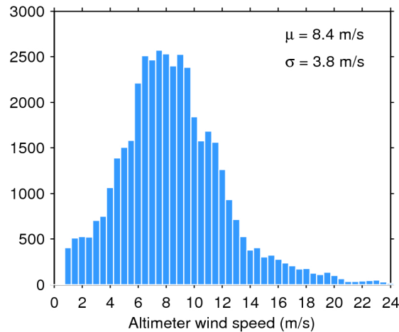
Figure 33. Histogram of flag-valid wind over oceans and lakes for 27/04/2020. The mean ( \mu ) and standard deviation ( \sigma ) are also shown. Note that values larger than 24 m/s are excluded from the histogram for the sake of readability but not from the computation of \mu and \sigma .
