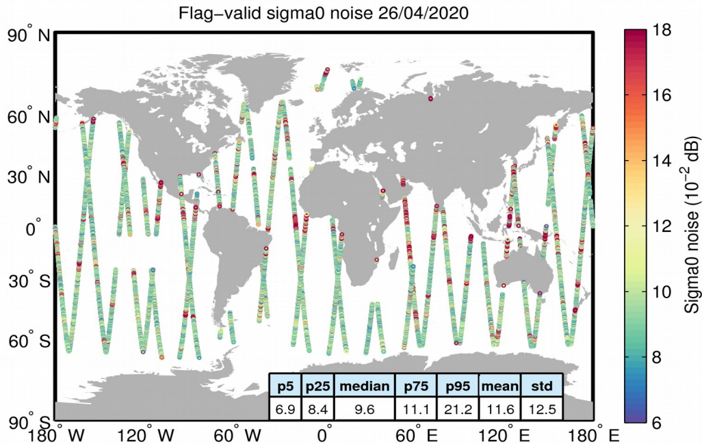
Figure 26. Geographical distribution of flag-valid 20-Hz sigma0 measurement noise over oceans and lakes for 26/04/2020. The statistical values shown in the table refer to the sigma0 noise and are calculated over all measurements shown in the figure.
