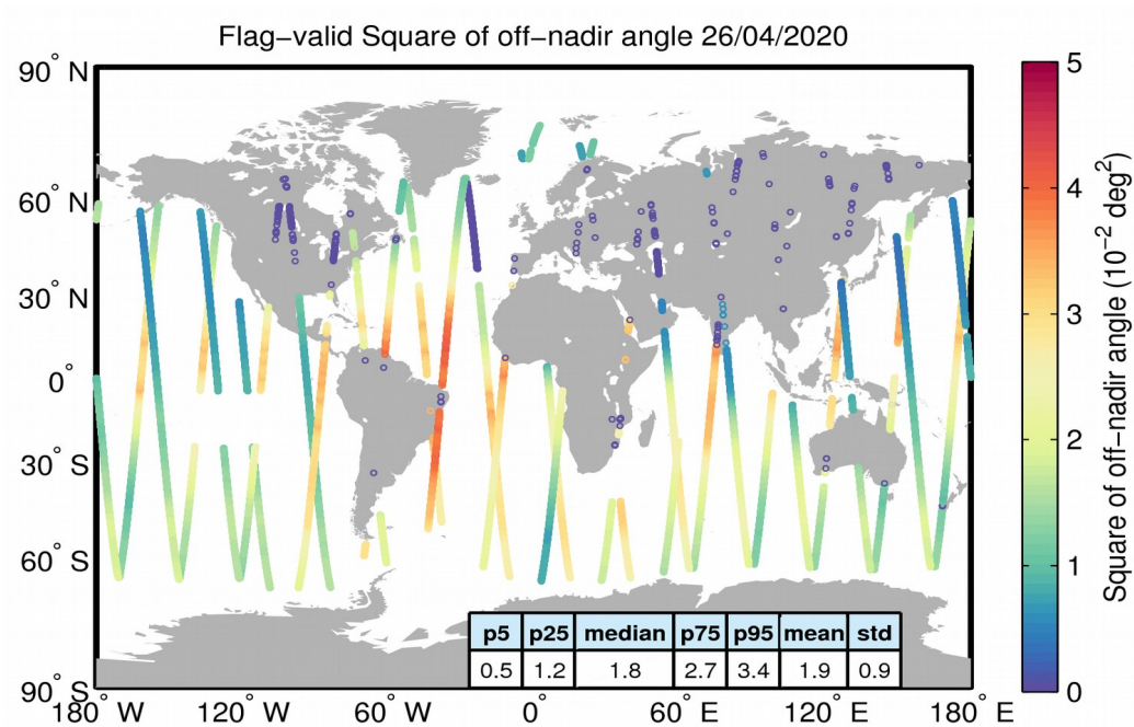
Figure 37. Geographical distribution of flag-valid mispointing data over oceans and lakes for 26/04/2020. The statistical values shown in the table refer to the mispointing in 10^{-2} \text{ deg}^2 and are calculated over all measurements shown in the figure.
