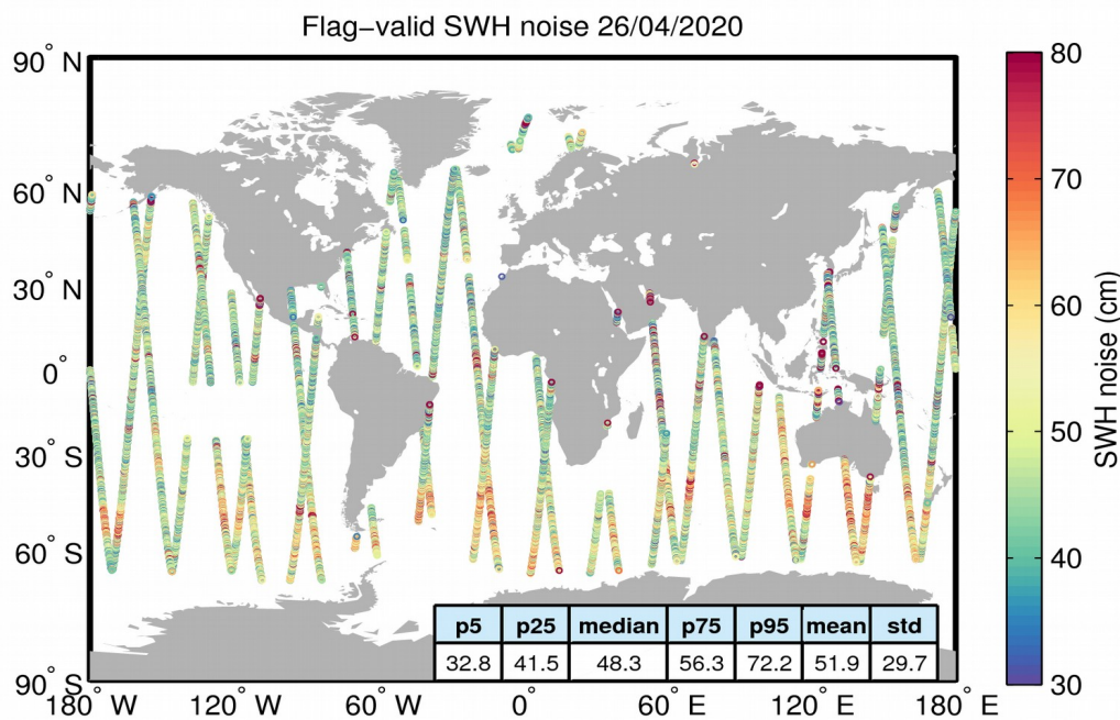
Figure 18. Geographical distribution of flag-valid 20-Hz SWH measurement noise over oceans and lakes for 26/04/2020. The statistical values shown in the figure refer to the SWH noise and are calculated over all measurements shown in the figure.
