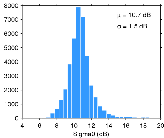
Figure 28. Histogram of science-valid sigma0 over oceans and lakes for 26/04/2020. The mean ( \mu ) and standard deviation ( \sigma ) are also shown. Note that values outside [4 20] dB are excluded from the histogram for the sake of readability but not from the computation of \mu and \sigma .
