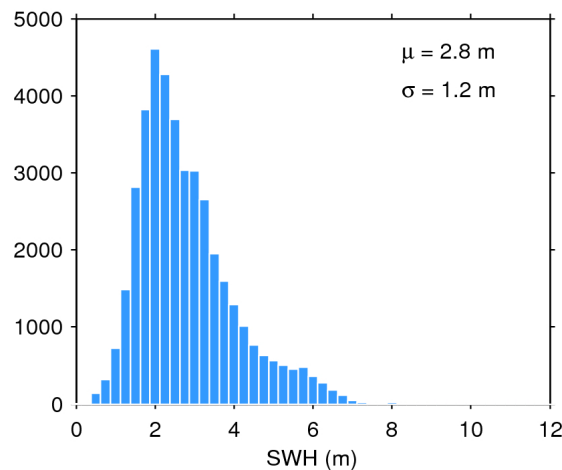
Figure 20. Histogram of science-valid SWH over oceans and lakes for 26/04/2020. The mean ( \mu ) and standard deviation ( \sigma ) are also shown. Note that values larger than 12 m are excluded from the histogram for the sake of readability but not from the computation of \mu and \sigma .
