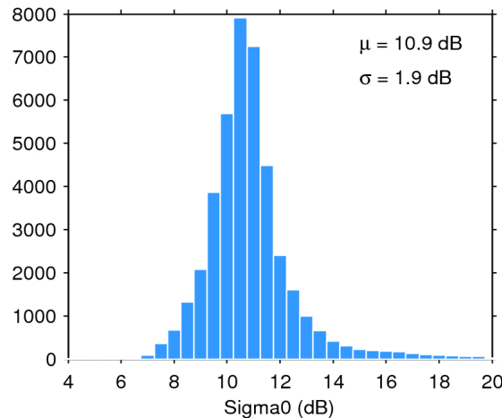
Figure 25. Histogram of flag-valid sigma0 over oceans and lakes for 26/04/2020. The mean ( \mu ) and standard deviation ( \sigma ) are also shown. Note that values outside [4 20] dB are excluded from the histogram for the sake of readability but not from the computation of \mu and \sigma .
