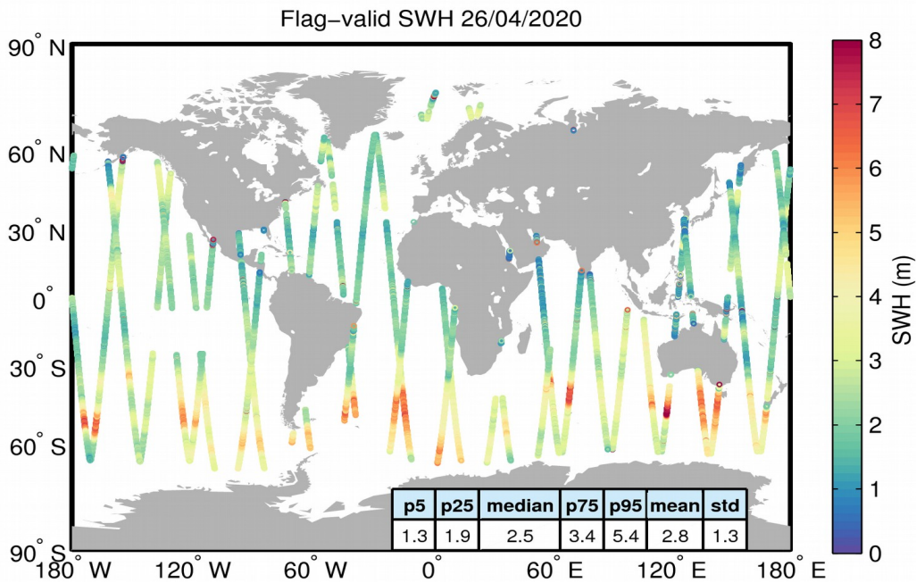
Figure 15. Geographical distribution of flag-valid SWH data over oceans and lakes for 26/04/2020. The statistical values shown in the table refer to the SWH in m and are calculated over all measurements shown in the figure.
