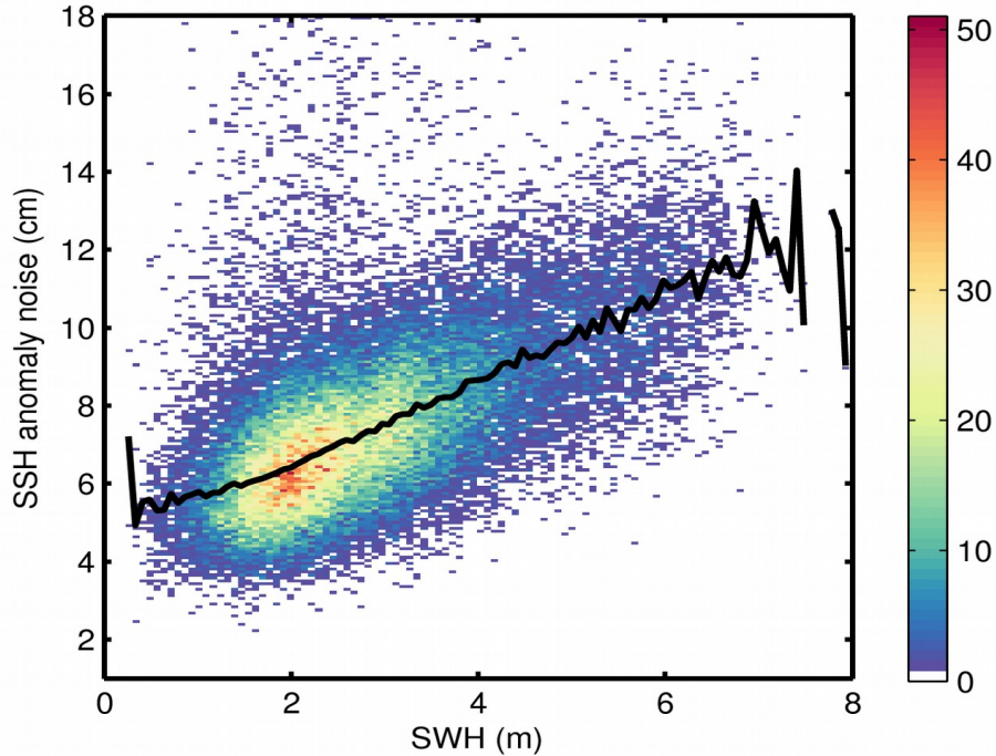
Figure 9. 2D histogram showing flag-valid SSH anomaly noise as a function of SWH for 26/04/2020. The black line denotes the median SSH anomaly noise as a function of SWH.
