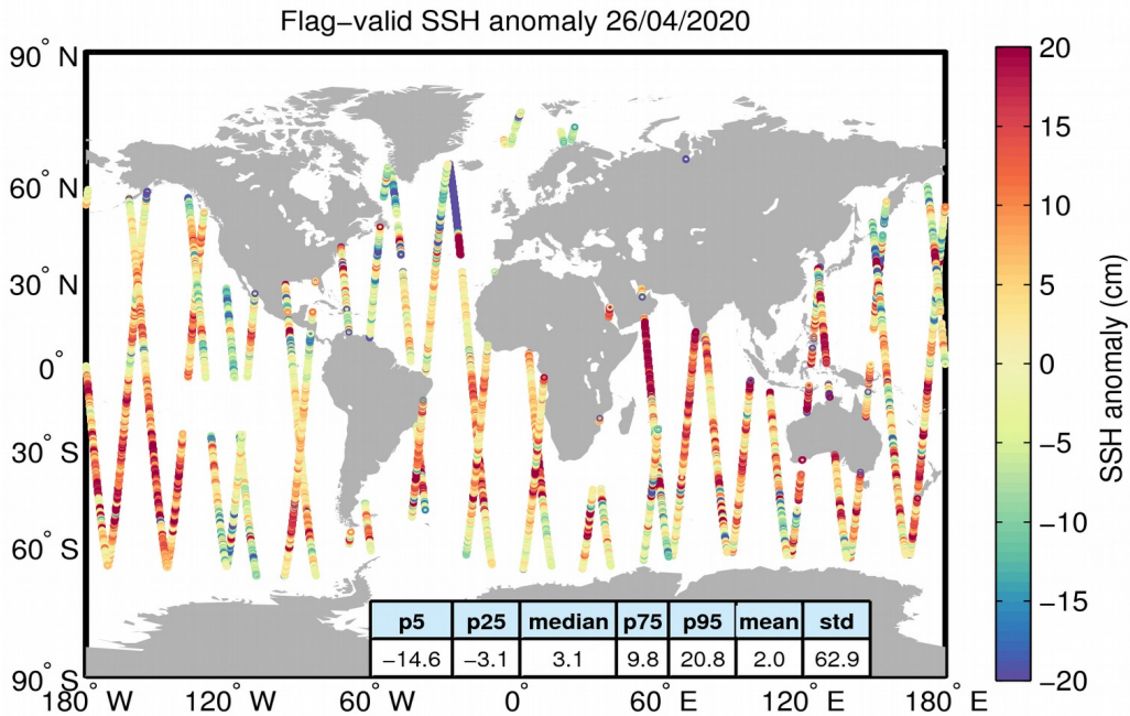
Figure 5. Geographical distribution of flag-valid 1-Hz SSH anomaly data over oceans and lakes for 26/04/2020. The statistical values shown in the table refer to the SSH anomaly in cm and are calculated over all measurements shown in the figure.
