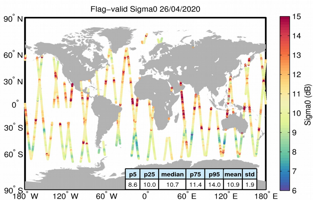
Figure 23. Geographical distribution of flag-valid sigma0 data over oceans and lakes for 26/04/2020. The statistical values shown in the table refer to the sigma0 in dB and are calculated over all measurements shown in the figure.
