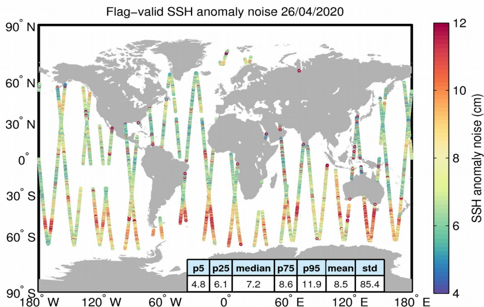
Figure 8. Geographical distribution of flag-valid 20-Hz SSH anomaly measurement noise over oceans and lakes for 26/04/2020. The statistical values shown in the table refer to the SSH anomaly noise and are calculated over all measurements shown in the figure.
