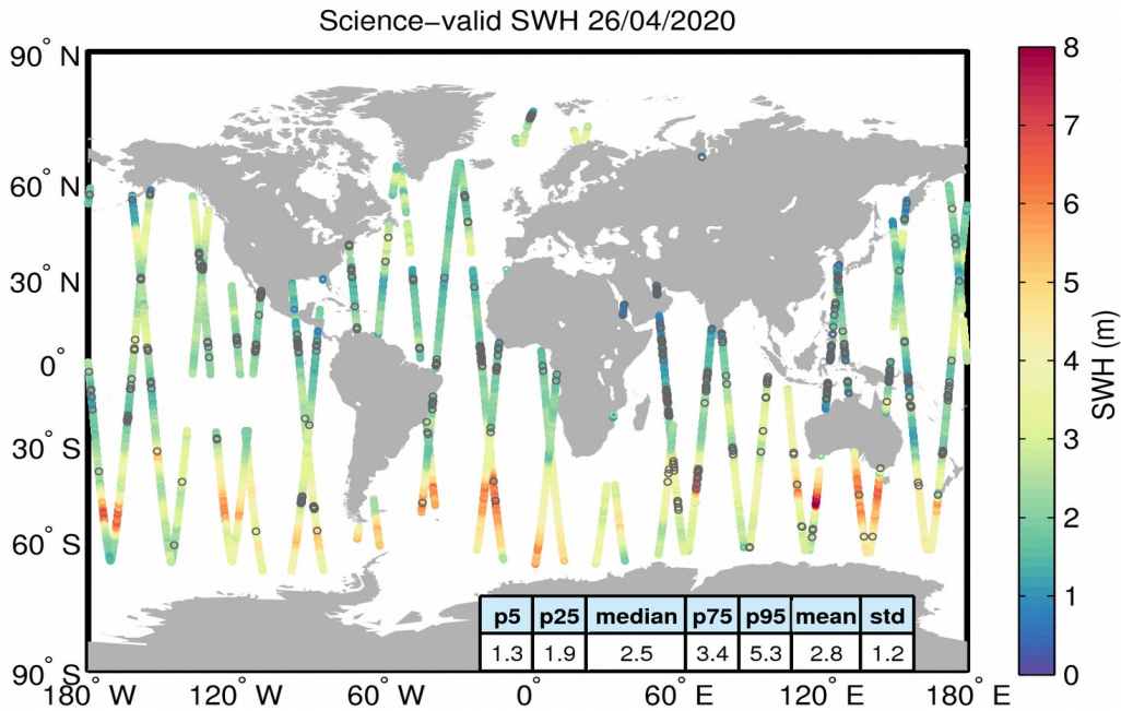
Figure 19. Geographical distribution of science-valid SWH data over oceans and lakes for 26/04/2020. The statistical values shown in the table refer to the SWH in m and are calculated over all measurements shown in the figure. Gray circles denote records that have been rejected based on the editing criteria described in Table 3.
