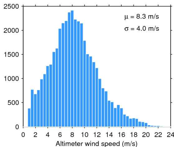
Figure 35. Histogram of science-valid wind over oceans and lakes for 26/04/2020. The mean ( \mu ) and standard deviation ( \sigma ) are also shown. Note that values larger than 24 m/s are excluded from the histogram for the sake of readability but not from the computation of \mu and \sigma .
