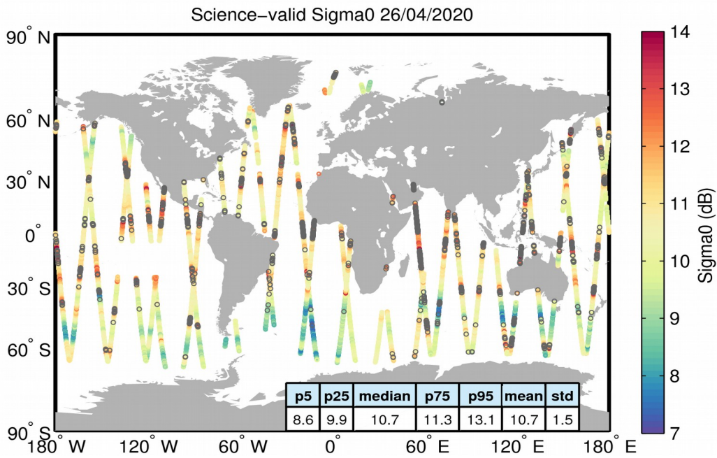
Figure 27. Geographical distribution of science-valid sigma0 data over oceans and lakes for 26/04/2020. The statistical values shown in the table refer to the sigma0 in dB and are calculated over all measurements shown in the figure. Gray circles denote records that have been rejected based on the editing criteria described in Table 4.
