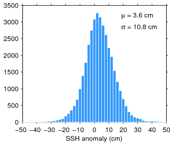
Figure 11. Histogram of science-valid SSH anomaly over oceans and lakes for 26/04/2020. The mean ( \mu ) and standard deviation ( \sigma ) are also shown. Note that values outside [-50 50] cm are excluded from the histogram for the sake of readability but not from the computation of \mu and \sigma .
