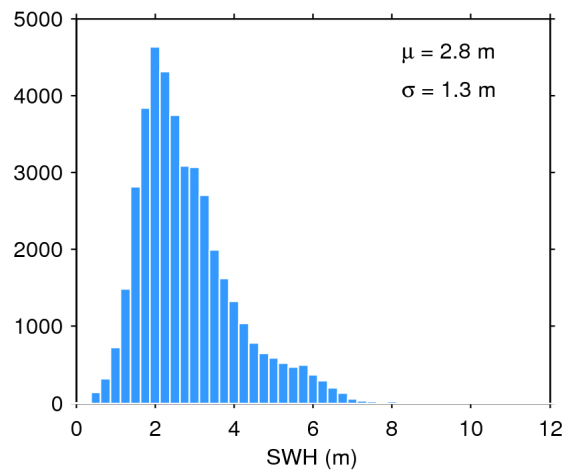
Figure 17. Histogram of flag-valid SWH over oceans and lakes for 26/04/2020. The mean ( \mu ) and standard deviation ( \sigma ) are also shown. Note that values larger than 12 m are excluded from the histogram for the sake of readability but not from the computation of \mu and \sigma .
