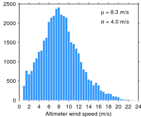
Figure 33. Histogram of flag-valid wind over oceans and lakes for 26/04/2020. The mean ( \mu ) and standard deviation ( \sigma ) are also shown. Note that values larger than 24 m/s are excluded from the histogram for the sake of readability but not from the computation of \mu and \sigma .
