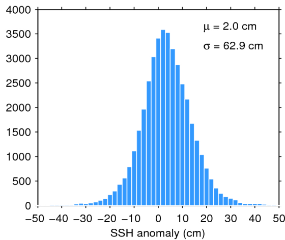
Figure 7. Histogram of flag-valid SSH anomaly over oceans and lakes for 26/04/2020. The mean ( \mu ) and standard deviation ( \sigma ) are also shown. Note that values outside [-50\ 50] cm are excluded from the histogram for the sake of readability but not from the computation of \mu and \sigma .
