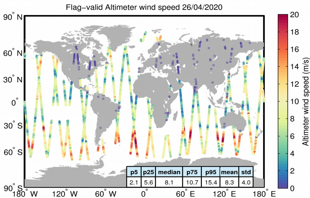
Figure 31. Geographical distribution of flag-valid wind data over oceans and lakes for 26/04/2020. The statistical values shown in the table refer to the wind in m/s and are calculated over all measurements shown in the figure.
