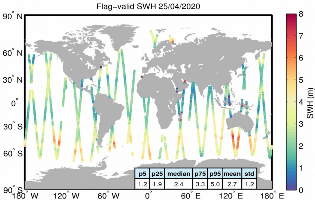
Figure 15. Geographical distribution of flag-valid SWH data over oceans and lakes for 25/04/2020. The statistical values shown in the table refer to the SWH in m and are calculated over all measurements shown in the figure.
