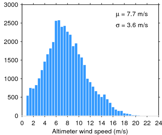
Figure 33. Histogram of flag-valid wind over oceans and lakes for 25/04/2020. The mean ( \mu ) and standard deviation ( \sigma ) are also shown. Note that values larger than 24 m/s are excluded from the histogram for the sake of readability but not from the computation of \mu and \sigma .
