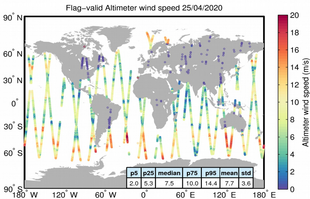
Figure 31. Geographical distribution of flag-valid wind data over oceans and lakes for 25/04/2020. The statistical values shown in the table refer to the wind in m/s and are calculated over all measurements shown in the figure.
