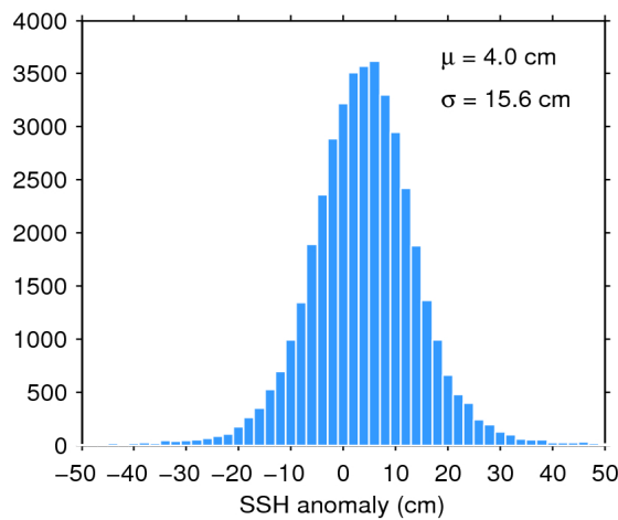
Figure 7. Histogram of flag-valid SSH anomaly over oceans and lakes for 25/04/2020. The mean ( \mu ) and standard deviation ( \sigma ) are also shown. Note that values outside [-50 50] cm are excluded from the histogram for the sake of readability but not from the computation of \mu and \sigma .
