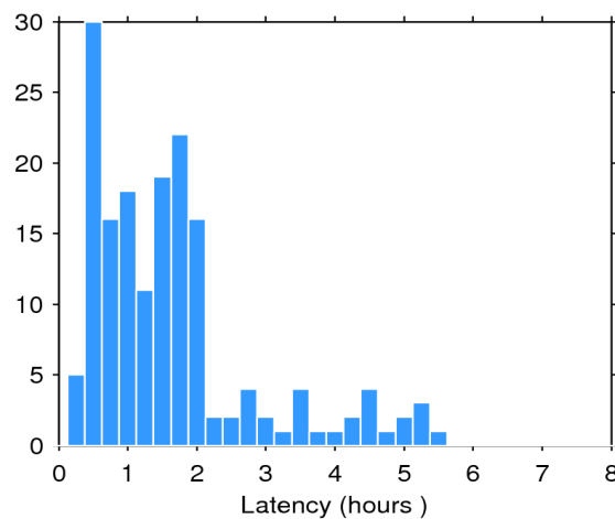
Figure 2. Histogram of the data latency for 25/04/2020. The y-axis denotes the number of files that are made available with a delay of x-hours with respect to the mean time of the records stored in the file.
