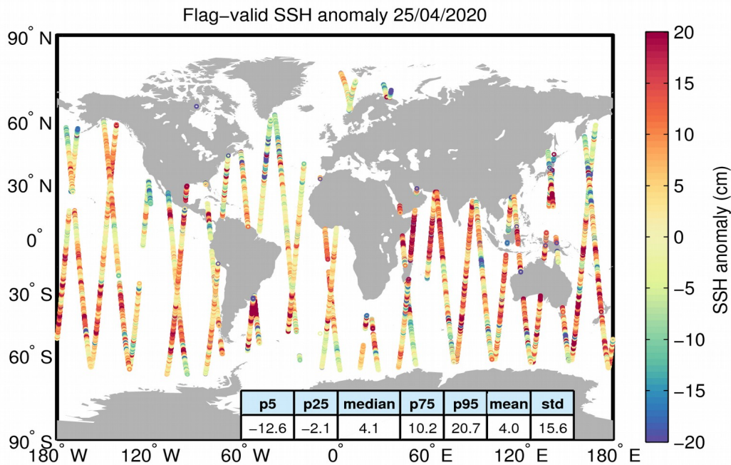
Figure 5. Geographical distribution of flag-valid 1-Hz SSH anomaly data over oceans and lakes for 25/04/2020. The statistical values shown in the table refer to the SSH anomaly in cm and are calculated over all measurements shown in the figure.
