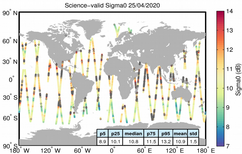
Figure 27. Geographical distribution of science-valid sigma0 data over oceans and lakes for 25/04/2020. The statistical values shown in the table refer to the sigma0 in dB and are calculated over all measurements shown in the figure. Gray circles denote records that have been rejected based on the editing criteria described in Table 4.
