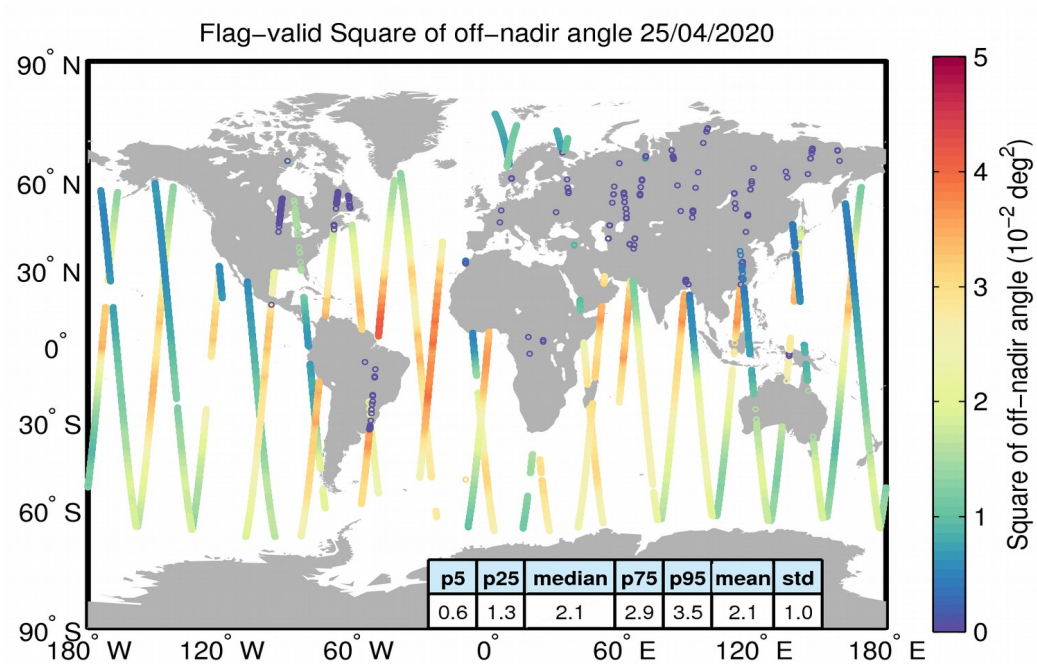
Figure 37. Geographical distribution of flag-valid mispointing data over oceans and lakes for 25/04/2020. The statistical values shown in the table refer to the mispointing in 10^{-2} \text{ deg}^2 and are calculated over all measurements shown in the figure.
