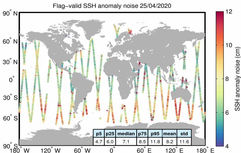
Figure 8. Geographical distribution of flag-valid 20-Hz SSH anomaly measurement noise over oceans and lakes for 25/04/2020. The statistical values shown in the table refer to the SSH anomaly noise and are calculated over all measurements shown in the figure.
