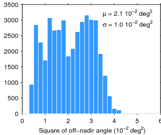
Figure 39. Histogram of flag-valid mispointing over oceans and lakes for 25/04/2020. The mean ( \mu ) and standard deviation ( \sigma ) are also shown. Note that values larger than 6 \cdot 10^{-2} \text{ deg}^2 are excluded from the histogram for the sake of readability but not from the computation of \mu and \sigma .
