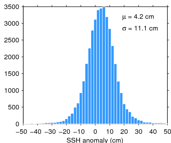
Figure 11. Histogram of science-valid SSH anomaly over oceans and lakes for 25/04/2020. The mean ( \mu ) and standard deviation ( \sigma ) are also shown. Note that values outside [-50 50] cm are excluded from the histogram for the sake of readability but not from the computation of \mu and \sigma .
