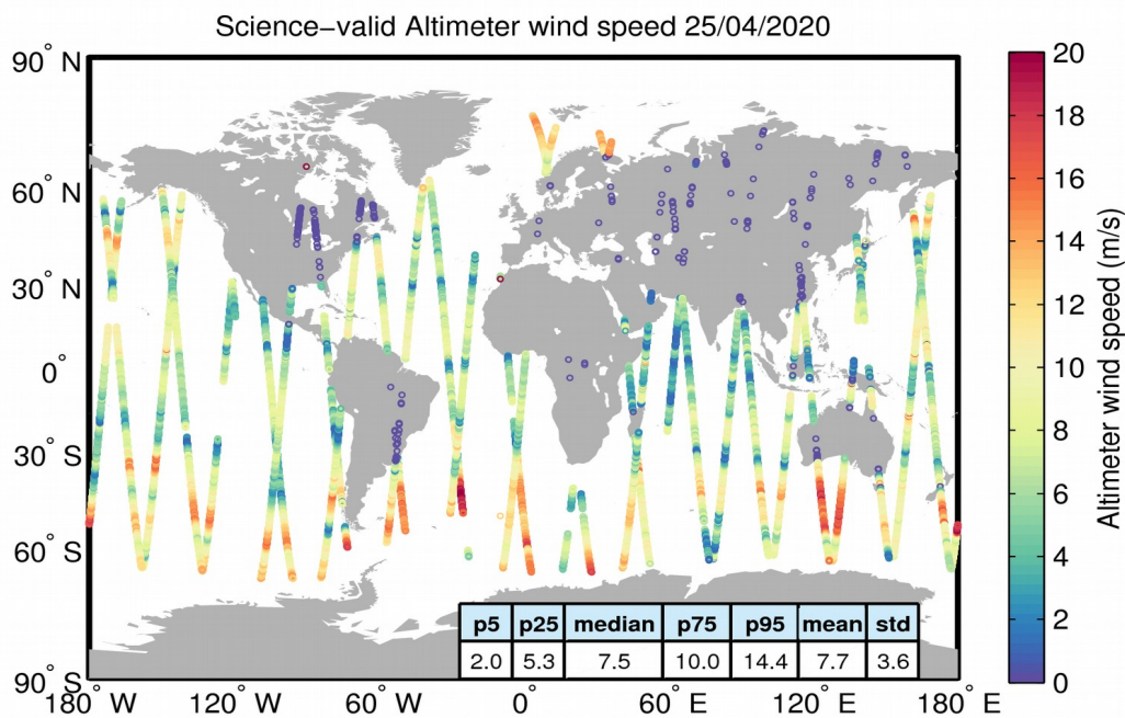
Figure 34. Geographical distribution of science-valid wind data over oceans and lakes for 25/04/2020. The statistical values shown in the table refer to the wind in m/s and are calculated over all measurements shown in the figure. Gray circles denote records that have been rejected based on the editing criteria described in Table 5.
