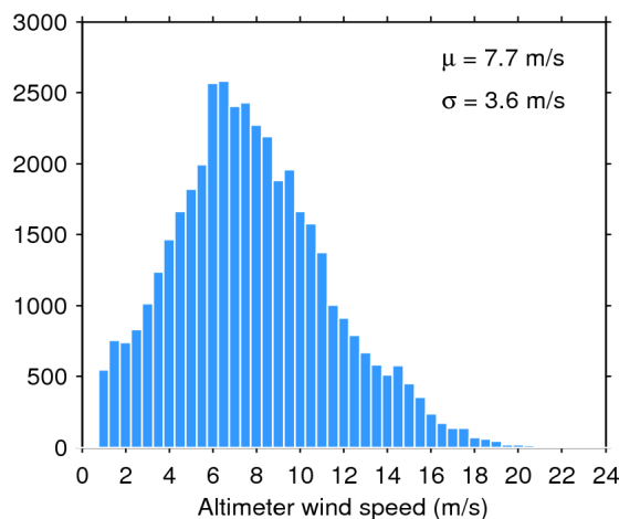
Figure 35. Histogram of science-valid wind over oceans and lakes for 25/04/2020. The mean ( \mu ) and standard deviation ( \sigma ) are also shown. Note that values larger than 24 m/s are excluded from the histogram for the sake of readability but not from the computation of \mu and \sigma .
