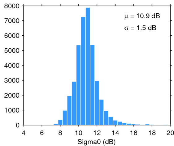
Figure 28. Histogram of science-valid sigma0 over oceans and lakes for 25/04/2020. The mean ( \mu ) and standard deviation ( \sigma ) are also shown. Note that values outside [4 20] dB are excluded from the histogram for the sake of readability but not from the computation of \mu and \sigma .
