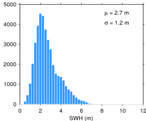
Figure 20. Histogram of science-valid SWH over oceans and lakes for 25/04/2020. The mean ( \mu ) and standard deviation ( \sigma ) are also shown. Note that values larger than 12 m are excluded from the histogram for the sake of readability but not from the computation of \mu and \sigma .
