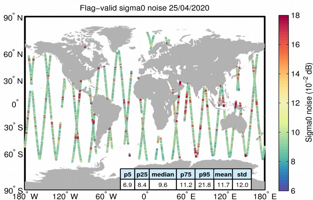
Figure 26. Geographical distribution of flag-valid 20-Hz sigma0 measurement noise over oceans and lakes for 25/04/2020. The statistical values shown in the table refer to the sigma0 noise and are calculated over all measurements shown in the figure.
