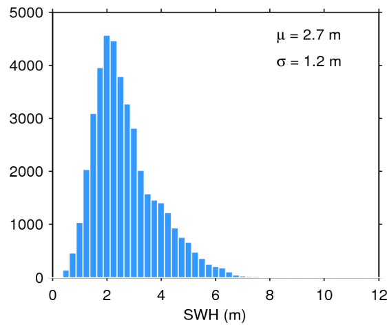
Figure 17. Histogram of flag-valid SWH over oceans and lakes for 25/04/2020. The mean ( \mu ) and standard deviation ( \sigma ) are also shown. Note that values larger than 12 m are excluded from the histogram for the sake of readability but not from the computation of \mu and \sigma .
