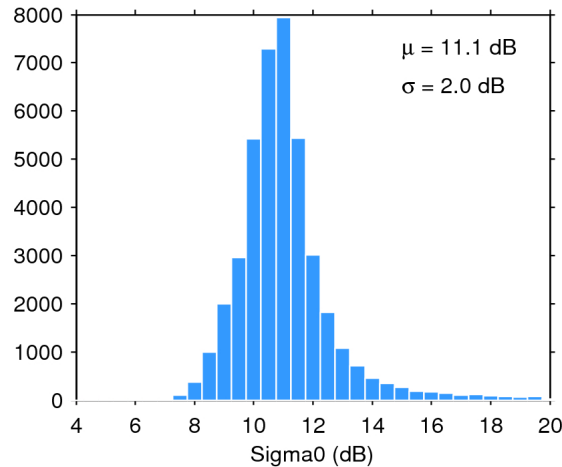
Figure 25. Histogram of flag-valid sigma0 over oceans and lakes for 25/04/2020. The mean ( \mu ) and standard deviation ( \sigma ) are also shown. Note that values outside [4 20] dB are excluded from the histogram for the sake of readability but not from the computation of \mu and \sigma .
