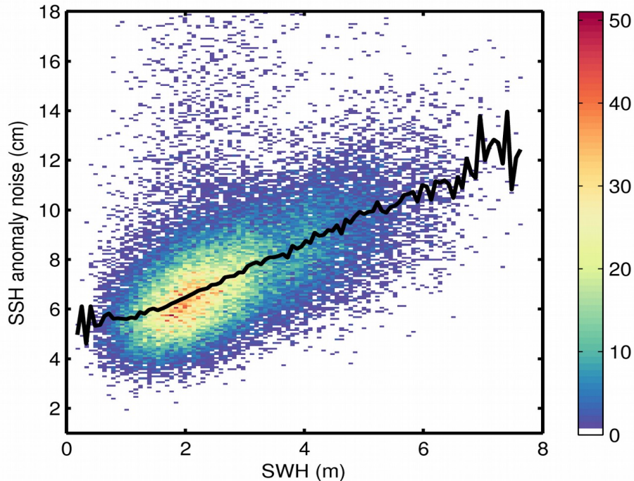
Figure 9. 2D histogram showing flag-valid SSH anomaly noise as a function of SWH for 25/04/2020. The black line denotes the median SSH anomaly noise as a function of SWH.
