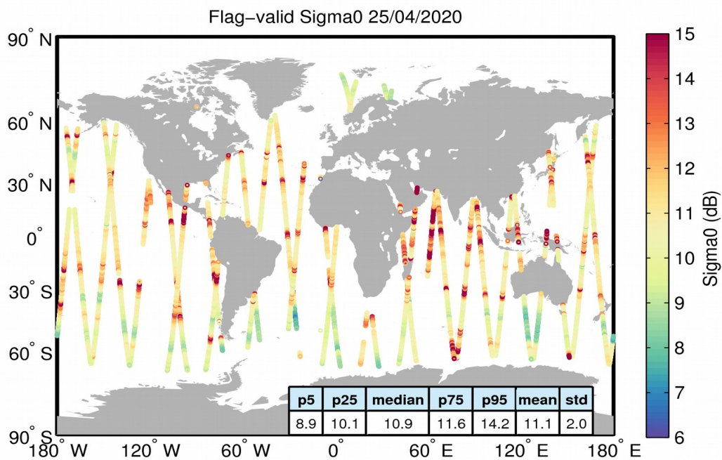
Figure 23. Geographical distribution of flag-valid sigma0 data over oceans and lakes for 25/04/2020. The statistical values shown in the table refer to the sigma0 in dB and are calculated over all measurements shown in the figure.
