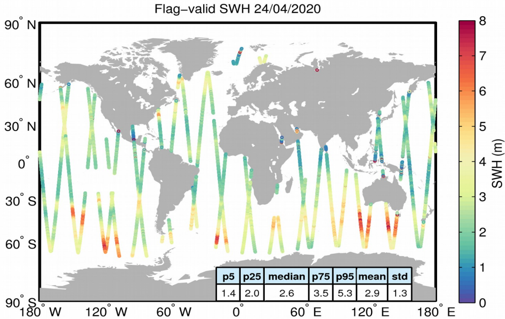
Figure 15. Geographical distribution of flag-valid SWH data over oceans and lakes for 24/04/2020. The statistical values shown in the table refer to the SWH in m and are calculated over all measurements shown in the figure.
