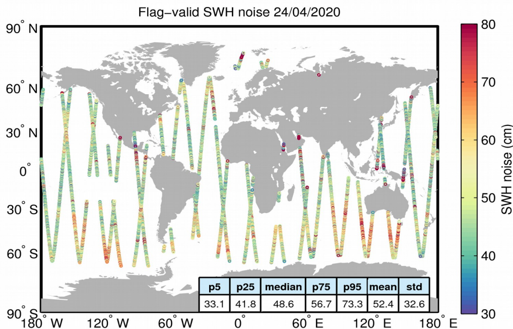
Figure 18. Geographical distribution of flag-valid 20-Hz SWH measurement noise over oceans and lakes for 24/04/2020. The statistical values shown in the figure refer to the SWH noise and are calculated over all measurements shown in the figure.
