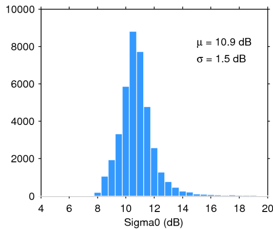
Figure 28. Histogram of science-valid sigma0 over oceans and lakes for 24/04/2020. The mean ( \mu ) and standard deviation ( \sigma ) are also shown. Note that values outside [4 20] dB are excluded from the histogram for the sake of readability but not from the computation of \mu and \sigma .
