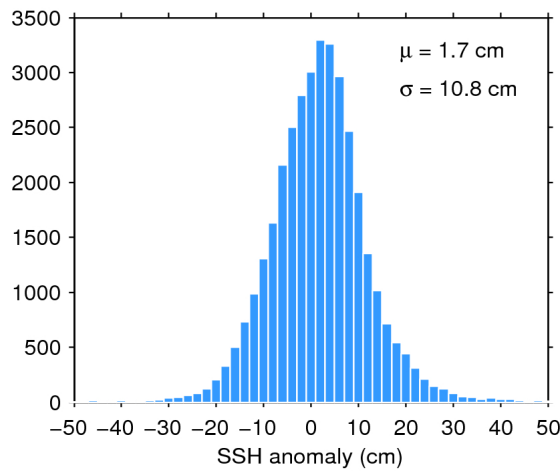
Figure 11. Histogram of science-valid SSH anomaly over oceans and lakes for 24/04/2020. The mean ( \mu ) and standard deviation ( \sigma ) are also shown. Note that values outside [-50 50] cm are excluded from the histogram for the sake of readability but not from the computation of \mu and \sigma .
