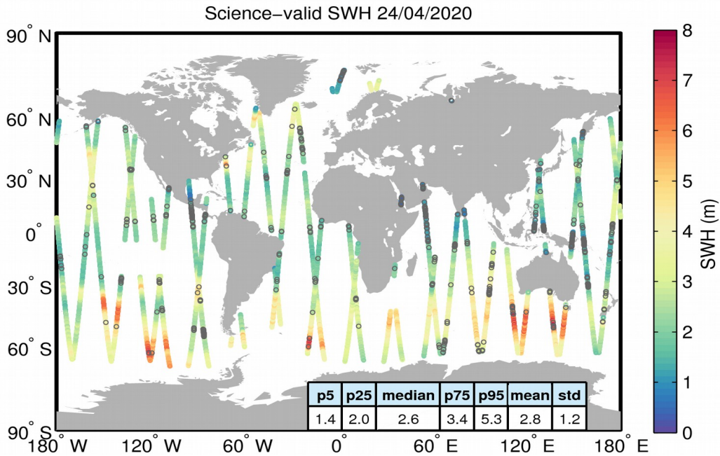
Figure 19. Geographical distribution of science-valid SWH data over oceans and lakes for 24/04/2020. The statistical values shown in the table refer to the SWH in m and are calculated over all measurements shown in the figure. Gray circles denote records that have been rejected based on the editing criteria described in Table 3.
