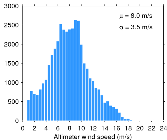
Figure 35. Histogram of science-valid wind over oceans and lakes for 24/04/2020. The mean ( \mu ) and standard deviation ( \sigma ) are also shown. Note that values larger than 24 m/s are excluded from the histogram for the sake of readability but not from the computation of \mu and \sigma .
