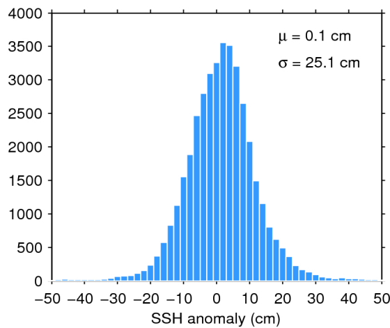
Figure 7. Histogram of flag-valid SSH anomaly over oceans and lakes for 24/04/2020. The mean ( \mu ) and standard deviation ( \sigma ) are also shown. Note that values outside [-50 50] cm are excluded from the histogram for the sake of readability but not from the computation of \mu and \sigma .
