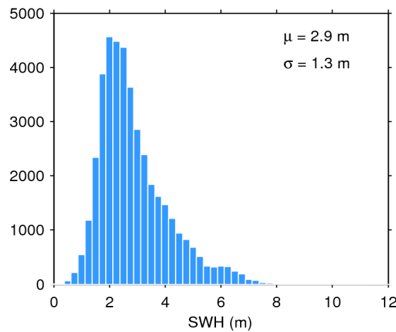
Figure 17. Histogram of flag-valid SWH over oceans and lakes for 24/04/2020. The mean ( \mu ) and standard deviation ( \sigma ) are also shown. Note that values larger than 12 m are excluded from the histogram for the sake of readability but not from the computation of \mu and \sigma .
