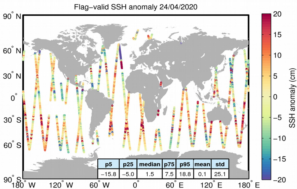
Figure 5. Geographical distribution of flag-valid 1-Hz SSH anomaly data over oceans and lakes for 24/04/2020. The statistical values shown in the table refer to the SSH anomaly in cm and are calculated over all measurements shown in the figure.
