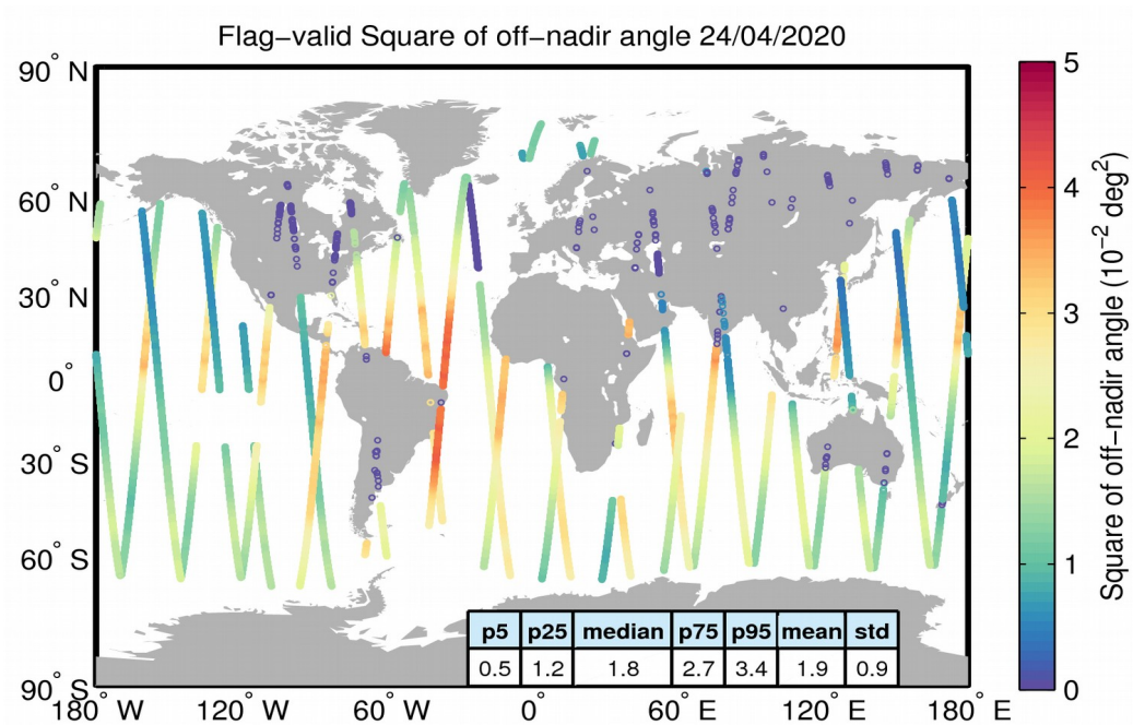
Figure 37. Geographical distribution of flag-valid mispointing data over oceans and lakes for 24/04/2020. The statistical values shown in the table refer to the mispointing in 10^{-2} \text{ deg}^2 and are calculated over all measurements shown in the figure.
