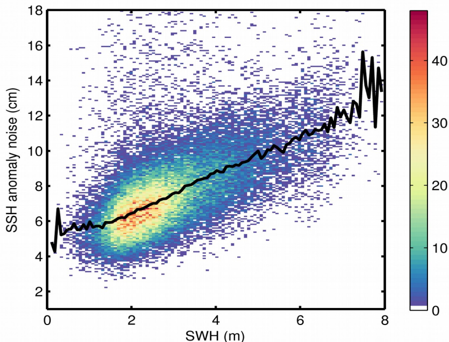
Figure 9. 2D histogram showing flag-valid SSH anomaly noise as a function of SWH for 24/04/2020. The black line denotes the median SSH anomaly noise as a function of SWH.
