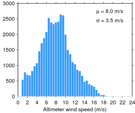
Figure 33. Histogram of flag-valid wind over oceans and lakes for 24/04/2020. The mean ( \mu ) and standard deviation ( \sigma ) are also shown. Note that values larger than 24 m/s are excluded from the histogram for the sake of readability but not from the computation of \mu and \sigma .
