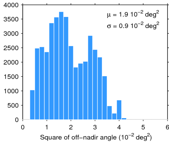
Figure 39. Histogram of flag-valid mispointing over oceans and lakes for 24/04/2020. The mean ( \mu ) and standard deviation ( \sigma ) are also shown. Note that values larger than 6 \cdot 10^{-2} \text{ deg}^2 are excluded from the histogram for the sake of readability but not from the computation of \mu and \sigma .
