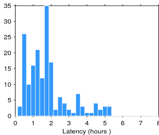
Figure 2. Histogram of the data latency for 24/04/2020. The y-axis denotes the number of files that are made available with a delay of x-hours with respect to the mean time of the records stored in the file.
