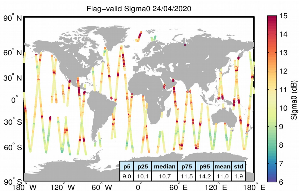
Figure 23. Geographical distribution of flag-valid sigma0 data over oceans and lakes for 24/04/2020. The statistical values shown in the table refer to the sigma0 in dB and are calculated over all measurements shown in the figure.
