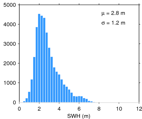
Figure 20. Histogram of science-valid SWH over oceans and lakes for 24/04/2020. The mean ( \mu ) and standard deviation ( \sigma ) are also shown. Note that values larger than 12 m are excluded from the histogram for the sake of readability but not from the computation of \mu and \sigma .
