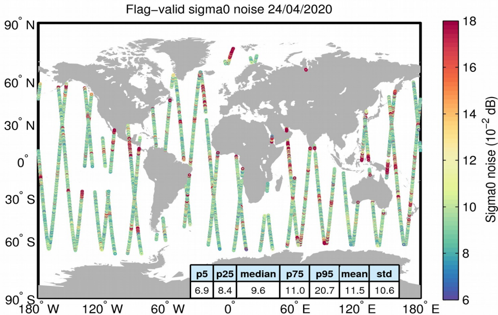
Figure 26. Geographical distribution of flag-valid 20-Hz sigma0 measurement noise over oceans and lakes for 24/04/2020. The statistical values shown in the table refer to the sigma0 noise and are calculated over all measurements shown in the figure.
