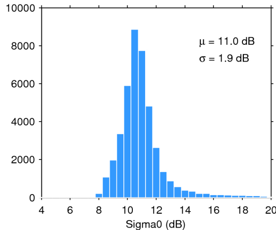
Figure 25. Histogram of flag-valid sigma0 over oceans and lakes for 24/04/2020. The mean ( \mu ) and standard deviation ( \sigma ) are also shown. Note that values outside [4 20] dB are excluded from the histogram for the sake of readability but not from the computation of \mu and \sigma .
