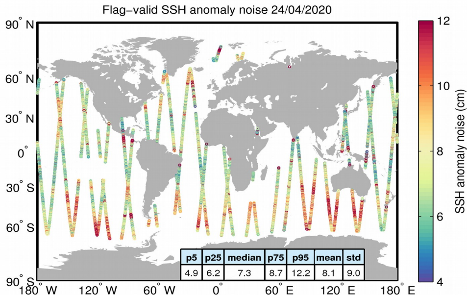
Figure 8. Geographical distribution of flag-valid 20-Hz SSH anomaly measurement noise over oceans and lakes for 24/04/2020. The statistical values shown in the table refer to the SSH anomaly noise and are calculated over all measurements shown in the figure.
