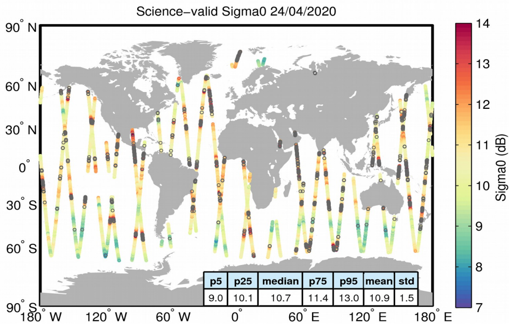
Figure 27. Geographical distribution of science-valid sigma0 data over oceans and lakes for 24/04/2020. The statistical values shown in the table refer to the sigma0 in dB and are calculated over all measurements shown in the figure. Gray circles denote records that have been rejected based on the editing criteria described in Table 4.
