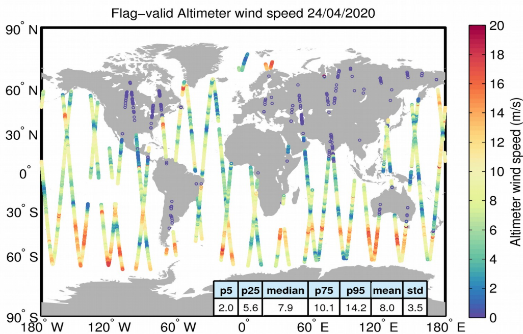
Figure 31. Geographical distribution of flag-valid wind data over oceans and lakes for 24/04/2020. The statistical values shown in the table refer to the wind in m/s and are calculated over all measurements shown in the figure.
