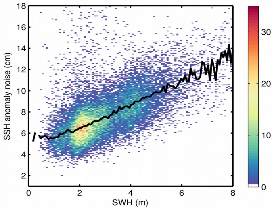
Figure 9. 2D histogram showing flag-valid SSH anomaly noise as a function of SWH for 22/04/2020. The black line denotes the median SSH anomaly noise as a function of SWH.
