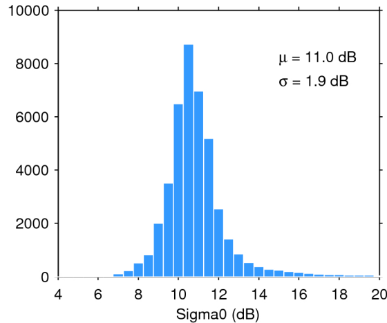
Figure 25. Histogram of flag-valid sigma0 over oceans and lakes for 22/04/2020. The mean ( \mu ) and standard deviation ( \sigma ) are also shown. Note that values outside [4 20] dB are excluded from the histogram for the sake of readability but not from the computation of \mu and \sigma .
