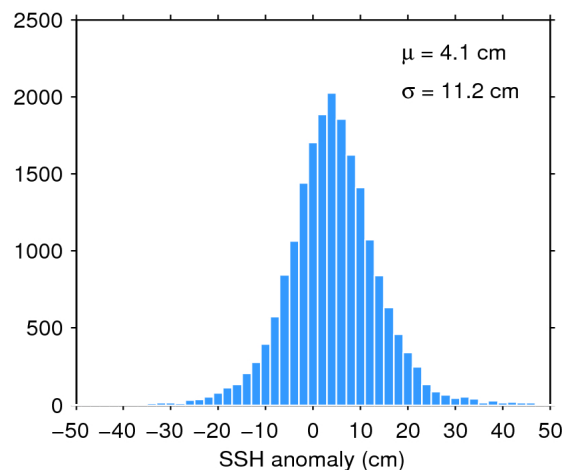
Figure 11. Histogram of science-valid SSH anomaly over oceans and lakes for 22/04/2020. The mean ( \mu ) and standard deviation ( \sigma ) are also shown. Note that values outside [-50 50] cm are excluded from the histogram for the sake of readability but not from the computation of \mu and \sigma .
