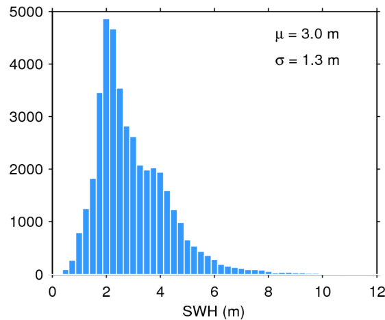
Figure 20. Histogram of science-valid SWH over oceans and lakes for 22/04/2020. The mean ( \mu ) and standard deviation ( \sigma ) are also shown. Note that values larger than 12 m are excluded from the histogram for the sake of readability but not from the computation of \mu and \sigma .
