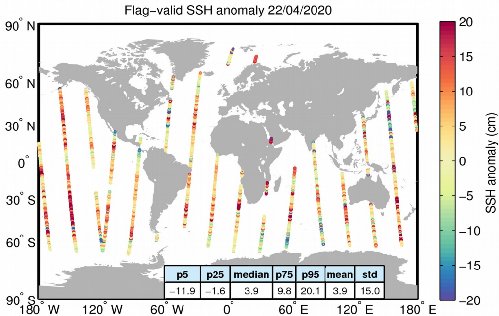
Figure 5. Geographical distribution of flag-valid 1-Hz SSH anomaly data over oceans and lakes for 22/04/2020. The statistical values shown in the table refer to the SSH anomaly in cm and are calculated over all measurements shown in the figure.
