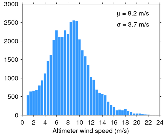
Figure 33. Histogram of flag-valid wind over oceans and lakes for 22/04/2020. The mean ( \mu ) and standard deviation ( \sigma ) are also shown. Note that values larger than 24 m/s are excluded from the histogram for the sake of readability but not from the computation of \mu and \sigma .
