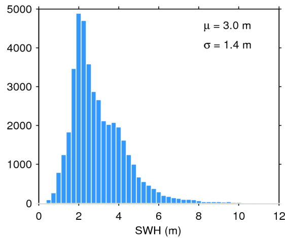
Figure 17. Histogram of flag-valid SWH over oceans and lakes for 22/04/2020. The mean ( \mu ) and standard deviation ( \sigma ) are also shown. Note that values larger than 12 m are excluded from the histogram for the sake of readability but not from the computation of \mu and \sigma .
