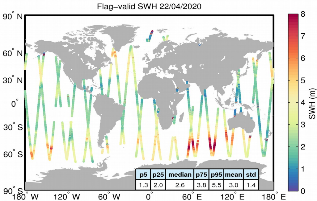
Figure 15. Geographical distribution of flag-valid SWH data over oceans and lakes for 22/04/2020. The statistical values shown in the table refer to the SWH in m and are calculated over all measurements shown in the figure.
