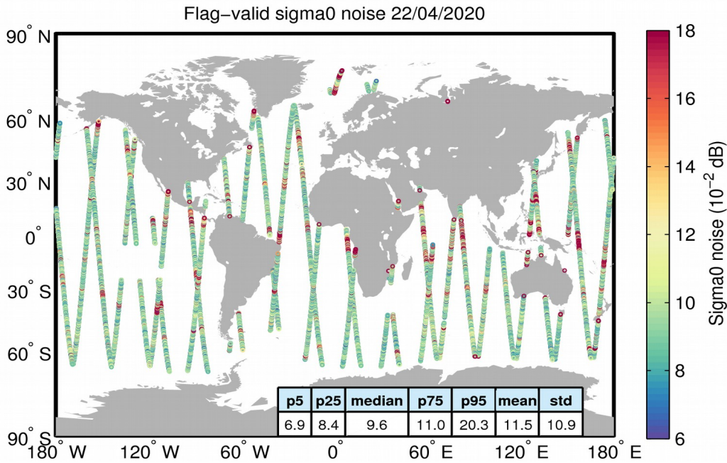
Figure 26. Geographical distribution of flag-valid 20-Hz sigma0 measurement noise over oceans and lakes for 22/04/2020. The statistical values shown in the table refer to the sigma0 noise and are calculated over all measurements shown in the figure.
