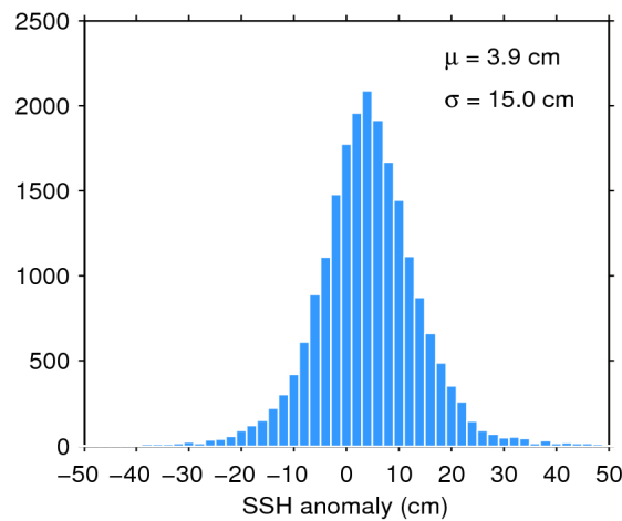
Figure 7. Histogram of flag-valid SSH anomaly over oceans and lakes for 22/04/2020. The mean ( \mu ) and standard deviation ( \sigma ) are also shown. Note that values outside [-50 50] cm are excluded from the histogram for the sake of readability but not from the computation of \mu and \sigma .
