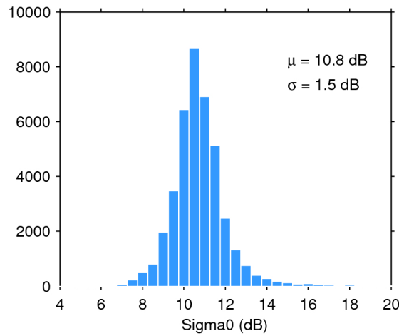
Figure 28. Histogram of science-valid sigma0 over oceans and lakes for 22/04/2020. The mean ( \mu ) and standard deviation ( \sigma ) are also shown. Note that values outside [4 20] dB are excluded from the histogram for the sake of readability but not from the computation of \mu and \sigma .
