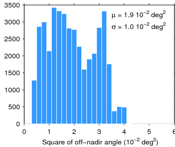
Figure 39. Histogram of flag-valid mispointing over oceans and lakes for 22/04/2020. The mean ( \mu ) and standard deviation ( \sigma ) are also shown. Note that values larger than 6 \cdot 10^{-2} \text{ deg}^2 are excluded from the histogram for the sake of readability but not from the computation of \mu and \sigma .
