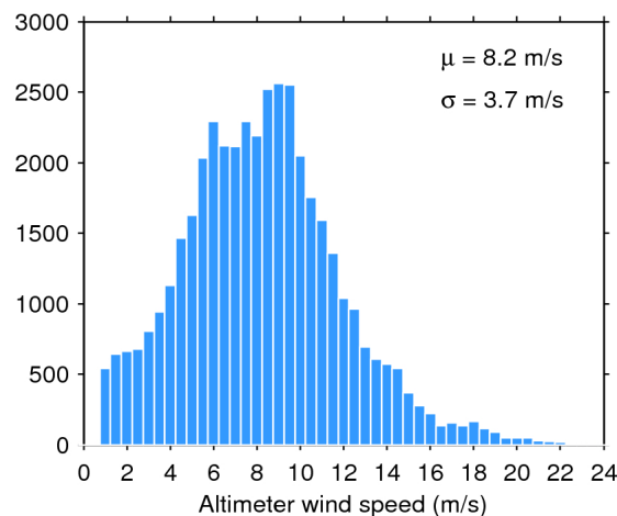
Figure 35. Histogram of science-valid wind over oceans and lakes for 22/04/2020. The mean ( \mu ) and standard deviation ( \sigma ) are also shown. Note that values larger than 24 m/s are excluded from the histogram for the sake of readability but not from the computation of \mu and \sigma .
