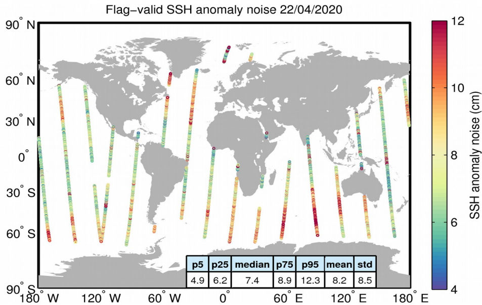
Figure 8. Geographical distribution of flag-valid 20-Hz SSH anomaly measurement noise over oceans and lakes for 22/04/2020. The statistical values shown in the table refer to the SSH anomaly noise and are calculated over all measurements shown in the figure.
