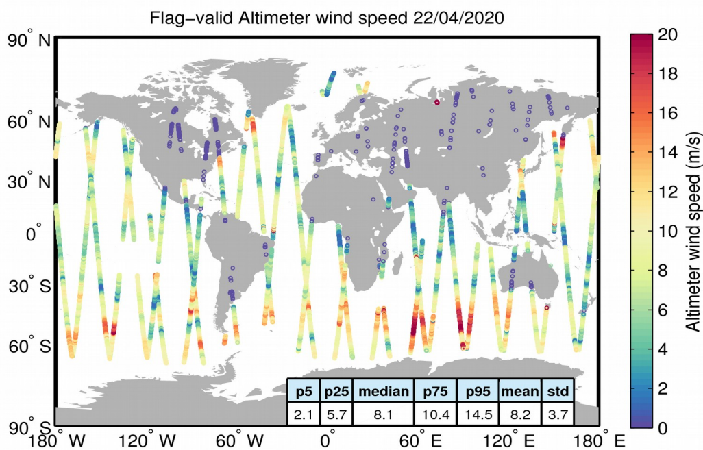
Figure 31. Geographical distribution of flag-valid wind data over oceans and lakes for 22/04/2020. The statistical values shown in the table refer to the wind in m/s and are calculated over all measurements shown in the figure.
