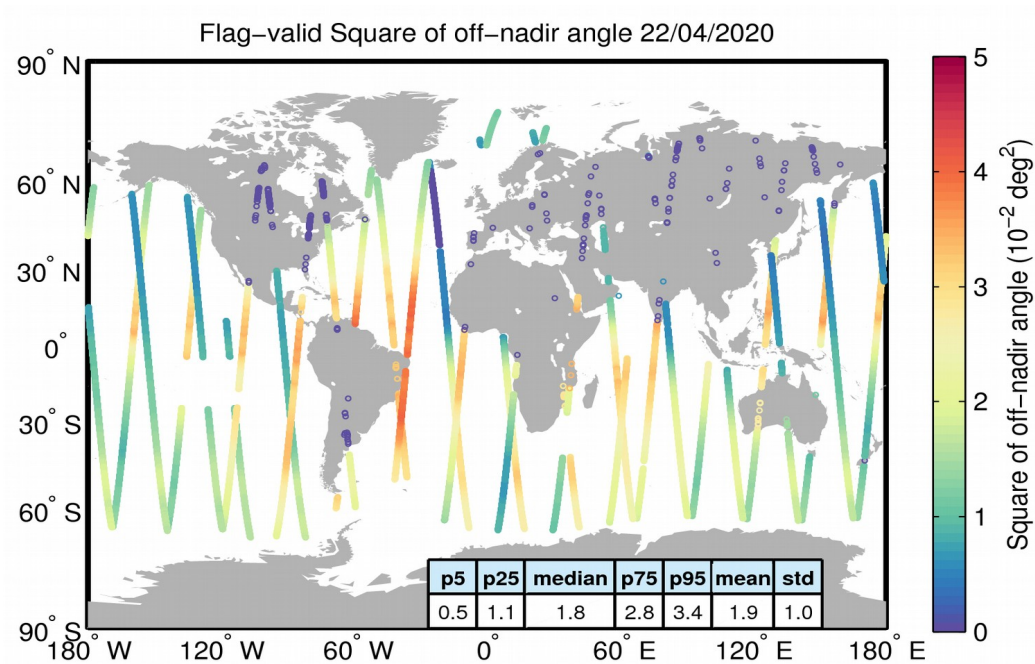
Figure 37. Geographical distribution of flag-valid mispointing data over oceans and lakes for 22/04/2020. The statistical values shown in the table refer to the mispointing in 10^{-2} deg 2 and are calculated over all measurements shown in the figure.
