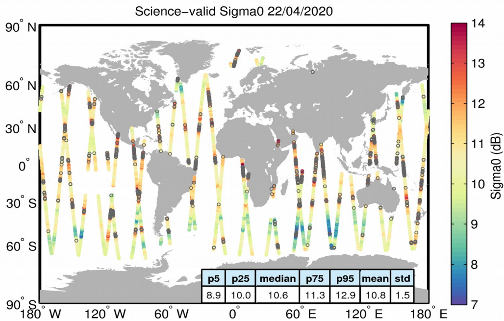
Figure 27. Geographical distribution of science-valid sigma0 data over oceans and lakes for 22/04/2020. The statistical values shown in the table refer to the sigma0 in dB and are calculated over all measurements shown in the figure. Gray circles denote records that have been rejected based on the editing criteria described in Table 4.
