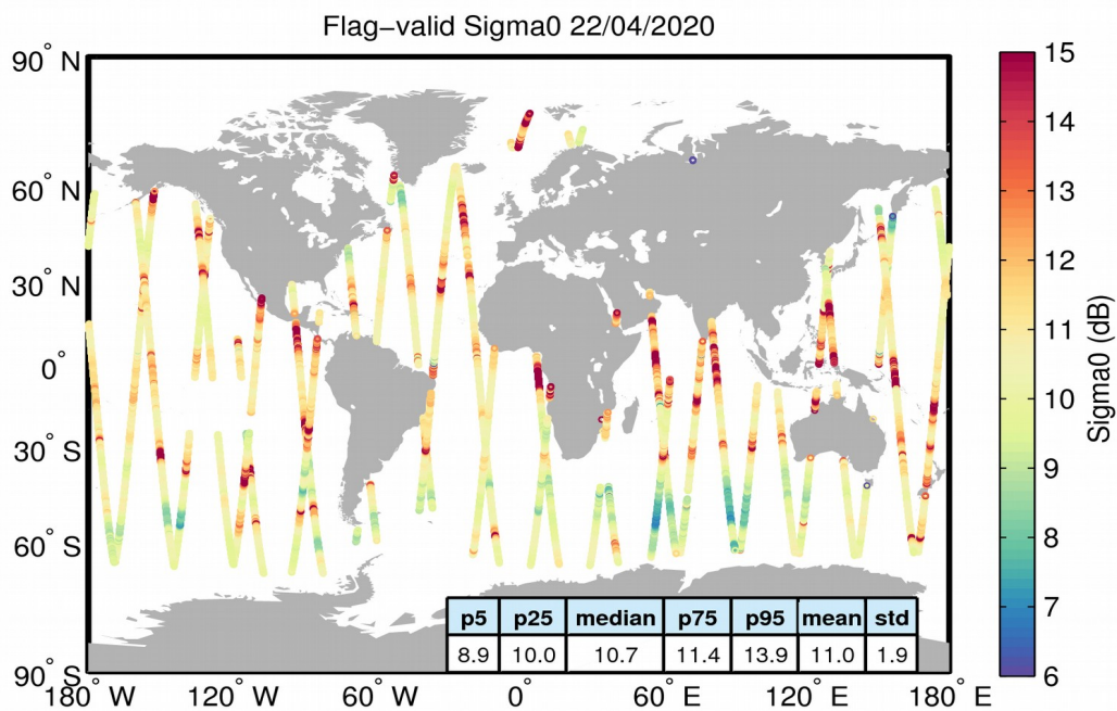
Figure 23. Geographical distribution of flag-valid sigma0 data over oceans and lakes for 22/04/2020. The statistical values shown in the table refer to the sigma0 in dB and are calculated over all measurements shown in the figure.
