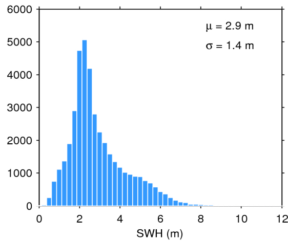
Figure 17. Histogram of flag-valid SWH over oceans and lakes for 21/04/2020. The mean ( \mu ) and standard deviation ( \sigma ) are also shown. Note that values larger than 12 m are excluded from the histogram for the sake of readability but not from the computation of \mu and \sigma .
