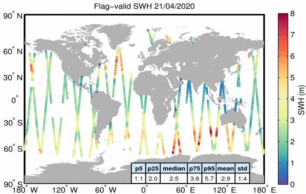
Figure 15. Geographical distribution of flag-valid SWH data over oceans and lakes for 21/04/2020. The statistical values shown in the table refer to the SWH in m and are calculated over all measurements shown in the figure.
