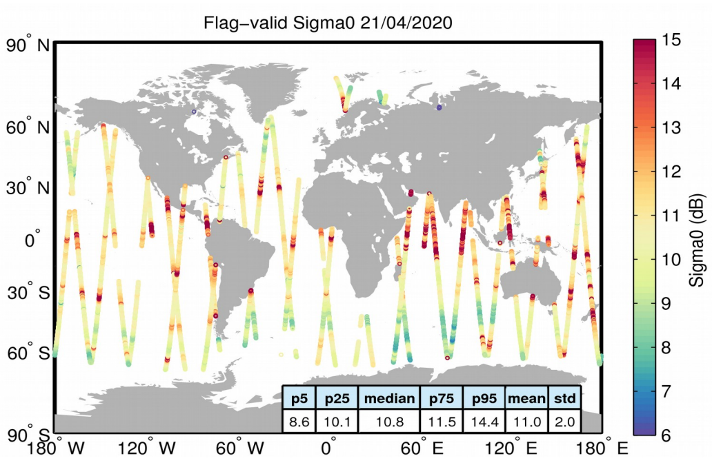
Figure 23. Geographical distribution of flag-valid sigma0 data over oceans and lakes for 21/04/2020. The statistical values shown in the table refer to the sigma0 in dB and are calculated over all measurements shown in the figure.
