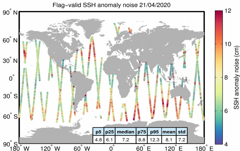
Figure 8. Geographical distribution of flag-valid 20-Hz SSH anomaly measurement noise over oceans and lakes for 21/04/2020. The statistical values shown in the table refer to the SSH anomaly noise and are calculated over all measurements shown in the figure.
