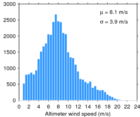
Figure 33. Histogram of flag-valid wind over oceans and lakes for 21/04/2020. The mean ( \mu ) and standard deviation ( \sigma ) are also shown. Note that values larger than 24 m/s are excluded from the histogram for the sake of readability but not from the computation of \mu and \sigma .
