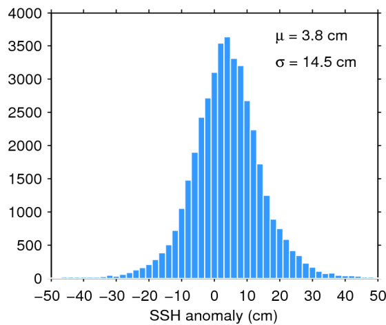
Figure 7. Histogram of flag-valid SSH anomaly over oceans and lakes for 21/04/2020. The mean ( \mu ) and standard deviation ( \sigma ) are also shown. Note that values outside [-50 50] cm are excluded from the histogram for the sake of readability but not from the computation of \mu and \sigma .
