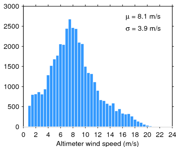
Figure 35. Histogram of science-valid wind over oceans and lakes for 21/04/2020. The mean ( \mu ) and standard deviation ( \sigma ) are also shown. Note that values larger than 24 m/s are excluded from the histogram for the sake of readability but not from the computation of \mu and \sigma .
