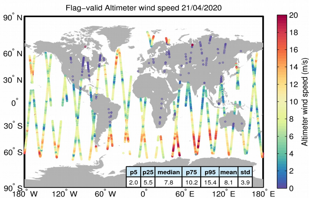
Figure 31. Geographical distribution of flag-valid wind data over oceans and lakes for 21/04/2020. The statistical values shown in the table refer to the wind in m/s and are calculated over all measurements shown in the figure.
