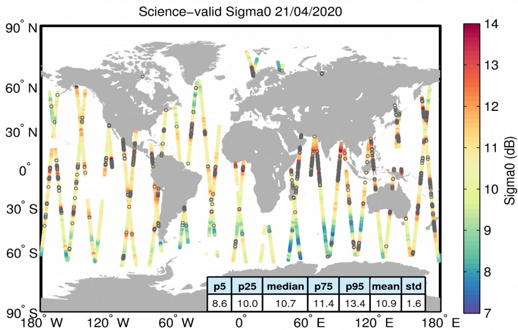
Figure 27. Geographical distribution of science-valid sigma0 data over oceans and lakes for 21/04/2020. The statistical values shown in the table refer to the sigma0 in dB and are calculated over all measurements shown in the figure. Gray circles denote records that have been rejected based on the editing criteria described in Table 4.
