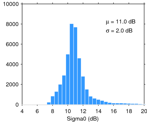
Figure 25. Histogram of flag-valid sigma0 over oceans and lakes for 21/04/2020. The mean ( \mu ) and standard deviation ( \sigma ) are also shown. Note that values outside [4 20] dB are excluded from the histogram for the sake of readability but not from the computation of \mu and \sigma .
