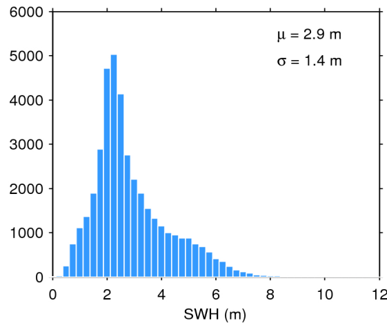
Figure 20. Histogram of science-valid SWH over oceans and lakes for 21/04/2020. The mean ( \mu ) and standard deviation ( \sigma ) are also shown. Note that values larger than 12 m are excluded from the histogram for the sake of readability but not from the computation of \mu and \sigma .
