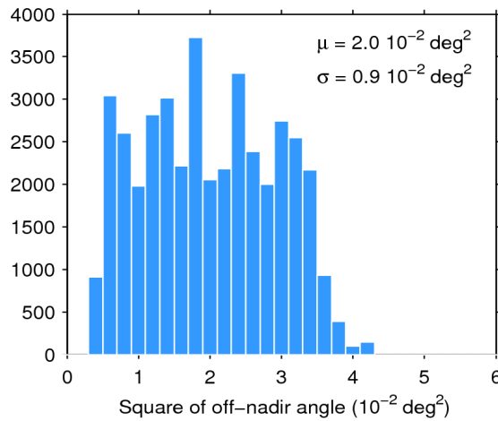
Figure 39. Histogram of flag-valid mispointing over oceans and lakes for 21/04/2020. The mean ( \mu ) and standard deviation ( \sigma ) are also shown. Note that values larger than 6 \cdot 10^{-2} \text{ deg}^2 are excluded from the histogram for the sake of readability but not from the computation of \mu and \sigma .
