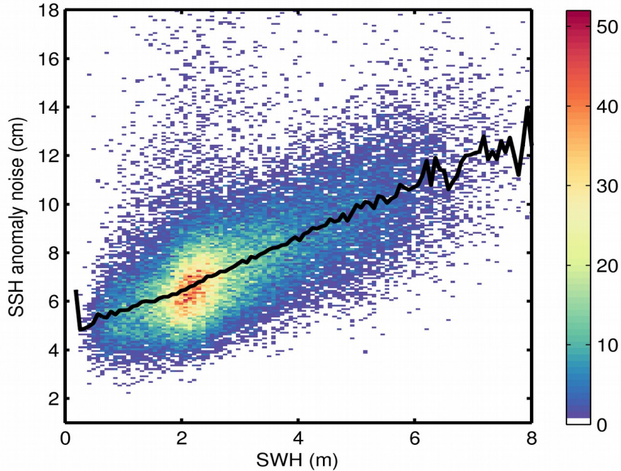
Figure 9. 2D histogram showing flag-valid SSH anomaly noise as a function of SWH for 21/04/2020. The black line denotes the median SSH anomaly noise as a function of SWH.
