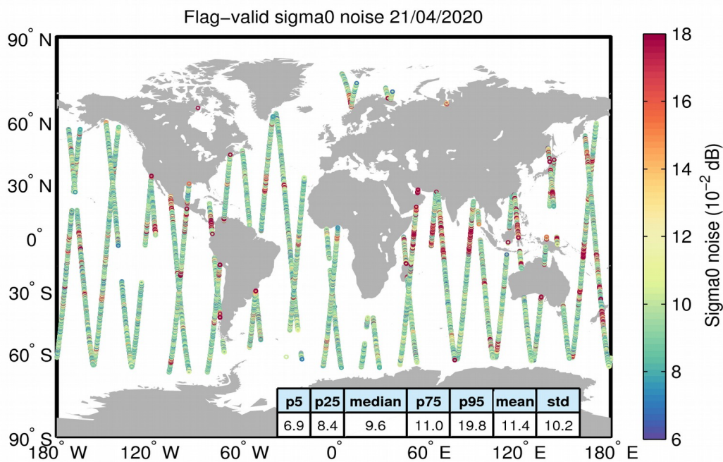
Figure 26. Geographical distribution of flag-valid 20-Hz sigma0 measurement noise over oceans and lakes for 21/04/2020. The statistical values shown in the table refer to the sigma0 noise and are calculated over all measurements shown in the figure.
