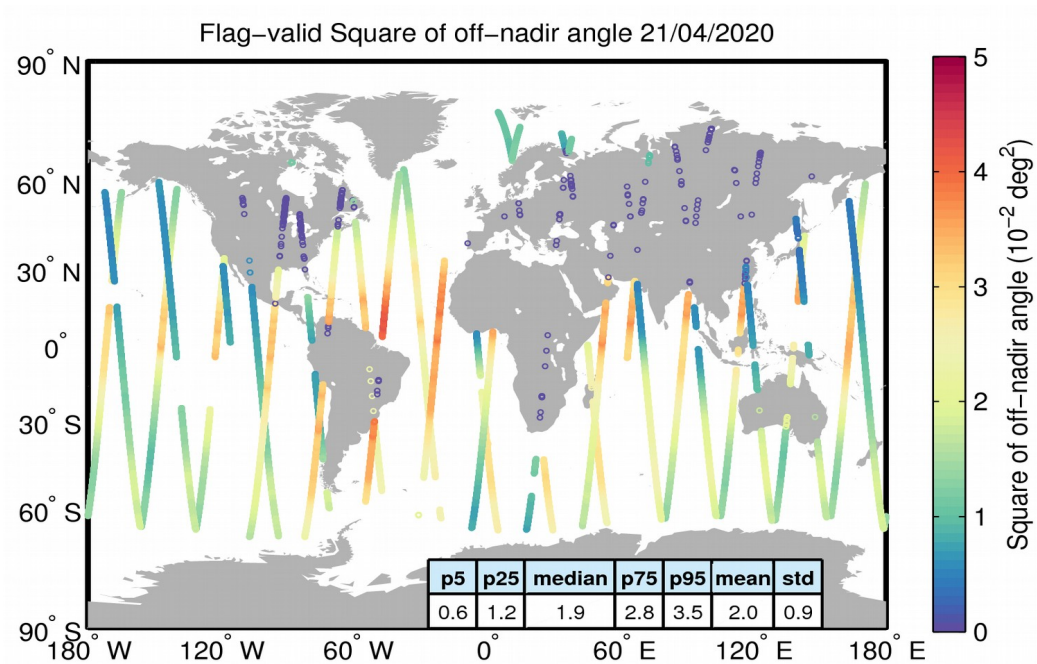
Figure 37. Geographical distribution of flag-valid mispointing data over oceans and lakes for 21/04/2020. The statistical values shown in the table refer to the mispointing in 10^{-2} \text{ deg}^2 and are calculated over all measurements shown in the figure.
