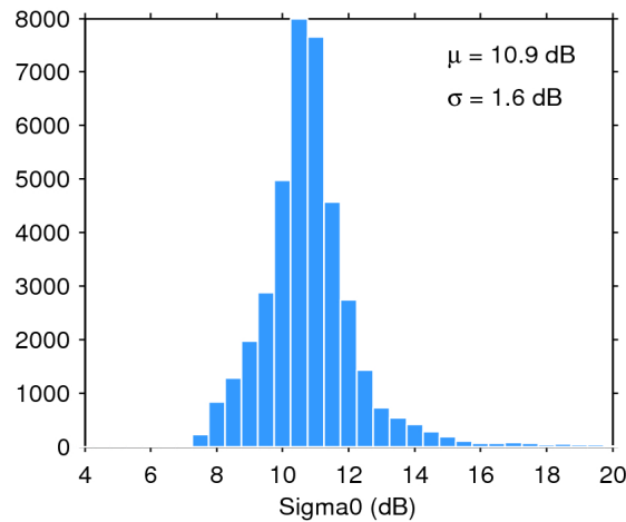
Figure 28. Histogram of science-valid sigma0 over oceans and lakes for 21/04/2020. The mean ( \mu ) and standard deviation ( \sigma ) are also shown. Note that values outside [4 20] dB are excluded from the histogram for the sake of readability but not from the computation of \mu and \sigma .
