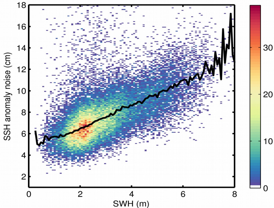
Figure 9. 2D histogram showing flag-valid SSH anomaly noise as a function of SWH for 20/04/2020. The black line denotes the median SSH anomaly noise as a function of SWH.
