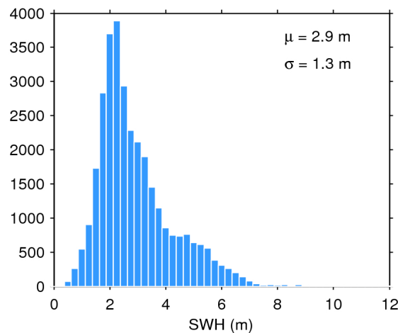
Figure 20. Histogram of science-valid SWH over oceans and lakes for 20/04/2020. The mean ( \mu ) and standard deviation ( \sigma ) are also shown. Note that values larger than 12 m are excluded from the histogram for the sake of readability but not from the computation of \mu and \sigma .
