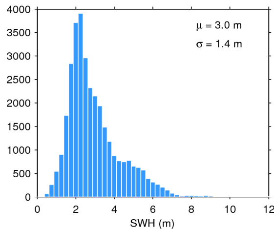
Figure 17. Histogram of flag-valid SWH over oceans and lakes for 20/04/2020. The mean ( \mu ) and standard deviation ( \sigma ) are also shown. Note that values larger than 12 m are excluded from the histogram for the sake of readability but not from the computation of \mu and \sigma .
