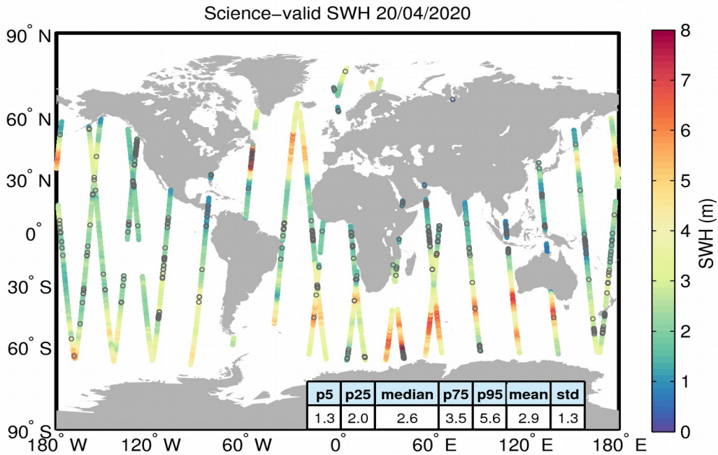
Figure 19. Geographical distribution of science-valid SWH data over oceans and lakes for 20/04/2020. The statistical values shown in the table refer to the SWH in m and are calculated over all measurements shown in the figure. Gray circles denote records that have been rejected based on the editing criteria described in Table 3.
