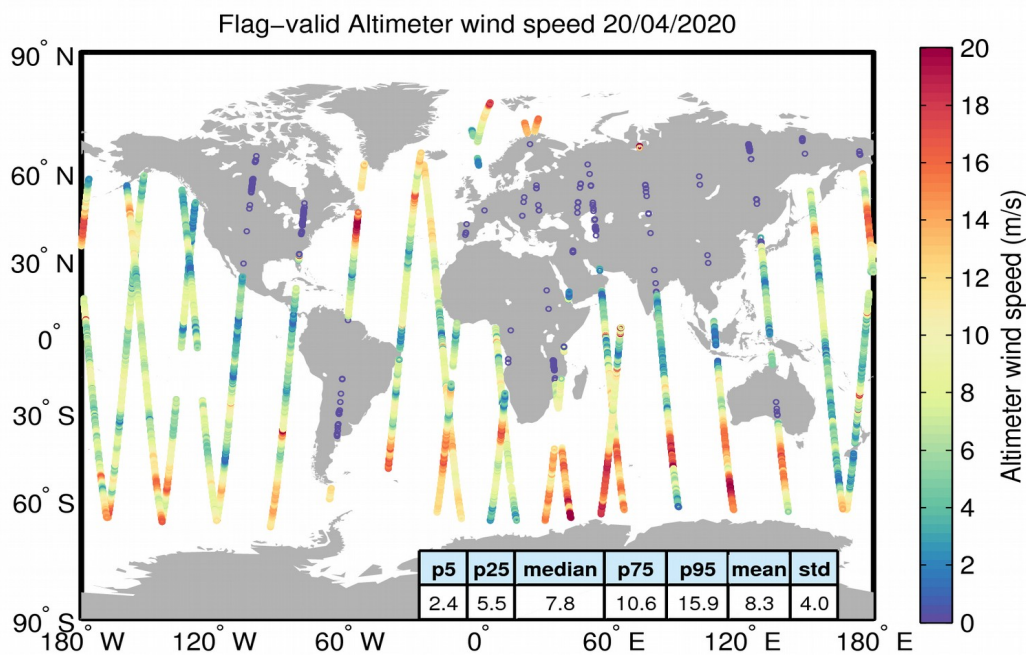
Figure 31. Geographical distribution of flag-valid wind data over oceans and lakes for 20/04/2020. The statistical values shown in the table refer to the wind in m/s and are calculated over all measurements shown in the figure.
