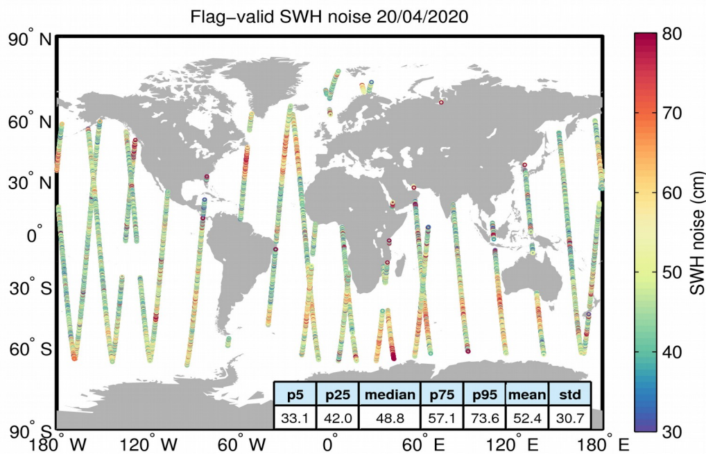
Figure 18. Geographical distribution of flag-valid 20-Hz SWH measurement noise over oceans and lakes for 20/04/2020. The statistical values shown in the table refer to the SWH noise and are calculated over all measurements shown in the figure.
