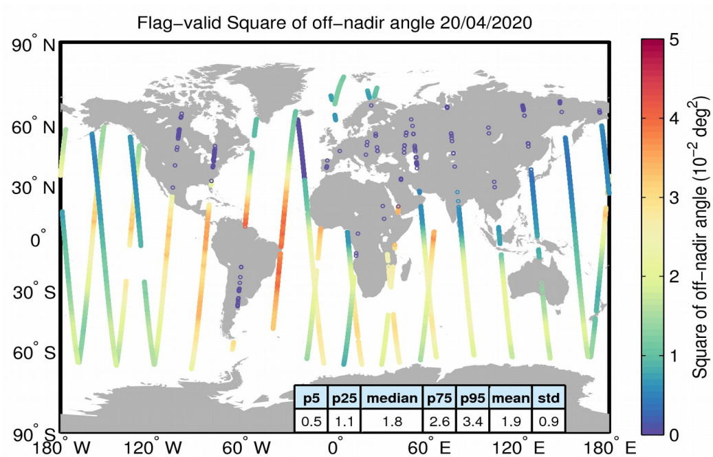
Figure 37. Geographical distribution of flag-valid mispointing data over oceans and lakes for 20/04/2020. The statistical values shown in the table refer to the mispointing in 10^{-2} deg 2 and are calculated over all measurements shown in the figure.
