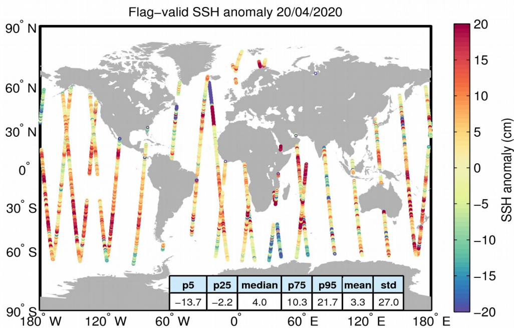
Figure 5. Geographical distribution of flag-valid 1-Hz SSH anomaly data over oceans and lakes for 20/04/2020. The statistical values shown in the table refer to the SSH anomaly in cm and are calculated over all measurements shown in the figure.
