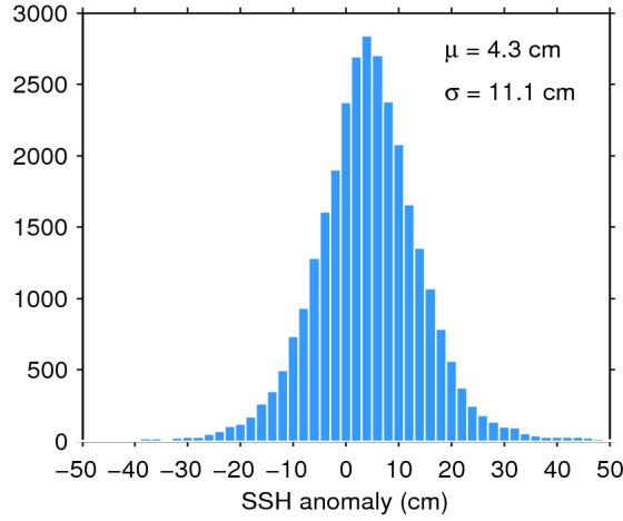
Figure 11. Histogram of science-valid SSH anomaly over oceans and lakes for 20/04/2020. The mean ( \mu ) and standard deviation ( \sigma ) are also shown. Note that values outside [-50 50] cm are excluded from the histogram for the sake of readability but not from the computation of \mu and \sigma .
