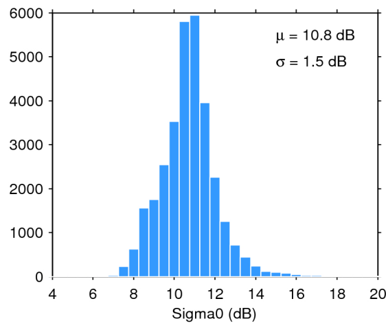
Figure 28. Histogram of science-valid sigma0 over oceans and lakes for 20/04/2020. The mean ( \mu ) and standard deviation ( \sigma ) are also shown. Note that values outside [4 20] dB are excluded from the histogram for the sake of readability but not from the computation of \mu and \sigma .
