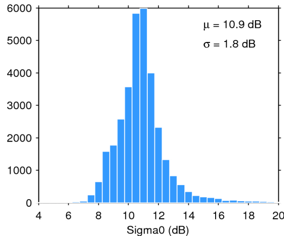
Figure 25. Histogram of flag-valid sigma0 over oceans and lakes for 20/04/2020. The mean ( \mu ) and standard deviation ( \sigma ) are also shown. Note that values outside [4 20] dB are excluded from the histogram for the sake of readability but not from the computation of \mu and \sigma .
