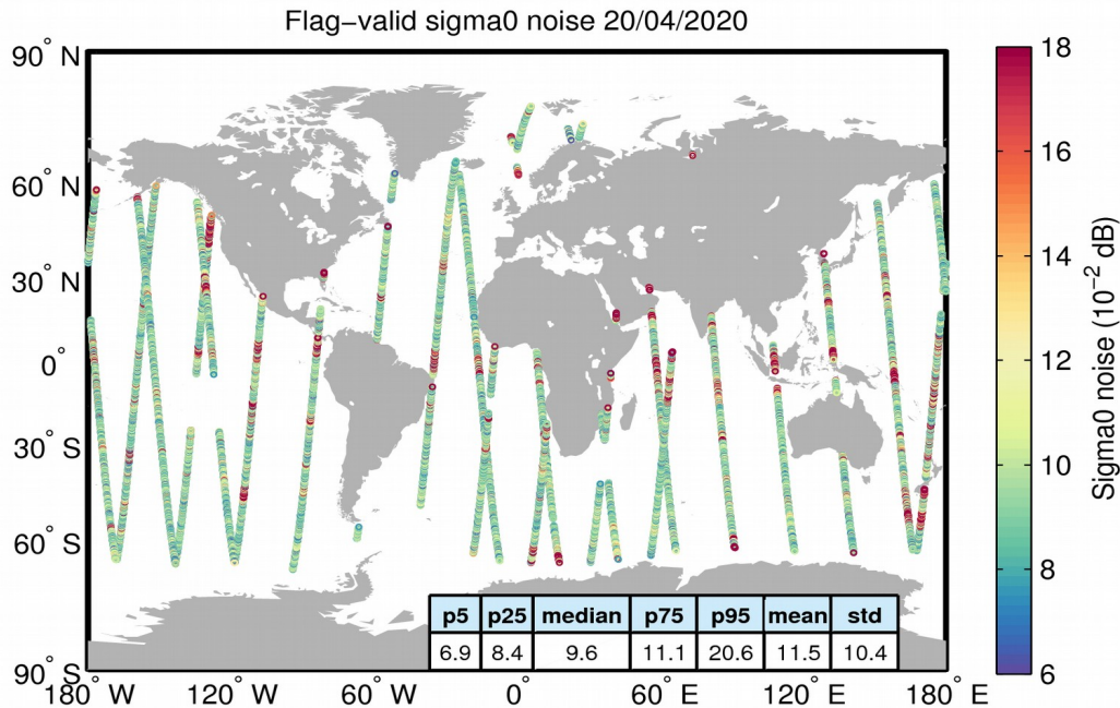
Figure 26. Geographical distribution of flag-valid 20-Hz sigma0 measurement noise over oceans and lakes for 20/04/2020. The statistical values shown in the table refer to the sigma0 noise and are calculated over all measurements shown in the figure.
