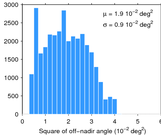
Figure 39. Histogram of flag-valid mispointing over oceans and lakes for 20/04/2020. The mean ( \mu ) and standard deviation ( \sigma ) are also shown. Note that values larger than 6 \cdot 10^{-2} \text{ deg}^2 are excluded from the histogram for the sake of readability but not from the computation of \mu and \sigma .
