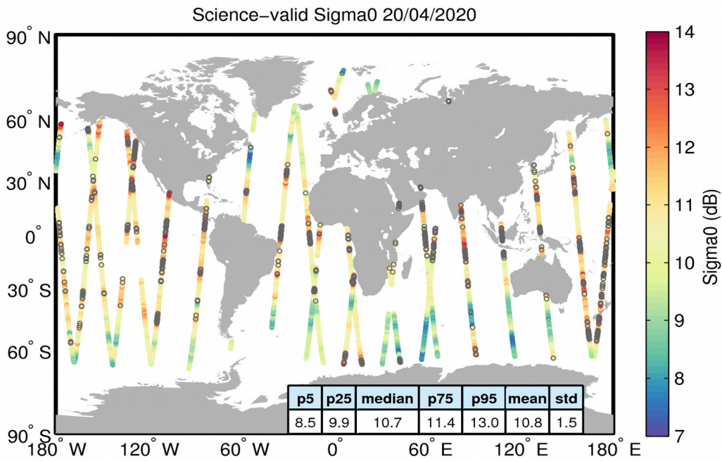
Figure 27. Geographical distribution of science-valid sigma0 data over oceans and lakes for 20/04/2020. The statistical values shown in the table refer to the sigma0 in dB and are calculated over all measurements shown in the figure. Gray circles denote records that have been rejected based on the editing criteria described in Table 4.
