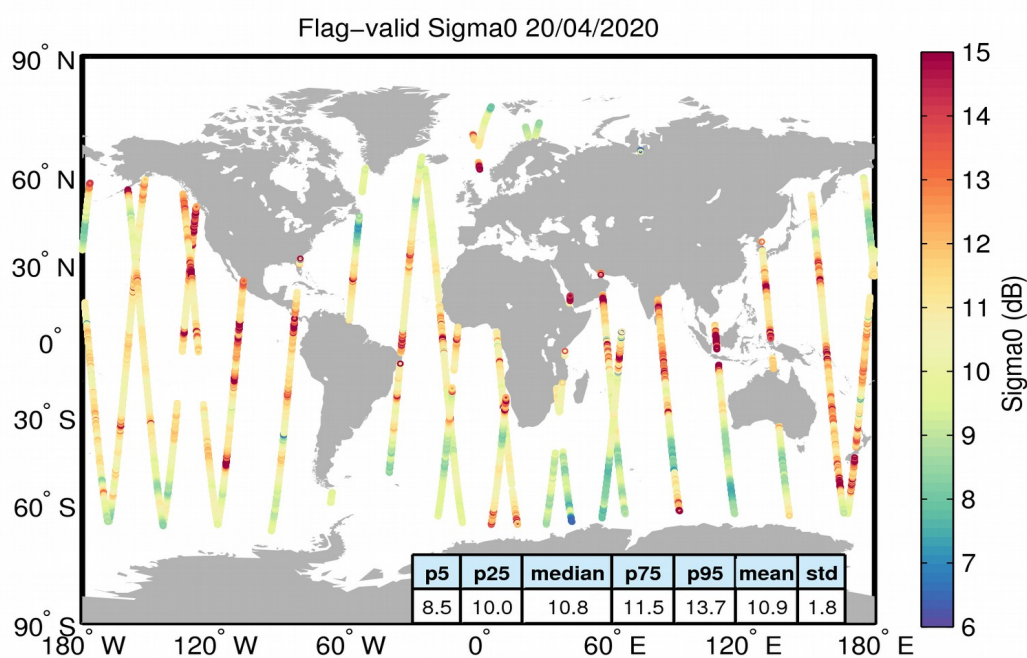
Figure 23. Geographical distribution of flag-valid sigma0 data over oceans and lakes for 20/04/2020. The statistical values shown in the table refer to the sigma0 in dB and are calculated over all measurements shown in the figure.
