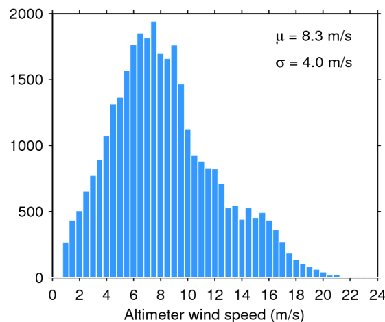
Figure 35. Histogram of science-valid wind over oceans and lakes for 20/04/2020. The mean ( \mu ) and standard deviation ( \sigma ) are also shown. Note that values larger than 24 m/s are excluded from the histogram for the sake of readability but not from the computation of \mu and \sigma .
