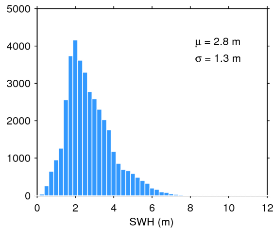
Figure 17. Histogram of flag-valid SWH over oceans and lakes for 19/04/2020. The mean ( \mu ) and standard deviation ( \sigma ) are also shown. Note that values larger than 12 m are excluded from the histogram for the sake of readability but not from the computation of \mu and \sigma .
