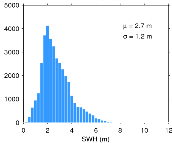
Figure 20. Histogram of science-valid SWH over oceans and lakes for 19/04/2020. The mean ( \mu ) and standard deviation ( \sigma ) are also shown. Note that values larger than 12 m are excluded from the histogram for the sake of readability but not from the computation of \mu and \sigma .
