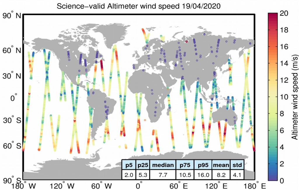
Figure 34. Geographical distribution of science-valid wind data over oceans and lakes for 19/04/2020. The statistical values shown in the table refer to the wind in m/s and are calculated over all measurements shown in the figure. Gray circles denote records that have been rejected based on the editing criteria described in Table 5.
