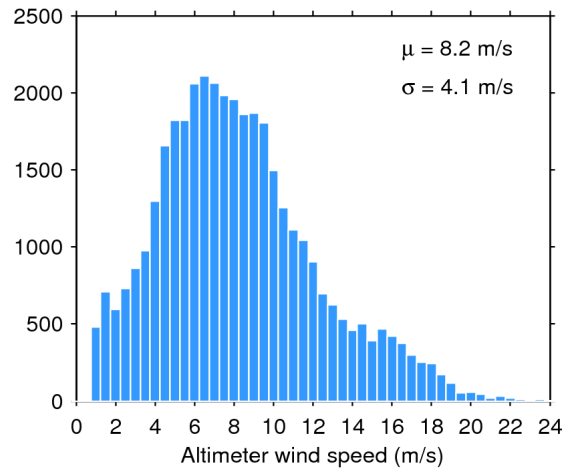
Figure 33. Histogram of flag-valid wind over oceans and lakes for 19/04/2020. The mean ( \mu ) and standard deviation ( \sigma ) are also shown. Note that values larger than 24 m/s are excluded from the histogram for the sake of readability but not from the computation of \mu and \sigma .
