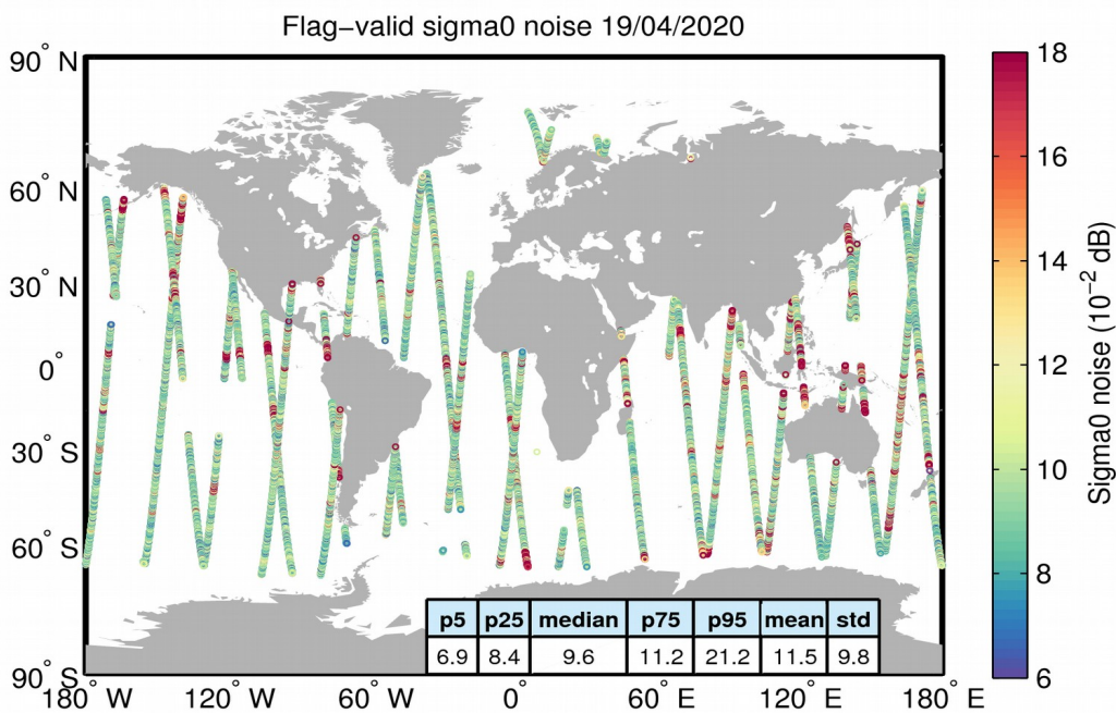
Figure 26. Geographical distribution of flag-valid 20-Hz sigma0 measurement noise over oceans and lakes for 19/04/2020. The statistical values shown in the table refer to the sigma0 noise and are calculated over all measurements shown in the figure.
