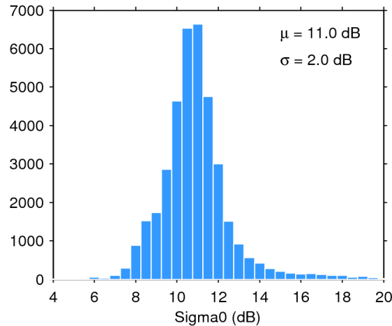
Figure 25. Histogram of flag-valid sigma0 over oceans and lakes for 19/04/2020. The mean ( \mu ) and standard deviation ( \sigma ) are also shown. Note that values outside [4 20] dB are excluded from the histogram for the sake of readability but not from the computation of \mu and \sigma .
