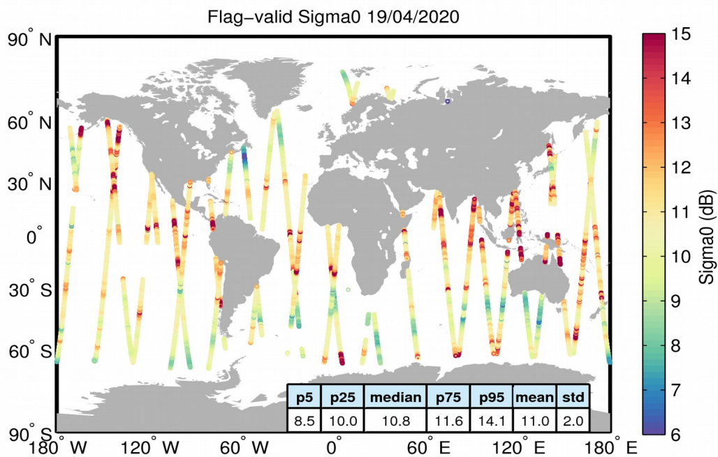
Figure 23. Geographical distribution of flag-valid sigma0 data over oceans and lakes for 19/04/2020. The statistical values shown in the table refer to the sigma0 in dB and are calculated over all measurements shown in the figure.
