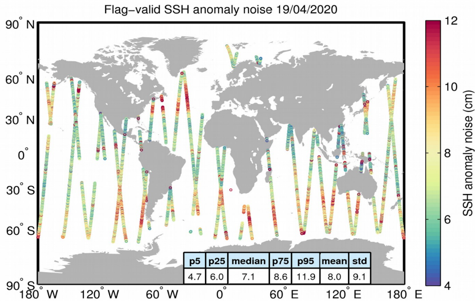
Figure 8. Geographical distribution of flag-valid 20-Hz SSH anomaly measurement noise over oceans and lakes for 19/04/2020. The statistical values shown in the table refer to the SSH anomaly noise and are calculated over all measurements shown in the figure.
