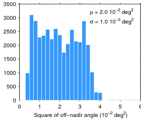
Figure 39. Histogram of flag-valid mispointing over oceans and lakes for 19/04/2020. The mean ( \mu ) and standard deviation ( \sigma ) are also shown. Note that values larger than 6 \cdot 10^{-2} \text{ deg}^2 are excluded from the histogram for the sake of readability but not from the computation of \mu and \sigma .
