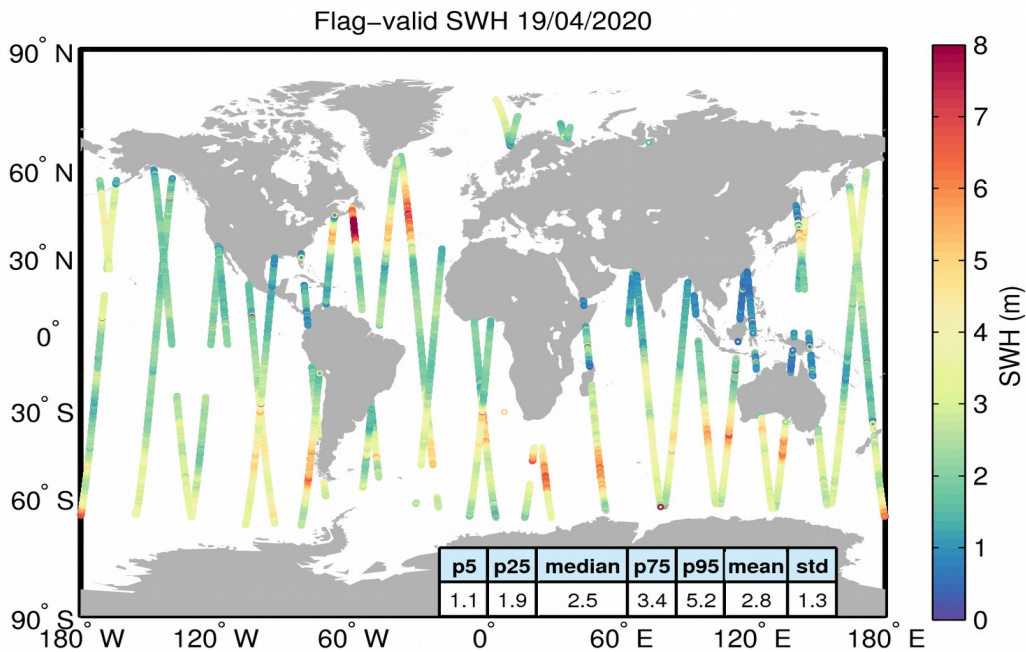
Figure 15. Geographical distribution of flag-valid SWH data over oceans and lakes for 19/04/2020. The statistical values shown in the table refer to the SWH in m and are calculated over all measurements shown in the figure.
