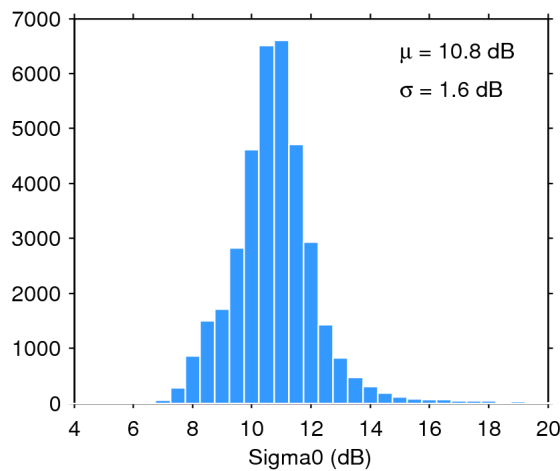
Figure 28. Histogram of science-valid sigma0 over oceans and lakes for 19/04/2020. The mean ( \mu ) and standard deviation ( \sigma ) are also shown. Note that values outside [4 20] dB are excluded from the histogram for the sake of readability but not from the computation of \mu and \sigma .
