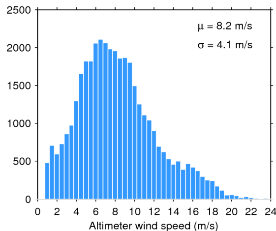
Figure 35. Histogram of science-valid wind over oceans and lakes for 19/04/2020. The mean ( \mu ) and standard deviation ( \sigma ) are also shown. Note that values larger than 24 m/s are excluded from the histogram for the sake of readability but not from the computation of \mu and \sigma .
