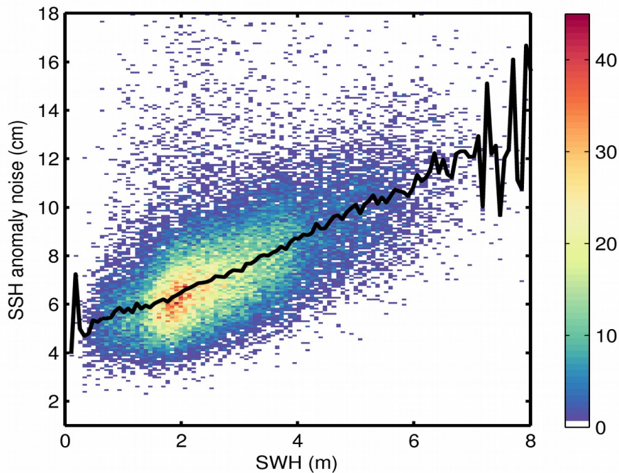
Figure 9. 2D histogram showing flag-valid SSH anomaly noise as a function of SWH for 19/04/2020. The black line denotes the median SSH anomaly noise as a function of SWH.
