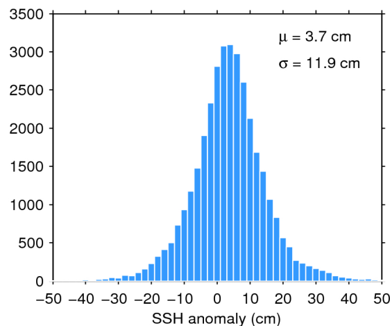
Figure 11. Histogram of science-valid SSH anomaly over oceans and lakes for 19/04/2020. The mean ( \mu ) and standard deviation ( \sigma ) are also shown. Note that values outside [-50 50] cm are excluded from the histogram for the sake of readability but not from the computation of \mu and \sigma .
