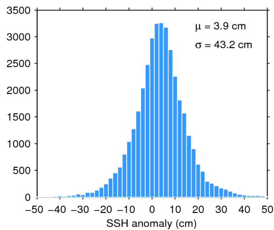
Figure 7. Histogram of flag-valid SSH anomaly over oceans and lakes for 19/04/2020. The mean ( \mu ) and standard deviation ( \sigma ) are also shown. Note that values outside [-50 50] cm are excluded from the histogram for the sake of readability but not from the computation of \mu and \sigma .
