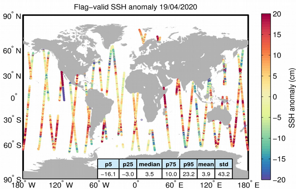
Figure 5. Geographical distribution of flag-valid 1-Hz SSH anomaly data over oceans and lakes for 19/04/2020. The statistical values shown in the table refer to the SSH anomaly in cm and are calculated over all measurements shown in the figure.
