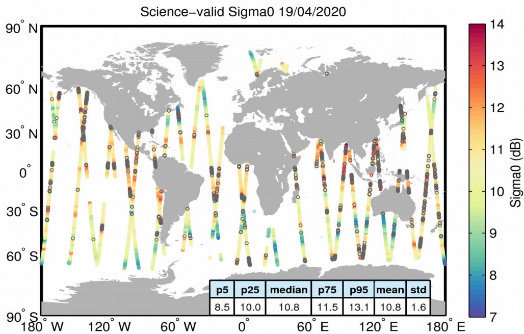
Figure 27. Geographical distribution of science-valid sigma0 data over oceans and lakes for 19/04/2020. The statistical values shown in the table refer to the sigma0 in dB and are calculated over all measurements shown in the figure. Gray circles denote records that have been rejected based on the editing criteria described in Table 4.
