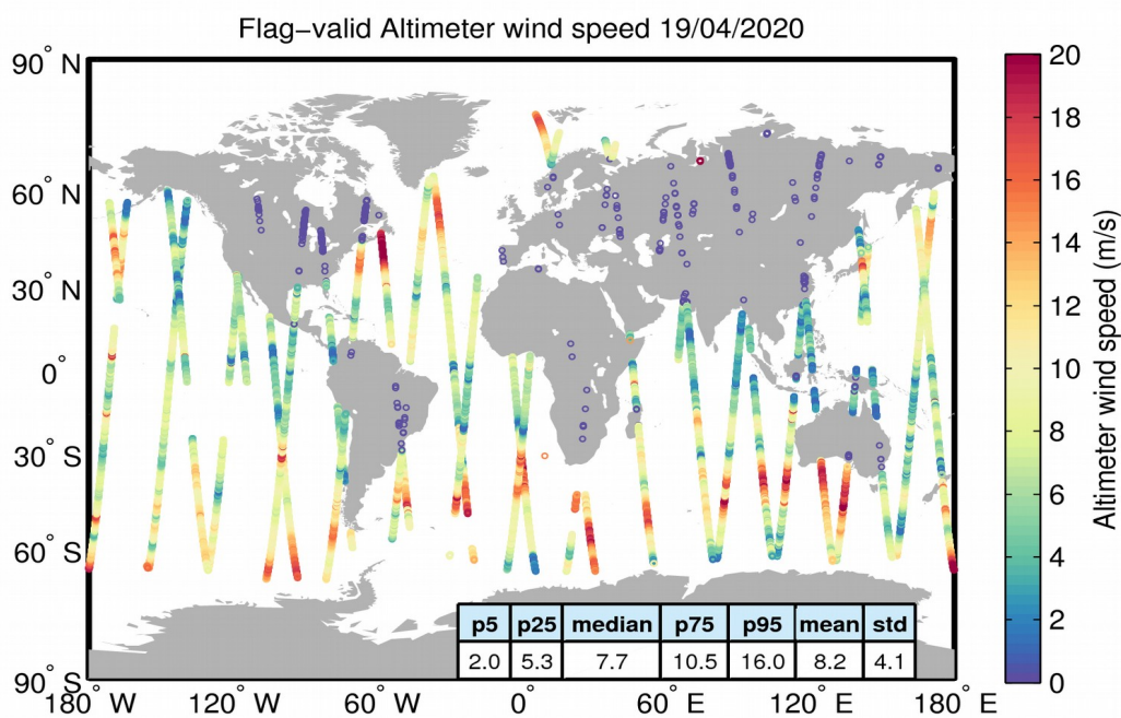
Figure 31. Geographical distribution of flag-valid wind data over oceans and lakes for 19/04/2020. The statistical values shown in the table refer to the wind in m/s and are calculated over all measurements shown in the figure.
