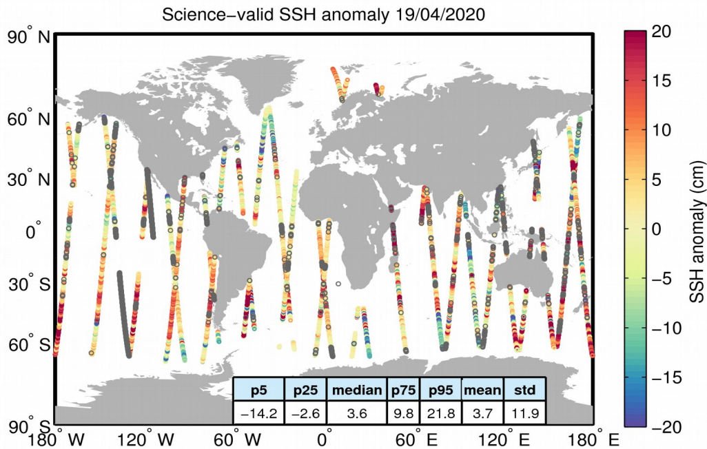
Figure 10. Geographical distribution of science-valid SSH anomaly data over oceans and lakes for 19/04/2020. The statistical values shown in the table refer to the SSH anomaly in cm and are calculated over all measurements shown in the figure. Gray circles denote records that have been rejected based on the editing criteria described in Table 2.
