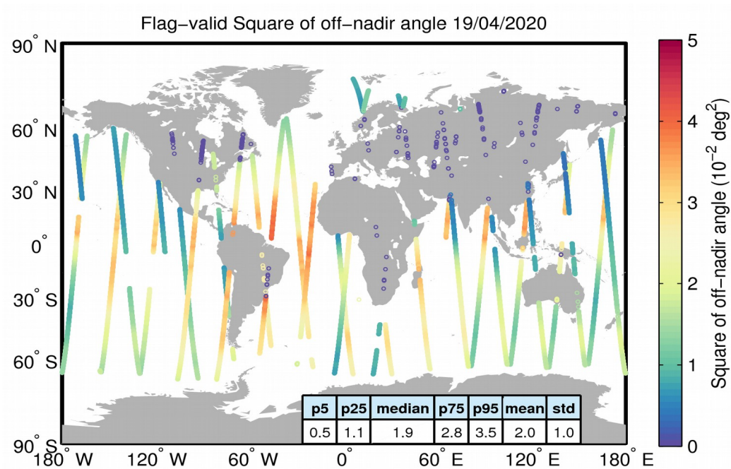
Figure 37. Geographical distribution of flag-valid mispointing data over oceans and lakes for 19/04/2020. The statistical values shown in the table refer to the mispointing in 10^{-2} deg 2 and are calculated over all measurements shown in the figure.
