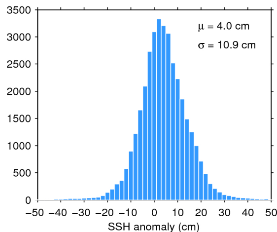
Figure 11. Histogram of science-valid SSH anomaly over oceans and lakes for 18/04/2020. The mean ( \mu ) and standard deviation ( \sigma ) are also shown. Note that values outside [-50 50] cm are excluded from the histogram for the sake of readability but not from the computation of \mu and \sigma .
