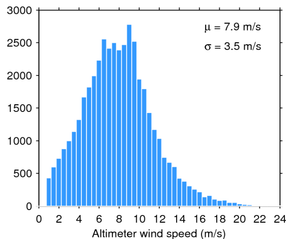
Figure 35. Histogram of science-valid wind over oceans and lakes for 18/04/2020. The mean ( \mu ) and standard deviation ( \sigma ) are also shown. Note that values larger than 24 m/s are excluded from the histogram for the sake of readability but not from the computation of \mu and \sigma .
