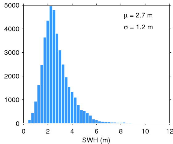
Figure 20. Histogram of science-valid SWH over oceans and lakes for 18/04/2020. The mean ( \mu ) and standard deviation ( \sigma ) are also shown. Note that values larger than 12 m are excluded from the histogram for the sake of readability but not from the computation of \mu and \sigma .
