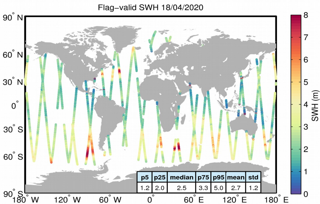
Figure 15. Geographical distribution of flag-valid SWH data over oceans and lakes for 18/04/2020. The statistical values shown in the table refer to the SWH in m and are calculated over all measurements shown in the figure.
