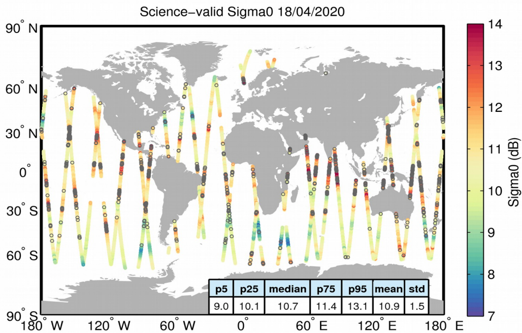
Figure 27. Geographical distribution of science-valid sigma0 data over oceans and lakes for 18/04/2020. The statistical values shown in the table refer to the sigma0 in dB and are calculated over all measurements shown in the figure. Gray circles denote records that have been rejected based on the editing criteria described in Table 4.
