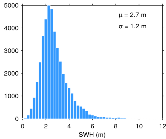
Figure 17. Histogram of flag-valid SWH over oceans and lakes for 18/04/2020. The mean ( \mu ) and standard deviation ( \sigma ) are also shown. Note that values larger than 12 m are excluded from the histogram for the sake of readability but not from the computation of \mu and \sigma .
