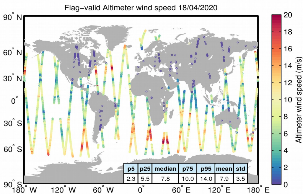
Figure 31. Geographical distribution of flag-valid wind data over oceans and lakes for 18/04/2020. The statistical values shown in the table refer to the wind in m/s and are calculated over all measurements shown in the figure.
