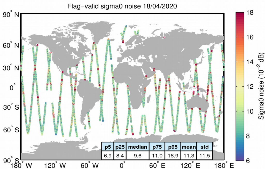
Figure 26. Geographical distribution of flag-valid 20-Hz sigma0 measurement noise over oceans and lakes for 18/04/2020. The statistical values shown in the table refer to the sigma0 noise and are calculated over all measurements shown in the figure.
