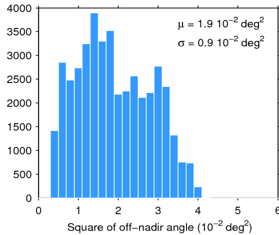
Figure 39. Histogram of flag-valid mispointing over oceans and lakes for 18/04/2020. The mean ( \mu ) and standard deviation ( \sigma ) are also shown. Note that values larger than 6 \cdot 10^{-2} \text{ deg}^2 are excluded from the histogram for the sake of readability but not from the computation of \mu and \sigma .
