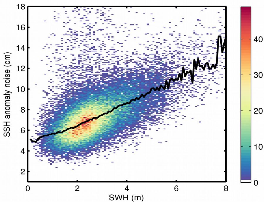
Figure 9. 2D histogram showing flag-valid SSH anomaly noise as a function of SWH for 18/04/2020. The black line denotes the median SSH anomaly noise as a function of SWH.
