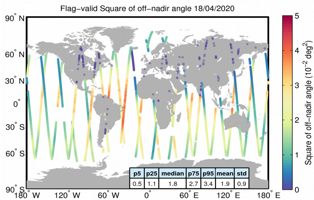
Figure 37. Geographical distribution of flag-valid mispointing data over oceans and lakes for 18/04/2020. The statistical values shown in the table refer to the mispointing in 10^{-2} \text{ deg}^2 and are calculated over all measurements shown in the figure.
