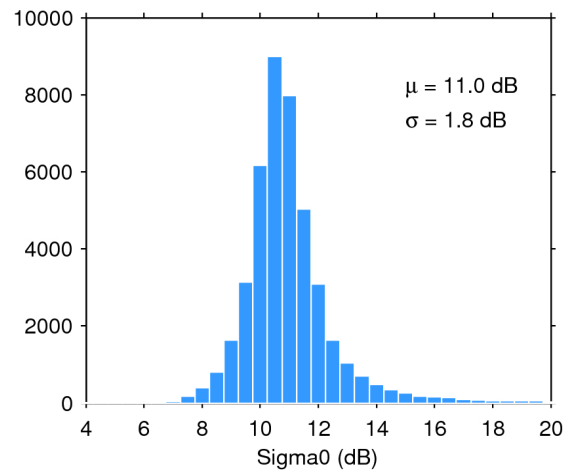
Figure 25. Histogram of flag-valid sigma0 over oceans and lakes for 18/04/2020. The mean ( \mu ) and standard deviation ( \sigma ) are also shown. Note that values outside [4 20] dB are excluded from the histogram for the sake of readability but not from the computation of \mu and \sigma .
