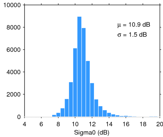
Figure 28. Histogram of science-valid sigma0 over oceans and lakes for 18/04/2020. The mean ( \mu ) and standard deviation ( \sigma ) are also shown. Note that values outside [4 20] dB are excluded from the histogram for the sake of readability but not from the computation of \mu and \sigma .
