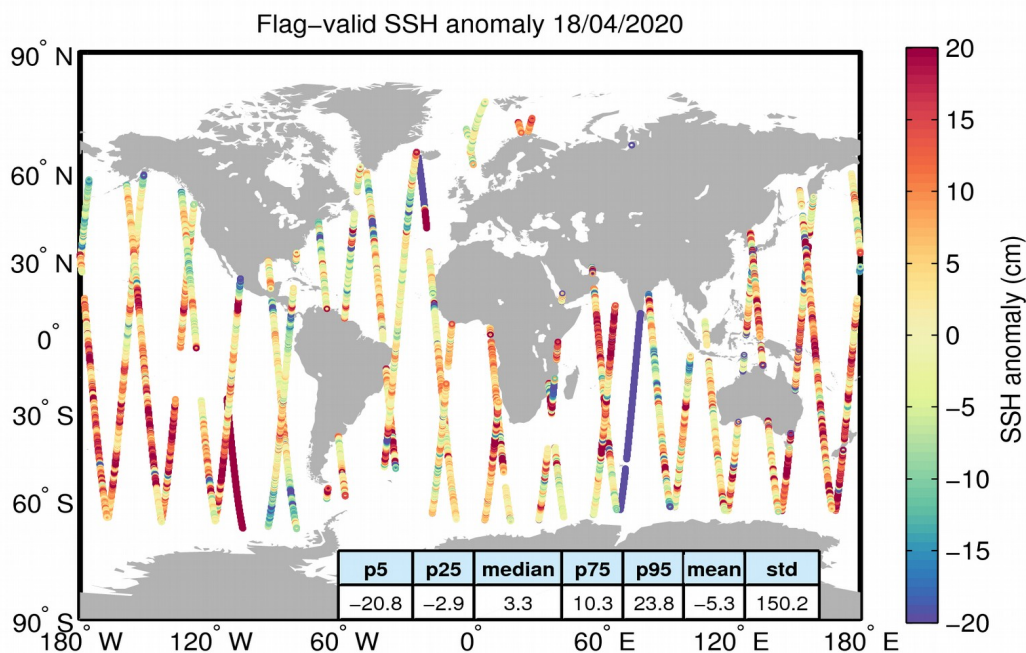
Figure 5. Geographical distribution of flag-valid 1-Hz SSH anomaly data over oceans and lakes for 18/04/2020. The statistical values shown in the table refer to the SSH anomaly in cm and are calculated over all measurements shown in the figure.
