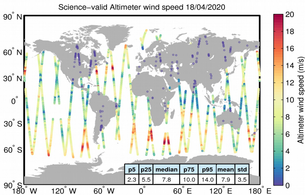
Figure 34. Geographical distribution of science-valid wind data over oceans and lakes for 18/04/2020. The statistical values shown in the table refer to the wind in m/s and are calculated over all measurements shown in the figure. Gray circles denote records that have been rejected based on the editing criteria described in Table 5.
