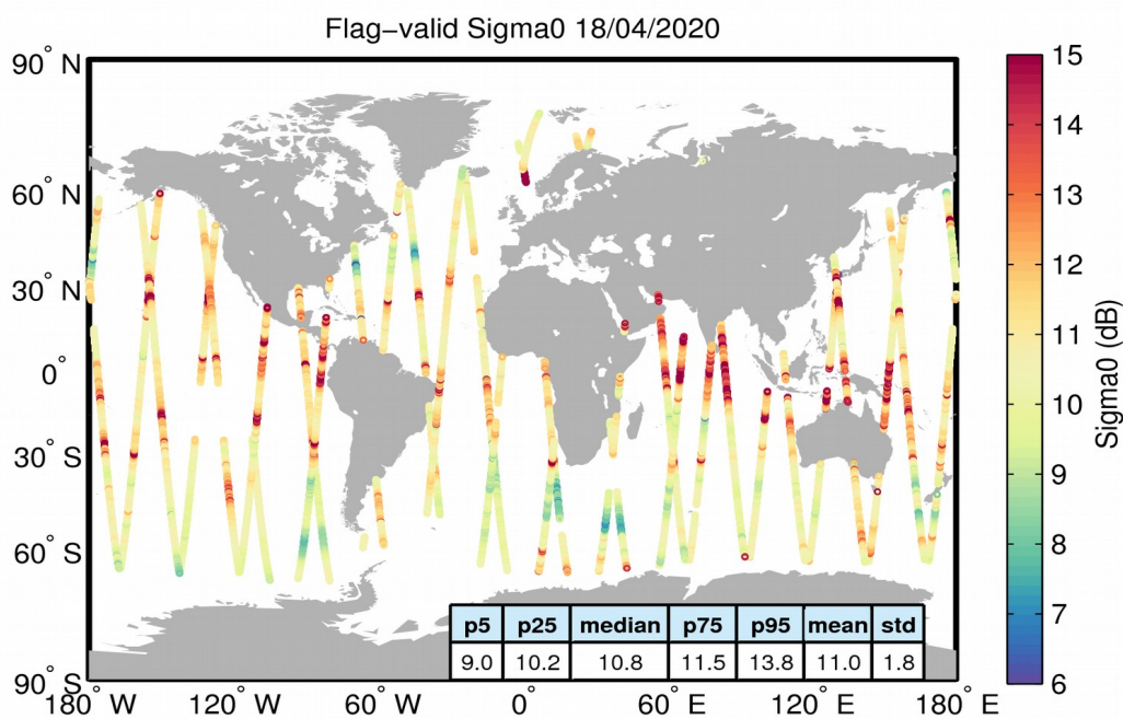
Figure 23. Geographical distribution of flag-valid sigma0 data over oceans and lakes for 18/04/2020. The statistical values shown in the table refer to the sigma0 in dB and are calculated over all measurements shown in the figure.
