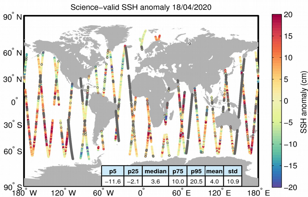
Figure 10. Geographical distribution of science-valid SSH anomaly data over oceans and lakes for 18/04/2020. The statistical values shown in the table refer to the SSH anomaly in cm and are calculated over all measurements shown in the figure. Gray circles denote records that have been rejected based on the editing criteria described in Table 2.
