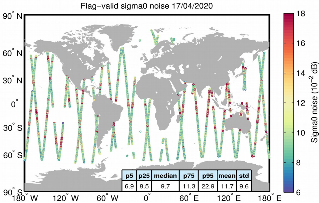
Figure 26. Geographical distribution of flag-valid 20-Hz sigma0 measurement noise over oceans and lakes for 17/04/2020. The statistical values shown in the table refer to the sigma0 noise and are calculated over all measurements shown in the figure.
