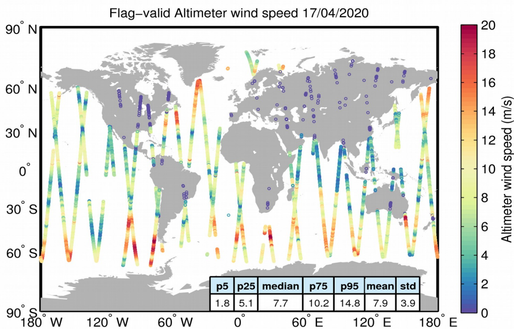
Figure 31. Geographical distribution of flag-valid wind data over oceans and lakes for 17/04/2020. The statistical values shown in the table refer to the wind in m/s and are calculated over all measurements shown in the figure.
