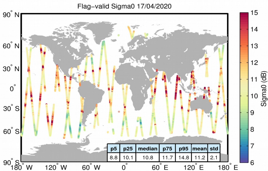
Figure 23. Geographical distribution of flag-valid sigma0 data over oceans and lakes for 17/04/2020. The statistical values shown in the table refer to the sigma0 in dB and are calculated over all measurements shown in the figure.
