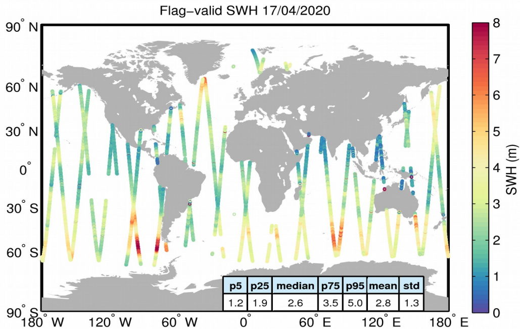
Figure 15. Geographical distribution of flag-valid SWH data over oceans and lakes for 17/04/2020. The statistical values shown in the table refer to the SWH in m and are calculated over all measurements shown in the figure.
