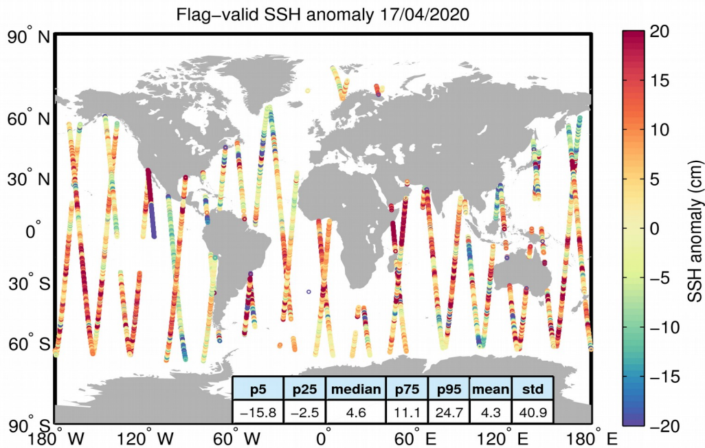
Figure 5. Geographical distribution of flag-valid 1-Hz SSH anomaly data over oceans and lakes for 17/04/2020. The statistical values shown in the table refer to the SSH anomaly in cm and are calculated over all measurements shown in the figure.
