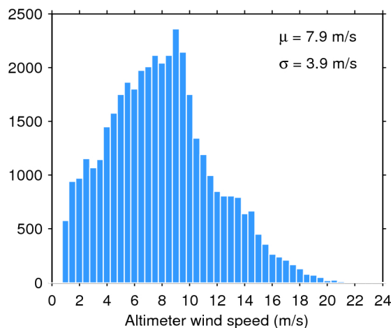
Figure 35. Histogram of science-valid wind over oceans and lakes for 17/04/2020. The mean ( \mu ) and standard deviation ( \sigma ) are also shown. Note that values larger than 24 m/s are excluded from the histogram for the sake of readability but not from the computation of \mu and \sigma .
