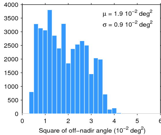
Figure 39. Histogram of flag-valid mispointing over oceans and lakes for 17/04/2020. The mean ( \mu ) and standard deviation ( \sigma ) are also shown. Note that values larger than 6 \cdot 10^{-2} \text{ deg}^2 are excluded from the histogram for the sake of readability but not from the computation of \mu and \sigma .
