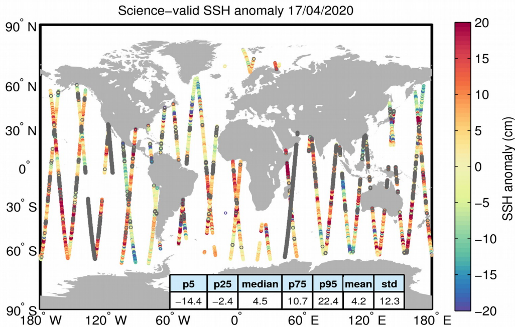
Figure 10. Geographical distribution of science-valid SSH anomaly data over oceans and lakes for 17/04/2020. The statistical values shown in the table refer to the SSH anomaly in cm and are calculated over all measurements shown in the figure. Gray circles denote records that have been rejected based on the editing criteria described in Table 2.
