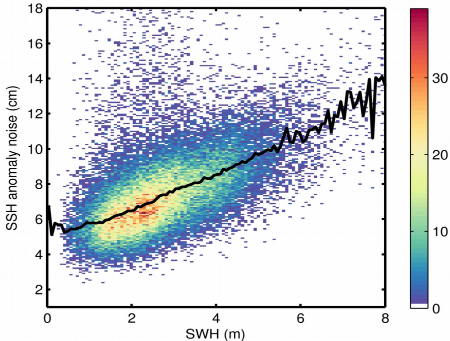
Figure 9. 2D histogram showing flag-valid SSH anomaly noise as a function of SWH for 17/04/2020. The black line denotes the median SSH anomaly noise as a function of SWH.
