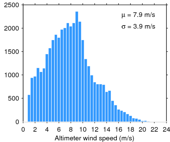
Figure 33. Histogram of flag-valid wind over oceans and lakes for 17/04/2020. The mean ( \mu ) and standard deviation ( \sigma ) are also shown. Note that values larger than 24 m/s are excluded from the histogram for the sake of readability but not from the computation of \mu and \sigma .
