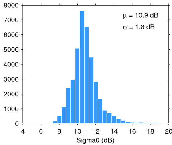
Figure 28. Histogram of science-valid sigma0 over oceans and lakes for 17/04/2020. The mean ( \mu ) and standard deviation ( \sigma ) are also shown. Note that values outside [4 20] dB are excluded from the histogram for the sake of readability but not from the computation of \mu and \sigma .
