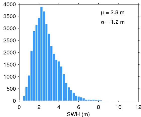
Figure 20. Histogram of science-valid SWH over oceans and lakes for 17/04/2020. The mean ( \mu ) and standard deviation ( \sigma ) are also shown. Note that values larger than 12 m are excluded from the histogram for the sake of readability but not from the computation of \mu and \sigma .
