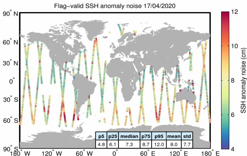
Figure 8. Geographical distribution of flag-valid 20-Hz SSH anomaly measurement noise over oceans and lakes for 17/04/2020. The statistical values shown in the table refer to the SSH anomaly noise and are calculated over all measurements shown in the figure.
