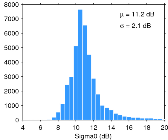
Figure 25. Histogram of flag-valid sigma0 over oceans and lakes for 17/04/2020. The mean ( \mu ) and standard deviation ( \sigma ) are also shown. Note that values outside [4 20] dB are excluded from the histogram for the sake of readability but not from the computation of \mu and \sigma .
