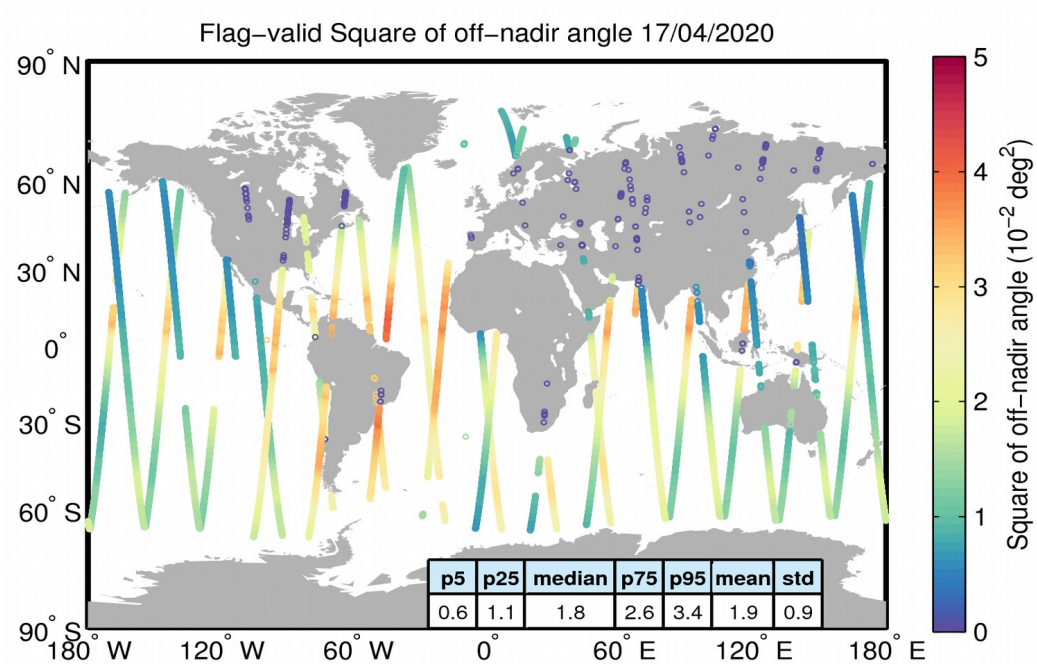
Figure 37. Geographical distribution of flag-valid mispointing data over oceans and lakes for 17/04/2020. The statistical values shown in the table refer to the mispointing in 10^{-2} \text{ deg}^2 and are calculated over all measurements shown in the figure.
