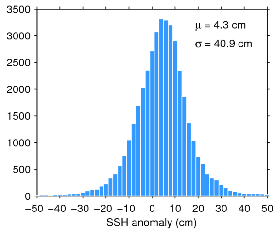
Figure 7. Histogram of flag-valid SSH anomaly over oceans and lakes for 17/04/2020. The mean ( \mu ) and standard deviation ( \sigma ) are also shown. Note that values outside [-50 50] cm are excluded from the histogram for the sake of readability but not from the computation of \mu and \sigma .
