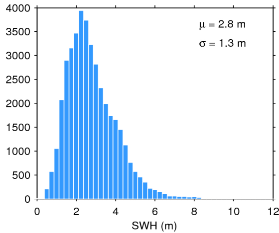
Figure 17. Histogram of flag-valid SWH over oceans and lakes for 17/04/2020. The mean ( \mu ) and standard deviation ( \sigma ) are also shown. Note that values larger than 12 m are excluded from the histogram for the sake of readability but not from the computation of \mu and \sigma .
