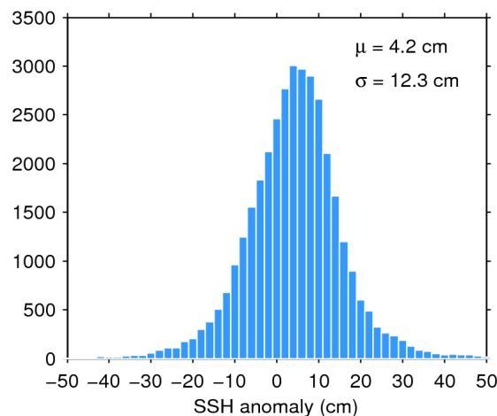
Figure 11. Histogram of science-valid SSH anomaly over oceans and lakes for 17/04/2020. The mean ( \mu ) and standard deviation ( \sigma ) are also shown. Note that values outside [-50 50] cm are excluded from the histogram for the sake of readability but not from the computation of \mu and \sigma .
