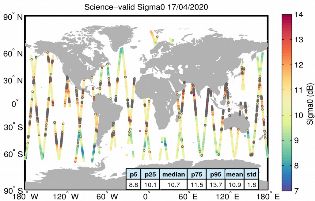
Figure 27. Geographical distribution of science-valid sigma0 data over oceans and lakes for 17/04/2020. The statistical values shown in the table refer to the sigma0 in dB and are calculated over all measurements shown in the figure. Gray circles denote records that have been rejected based on the editing criteria described in Table 4.
