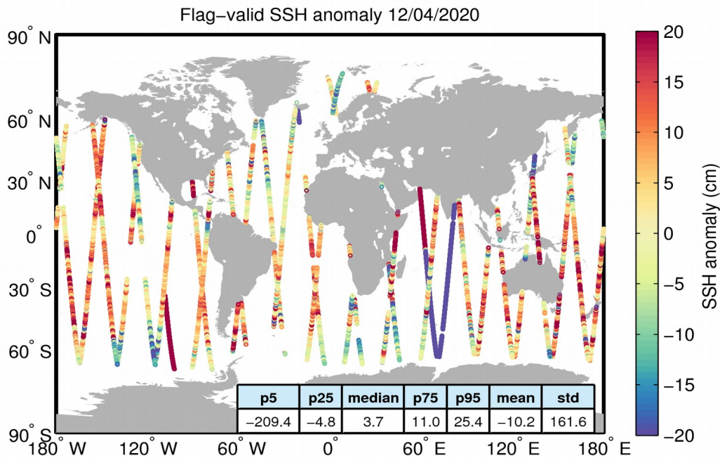
Figure 5. Geographical distribution of flag-valid 1-Hz SSH anomaly data over oceans and lakes for 12/04/2020. The statistical values shown in the table refer to the SSH anomaly in cm and are calculated over all measurements shown in the figure.
