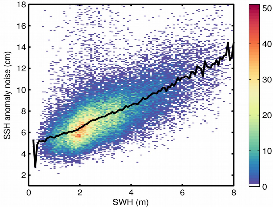
Figure 9. 2D histogram showing flag-valid SSH anomaly noise as a function of SWH for 12/04/2020. The black line denotes the median SSH anomaly noise as a function of SWH.
