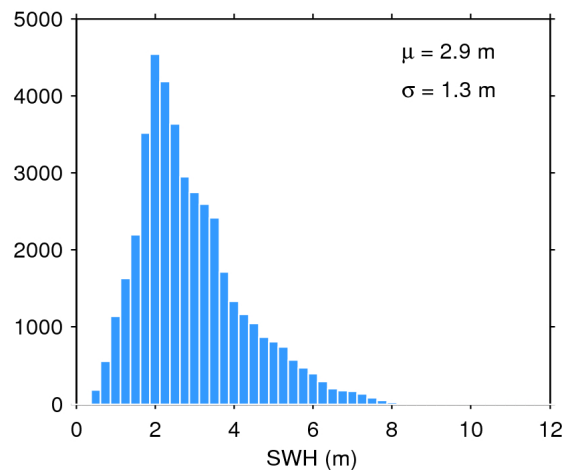
Figure 20. Histogram of science-valid SWH over oceans and lakes for 12/04/2020. The mean ( \mu ) and standard deviation ( \sigma ) are also shown. Note that values larger than 12 m are excluded from the histogram for the sake of readability but not from the computation of \mu and \sigma .
