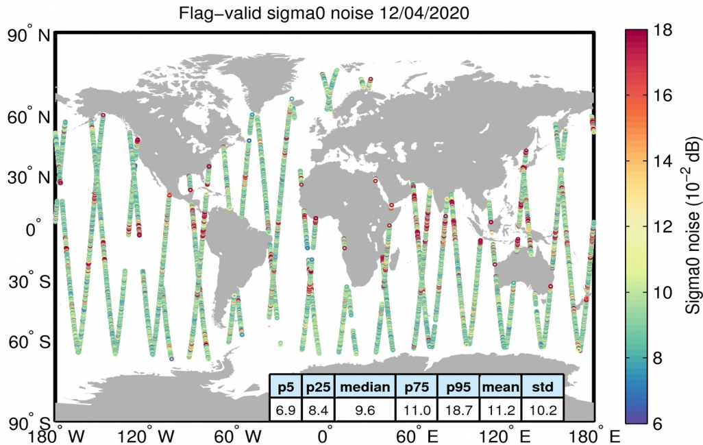
Figure 26. Geographical distribution of flag-valid 20-Hz sigma0 measurement noise over oceans and lakes for 12/04/2020. The statistical values shown in the table refer to the sigma0 noise and are calculated over all measurements shown in the figure.
