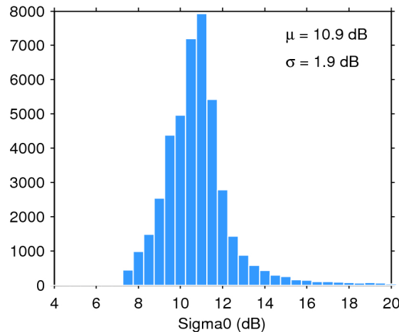
Figure 25. Histogram of flag-valid sigma0 over oceans and lakes for 12/04/2020. The mean ( \mu ) and standard deviation ( \sigma ) are also shown. Note that values outside [4 20] dB are excluded from the histogram for the sake of readability but not from the computation of \mu and \sigma .
