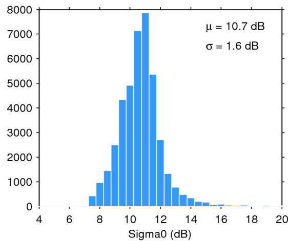
Figure 28. Histogram of science-valid sigma0 over oceans and lakes for 12/04/2020. The mean ( \mu ) and standard deviation ( \sigma ) are also shown. Note that values outside [4 20] dB are excluded from the histogram for the sake of readability but not from the computation of \mu and \sigma .
