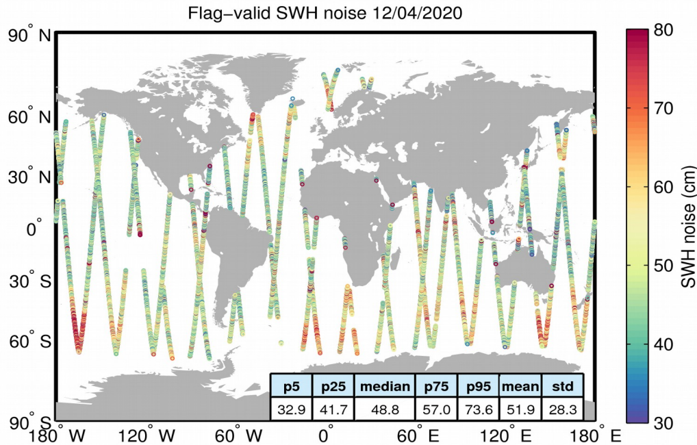
Figure 18. Geographical distribution of flag-valid 20-Hz SWH measurement noise over oceans and lakes for 12/04/2020. The statistical values shown in the figure refer to the SWH noise and are calculated over all measurements shown in the figure.
