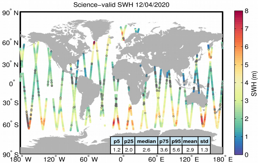
Figure 19. Geographical distribution of science-valid SWH data over oceans and lakes for 12/04/2020. The statistical values shown in the table refer to the SWH in m and are calculated over all measurements shown in the figure. Gray circles denote records that have been rejected based on the editing criteria described in Table 3.
