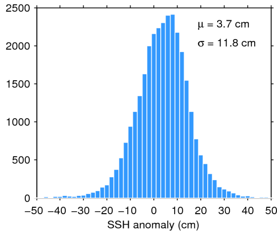
Figure 11. Histogram of science-valid SSH anomaly over oceans and lakes for 12/04/2020. The mean ( \mu ) and standard deviation ( \sigma ) are also shown. Note that values outside [-50 50] cm are excluded from the histogram for the sake of readability but not from the computation of \mu and \sigma .
