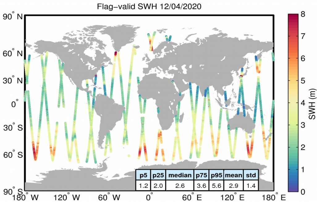
Figure 15. Geographical distribution of flag-valid SWH data over oceans and lakes for 12/04/2020. The statistical values shown in the table refer to the SWH in m and are calculated over all measurements shown in the figure.
