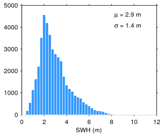
Figure 17. Histogram of flag-valid SWH over oceans and lakes for 12/04/2020. The mean ( \mu ) and standard deviation ( \sigma ) are also shown. Note that values larger than 12 m are excluded from the histogram for the sake of readability but not from the computation of \mu and \sigma .
