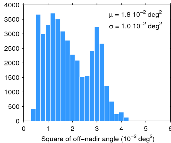
Figure 39. Histogram of flag-valid mispointing over oceans and lakes for 12/04/2020. The mean ( \mu ) and standard deviation ( \sigma ) are also shown. Note that values larger than 6 \cdot 10^{-2} \text{ deg}^2 are excluded from the histogram for the sake of readability but not from the computation of \mu and \sigma .
