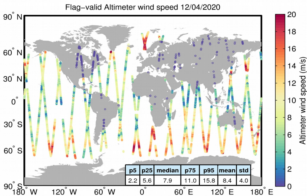
Figure 31. Geographical distribution of flag-valid wind data over oceans and lakes for 12/04/2020. The statistical values shown in the table refer to the wind in m/s and are calculated over all measurements shown in the figure.
