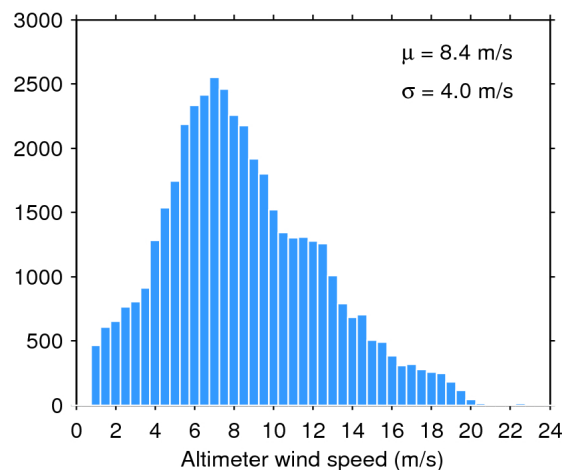
Figure 35. Histogram of science-valid wind over oceans and lakes for 12/04/2020. The mean ( \mu ) and standard deviation ( \sigma ) are also shown. Note that values larger than 24 m/s are excluded from the histogram for the sake of readability but not from the computation of \mu and \sigma .
