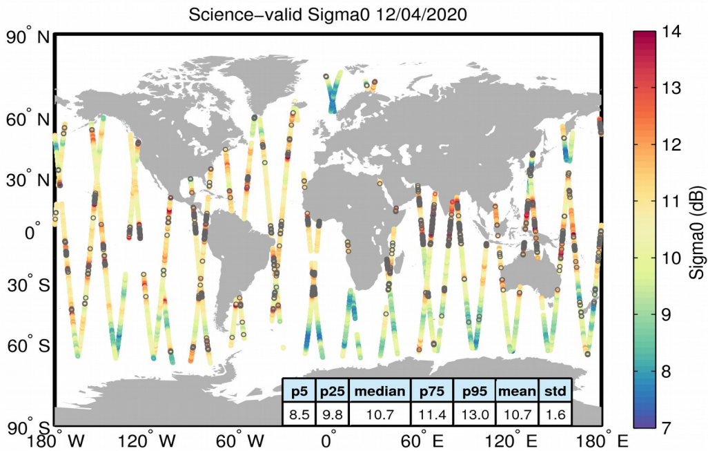
Figure 27. Geographical distribution of science-valid sigma0 data over oceans and lakes for 12/04/2020. The statistical values shown in the table refer to the sigma0 in dB and are calculated over all measurements shown in the figure. Gray circles denote records that have been rejected based on the editing criteria described in Table 4.
