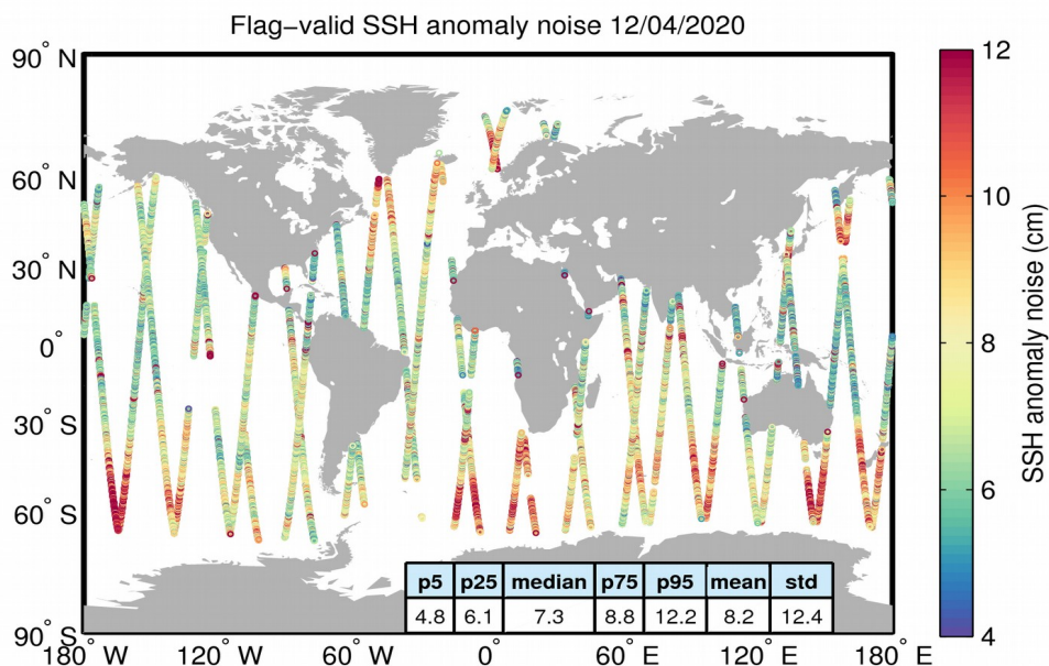
Figure 8. Geographical distribution of flag-valid 20-Hz SSH anomaly measurement noise over oceans and lakes for 12/04/2020. The statistical values shown in the table refer to the SSH anomaly noise and are calculated over all measurements shown in the figure.
