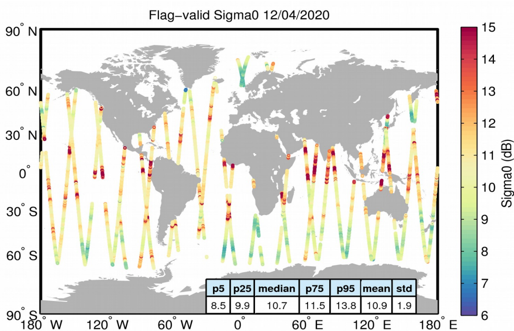
Figure 23. Geographical distribution of flag-valid sigma0 data over oceans and lakes for 12/04/2020. The statistical values shown in the table refer to the sigma0 in dB and are calculated over all measurements shown in the figure.
