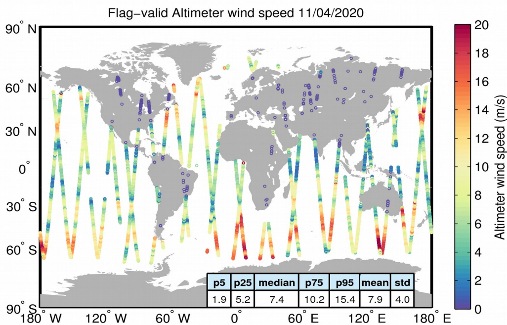
Figure 31. Geographical distribution of flag-valid wind data over oceans and lakes for 11/04/2020. The statistical values shown in the table refer to the wind in m/s and are calculated over all measurements shown in the figure.
