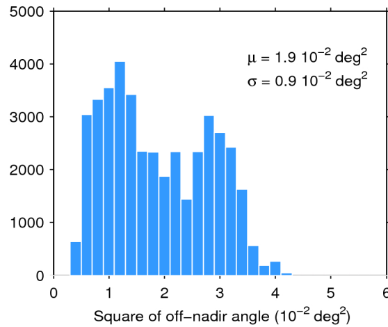
Figure 39. Histogram of flag-valid mispointing over oceans and lakes for 11/04/2020. The mean ( \mu ) and standard deviation ( \sigma ) are also shown. Note that values larger than 6 \cdot 10^{-2} \text{ deg}^2 are excluded from the histogram for the sake of readability but not from the computation of \mu and \sigma .
