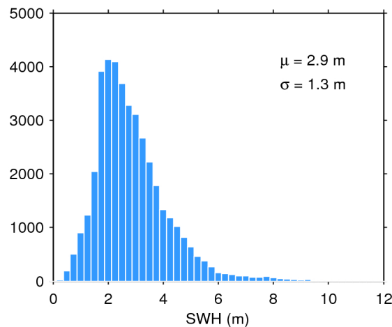
Figure 17. Histogram of flag-valid SWH over oceans and lakes for 11/04/2020. The mean ( \mu ) and standard deviation ( \sigma ) are also shown. Note that values larger than 12 m are excluded from the histogram for the sake of readability but not from the computation of \mu and \sigma .
