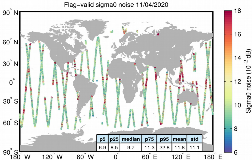
Figure 26. Geographical distribution of flag-valid 20-Hz sigma0 measurement noise over oceans and lakes for 11/04/2020. The statistical values shown in the table refer to the sigma0 noise and are calculated over all measurements shown in the figure.
