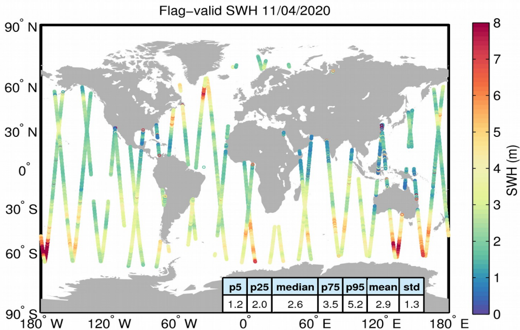
Figure 15. Geographical distribution of flag-valid SWH data over oceans and lakes for 11/04/2020. The statistical values shown in the table refer to the SWH in m and are calculated over all measurements shown in the figure.
