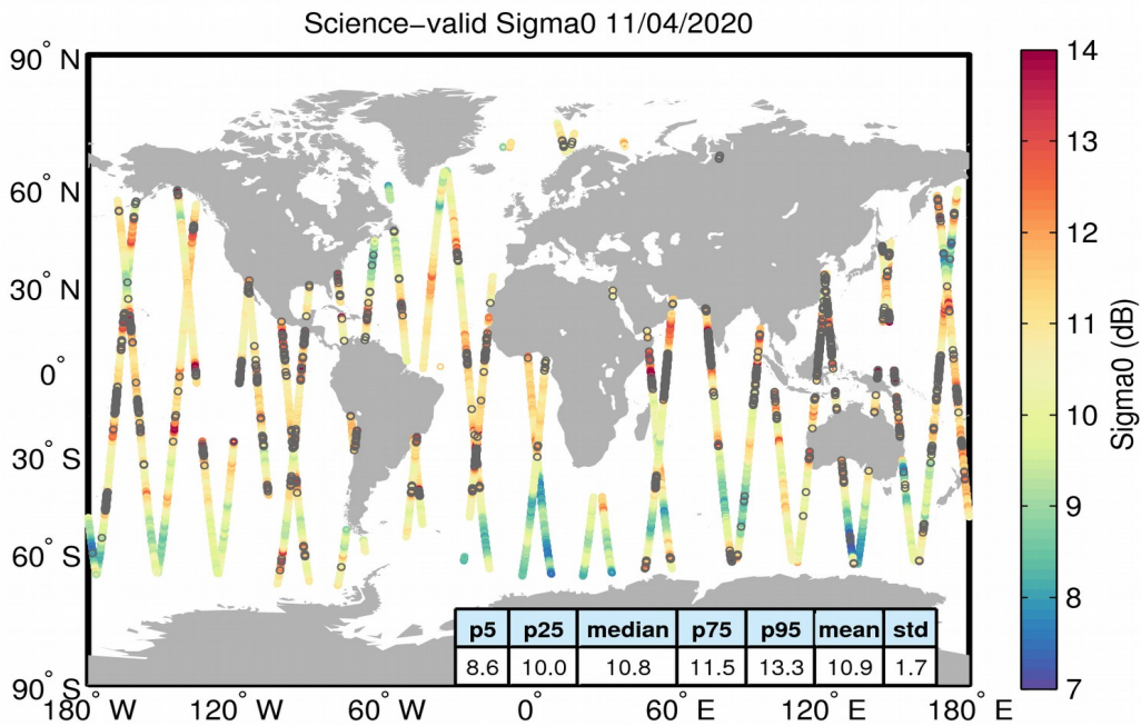
Figure 27. Geographical distribution of science-valid sigma0 data over oceans and lakes for 11/04/2020. The statistical values shown in the table refer to the sigma0 in dB and are calculated over all measurements shown in the figure. Gray circles denote records that have been rejected based on the editing criteria described in Table 4.
