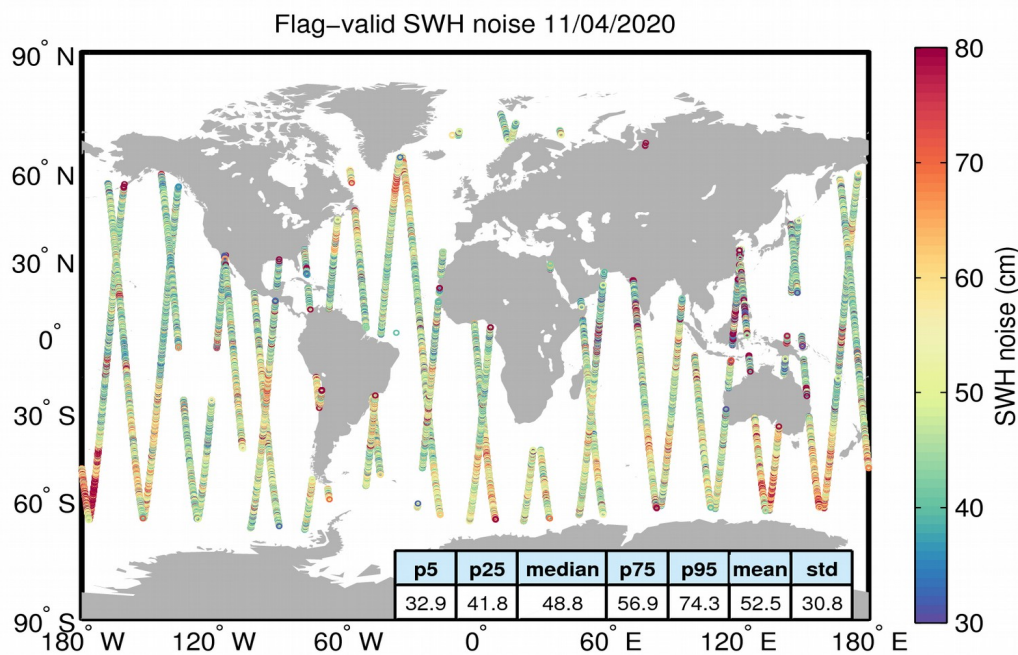
Figure 18. Geographical distribution of flag-valid 20-Hz SWH measurement noise over oceans and lakes for 11/04/2020. The statistical values shown in the figure refer to the SWH noise and are calculated over all measurements shown in the figure.
