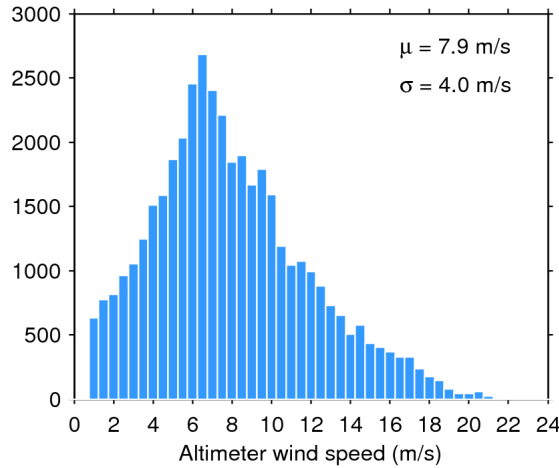
Figure 33. Histogram of flag-valid wind over oceans and lakes for 11/04/2020. The mean ( \mu ) and standard deviation ( \sigma ) are also shown. Note that values larger than 24 m/s are excluded from the histogram for the sake of readability but not from the computation of \mu and \sigma .
