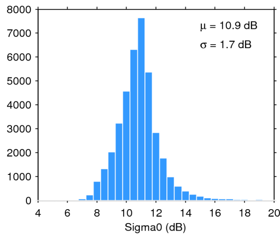
Figure 28. Histogram of science-valid sigma0 over oceans and lakes for 11/04/2020. The mean ( \mu ) and standard deviation ( \sigma ) are also shown. Note that values outside [4 20] dB are excluded from the histogram for the sake of readability but not from the computation of \mu and \sigma .
