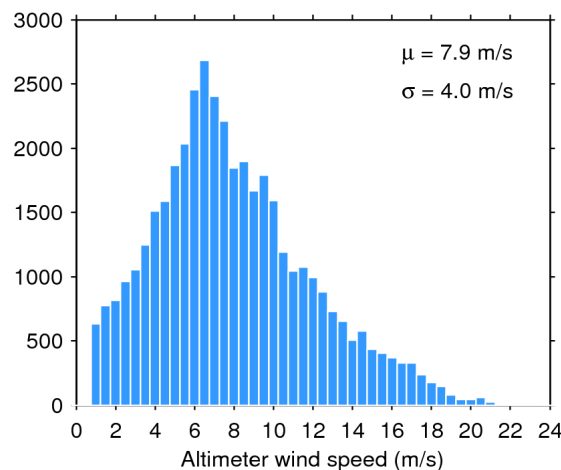
Figure 35. Histogram of science-valid wind over oceans and lakes for 11/04/2020. The mean ( \mu ) and standard deviation ( \sigma ) are also shown. Note that values larger than 24 m/s are excluded from the histogram for the sake of readability but not from the computation of \mu and \sigma .
