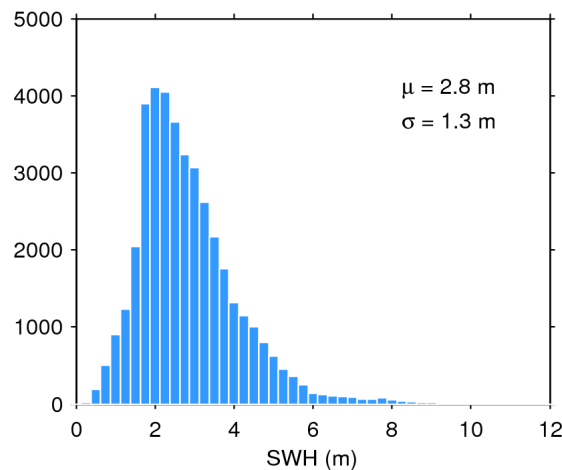
Figure 20. Histogram of science-valid SWH over oceans and lakes for 11/04/2020. The mean ( \mu ) and standard deviation ( \sigma ) are also shown. Note that values larger than 12 m are excluded from the histogram for the sake of readability but not from the computation of \mu and \sigma .
