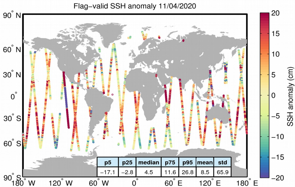
Figure 5. Geographical distribution of flag-valid 1-Hz SSH anomaly data over oceans and lakes for 11/04/2020. The statistical values shown in the table refer to the SSH anomaly in cm and are calculated over all measurements shown in the figure.
