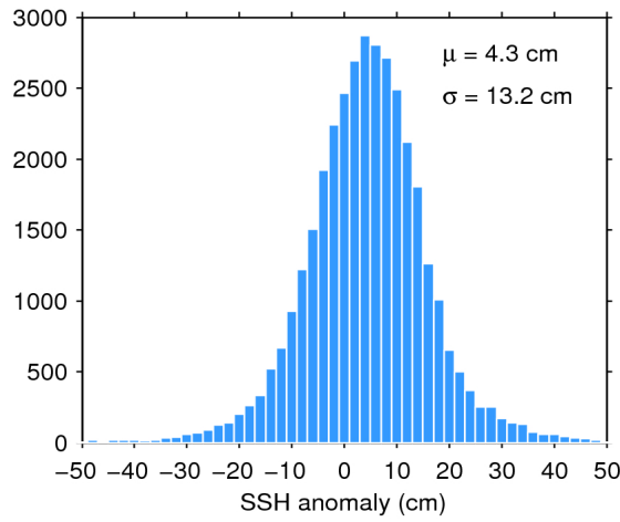
Figure 11. Histogram of science-valid SSH anomaly over oceans and lakes for 11/04/2020. The mean ( \mu ) and standard deviation ( \sigma ) are also shown. Note that values outside [-50 50] cm are excluded from the histogram for the sake of readability but not from the computation of \mu and \sigma .
