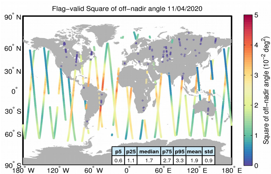
Figure 37. Geographical distribution of flag-valid mispointing data over oceans and lakes for 11/04/2020. The statistical values shown in the table refer to the mispointing in 10^{-2} \text{ deg}^2 and are calculated over all measurements shown in the figure.
