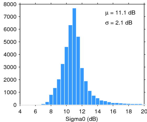
Figure 25. Histogram of flag-valid sigma0 over oceans and lakes for 11/04/2020. The mean ( \mu ) and standard deviation ( \sigma ) are also shown. Note that values outside [4 20] dB are excluded from the histogram for the sake of readability but not from the computation of \mu and \sigma .
