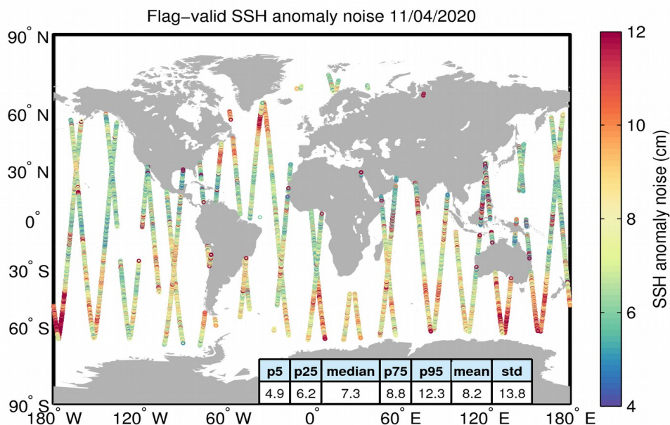
Figure 8. Geographical distribution of flag-valid 20-Hz SSH anomaly measurement noise over oceans and lakes for 11/04/2020. The statistical values shown in the table refer to the SSH anomaly noise and are calculated over all measurements shown in the figure.
