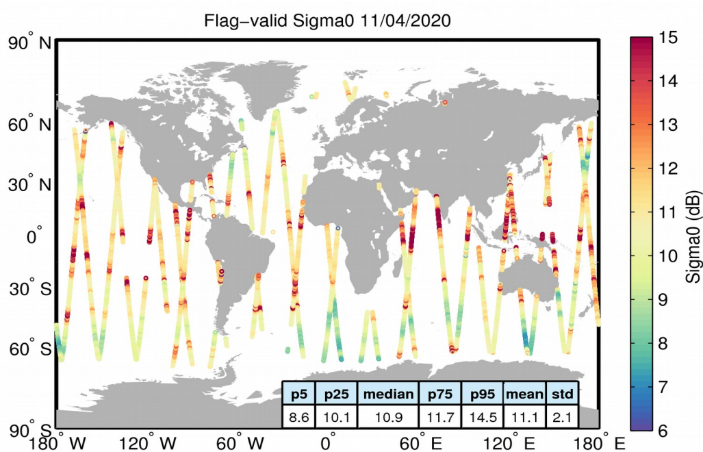
Figure 23. Geographical distribution of flag-valid sigma0 data over oceans and lakes for 11/04/2020. The statistical values shown in the table refer to the sigma0 in dB and are calculated over all measurements shown in the figure.
