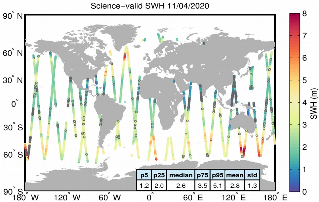
Figure 19. Geographical distribution of science-valid SWH data over oceans and lakes for 11/04/2020. The statistical values shown in the table refer to the SWH in m and are calculated over all measurements shown in the figure. Gray circles denote records that have been rejected based on the editing criteria described in Table 3.
