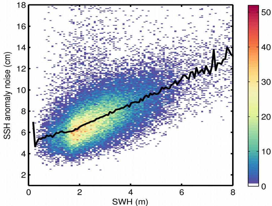
Figure 9. 2D histogram showing flag-valid SSH anomaly noise as a function of SWH for 11/04/2020. The black line denotes the median SSH anomaly noise as a function of SWH.
