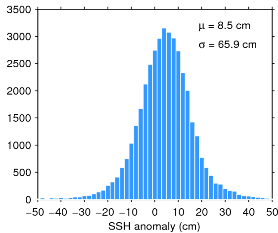
Figure 7. Histogram of flag-valid SSH anomaly over oceans and lakes for 11/04/2020. The mean ( \mu ) and standard deviation ( \sigma ) are also shown. Note that values outside [-50 50] cm are excluded from the histogram for the sake of readability but not from the computation of \mu and \sigma .
