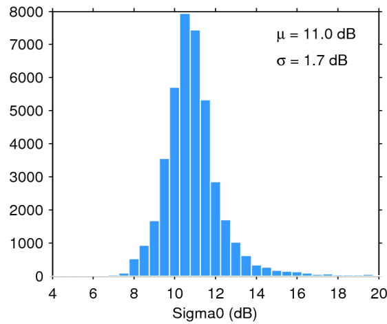
Figure 28. Histogram of science-valid sigma0 over oceans and lakes for 10/04/2020. The mean ( \mu ) and standard deviation ( \sigma ) are also shown. Note that values outside [4 20] dB are excluded from the histogram for the sake of readability but not from the computation of \mu and \sigma .
