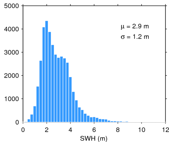
Figure 20. Histogram of science-valid SWH over oceans and lakes for 10/04/2020. The mean ( \mu ) and standard deviation ( \sigma ) are also shown. Note that values larger than 12 m are excluded from the histogram for the sake of readability but not from the computation of \mu and \sigma .
