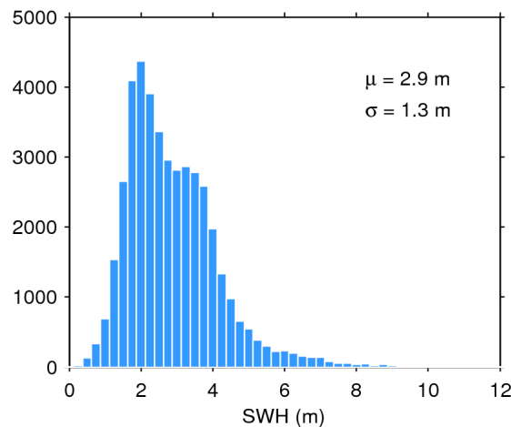
Figure 17. Histogram of flag-valid SWH over oceans and lakes for 10/04/2020. The mean ( \mu ) and standard deviation ( \sigma ) are also shown. Note that values larger than 12 m are excluded from the histogram for the sake of readability but not from the computation of \mu and \sigma .
