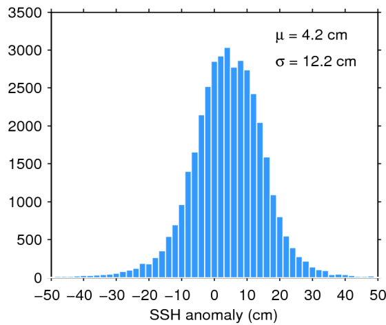
Figure 11. Histogram of science-valid SSH anomaly over oceans and lakes for 10/04/2020. The mean ( \mu ) and standard deviation ( \sigma ) are also shown. Note that values outside [-50 50] cm are excluded from the histogram for the sake of readability but not from the computation of \mu and \sigma .
