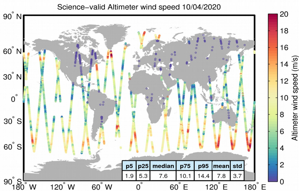
Figure 34. Geographical distribution of science-valid wind data over oceans and lakes for 10/04/2020. The statistical values shown in the table refer to the wind in m/s and are calculated over all measurements shown in the figure. Gray circles denote records that have been rejected based on the editing criteria described in Table 5.
