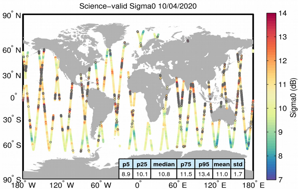
Figure 27. Geographical distribution of science-valid sigma0 data over oceans and lakes for 10/04/2020. The statistical values shown in the table refer to the sigma0 in dB and are calculated over all measurements shown in the figure. Gray circles denote records that have been rejected based on the editing criteria described in Table 4.
