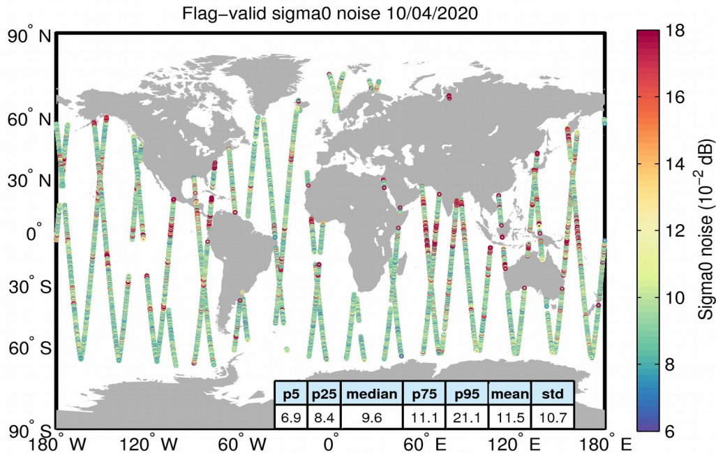
Figure 26. Geographical distribution of flag-valid 20-Hz sigma0 measurement noise over oceans and lakes for 10/04/2020. The statistical values shown in the table refer to the sigma0 noise and are calculated over all measurements shown in the figure.
