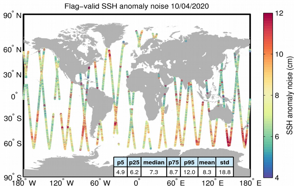
Figure 8. Geographical distribution of flag-valid 20-Hz SSH anomaly measurement noise over oceans and lakes for 10/04/2020. The statistical values shown in the table refer to the SSH anomaly noise and are calculated over all measurements shown in the figure.
