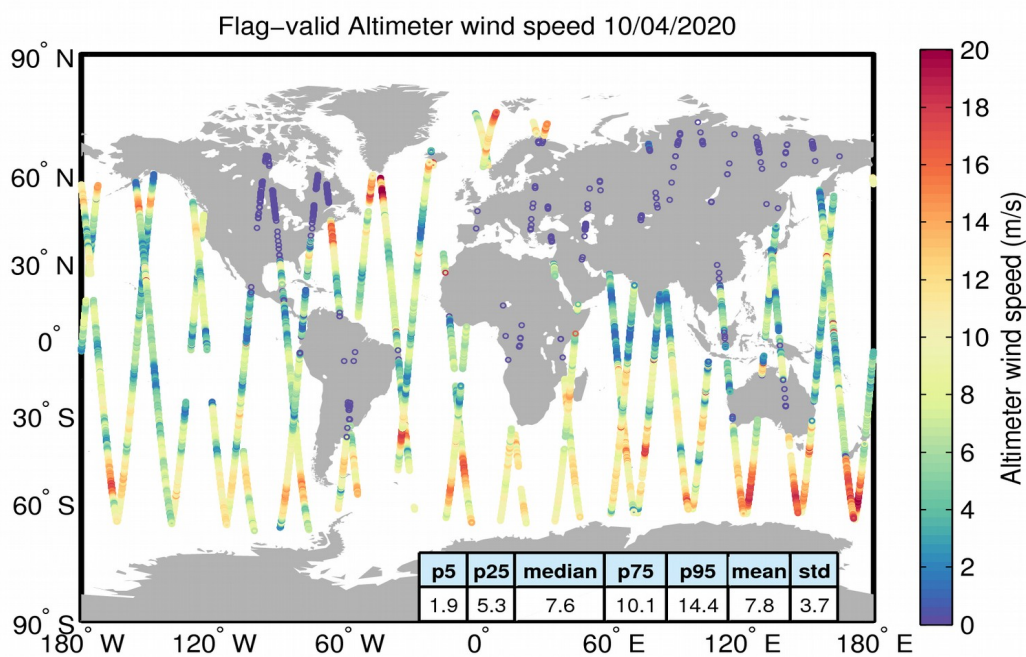
Figure 31. Geographical distribution of flag-valid wind data over oceans and lakes for 10/04/2020. The statistical values shown in the table refer to the wind in m/s and are calculated over all measurements shown in the figure.
