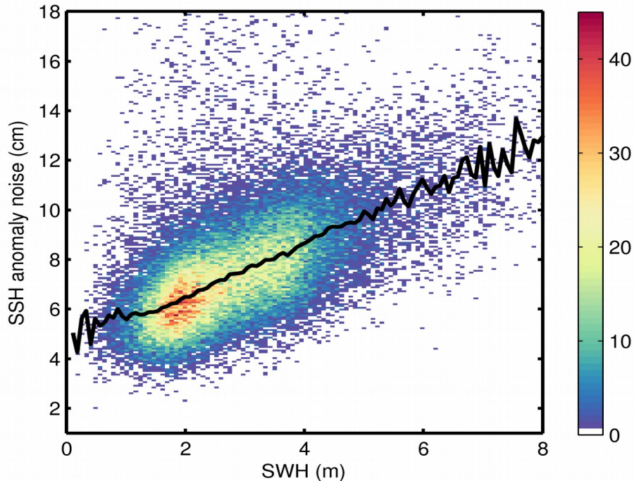
Figure 9. 2D histogram showing flag-valid SSH anomaly noise as a function of SWH for 10/04/2020. The black line denotes the median SSH anomaly noise as a function of SWH.
