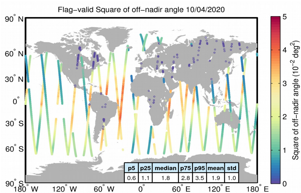
Figure 37. Geographical distribution of flag-valid mispointing data over oceans and lakes for 10/04/2020. The statistical values shown in the table refer to the mispointing in 10^{-2} deg 2 and are calculated over all measurements shown in the figure.
