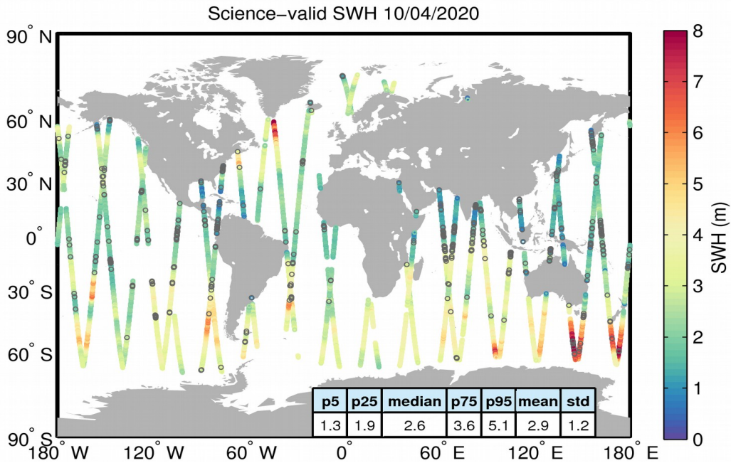
Figure 19. Geographical distribution of science-valid SWH data over oceans and lakes for 10/04/2020. The statistical values shown in the table refer to the SWH in m and are calculated over all measurements shown in the figure. Gray circles denote records that have been rejected based on the editing criteria described in Table 3.
