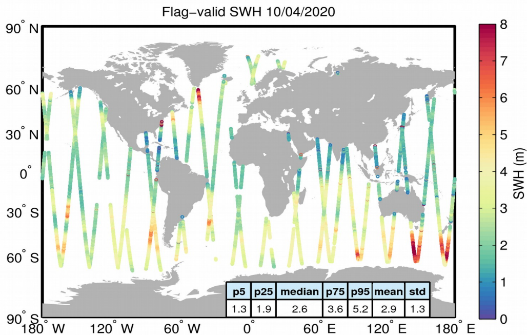
Figure 15. Geographical distribution of flag-valid SWH data over oceans and lakes for 10/04/2020. The statistical values shown in the table refer to the SWH in m and are calculated over all measurements shown in the figure.
