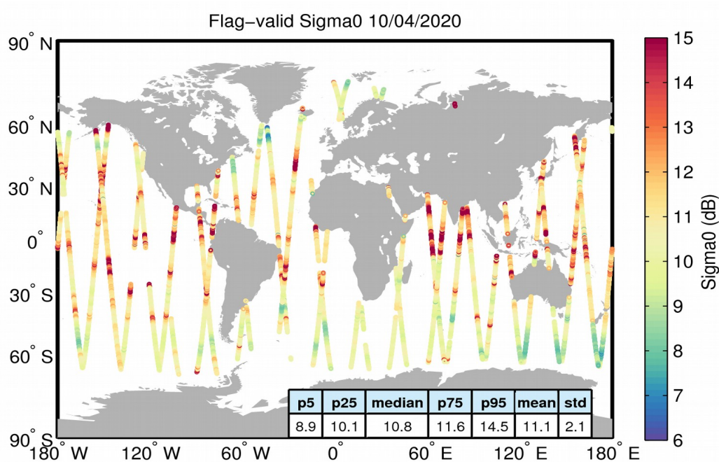
Figure 23. Geographical distribution of flag-valid sigma0 data over oceans and lakes for 10/04/2020. The statistical values shown in the table refer to the sigma0 in dB and are calculated over all measurements shown in the figure.
