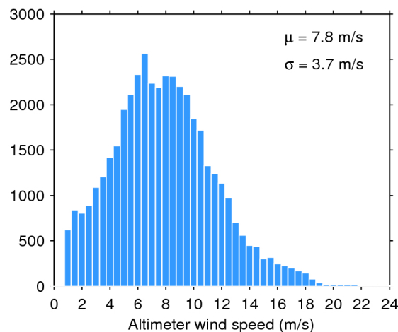
Figure 35. Histogram of science-valid wind over oceans and lakes for 10/04/2020. The mean ( \mu ) and standard deviation ( \sigma ) are also shown. Note that values larger than 24 m/s are excluded from the histogram for the sake of readability but not from the computation of \mu and \sigma .
