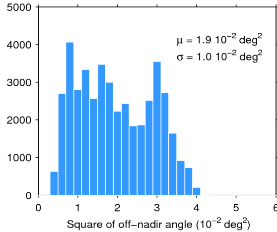
Figure 39. Histogram of flag-valid mispointing over oceans and lakes for 10/04/2020. The mean ( \mu ) and standard deviation ( \sigma ) are also shown. Note that values larger than 6 \cdot 10^{-2} \text{ deg}^2 are excluded from the histogram for the sake of readability but not from the computation of \mu and \sigma .
