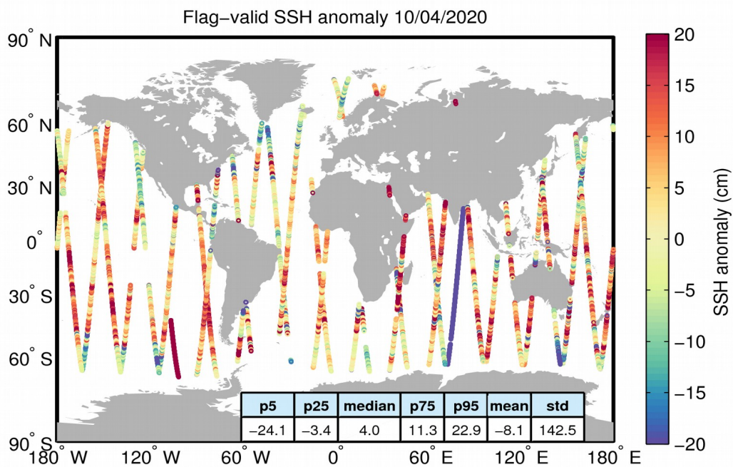
Figure 5. Geographical distribution of flag-valid 1-Hz SSH anomaly data over oceans and lakes for 10/04/2020. The statistical values shown in the table refer to the SSH anomaly in cm and are calculated over all measurements shown in the figure.
