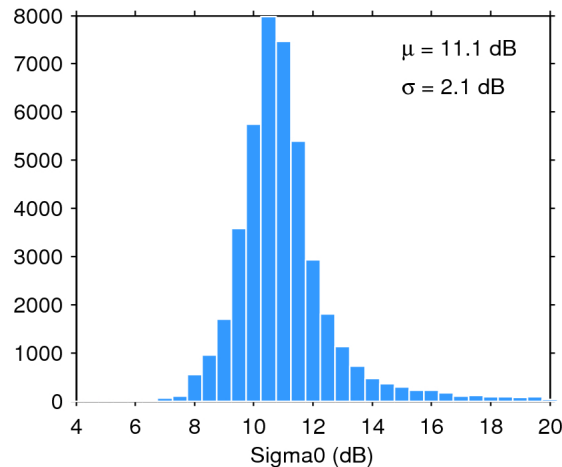
Figure 25. Histogram of flag-valid sigma0 over oceans and lakes for 10/04/2020. The mean ( \mu ) and standard deviation ( \sigma ) are also shown. Note that values outside [4 20] dB are excluded from the histogram for the sake of readability but not from the computation of \mu and \sigma .
